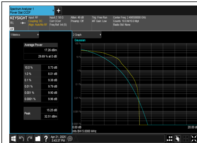
Band41-5MHz-16QAM-39675-1RB#0-PASS
