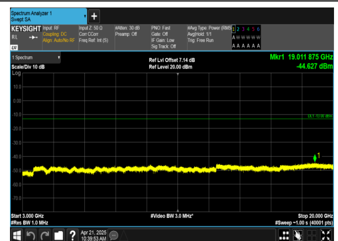
Band66-15MHz-16QAM-132047-75RB#0-3000~20000-PASS
