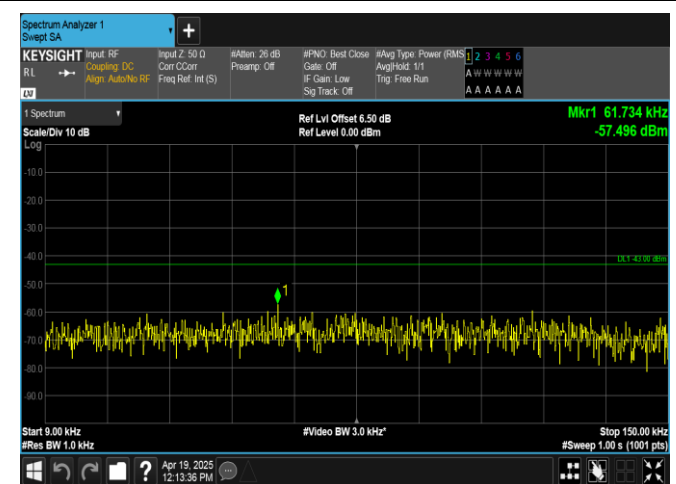
Band66-15MHz-QPSK-132597-1RB#74-0.009~0.15-PASS
