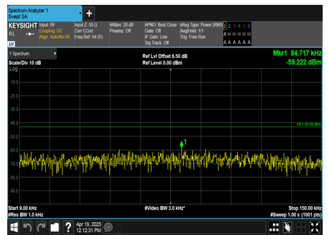
Band66-15MHz-16QAM-132597-1RB#0-0.009~0.15-PASS
