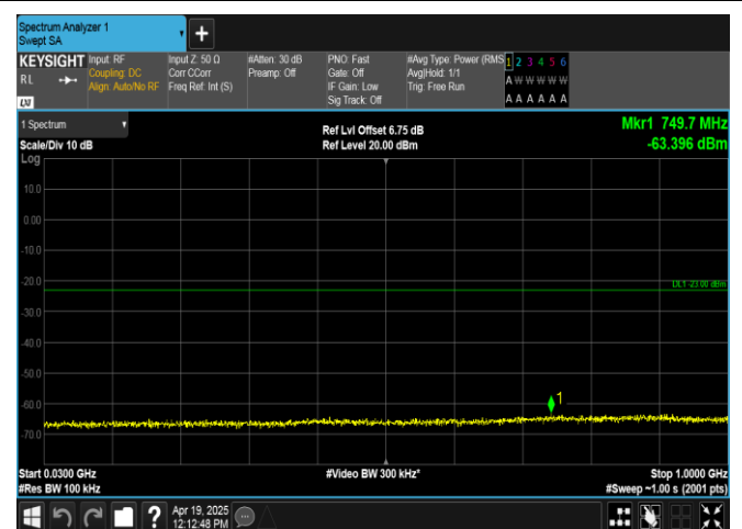
Band66-15MHz-16QAM-132597-1RB#0-30~1000-PASS
