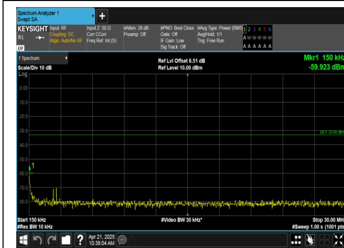
Band66-15MHz-16QAM-132047-75RB#0-0.15~30-PASS
