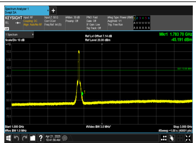
Band66-15MHz-16QAM-132322-75RB#0-1000~3000-PASS
