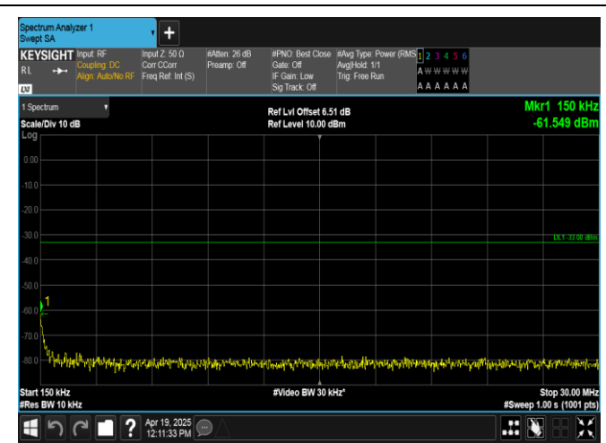
Band66-15MHz-QPSK-132597-1RB#0-0.15~30-PASS
