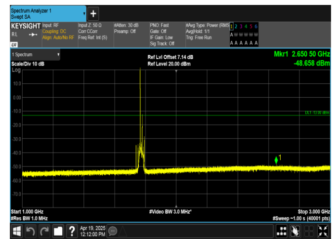
Band66-15MHz-QPSK-132597-1RB#0-1000~3000-PASS
