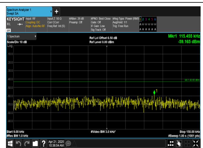
Band66-15MHz-16QAM-132047-75RB#0-0.009~0.15-PASS
