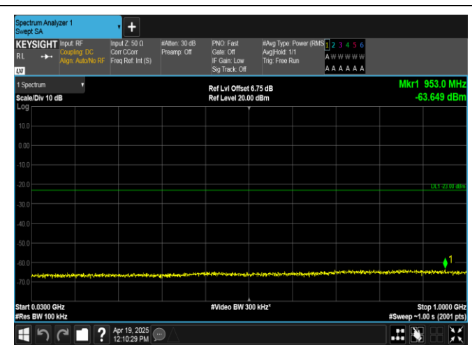
Band66-15MHz-16QAM-132322-1RB#74-30~1000-PASS
