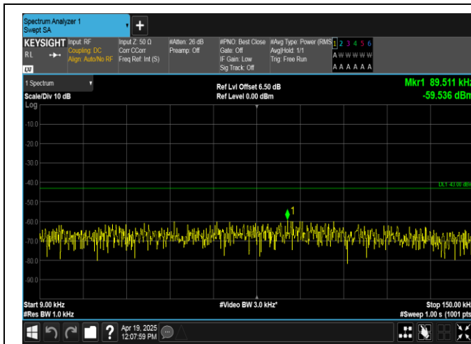
Band66-15MHz-16QAM-132322-1RB#0-0.009~0.15-PASS
