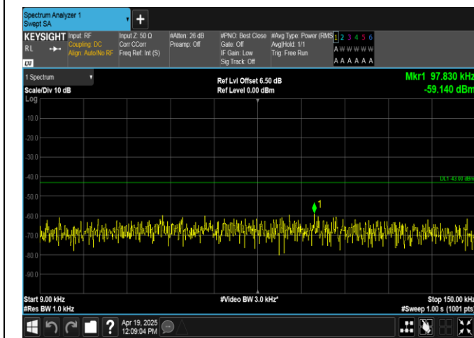
Band66-15MHz-QPSK-132322-1RB#74-0.009~0.15-PASS
