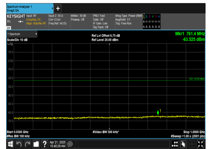
Band66-15MHz-QPSK-132322-75RB#0-30~1000-PASS
