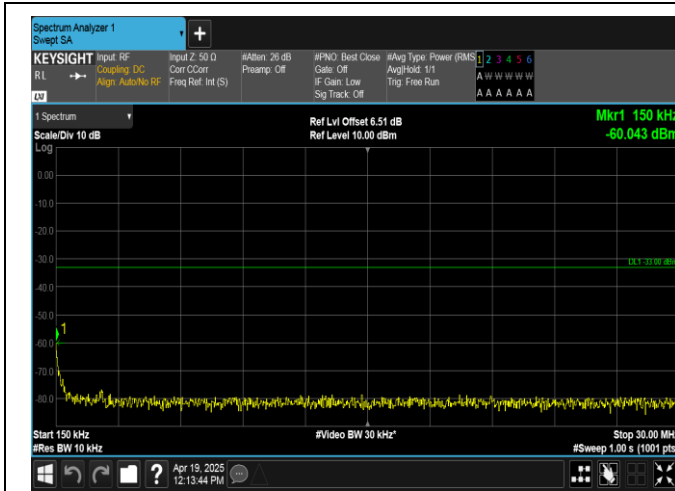
Band66-15MHz-QPSK-132597-1RB#74-0.15~30-PASS
