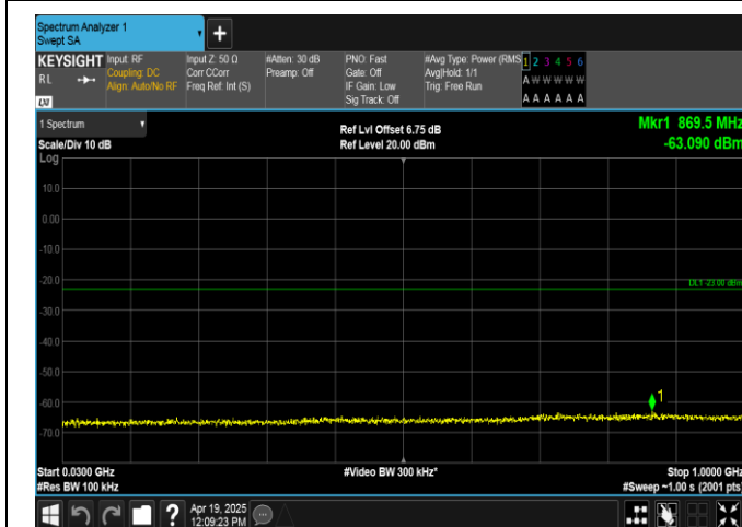
Band66-15MHz-QPSK-132322-1RB#74-30~1000-PASS
