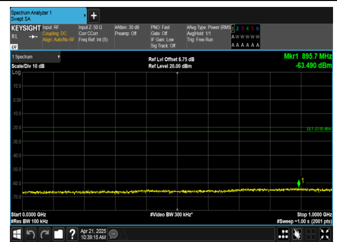
Band66-15MHz-16QAM-132047-75RB#0-30~1000-PASS
