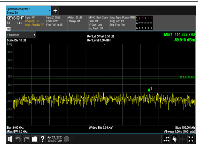
Band66-15MHz-QPSK-132322-75RB#0-0.009~0.15-PASS
