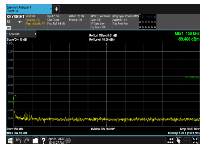
Band66-15MHz-16QAM-132322-75RB#0-0.15~30-PASS
