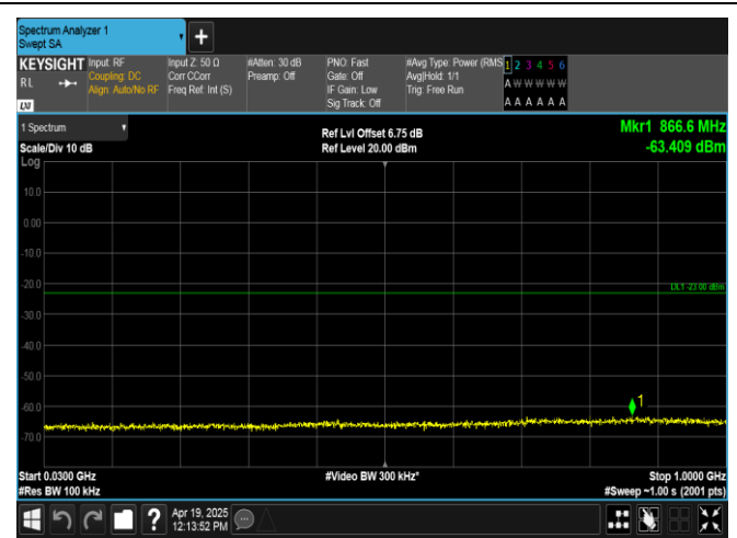
Band66-15MHz-QPSK-132597-1RB#74-30~1000-PASS
