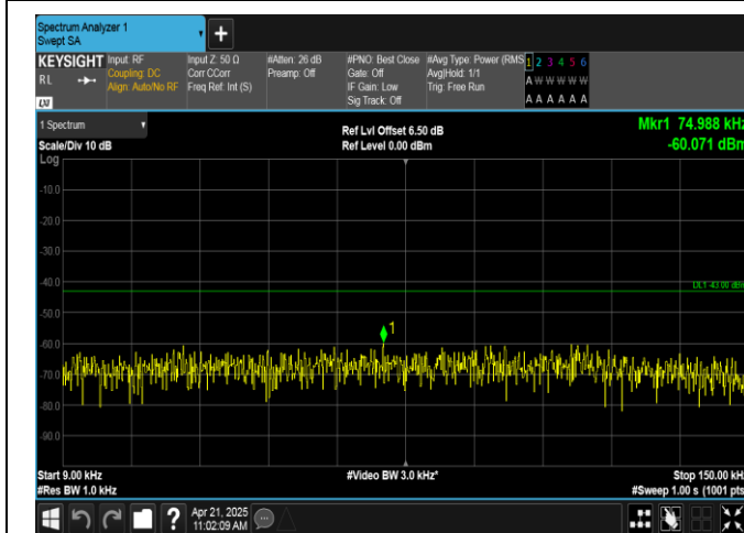
Band66-20MHz-QPSK-132072-100RB#0-0.009~0.15-PASS
