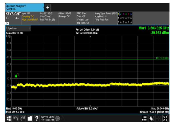
Band66-15MHz-16QAM-132322-1RB#74-3000~20000-PASS
