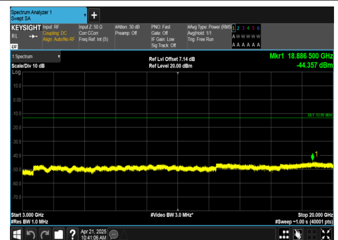
Band66-15MHz-QPSK-132322-75RB#0-3000~20000-PASS
