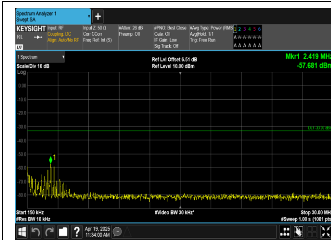
Band66-10MHz-16QAM-132322-1RB#49-0.15~30-PASS
