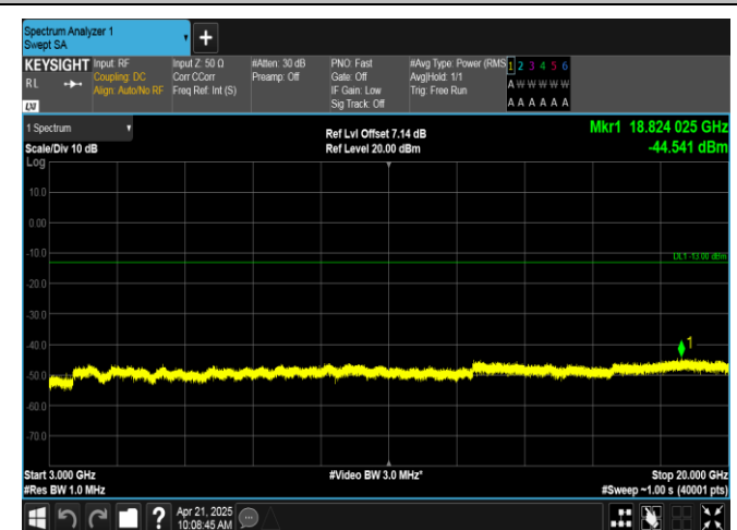
Band66-10MHz-16QAM-132022-50RB#0-3000~20000-PASS
