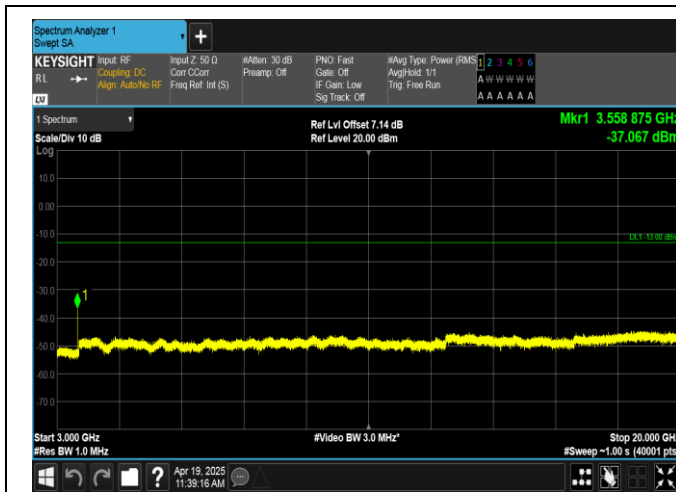
Band66-10MHz-16QAM-132622-1RB#49-3000~20000-PASS
