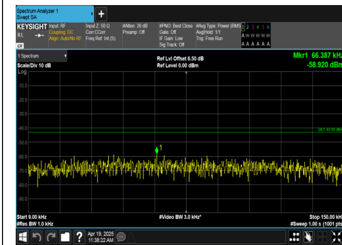
Band66-10MHz-16QAM-132622-1RB#49-0.009~0.15-PASS
