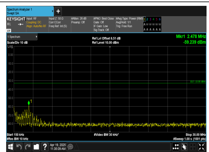
Band66-10MHz-QPSK-132622-1RB#0-0.15~30-PASS
