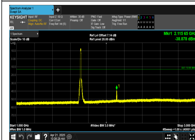
Band66-10MHz-16QAM-132022-50RB#0-1000~3000-PASS
