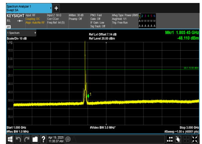
Band66-10MHz-QPSK-132622-1RB#0-1000~3000-PASS
