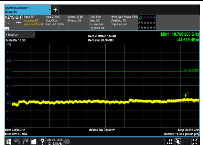
Band66-10MHz-16QAM-132622-50RB#0-3000~20000-PASS
