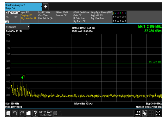
Band66-10MHz-16QAM-132622-1RB#49-0.15~30-PASS
