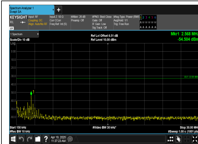
Band66-10MHz-QPSK-132622-1RB#49-0.15~30-PASS
