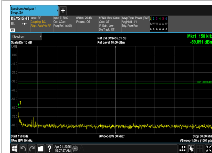
Band66-10MHz-16QAM-132022-50RB#0-0.15~30-PASS
