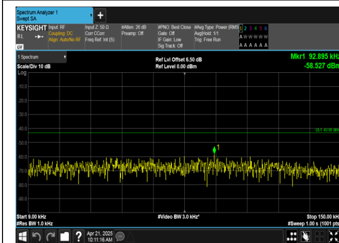
Band66-10MHz-QPSK-132622-50RB#0-0.009~0.15-PASS
