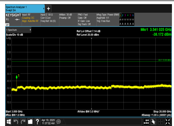
Band66-10MHz-16QAM-132622-1RB#0-3000~20000-PASS
