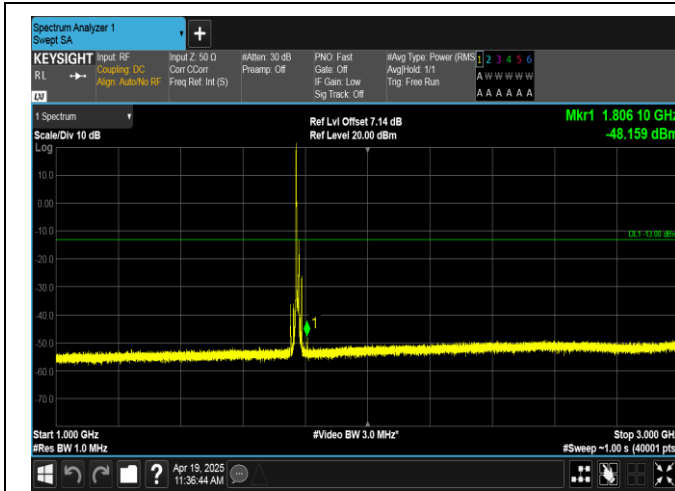
Band66-10MHz-16QAM-132622-1RB#0-1000~3000-PASS
