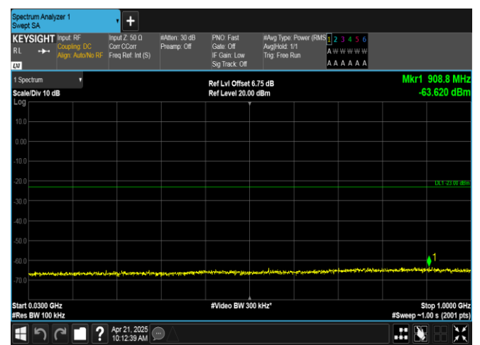
Band66-10MHz-16QAM-132622-50RB#0-30~1000-PASS
