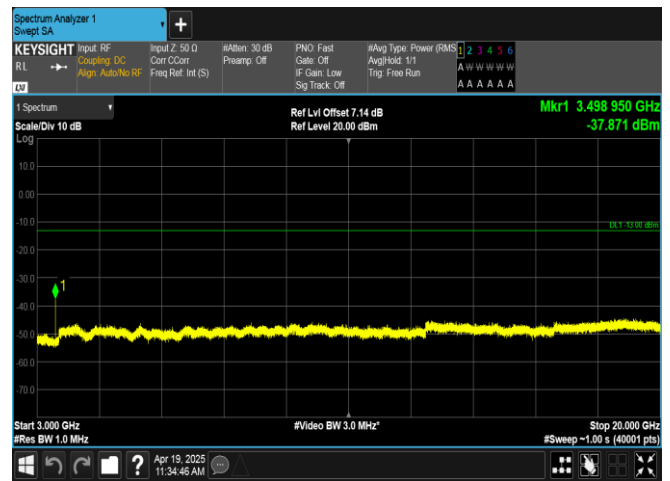
Band66-10MHz-16QAM-132322-1RB#49-3000~20000-PASS
