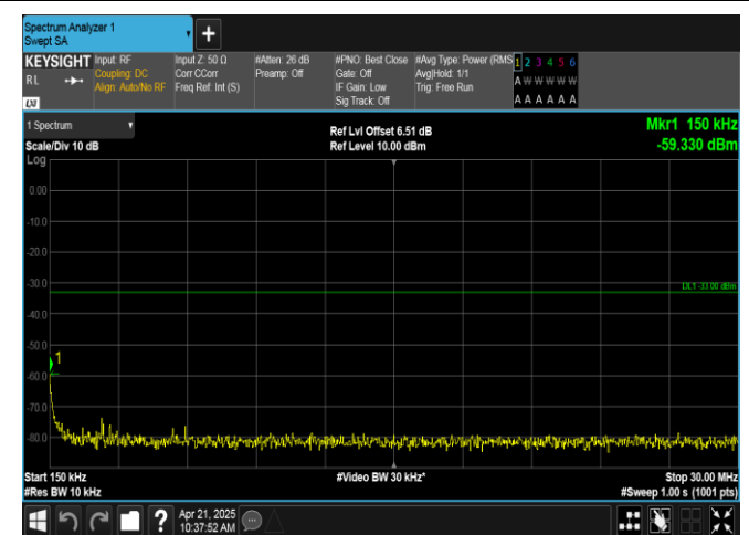
Band66-15MHz-QPSK-132047-75RB#0-0.15~30-PASS
