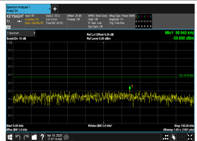
Band66-10MHz-QPSK-132622-1RB#49-0.009~0.15-PASS
