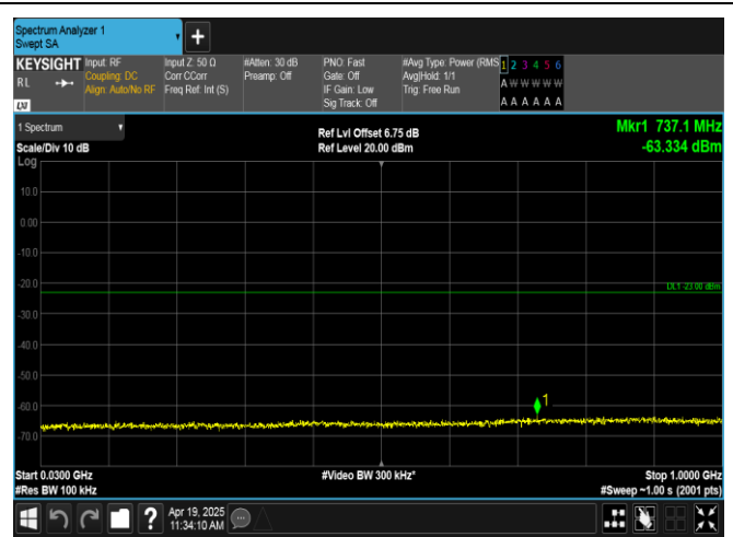
Band66-10MHz-16QAM-132322-1RB#49-30~1000-PASS
