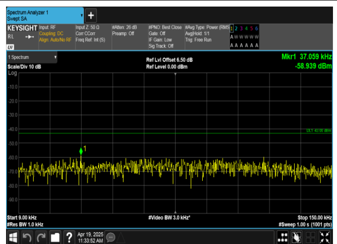
Band66-10MHz-16QAM-132322-1RB#49-0.009~0.15-PASS
