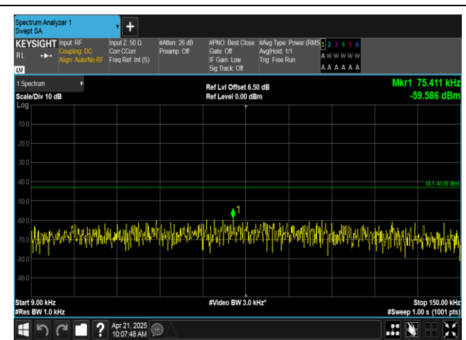
Band66-10MHz-16QAM-132022-50RB#0-0.009~0.15-PASS
