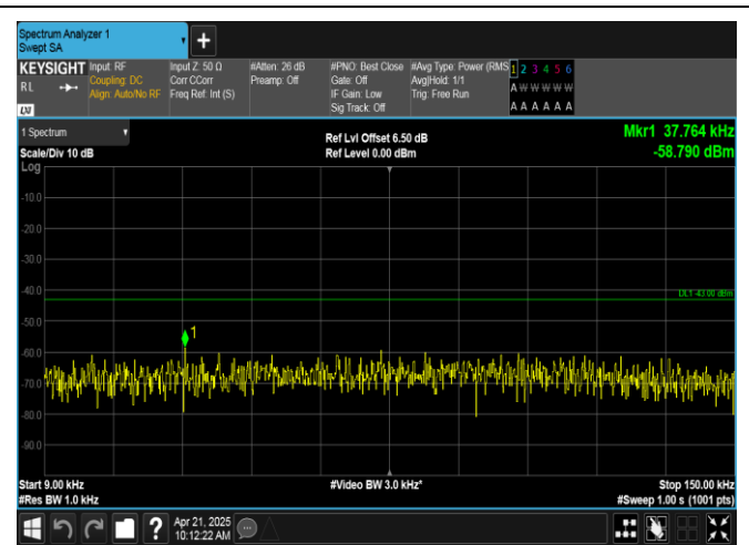
Band66-10MHz-16QAM-132622-50RB#0-0.009~0.15-PASS
