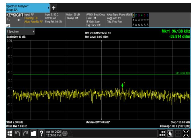
Band66-15MHz-QPSK-132322-1RB#0-0.009~0.15-PASS
