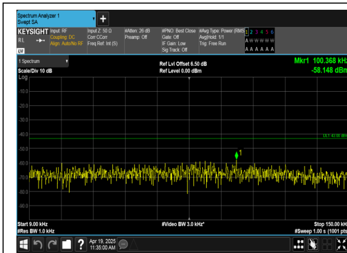
Band66-10MHz-QPSK-132622-1RB#0-0.009~0.15-PASS
