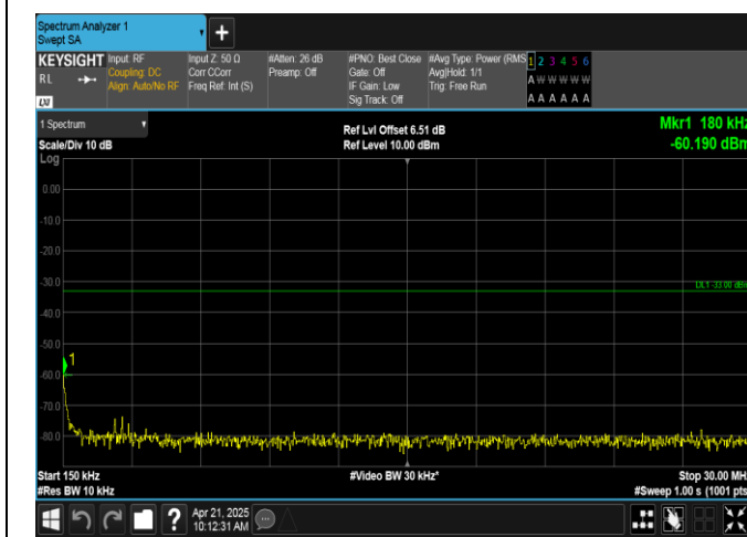
Band66-10MHz-16QAM-132622-50RB#0-0.15~30-PASS
