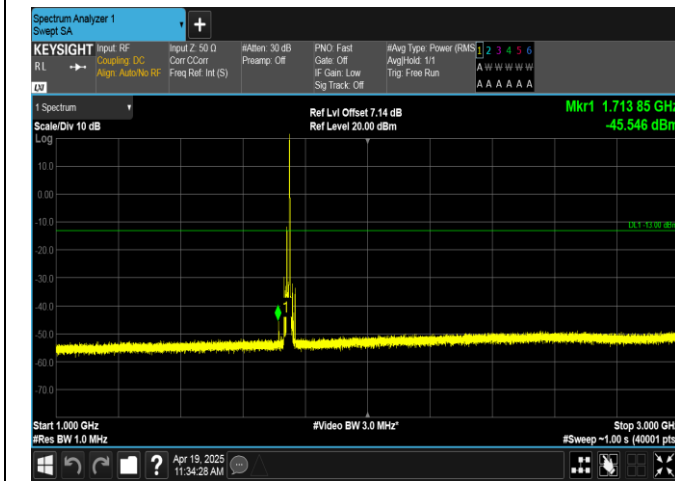
Band66-10MHz-16QAM-132322-1RB#49-1000~3000-PASS
