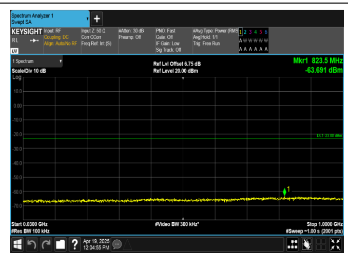
Band66-15MHz-QPSK-132047-1RB#74-30~1000-PASS
