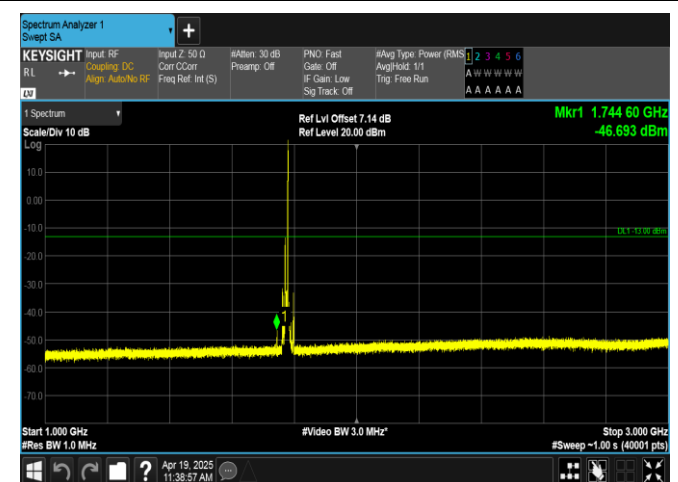
Band66-10MHz-16QAM-132622-1RB#49-1000~3000-PASS
