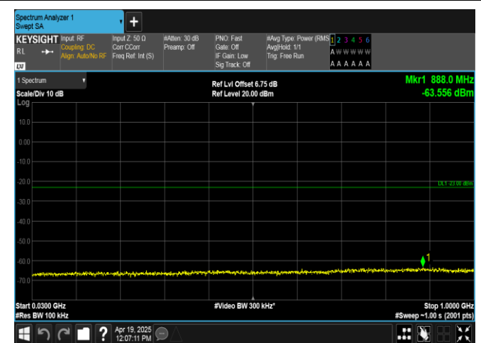
Band66-15MHz-QPSK-132322-1RB#0-30~1000-PASS
