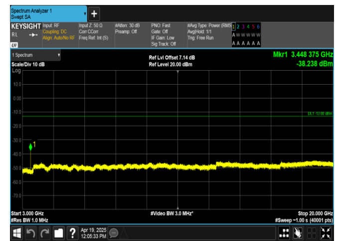
Band66-15MHz-QPSK-132047-1RB#74-3000~20000-PASS
