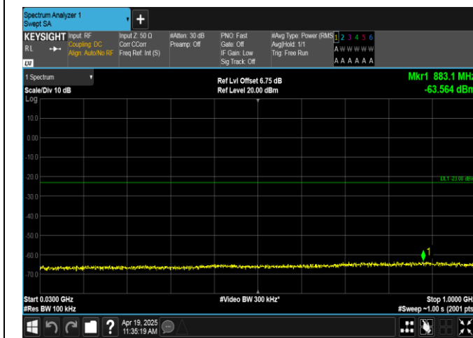
Band66-10MHz-QPSK-132622-1RB#0-30~1000-PASS
