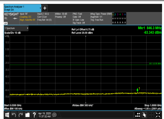
Band66-10MHz-QPSK-132622-1RB#49-30~1000-PASS
