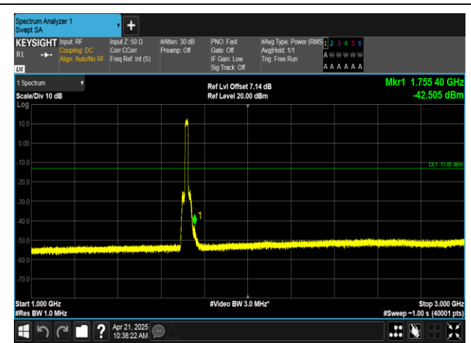
Band66-15MHz-QPSK-132047-75RB#0-1000~3000-PASS
