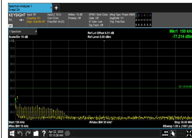
Band40(2350-2360)-10MHz-16QAM-39200-50RB#0-0.15~30-PASS
