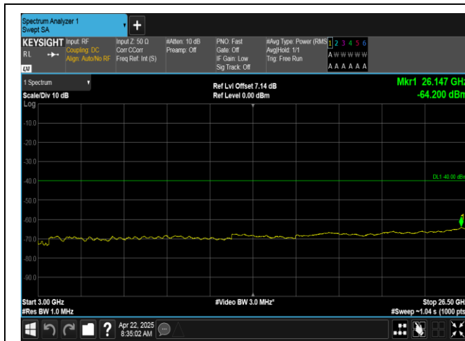
Band40(2350-2360)-5MHz-16QAM-39175-1RB#24-3000~26500-PASS
