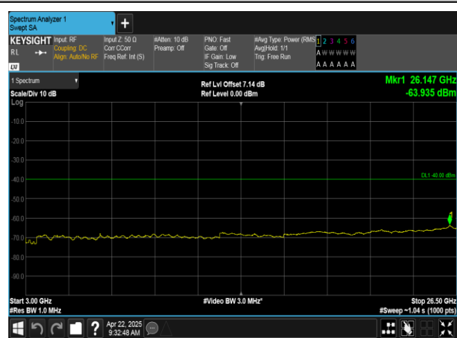
Band40(2350-2360)-10MHz-QPSK-39200-1RB#49-3000~26500-PASS
