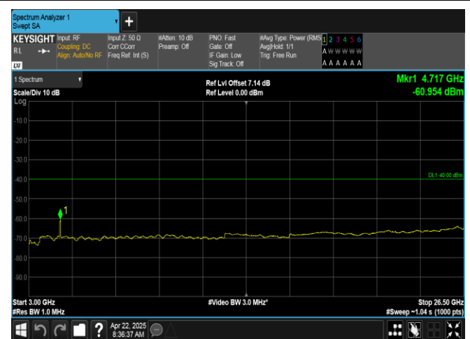
Band40(2350-2360)-5MHz-16QAM-39175-25RB#0-3000~26500-PASS
