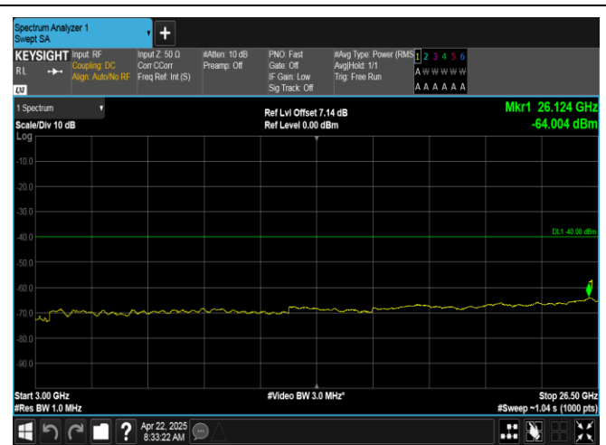
Band40(2350-2360)-5MHz-16QAM-39175-1RB#0-3000-26500-PASS
