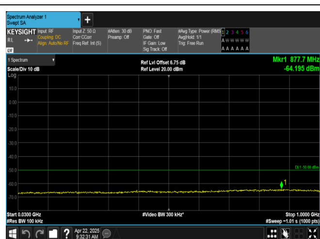
Band40(2350-2360)-10MHz-QPSK-39200-1RB#49-30~1000-PASS
