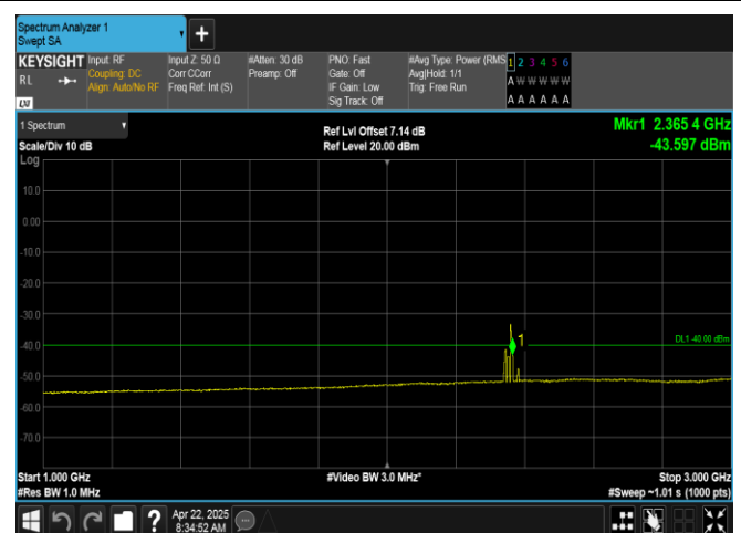
Band40(2350-2360)-5MHz-16QAM-39175-1RB#24-1000-3000-PASS
