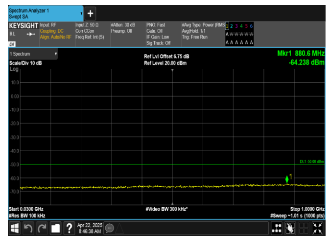
Band40(2350-2360)-5MHz-16QAM-39225-25RB#0-30~1000-PASS
