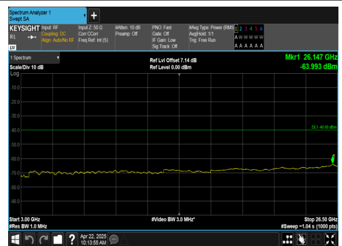
Band40(2350-2360)-10MHz-16QAM-39200-50RB#0-3000~26500-PASS
