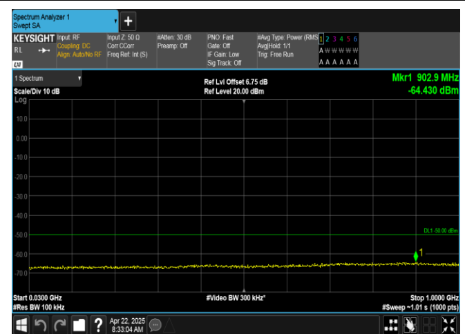
Band40(2350-2360)-5MHz-16QAM-39175-1RB#0-30~1000-PASS
