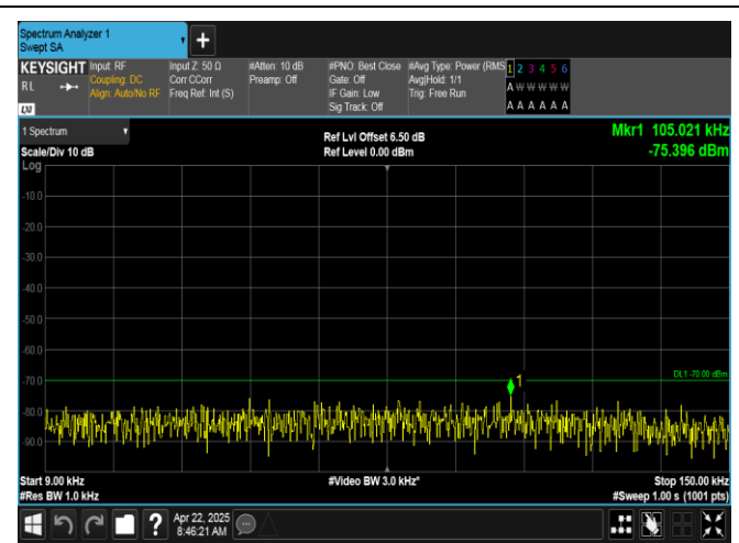
Band40(2350-2360)-5MHz-16QAM-39225-25RB#0-0.009~0.15-PASS
