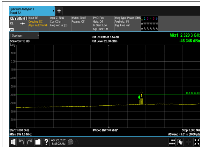
Band40(2350-2360)-5MHz-16QAM-39225-1RB#0-1000-3000-PASS
