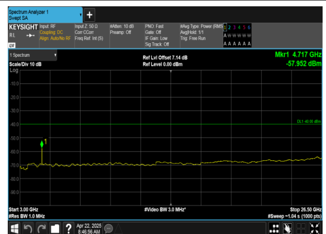
Band40(2350-2360)-5MHz-16QAM-39225-25RB#0-3000~26500-PASS
