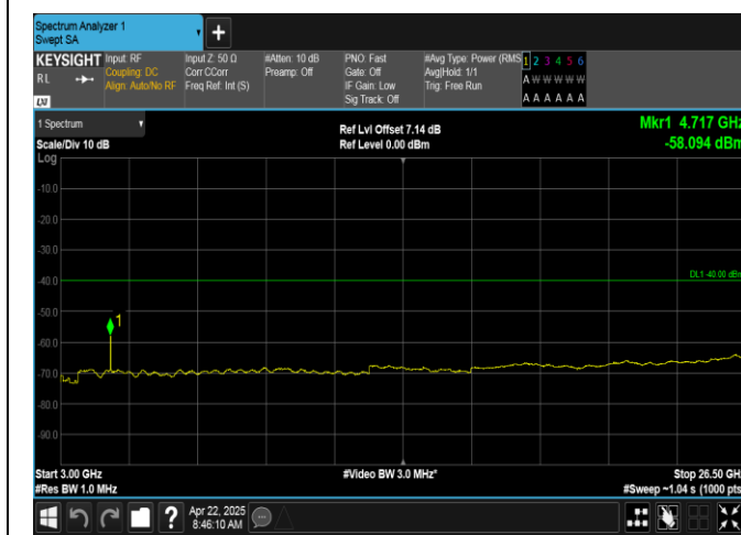
Band40(2350-2360)-5MHz-QPSK-39225-25RB#0-3000~26500-PASS
