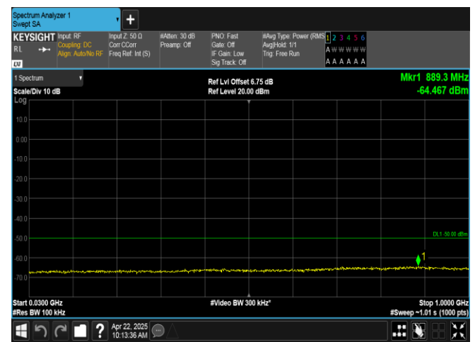
Band40(2350-2360)-10MHz-16QAM-39200-50RB#0-30~1000-PASS
