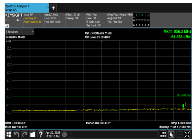
Band40(2350-2360)-5MHz-16QAM-39175-25RB#0-30~1000-PASS
