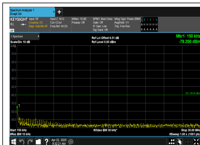
Band40(2350-2360)-10MHz-QPSK-39200-1RB#49-0.15~30-PASS
