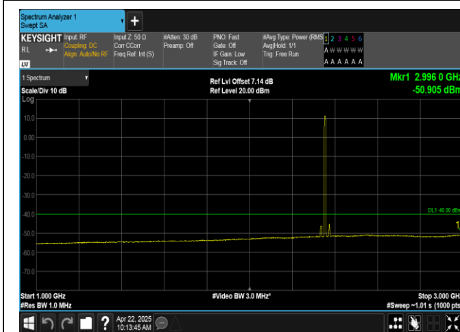
Band40(2350-2360)-10MHz-16QAM-39200-50RB#0-1000~3000-PASS
