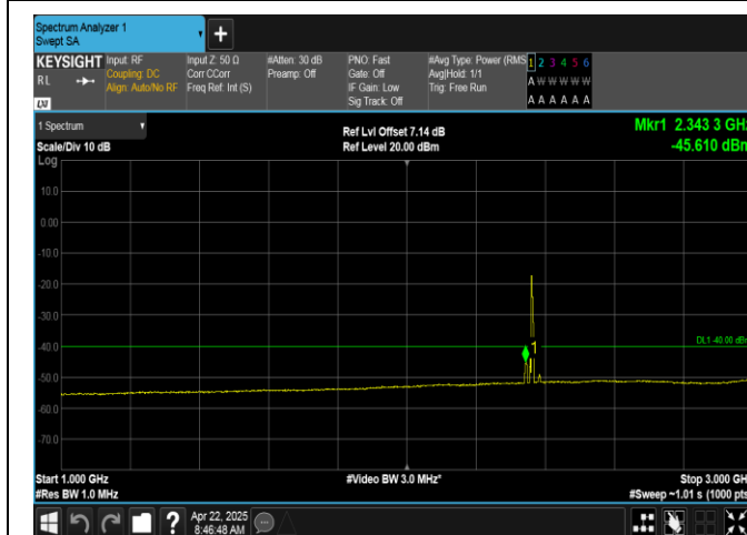
Band40(2350-2360)-5MHz-16QAM-39225-25RB#0-1000~3000-PASS
