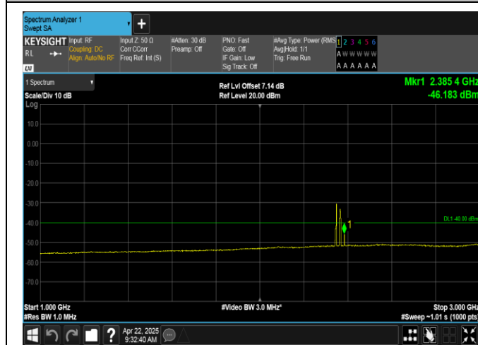
Band40(2350-2360)-10MHz-QPSK-39200-1RB#49-1000~3000-PASS
