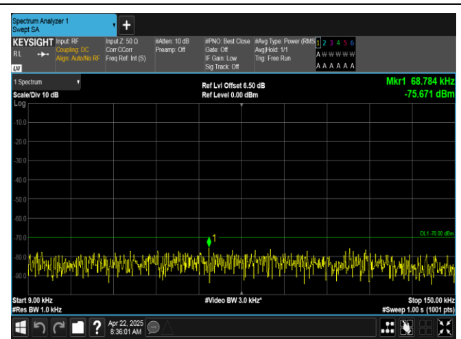
Band40(2350-2360)-5MHz-16QAM-39175-25RB#0-0.009~0.15-PASS
