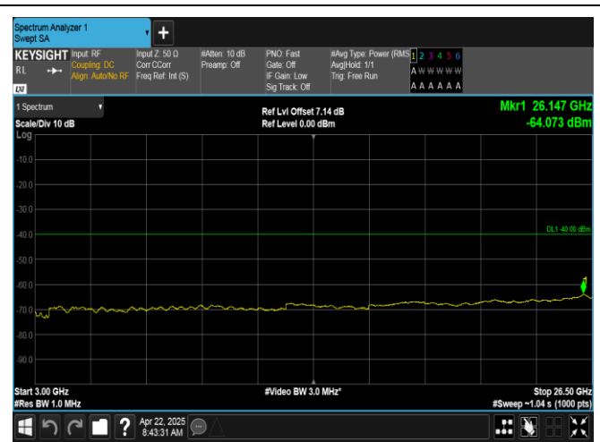
Band40(2350-2360)-5MHz-16QAM-39225-1RB#0-3000-26500-PASS
