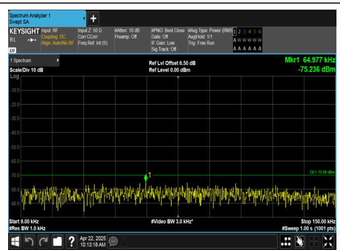
Band40(2350-2360)-10MHz-16QAM-39200-50RB#0-0.009~0.15-PASS
