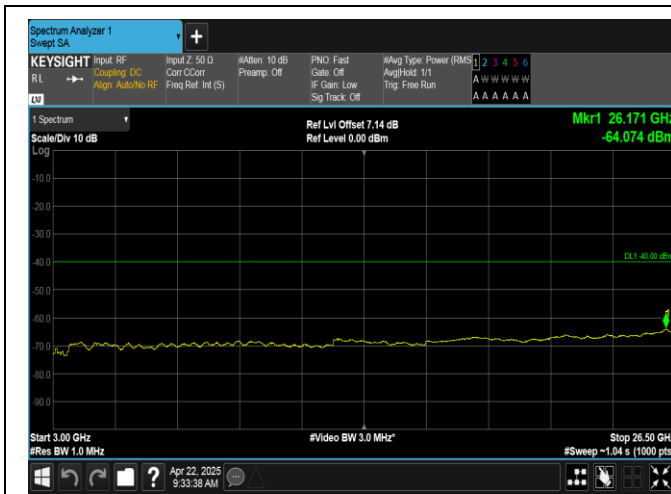
Band40(2350-2360)-10MHz-16QAM-39200-1RB#49-3000~26500-PASS
