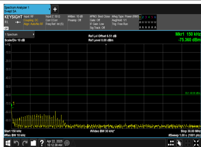
Band40(2350-2360)-10MHz-QPSK-39200-50RB#0-0.15~30-PASS
