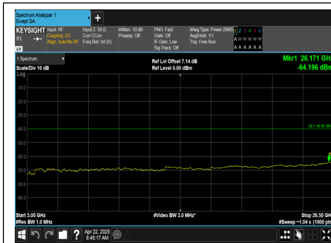
Band40(2350-2360)-5MHz-16QAM-39225-1RB#24-3000~26500-PASS
