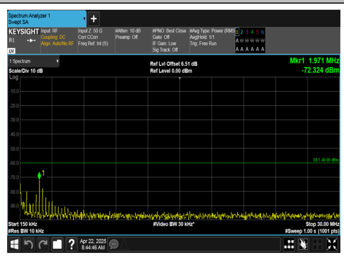
Band40(2350-2360)-5MHz-16QAM-39225-1RB#24-0.15-30-PASS
