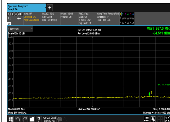
Band40(2350-2360)-5MHz-16QAM-39175-1RB#24-30-1000-PASS
