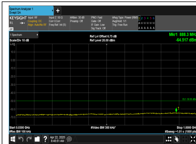
Band40(2350-2360)-5MHz-QPSK-39225-25RB#0-30~1000-PASS
