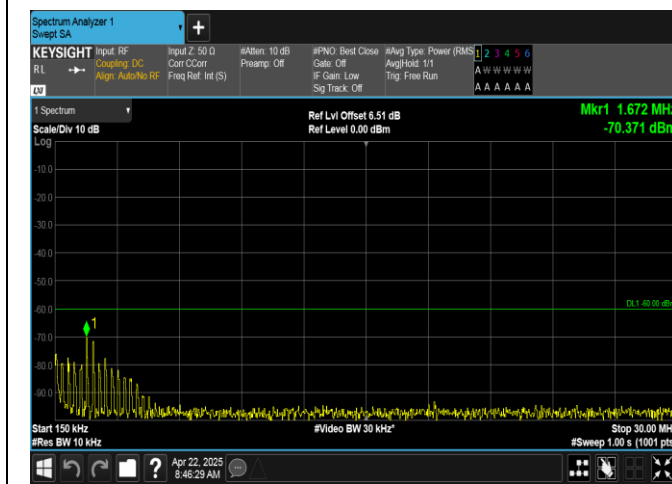
Band40(2350-2360)-5MHz-16QAM-39225-25RB#0-0.15~30-PASS
