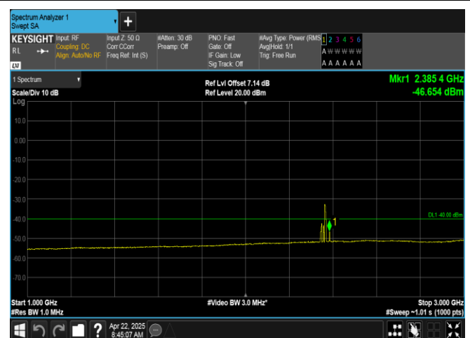
Band40(2350-2360)-5MHz-16QAM-39225-1RB#24-1000-3000-PASS
