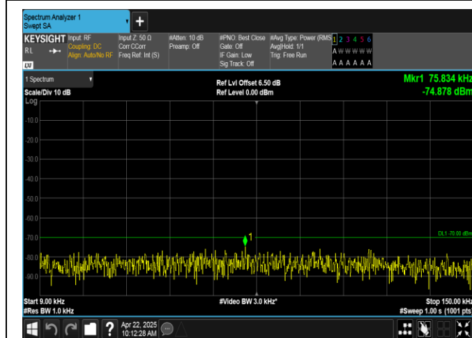
Band40(2350-2360)-10MHz-QPSK-39200-50RB#0-0.009~0.15-PASS
