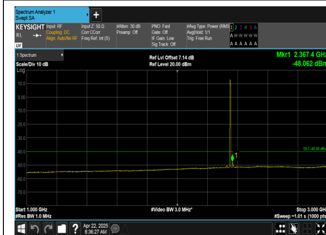
Band40(2350-2360)-5MHz-16QAM-39175-25RB#0-1000~3000-PASS
