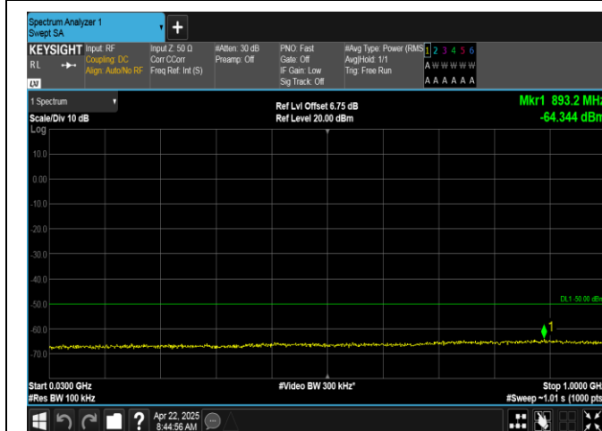
Band40(2350-2360)-5MHz-16QAM-39225-1RB#24-30-1000-PASS
