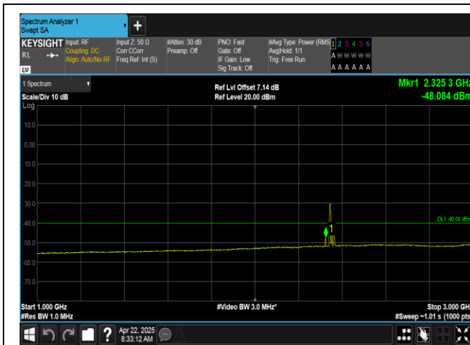
Band40(2350-2360)-5MHz-16QAM-39175-1RB#0-1000-3000-PASS
