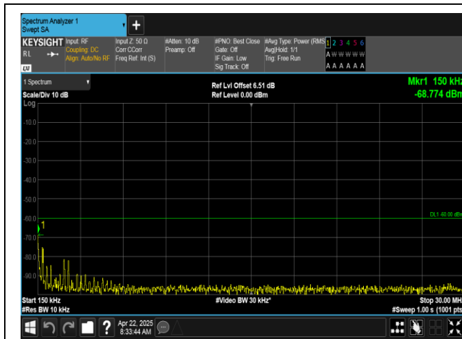
Band40(2350-2360)-5MHz-QPSK-39175-1RB#24-0.15~30-PASS
