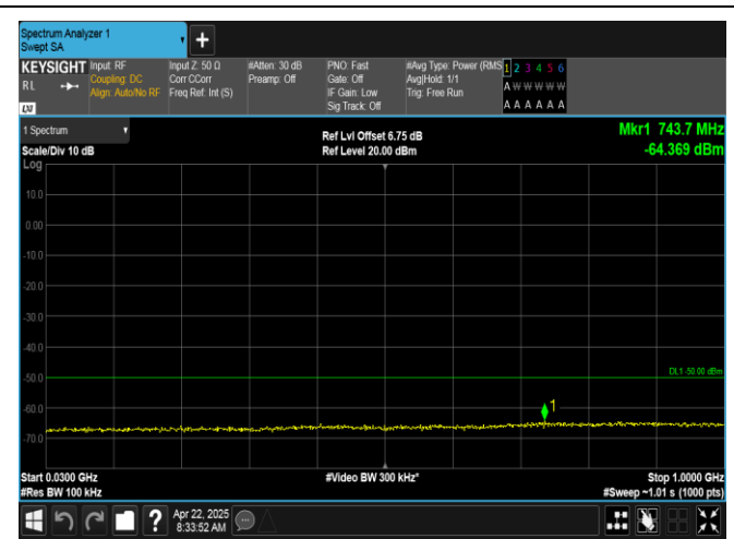
Band40(2350-2360)-5MHz-QPSK-39175-1RB#24-30~1000-PASS
