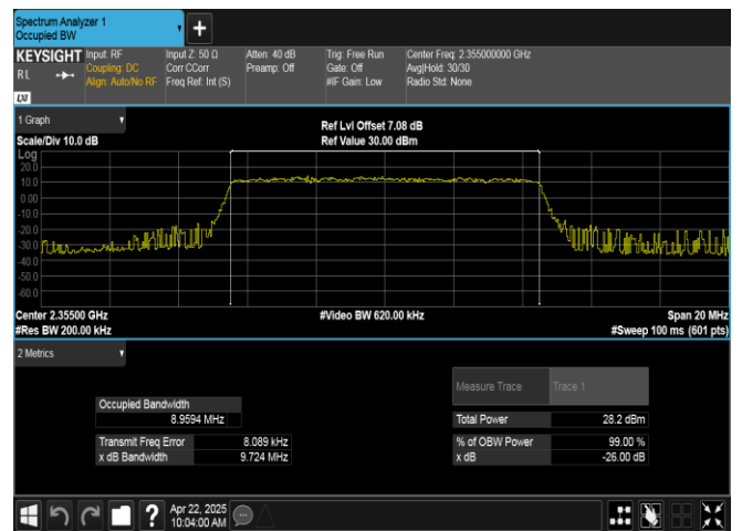
Band40(2350-2360)-10MHz-16QAM-39200-50RB#0-PASS
