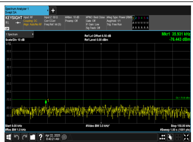
Band40(2350-2360)-5MHz-QPSK-39200-25RB#0-0.009~0.15-PASS
