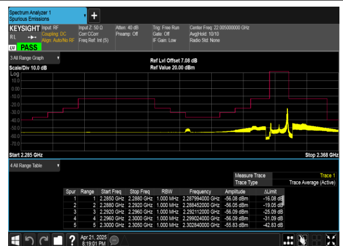
Band40(2350-2360)-5MHz-16QAM-39175-1RB#24-PASS
