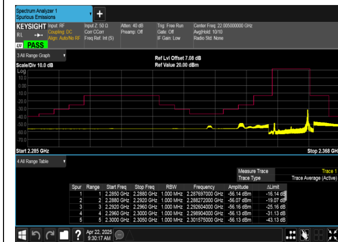
Band40(2350-2360)-10MHz-16QAM-39200-1RB#49-PASS
