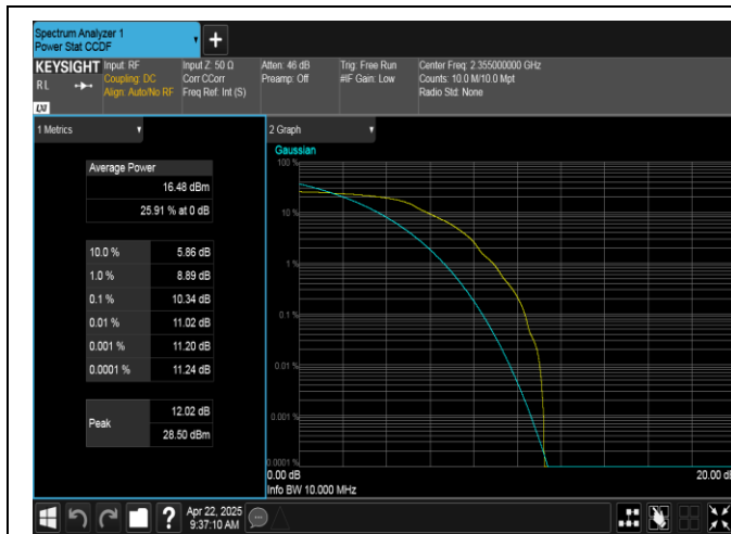
Band40(2350-2360)-10MHz-QPSK-39200-1RB#0-PASS
