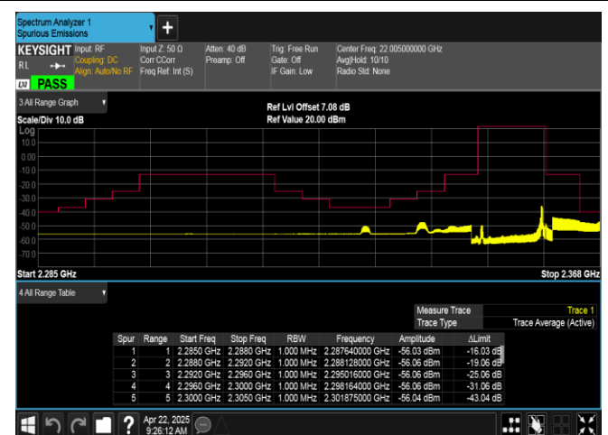
Band40(2350-2360)-10MHz-QPSK-39200-1RB#49-PASS
