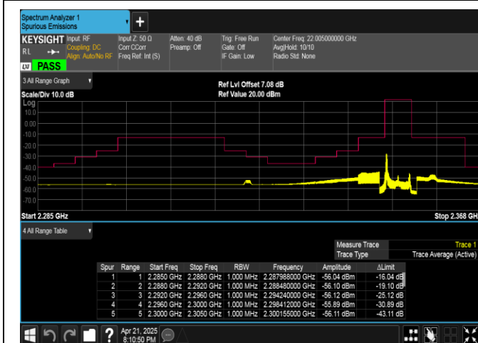
Band40(2350-2360)-5MHz-16QAM-39175-1RB#0-PASS
