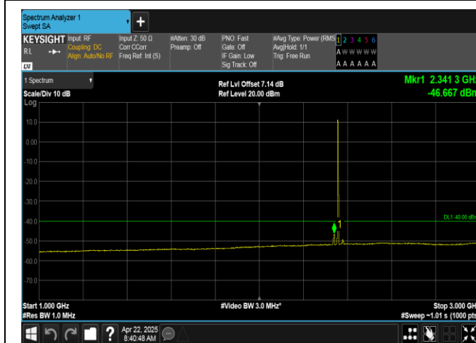
Band40(2350-2360)-5MHz-QPSK-39200-25RB#0-1000~3000-PASS
