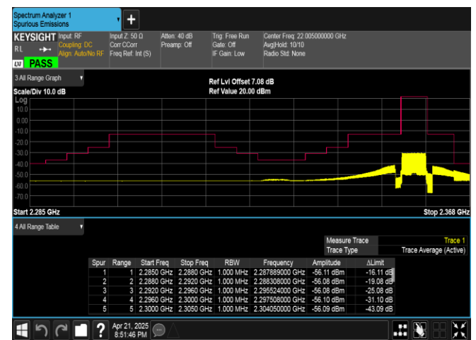
Band40(2350-2360)-5MHz-16QAM-39225-25RB#0-PASS
