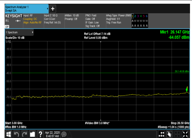
Band40(2350-2360)-5MHz-QPSK-39200-25RB#0-3000~26500-PASS
