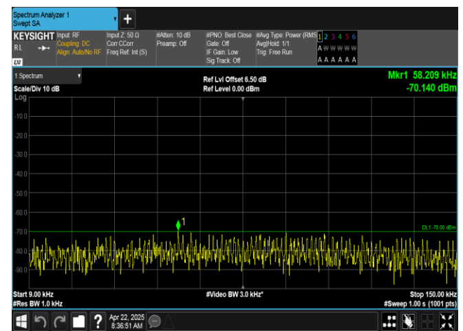
Band40(2350-2360)-5MHz-QPSK-39200-1RB#0-0.009~0.15-PASS
