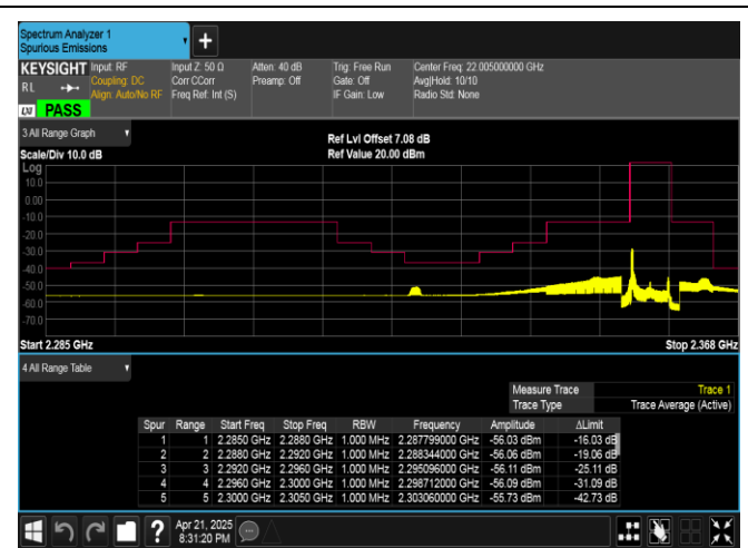
Band40(2350-2360)-5MHz-QPSK-39225-1RB#0-PASS
