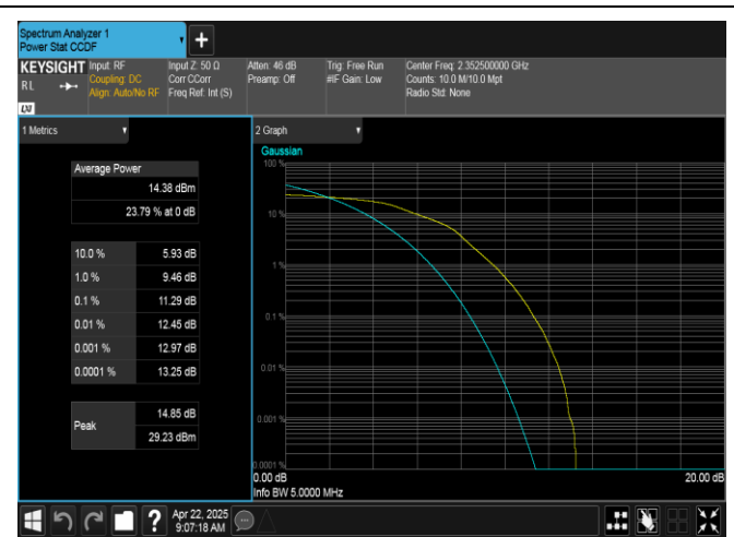
Band40(2350-2360)-5MHz-16QAM-39175-25RB#0-PASS
