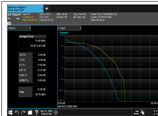
Band40(2350-2360)-5MHz-16QAM-39175-1RB#0-PASS
