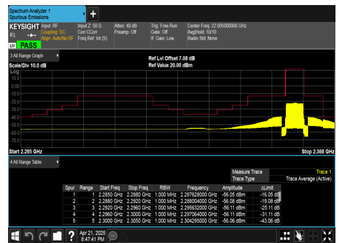
Band40(2350-2360)-5MHz-QPSK-39225-25RB#0-PASS
