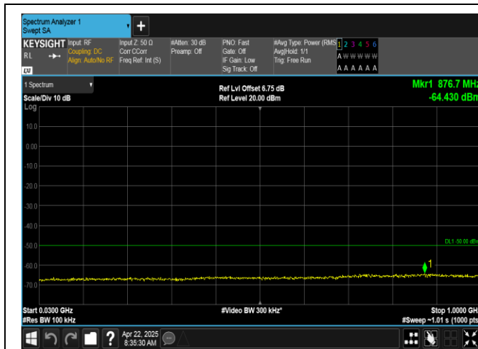
Band40(2350-2360)-5MHz-QPSK-39175-25RB#0-30~1000-PASS
