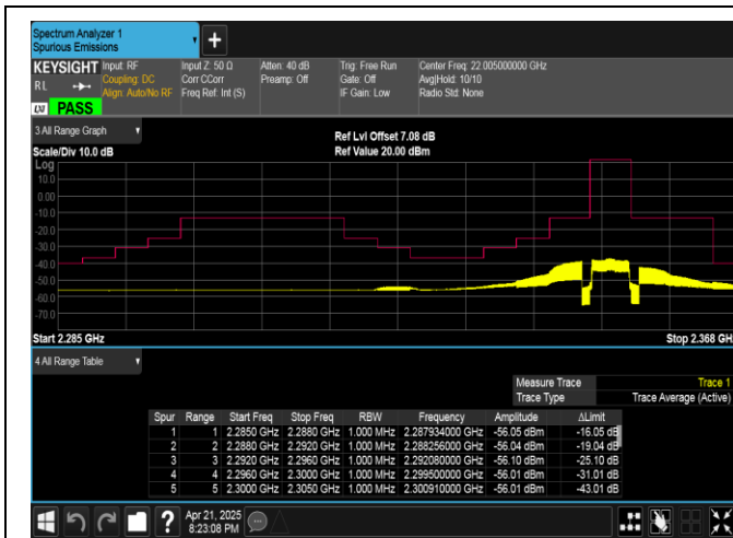
Band40(2350-2360)-5MHz-QPSK-39175-25RB#0-PASS
