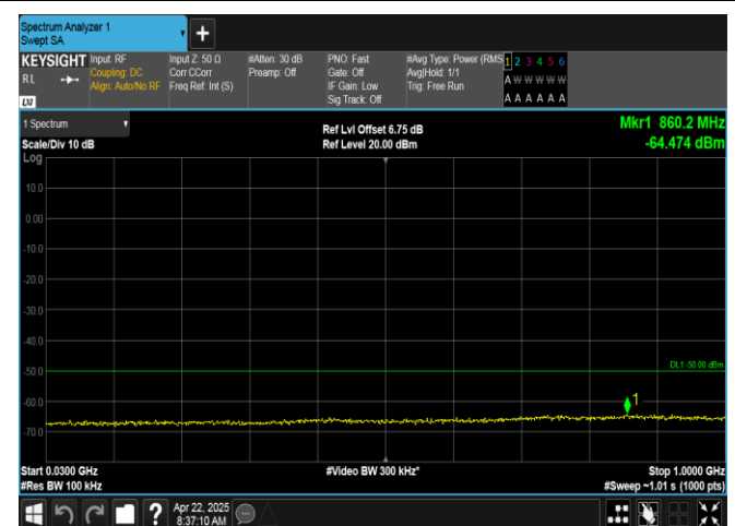
Band40(2350-2360)-5MHz-QPSK-39200-1RB#0-30~1000-PASS
