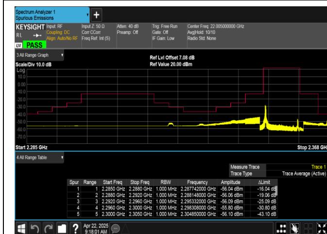
Band40(2350-2360)-10MHz-QPSK-39200-1RB#0-PASS
