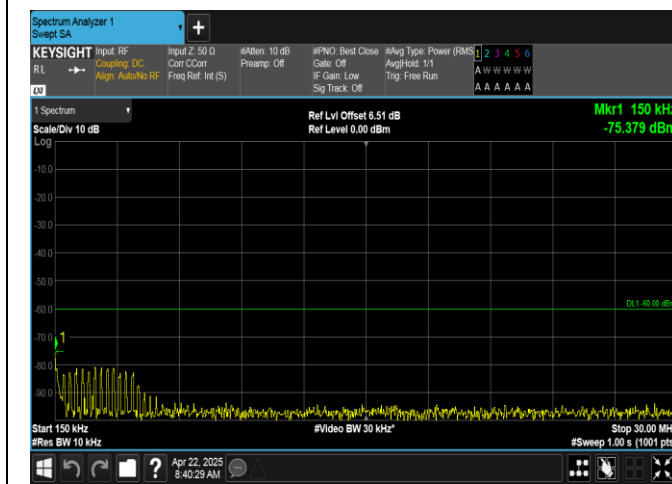
Band40(2350-2360)-5MHz-QPSK-39200-25RB#0-0.15~30-PASS
