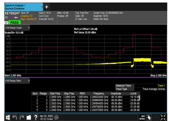
Band40(2350-2360)-10MHz-16QAM-39200-50RB#0-PASS
