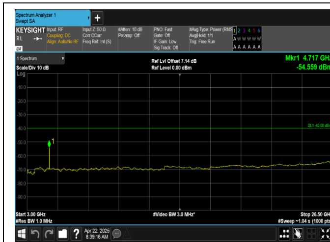
Band40(2350-2360)-5MHz-QPSK-39200-1RB#24-3000~26500-PASS
