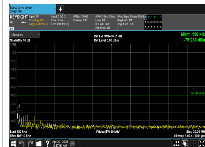
Band40(2350-2360)-5MHz-QPSK-39200-1RB#0-0.15~30-PASS
