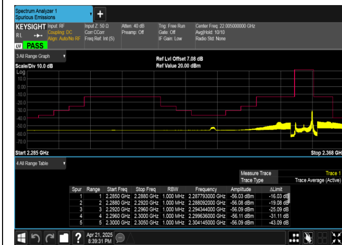
Band40(2350-2360)-5MHz-QPSK-39225-1RB#24-PASS
