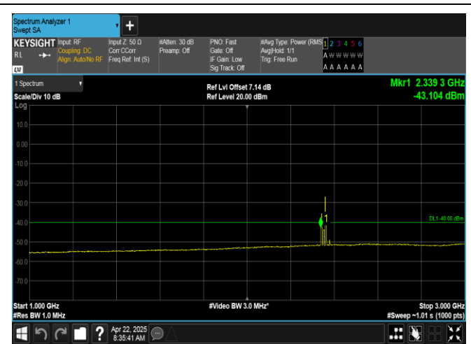
Band40(2350-2360)-5MHz-QPSK-39175-25RB#0-1000~3000-PASS
