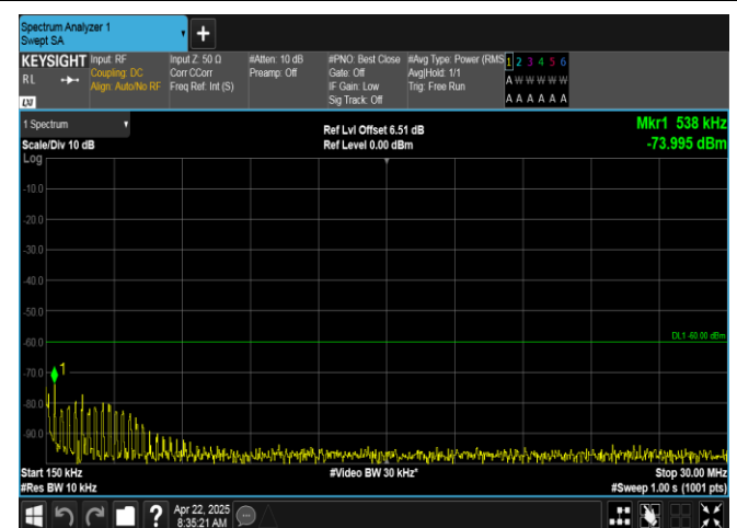
Band40(2350-2360)-5MHz-QPSK-39175-25RB#0-0.15~30-PASS
