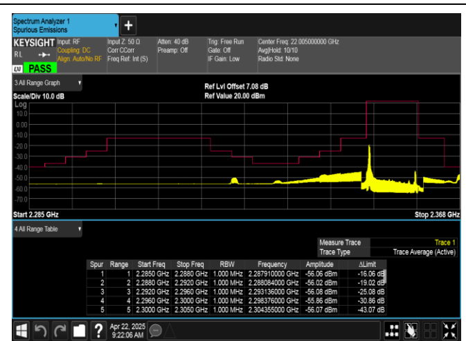
Band40(2350-2360)-10MHz-16QAM-39200-1RB#0-PASS
