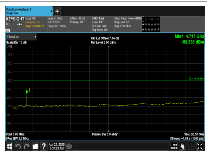
Band40(2350-2360)-5MHz-QPSK-39200-1RB#0-3000-26500-PASS
