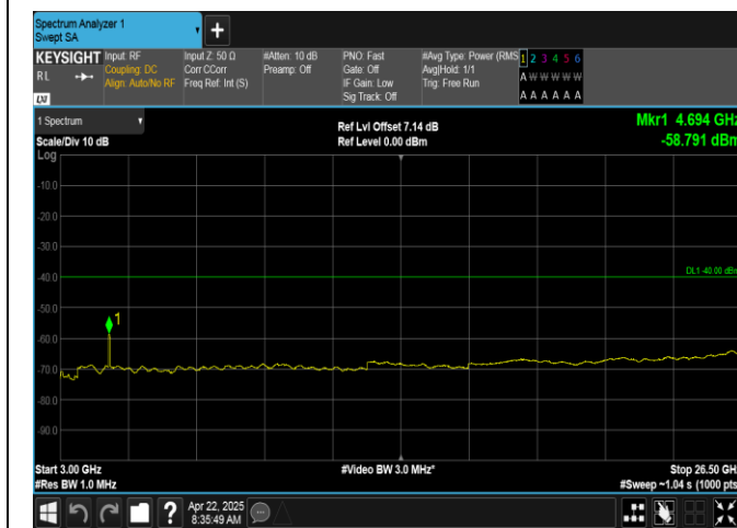
Band40(2350-2360)-5MHz-QPSK-39175-25RB#0-3000~26500-PASS
