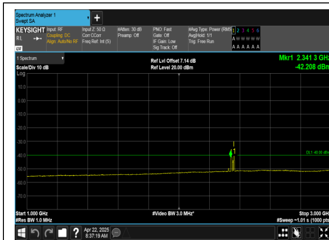
Band40(2350-2360)-5MHz-QPSK-39200-1RB#0-1000-3000-PASS
