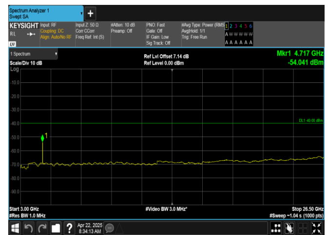
Band40(2350-2360)-5MHz-QPSK-39175-1RB#24-3000~26500-PASS
