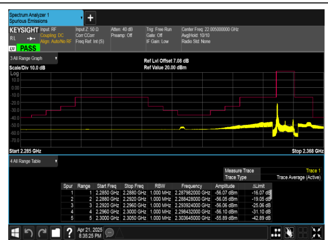
Band40(2350-2360)-5MHz-16QAM-39225-1RB#0-PASS
