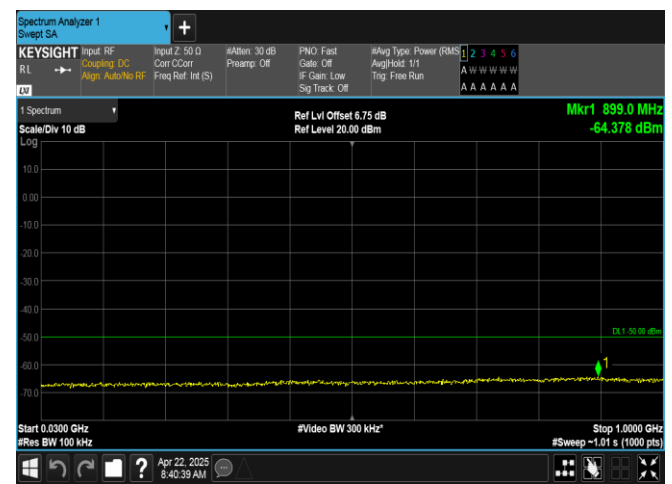
Band40(2350-2360)-5MHz-QPSK-39200-25RB#0-30~1000-PASS
