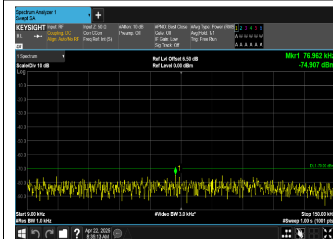
Band40(2350-2360)-5MHz-QPSK-39175-25RB#0-0.009~0.15-PASS
