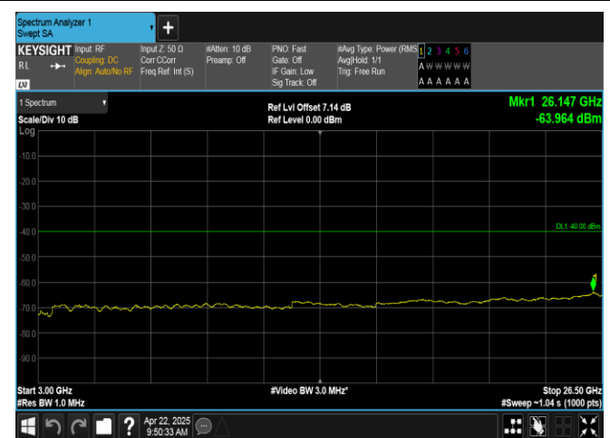
Band40(2305-2315)-10MHz-16QAM-38750-50RB#0-3000~26500-PASS
