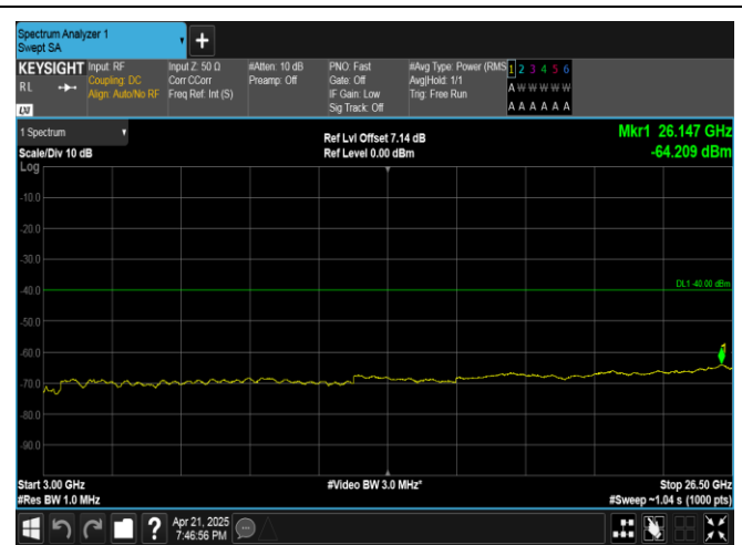
Band40(2305-2315)-10MHz-16QAM-38750-1RB#0-3000~26500-PASS
