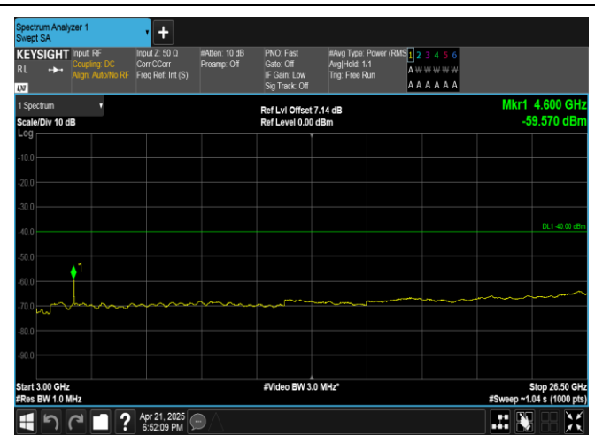
Band40(2305-2315)-5MHz-16QAM-38725-1RB#0-3000~26500-PASS
