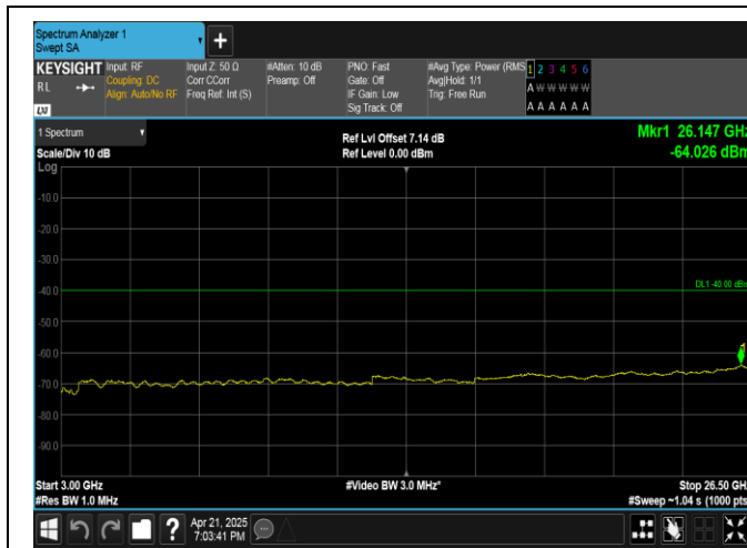
Band40(2305-2315)-5MHz-16QAM-38775-1RB#24-3000~26500-PASS
