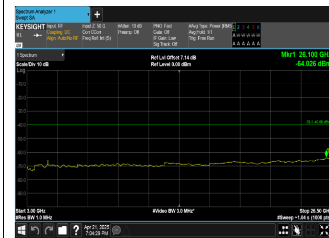
Band40(2305-2315)-5MHz-QPSK-38775-25RB#0-3000~26500-PASS
