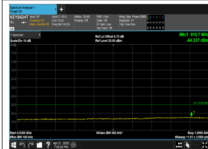
Band40(2305-2315)-5MHz-16QAM-38775-1RB#24-30~1000-PASS
