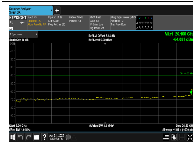
Band40(2305-2315)-5MHz-16QAM-38725-1RB#24-3000~26500-PASS
