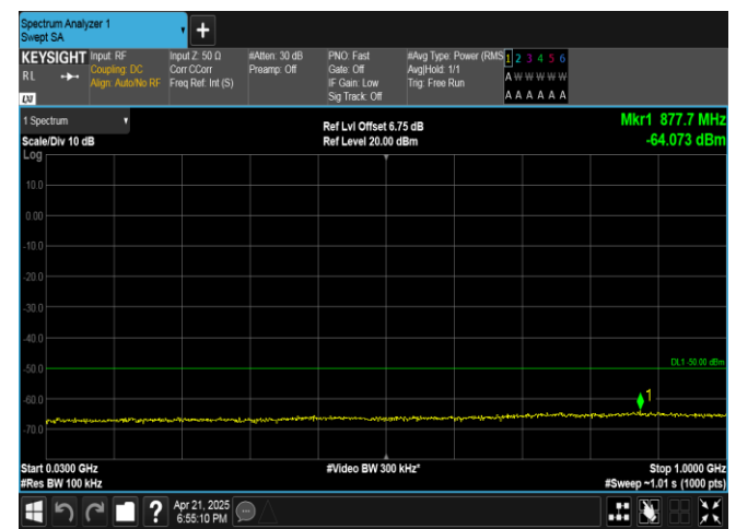
Band40(2305-2315)-5MHz-16QAM-38725-25RB#0-30~1000-PASS
