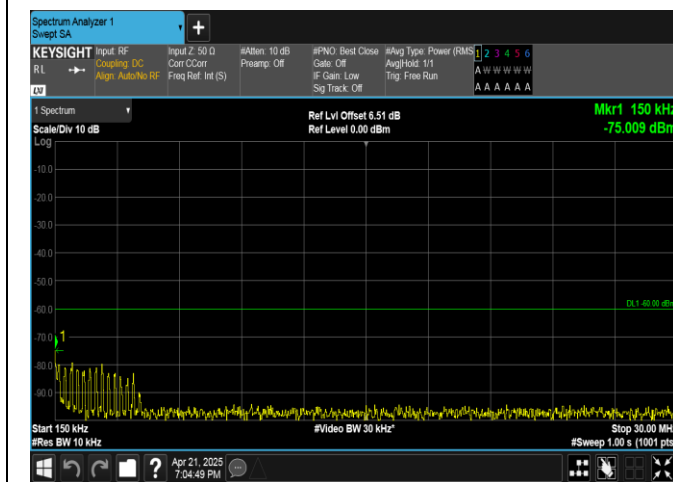
Band40(2305-2315)-5MHz-16QAM-38775-25RB#0-0.15~30-PASS
