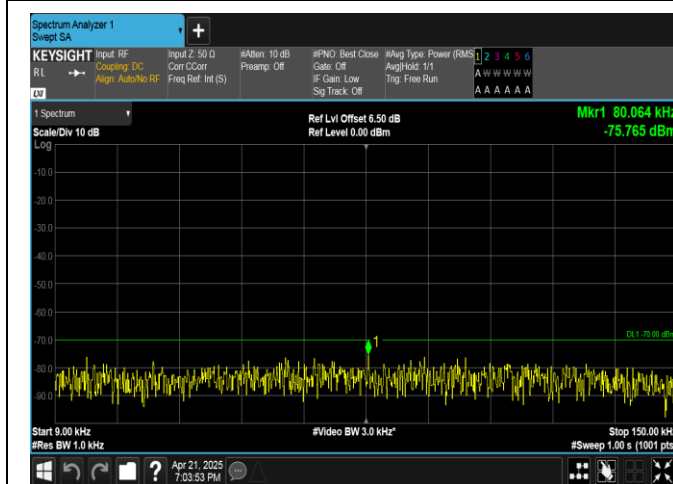
Band40(2305-2315)-5MHz-QPSK-38775-25RB#0-0.009~0.15-PASS
