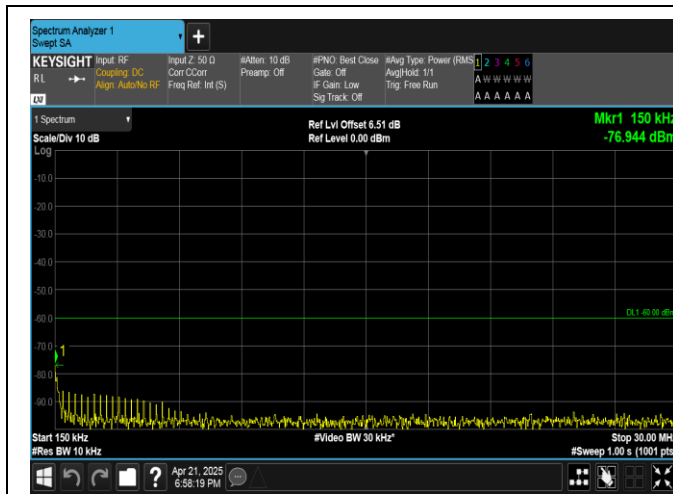
Band40(2305-2315)-5MHz-16QAM-38750-1RB#24-0.15~30-PASS
