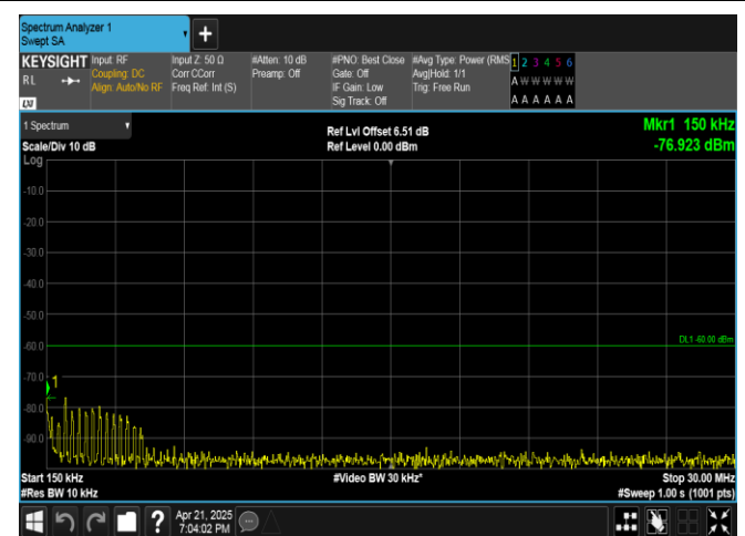
Band40(2305-2315)-5MHz-QPSK-38775-25RB#0-0.15~30-PASS
