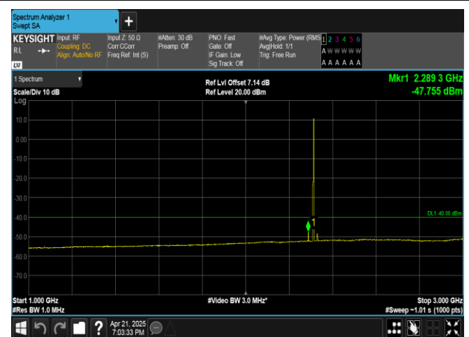
Band40(2305-2315)-5MHz-16QAM-38775-1RB#24-1000~3000-PASS
