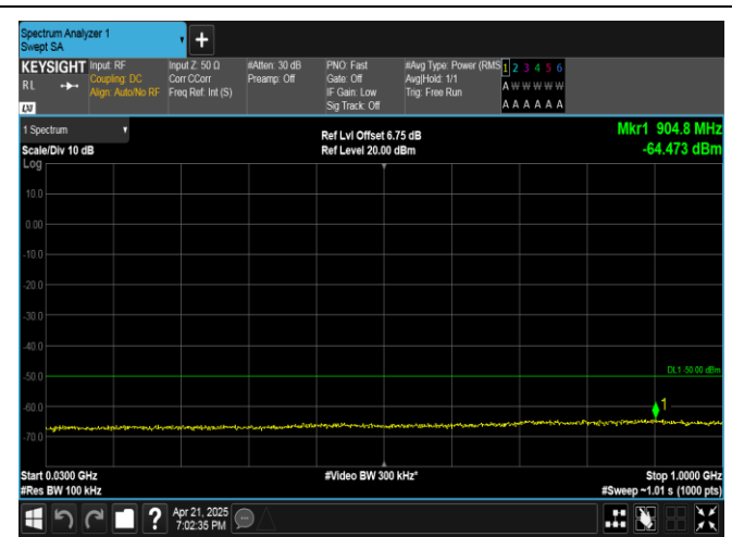
Band40(2305-2315)-5MHz-QPSK-38775-1RB#24-30~1000-PASS
