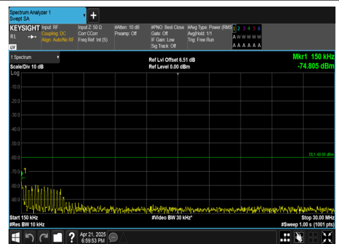
Band40(2305-2315)-5MHz-16QAM-38750-25RB#0-0.15~30-PASS
