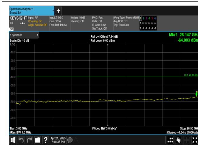
Band40(2305-2315)-10MHz-16QAM-38750-1RB#49-3000~26500-PASS
