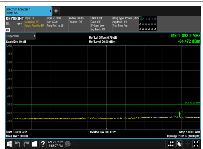
Band40(2305-2315)-5MHz-16QAM-38750-1RB#24-30~1000-PASS
