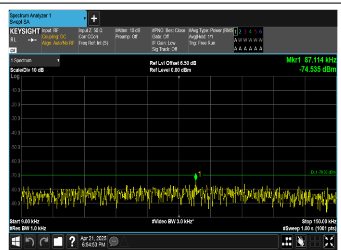
Band40(2305-2315)-5MHz-16QAM-38725-25RB#0-0.009~0.15-PASS
