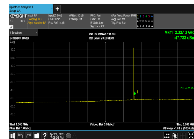
Band40(2305-2315)-5MHz-16QAM-38775-25RB#0-1000~3000-PASS
