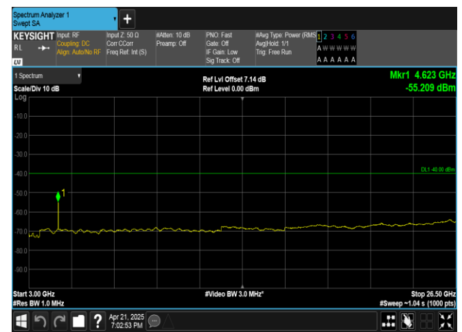
Band40(2305-2315)-5MHz-QPSK-38775-1RB#24-3000~26500-PASS
