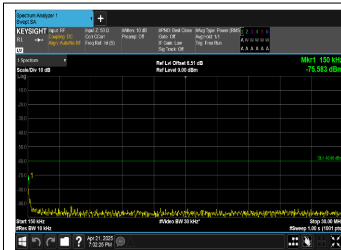
Band40(2305-2315)-5MHz-QPSK-38775-1RB#24-0.15~30-PASS
