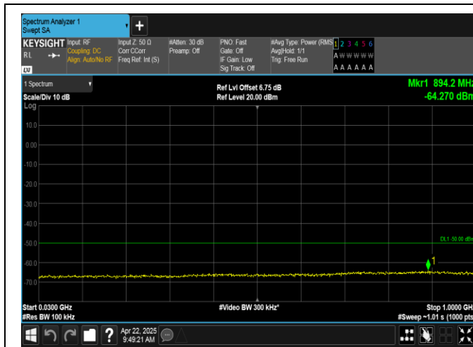
Band40(2305-2315)-10MHz-QPSK-38750-50RB#0-30~1000-PASS
