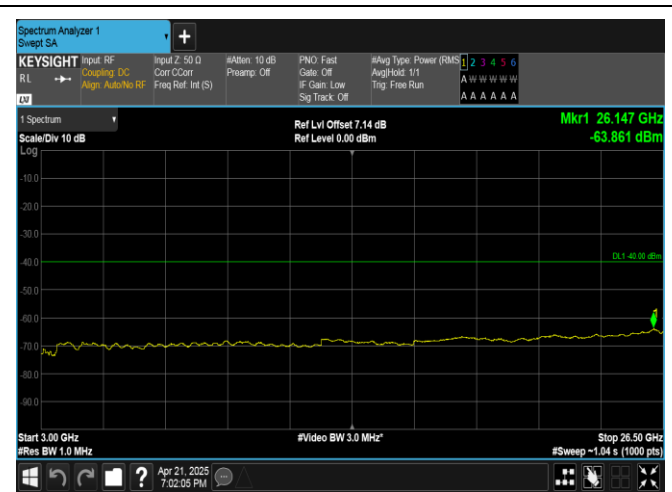
Band40(2305-2315)-5MHz-16QAM-38775-1RB#0-3000~26500-PASS
