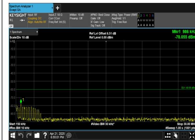
Band40(2305-2315)-5MHz-16QAM-38725-25RB#0-0.15~30-PASS
