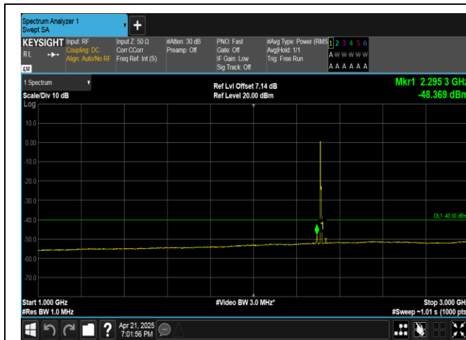
Band40(2305-2315)-5MHz-16QAM-38775-1RB#0-1000~3000-PASS
