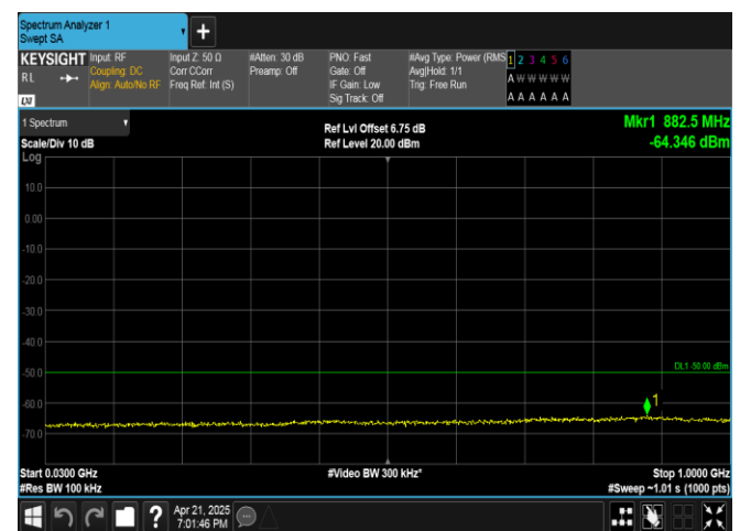
Band40(2305-2315)-5MHz-16QAM-38775-1RB#0-30~1000-PASS
