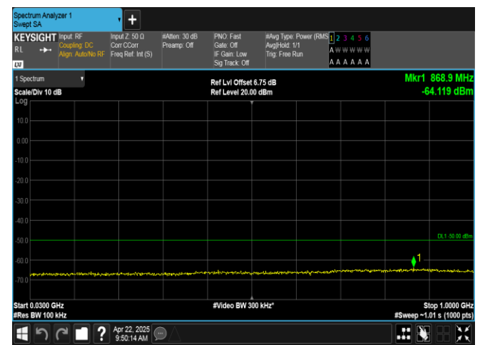
Band40(2305-2315)-10MHz-16QAM-38750-50RB#0-30~1000-PASS
