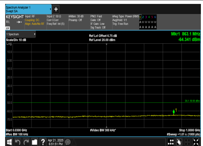
Band40(2305-2315)-5MHz-16QAM-38725-1RB#0-30~1000-PASS
