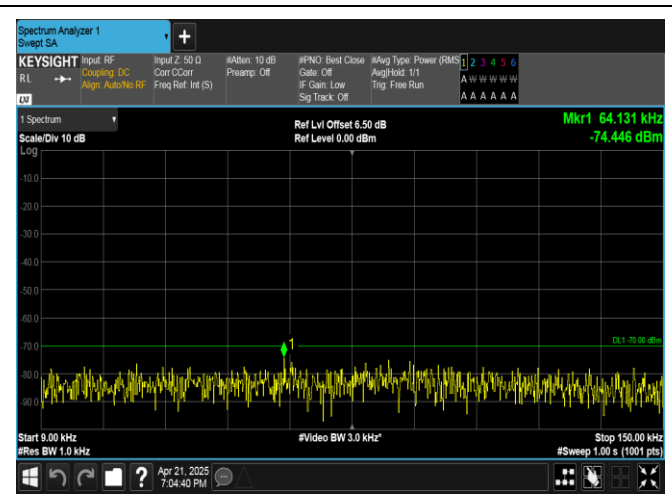
Band40(2305-2315)-5MHz-16QAM-38775-25RB#0-0.009~0.15-PASS
