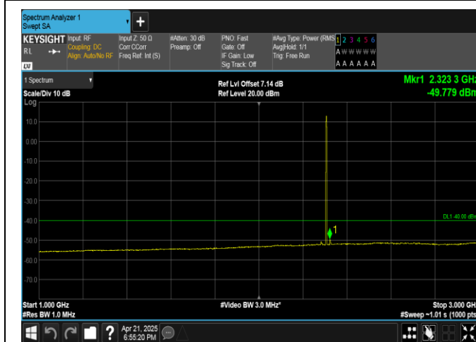
Band40(2305-2315)-5MHz-16QAM-38725-25RB#0-1000~3000-PASS
