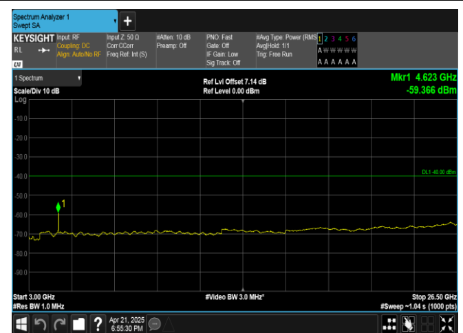
Band40(2305-2315)-5MHz-16QAM-38725-25RB#0-3000~26500-PASS
