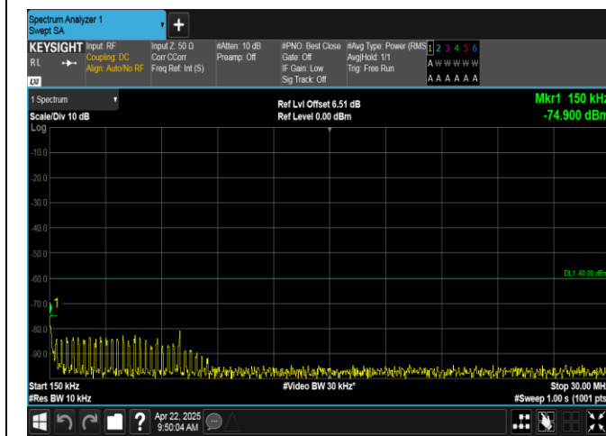
Band40(2305-2315)-10MHz-16QAM-38750-50RB#0-0.15~30-PASS
