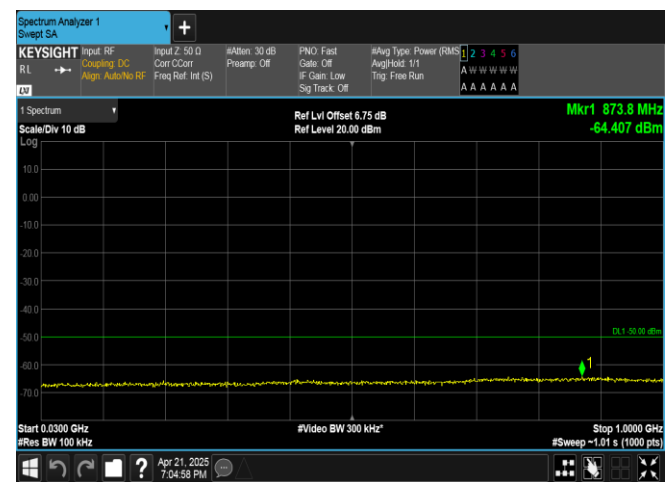
Band40(2305-2315)-5MHz-16QAM-38775-25RB#0-30~1000-PASS
