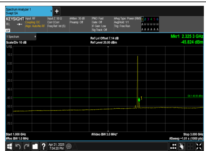
Band40(2305-2315)-5MHz-QPSK-38775-25RB#0-1000~3000-PASS
