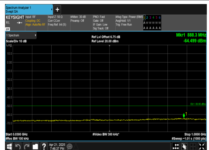
Band40(2305-2315)-10MHz-16QAM-38750-1RB#0-30~1000-PASS
