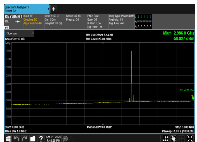
Band40(2305-2315)-10MHz-16QAM-38750-1RB#49-1000~3000-PASS
