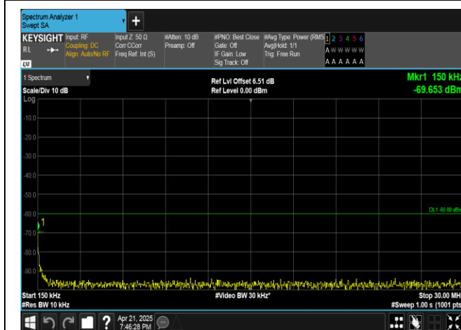
Band40(2305-2315)-10MHz-16QAM-38750-1RB#0-0.15~30-PASS
