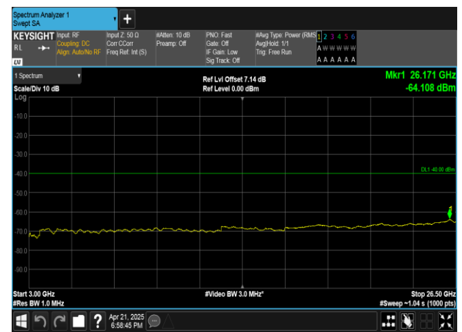
Band40(2305-2315)-5MHz-16QAM-38750-1RB#24-3000~26500-PASS
