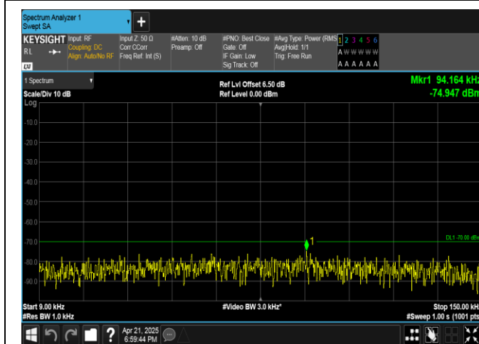
Band40(2305-2315)-5MHz-16QAM-38750-25RB#0-0.009~0.15-PASS
