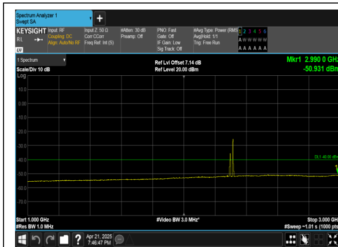
Band40(2305-2315)-10MHz-16QAM-38750-1RB#0-1000~3000-PASS
