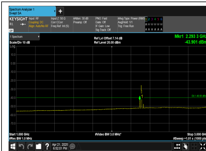
Band40(2305-2315)-5MHz-16QAM-38725-1RB#0-1000~3000-PASS
