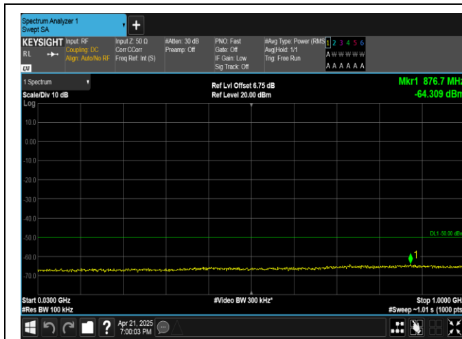
Band40(2305-2315)-5MHz-16QAM-38750-25RB#0-30~1000-PASS
