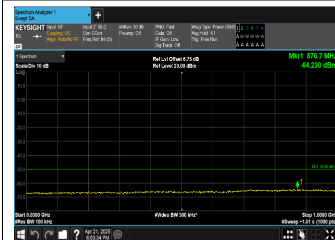
Band40(2305-2315)-5MHz-16QAM-38725-1RB#24-30~1000-PASS
