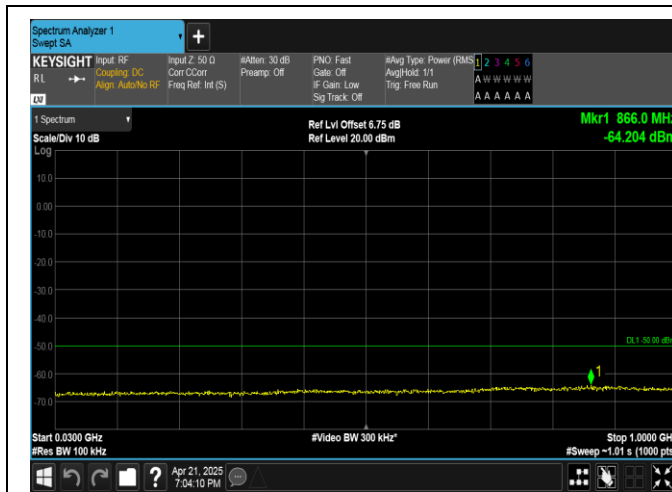
Band40(2305-2315)-5MHz-QPSK-38775-25RB#0-30~1000-PASS
