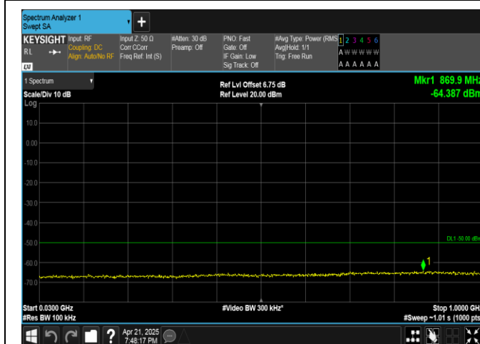
Band40(2305-2315)-10MHz-16QAM-38750-1RB#49-30~1000-PASS
