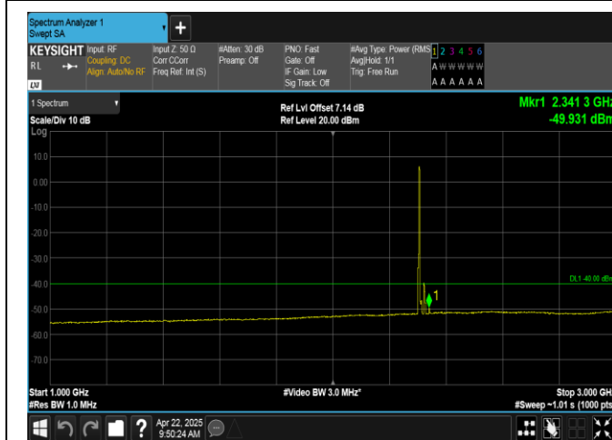
Band40(2305-2315)-10MHz-16QAM-38750-50RB#0-1000~3000-PASS
