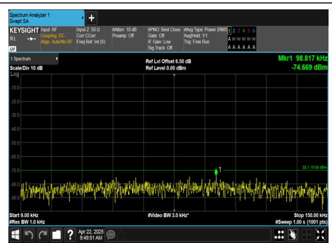
Band40(2305-2315)-10MHz-16QAM-38750-50RB#0-0.009~0.15-PASS
