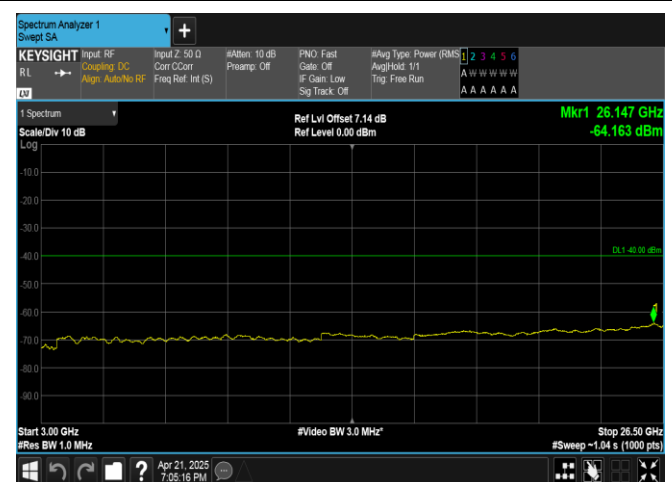
Band40(2305-2315)-5MHz-16QAM-38775-25RB#0-3000~26500-PASS
