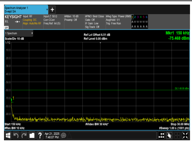
Band40(2305-2315)-10MHz-16QAM-38750-1RB#49-0.15~30-PASS
