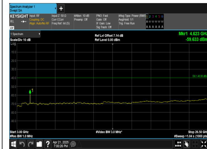
Band40(2305-2315)-5MHz-16QAM-38750-25RB#0-3000~26500-PASS
