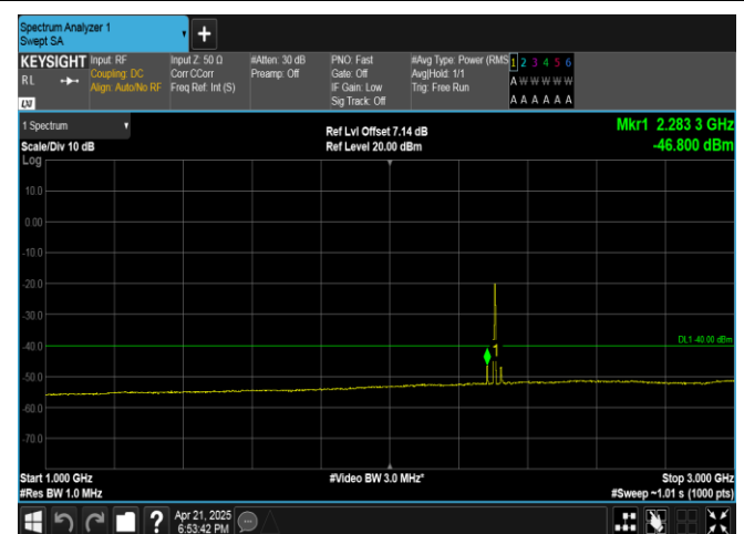
Band40(2305-2315)-5MHz-16QAM-38725-1RB#24-1000~3000-PASS
