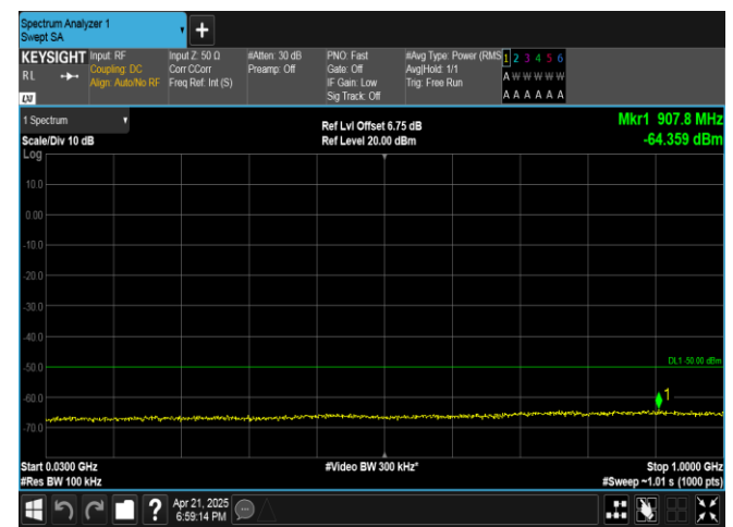
Band40(2305-2315)-5MHz-QPSK-38750-25RB#0-30~1000-PASS
