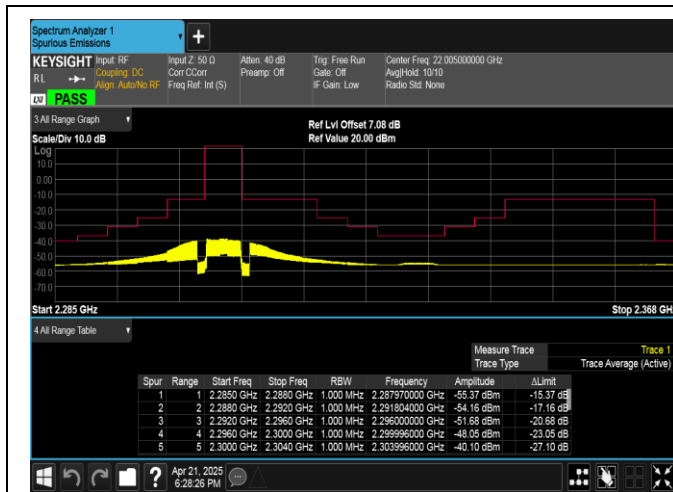
Band40(2305-2315)-5MHz-16QAM-38725-25RB#0-PASS
