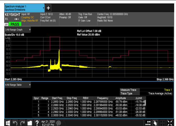
Band40(2305-2315)-5MHz-16QAM-38725-1RB#24-PASS
