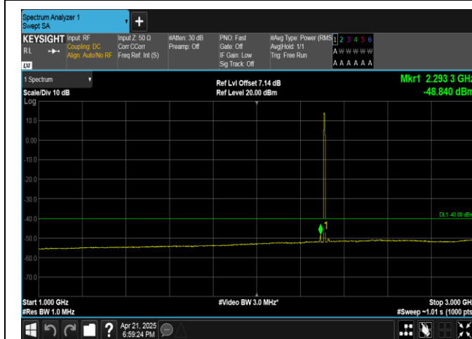
Band40(2305-2315)-5MHz-QPSK-38750-25RB#0-1000~3000-PASS
