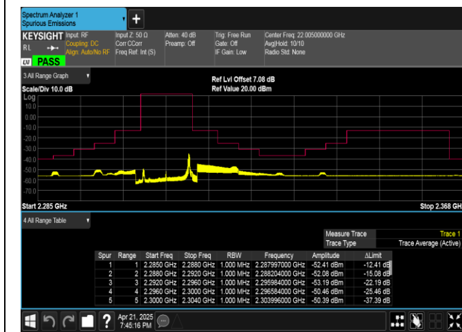
Band40(2305-2315)-10MHz-16QAM-38750-1RB#49-PASS
