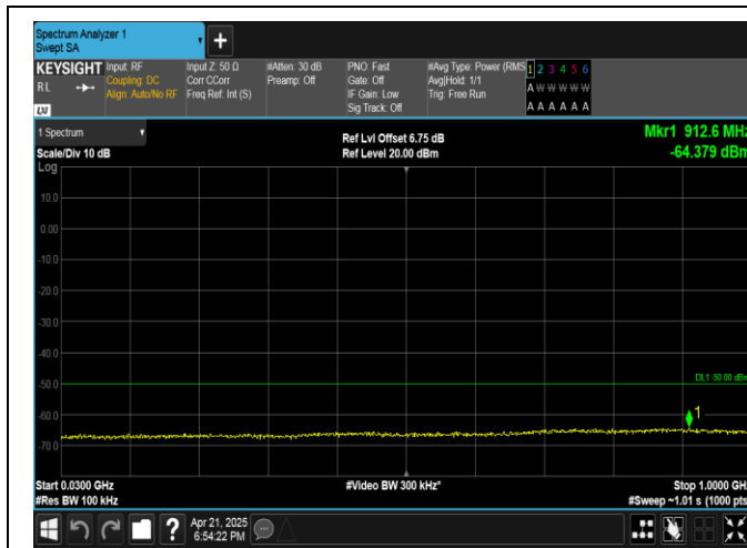
Band40(2305-2315)-5MHz-QPSK-38725-25RB#0-30~1000-PASS
