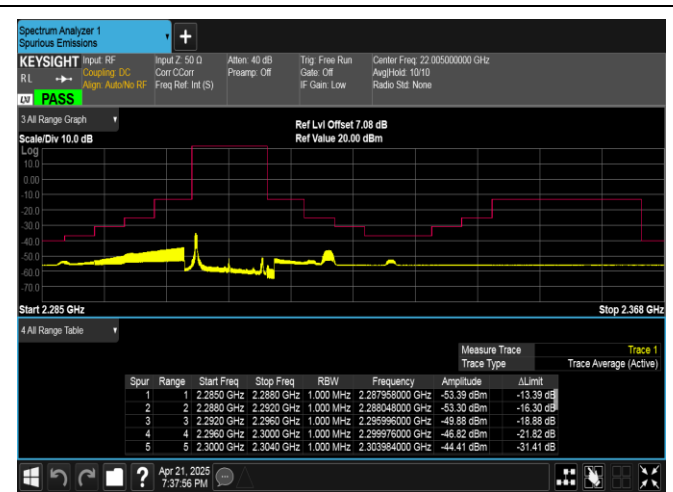
Band40(2305-2315)-10MHz-16QAM-38750-1RB#0-PASS
