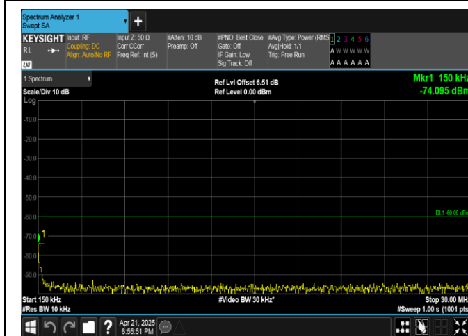
Band40(2305-2315)-5MHz-QPSK-38750-1RB#0-0.15~30-PASS
