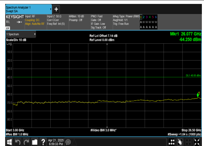
Band40(2305-2315)-5MHz-QPSK-38750-25RB#0-3000~26500-PASS
