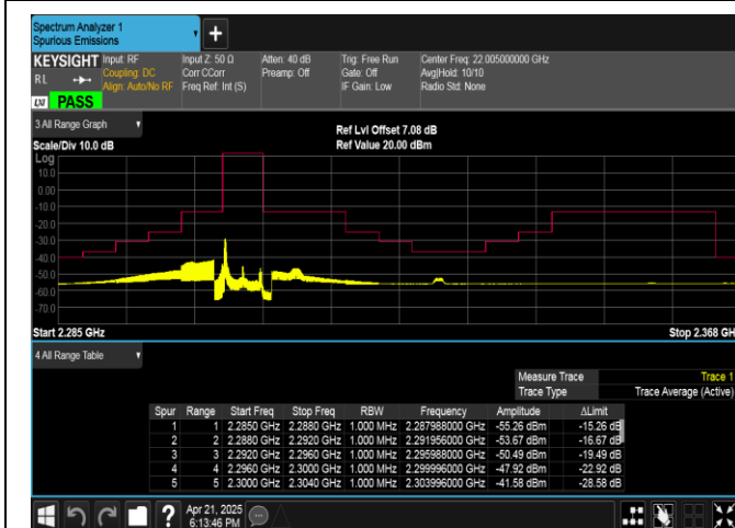
Band40(2305-2315)-5MHz-16QAM-38725-1RB#0-PASS
