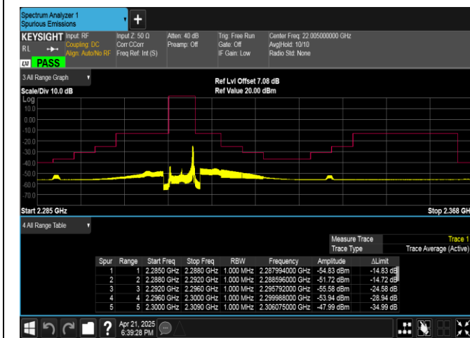
Band40(2305-2315)-5MHz-QPSK-38775-1RB#24-PASS
