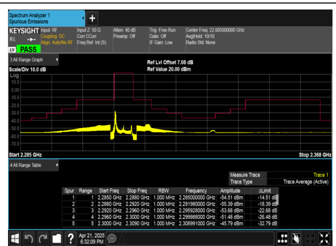
Band40(2305-2315)-5MHz-QPSK-38775-1RB#0-PASS
