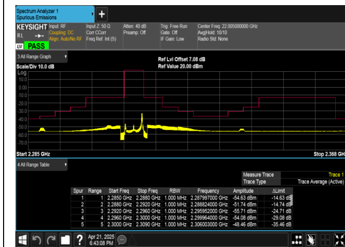
Band40(2305-2315)-5MHz-16QAM-38775-1RB#24-PASS
