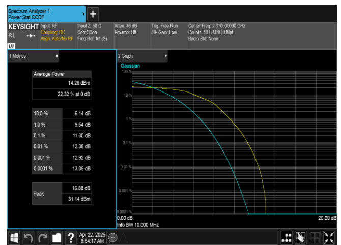
Band40(2305-2315)-10MHz-16QAM-38750-50RB#0-PASS
