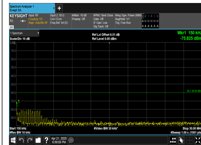
Band40(2305-2315)-5MHz-QPSK-38750-25RB#0-0.15~30-PASS
