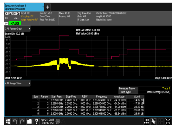
Band40(2305-2315)-5MHz-QPSK-38775-25RB#0-PASS
