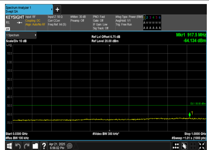
Band40(2305-2315)-5MHz-QPSK-38750-1RB#0-30~1000-PASS
