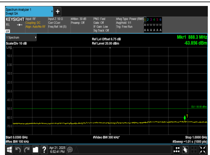
Band40(2305-2315)-5MHz-QPSK-38725-1RB#24-30~1000-PASS
