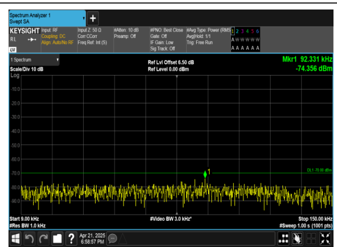
Band40(2305-2315)-5MHz-QPSK-38750-25RB#0-0.009~0.15-PASS
