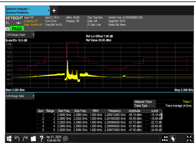
Band40(2305-2315)-5MHz-16QAM-38775-1RB#0-PASS
