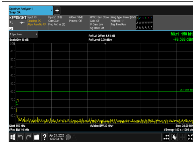
Band40(2305-2315)-5MHz-QPSK-38725-1RB#24-0.15~30-PASS
