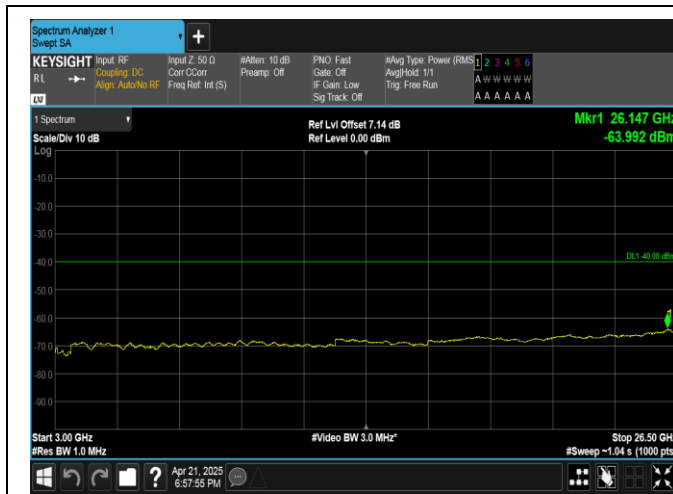
Band40(2305-2315)-5MHz-QPSK-38750-1RB#24-3000~26500-PASS
