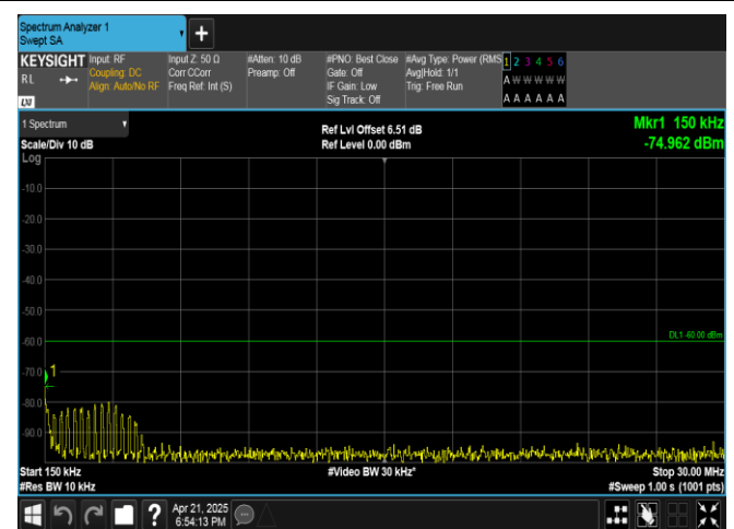
Band40(2305-2315)-5MHz-QPSK-38725-25RB#0-0.15~30-PASS
