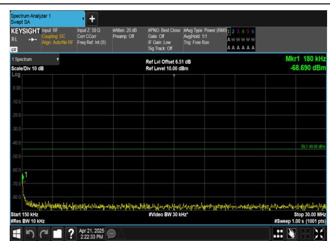
Band38-20MHz-QPSK-38000-1RB#99-0.15~30-PASS
