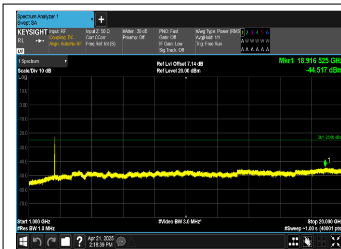
Band38-20MHz-QPSK-37850-1RB#99-1000~20000-PASS
