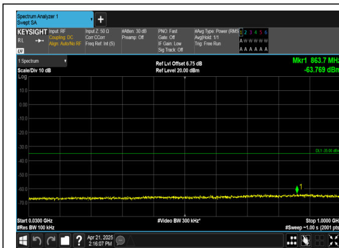
Band38-20MHz-QPSK-37850-1RB#0-30~1000-PASS
