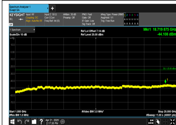
Band38-20MHz-16QAM-37850-1RB#0-1000~20000-PASS
