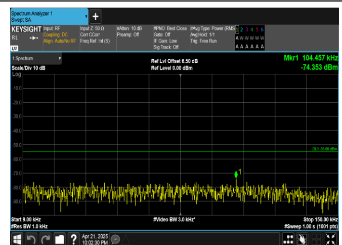
Band38-20MHz-QPSK-38000-100RB#0-0.009~0.15-PASS
