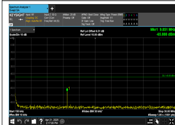
Band38-20MHz-16OAM-37850-1RB#0-0.15~30-PASS
