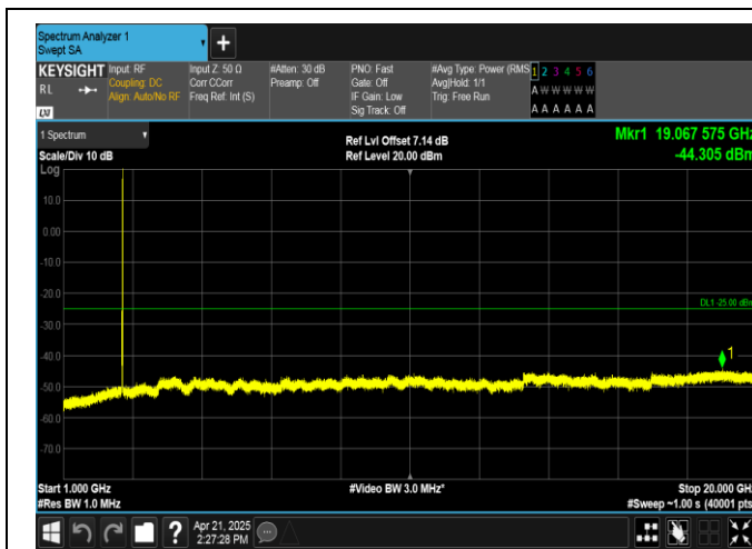
Band38-20MHz-QPSK-38150-1RB#99-1000~20000-PASS
