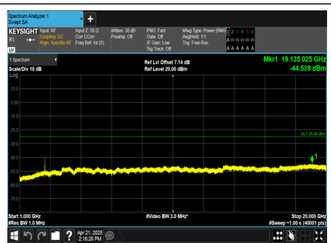
Band38-20MHz-QPSK-37850-1RB#0-1000~20000-PASS
