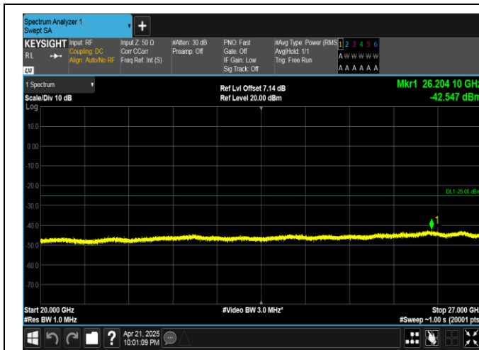
Band38-20MHz-QPSK-37850-100RB#0-20000~27000-PASS
