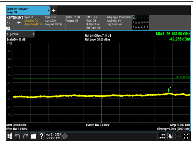
Band38-20MHz-16QAM-38000-1RB#99-20000~27000-PASS
