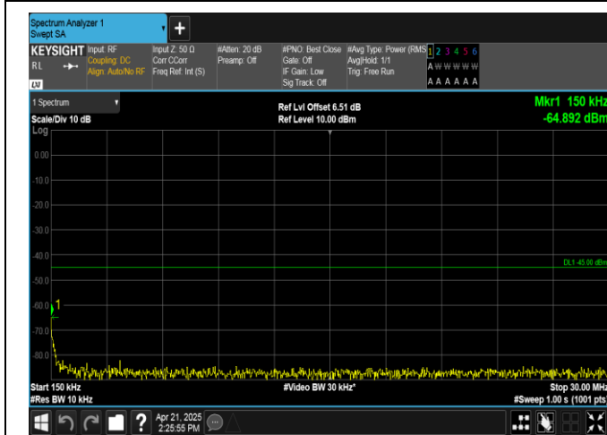
Band38-20MHz-16QAM-38150-1RB#0-0.15~30-PASS
