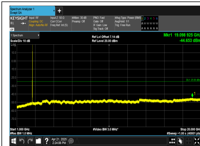
Band38-20MHz-16QAM-38000-1RB#99-1000~20000-PASS
