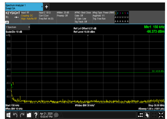
Band38-20MHz-16QAM-38000-100RB#0-0.15~30-PASS
