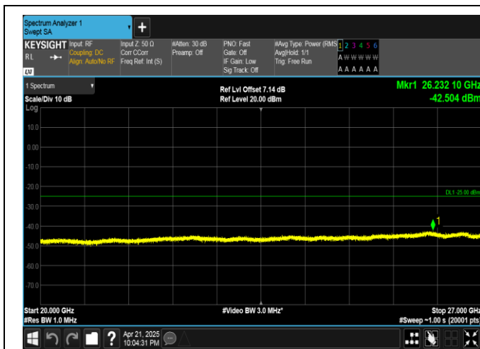
Band38-20MHz-16QAM-38000-100RB#0-20000~27000-PASS
