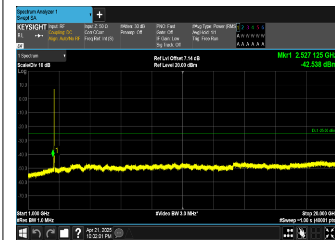
Band38-20MHz-16QAM-37850-100RB#0-1000~20000-PASS
