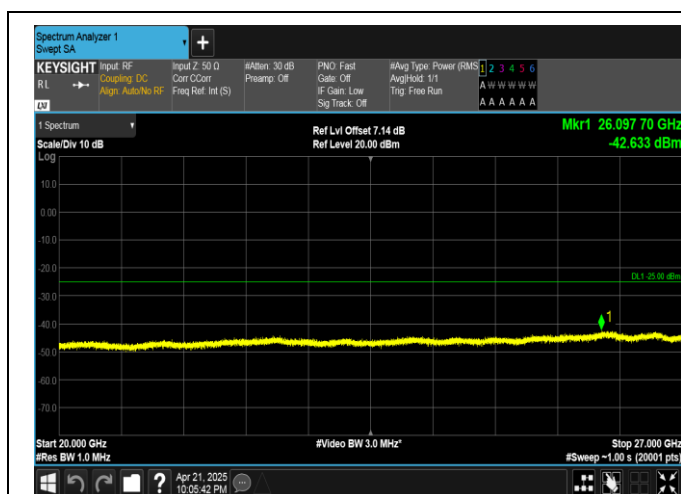
Band38-20MHz-OPSK-38150-100RB#0-20000~27000-PASS
