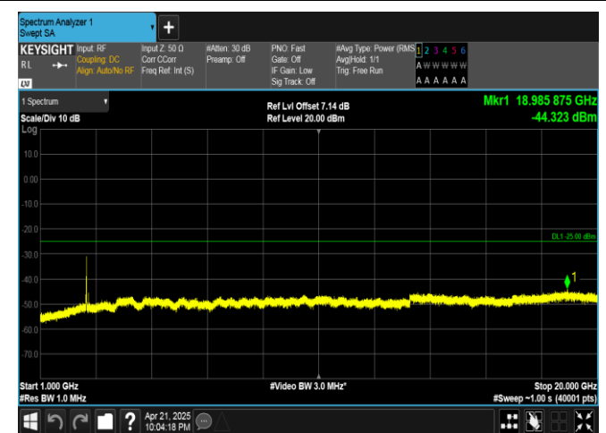
Band38-20MHz-16QAM-38000-100RB#0-1000~20000-PASS
