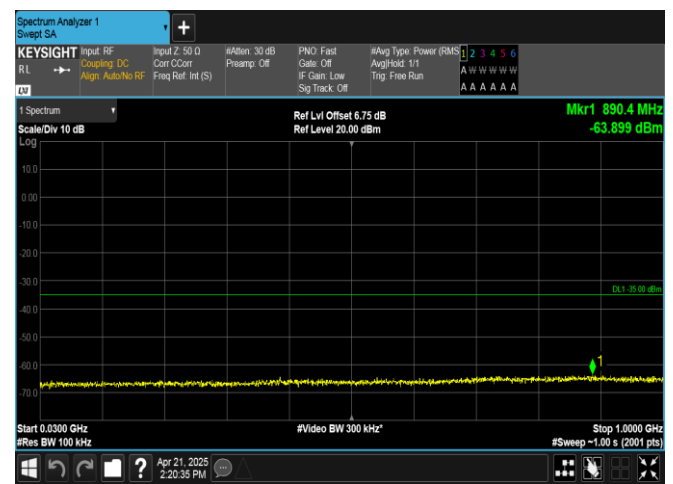
Band38-20MHz-QPSK-38000-1RB#0-30~1000-PASS
