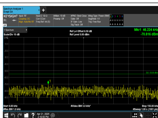
Band38-20MHz-16OAM-37850-1RB#0-0.009~0.15-PASS
