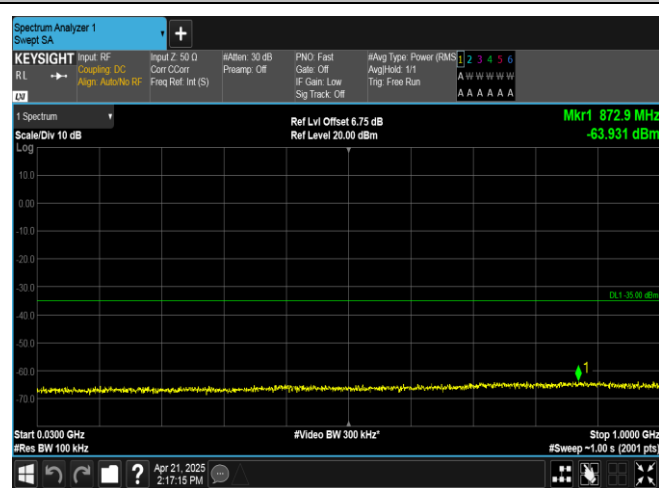
Band38-20MHz-16OAM-37850-1RB#0-30~1000-PASS
