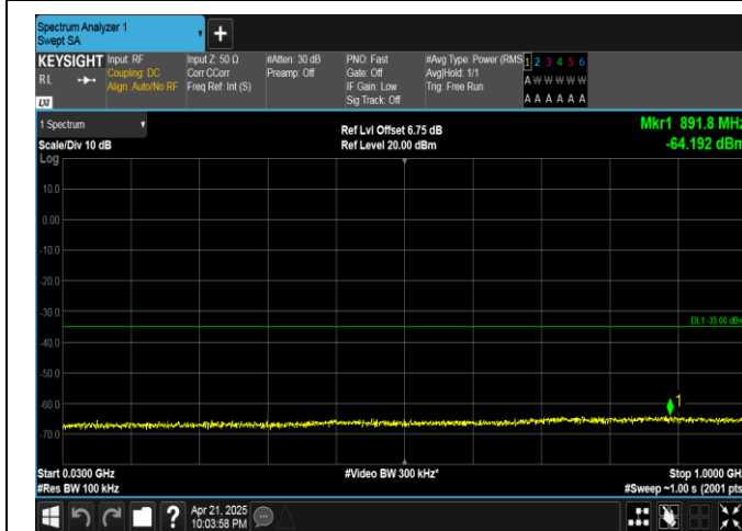
Band38-20MHz-16QAM-38000-100RB#0-30~1000-PASS
