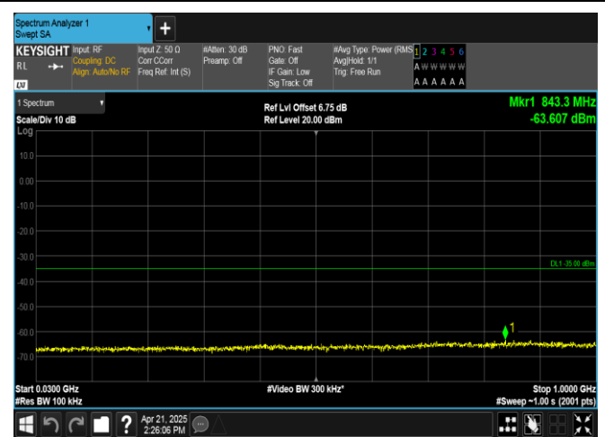
Band38-20MHz-16QAM-38150-1RB#0-30~1000-PASS
