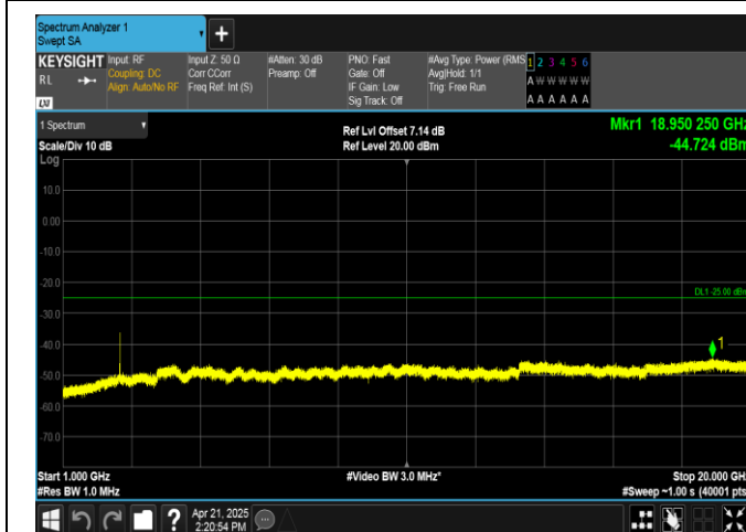
Band38-20MHz-QPSK-38000-1RB#0-1000~20000-PASS
