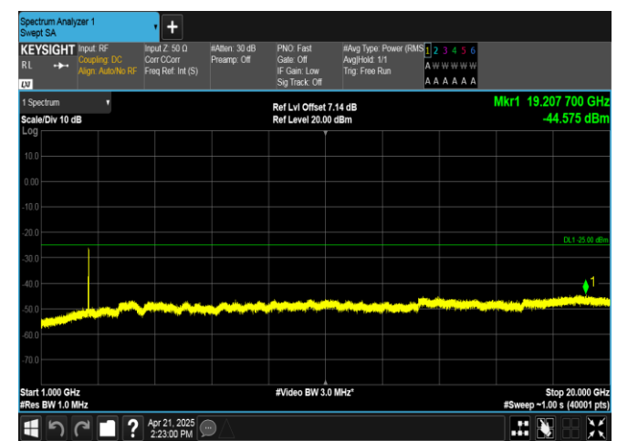
Band38-20MHz-QPSK-38000-1RB#99-1000~20000-PASS
