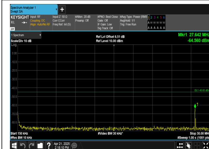
Band38-20MHz-QPSK-37850-1RB#99-0.15~30-PASS
