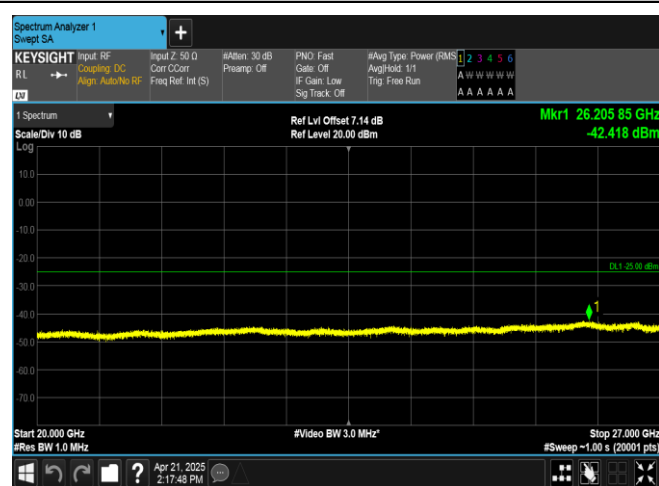
Band38-20MHz-16QAM-37850-1RB#0-20000~27000-PASS
