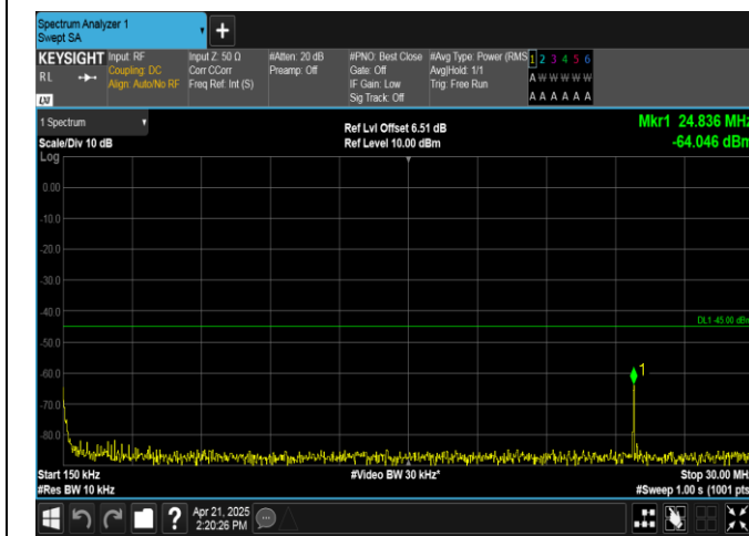
Band38-20MHz-QPSK-38000-1RB#0-0.15~30-PASS
