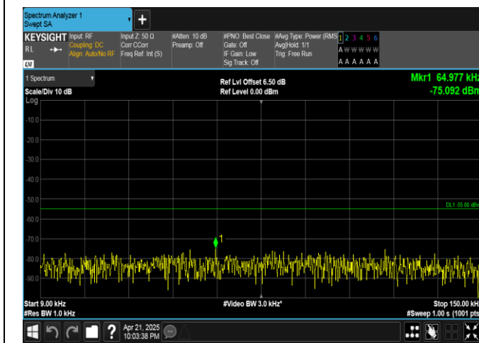
Band38-20MHz-16QAM-38000-100RB#0-0.009~0.15-PASS
