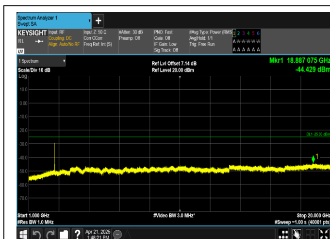
Band38-15MHz-OPSK-38175-1RB#74-1000~20000-PASS
