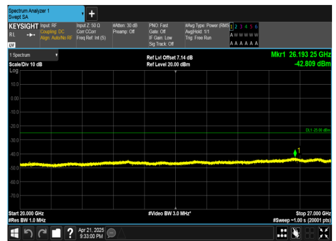
Band38-15MHz-QPSK-38000-75RB#0-20000~27000-PASS
