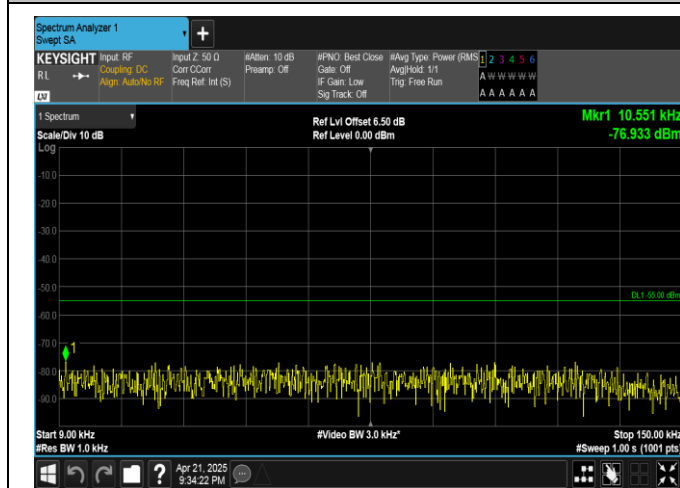
Band38-15MHz-OPSK-38175-75RB#0-0.009~0.15-PASS
