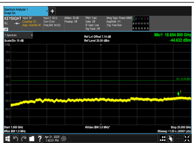
Band38-15MHz-16QAM-38000-1RB#0-1000~20000-PASS
