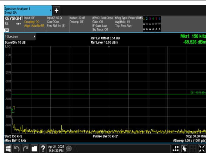
Band38-15MHz-OPSK-38175-75RB#0-0.15~30-PASS
