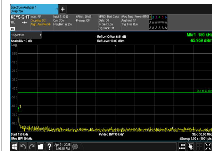
Band38-15MHz-16QAM-38175-1RB#0-0.15~30-PASS
