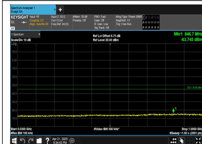
Band38-15MHz-QPSK-38175-75RB#0-30~1000-PASS
