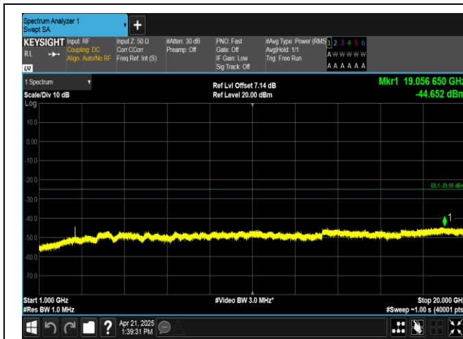
Band38-15MHz-QPSK-37825-1RB#74-1000~20000-PASS
