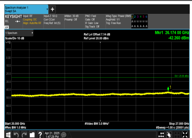
Band38-15MHz-16QAM-38175-1RB#0-20000~27000-PASS
