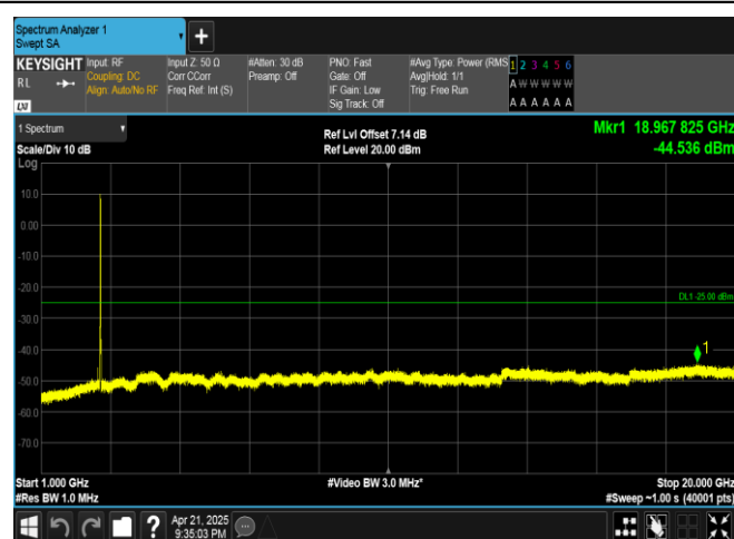
Band38-15MHz-QPSK-38175-75RB#0-1000~20000-PASS
