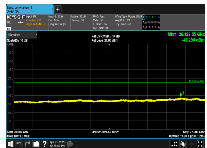
Band38-10MHz-16QAM-37800-1RB#0-20000~27000-PASS
