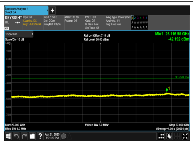
Band38-10MHz-16QAM-38000-1RB#49-20000~27000-PASS
