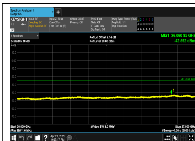
Band38-10MHz-16OAM-38000-50RB#0-20000~27000-PASS
