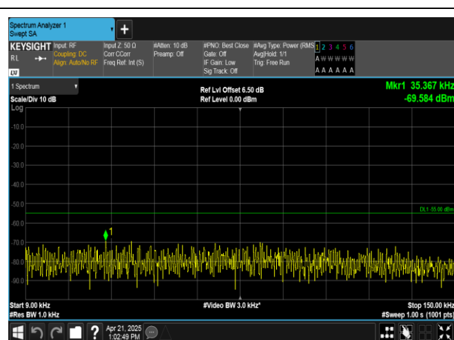
Band38-10MHz-16OAM-38200-1RB#0-0.009~0.15-PASS
