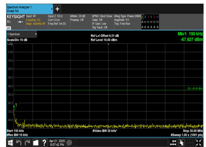
Band38-10MHz-QPSK-38200-50RB#0-0.15~30-PASS
