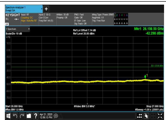
Band38-10MHz-QPSK-37800-1RB#49-20000~27000-PASS
