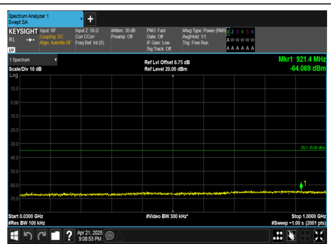
Band38-10MHz-16QAM-38200-50RB#0-30~1000-PASS
