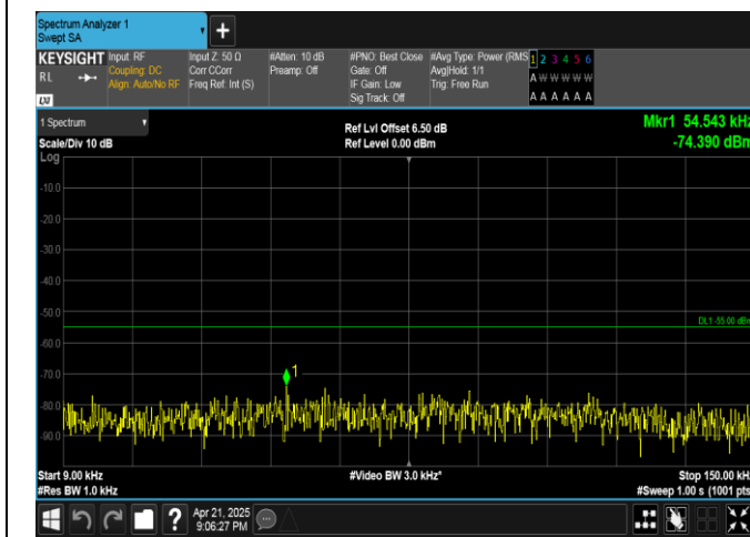
Band38-10MHz-16QAM-38000-50RB#0-0.009~0.15-PASS
