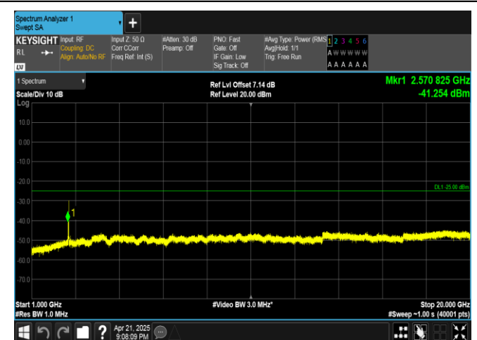
Band38-10MHz-QPSK-38200-50RB#0-1000~20000-PASS
