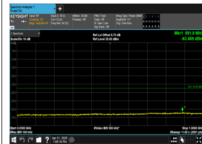
Band38-10MHz-16QAM-38200-1RB#49-30~1000-PASS
