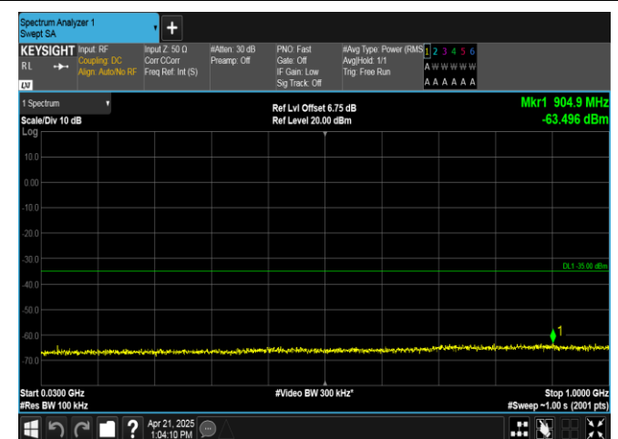
Band38-10MHz-QPSK-38200-1RB#49-30~1000-PASS
