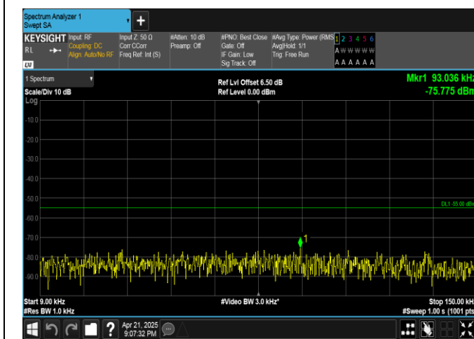
Band38-10MHz-QPSK-38200-50RB#0-0.009~0.15-PASS
