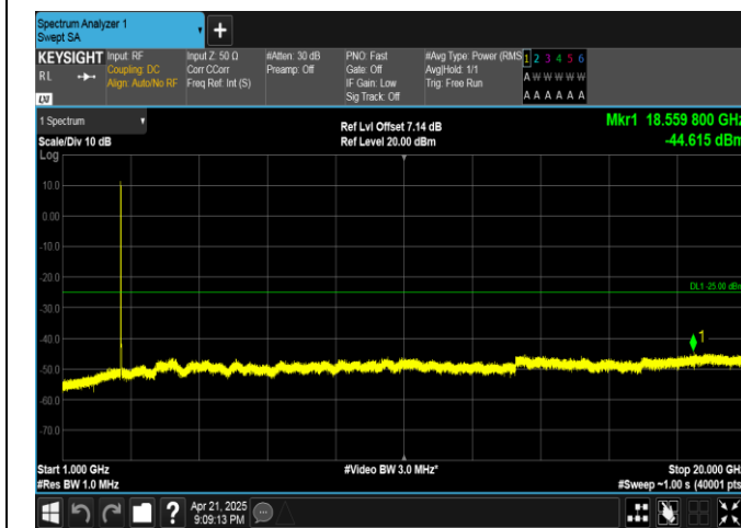
Band38-10MHz-16QAM-38200-50RB#0-1000~20000-PASS
