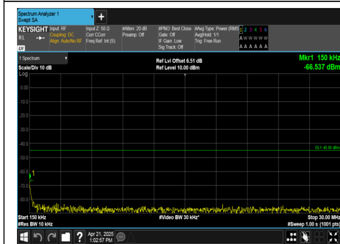
Band38-10MHz-16OAM-38200-1RB#0-0.15~30-PASS
