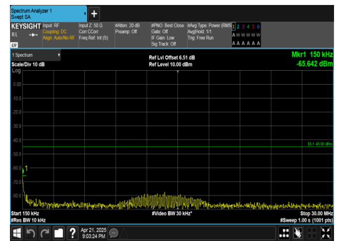
Band38-10MHz-QPSK-37800-50RB#0-0.15~30-PASS
