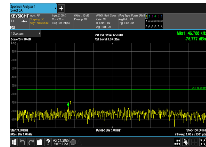
Band38-10MHz-QPSK-37800-50RB#0-0.009~0.15-PASS
