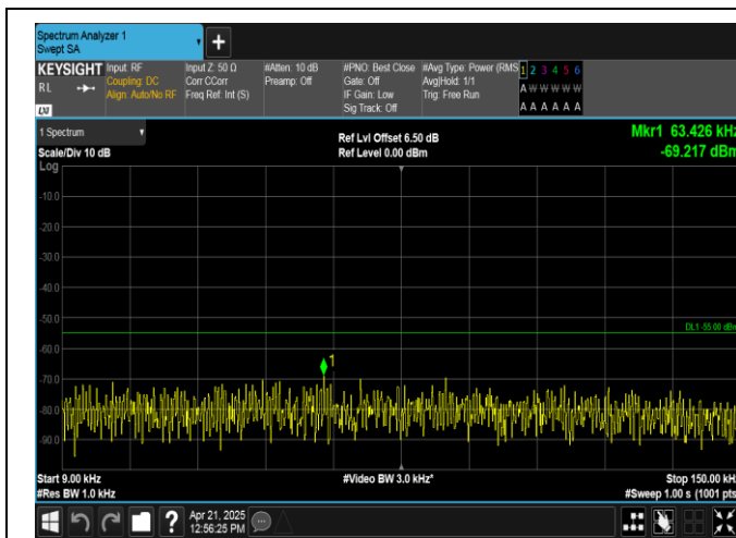
Band38-10MHz-16QAM-37800-1RB#49-0.009~0.15-PASS
