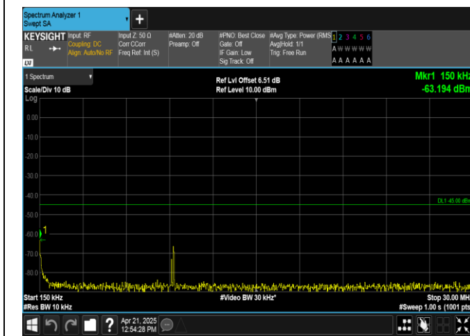
Band38-10MHz-16QAM-37800-1RB#0-0.15~30-PASS
