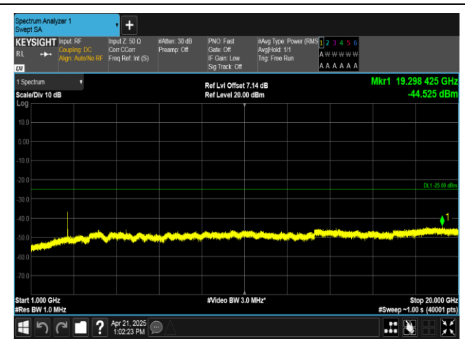
Band38-10MHz-QPSK-38200-1RB#0-1000~20000-PASS
