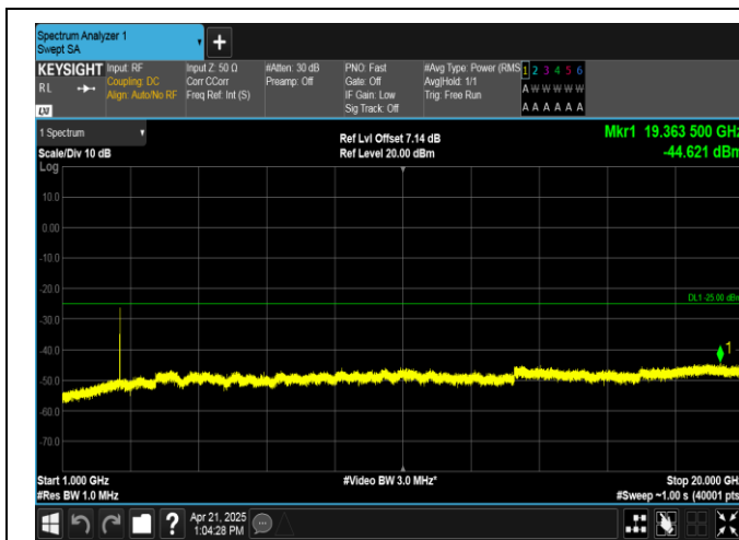
Band38-10MHz-QPSK-38200-1RB#49-1000~20000-PASS
