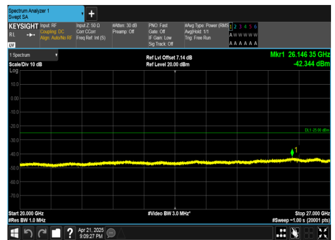
Band38-10MHz-16QAM-38200-50RB#0-20000~27000-PASS
