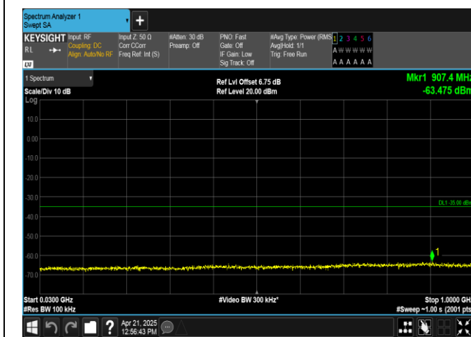
Band38-10MHz-16QAM-37800-1RB#49-30~1000-PASS
