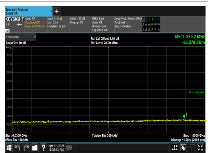
Band38-10MHz-QPSK-38000-50RB#0-30~1000-PASS
