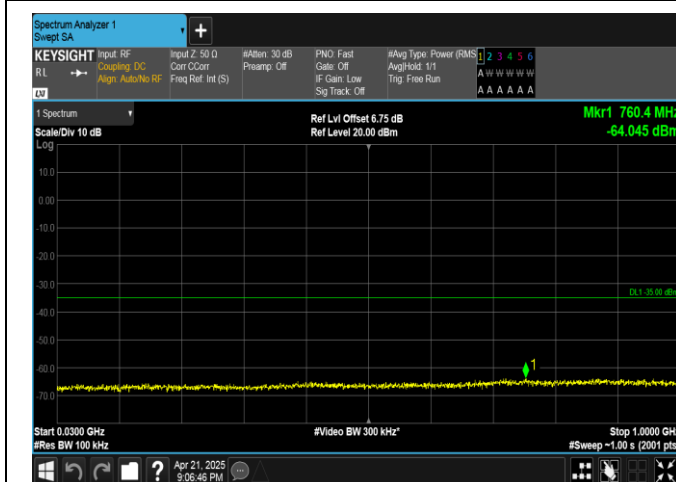
Band38-10MHz-16QAM-38000-50RB#0-30~1000-PASS
