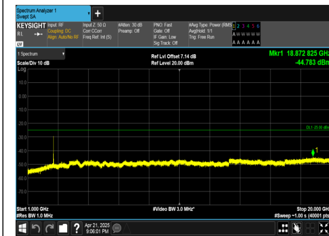
Band38-10MHz-QPSK-38000-50RB#0-1000~20000-PASS
