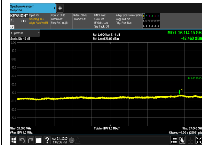
Band38-10MHz-QPSK-38200-1RB#0-20000~27000-PASS
