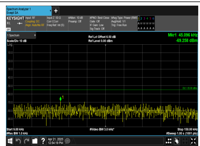
Band38-10MHz-16QAM-37800-1RB#0-0.009~0.15-PASS
