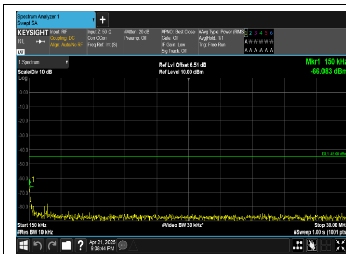
Band38-10MHz-16QAM-38200-50RB#0-0.15~30-PASS
