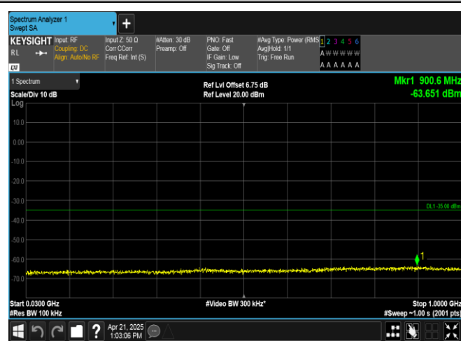
Band38-10MHz-16OAM-38200-1RB#0-30~1000-PASS
