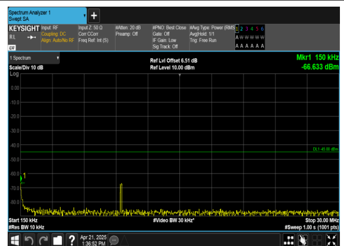
Band38-15MHz-QPSK-37825-1RB#0-0.15~30-PASS
