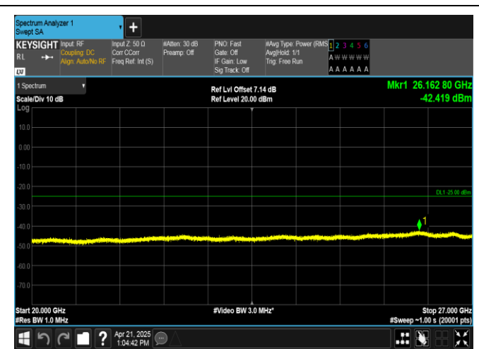
Band38-10MHz-QPSK-38200-1RB#49-20000~27000-PASS
