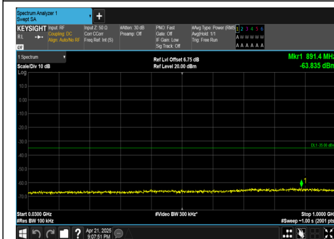
Band38-10MHz-QPSK-38200-50RB#0-30~1000-PASS
