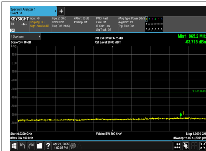
Band38-10MHz-QPSK-38200-1RB#0-30~1000-PASS
