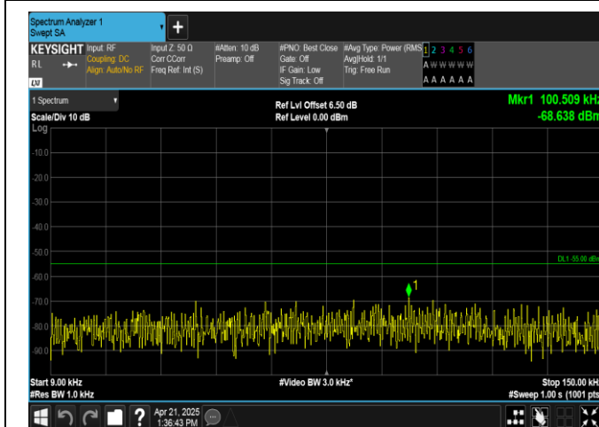
Band38-15MHz-QPSK-37825-1RB#0-0.009~0.15-PASS
