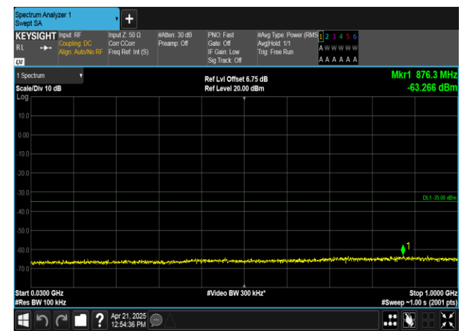
Band38-10MHz-16QAM-37800-1RB#0-30~1000-PASS
