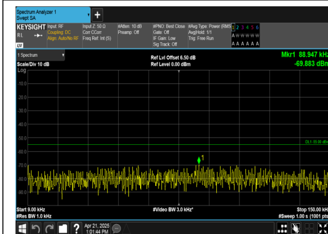
Band38-10MHz-QPSK-38200-1RB#0-0.009~0.15-PASS
