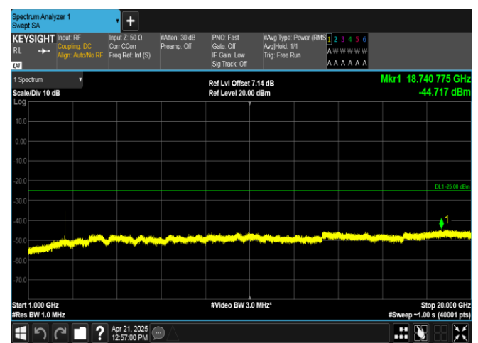
Band38-10MHz-16QAM-37800-1RB#49-1000~20000-PASS
