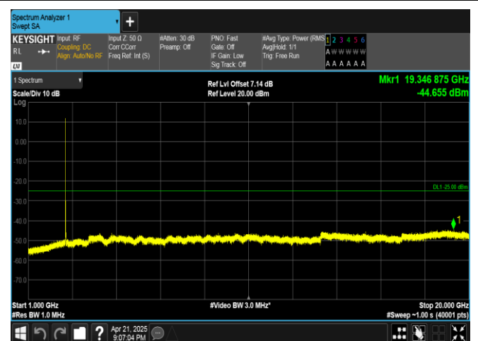
Band38-10MHz-16QAM-38000-50RB#0-1000~20000-PASS
