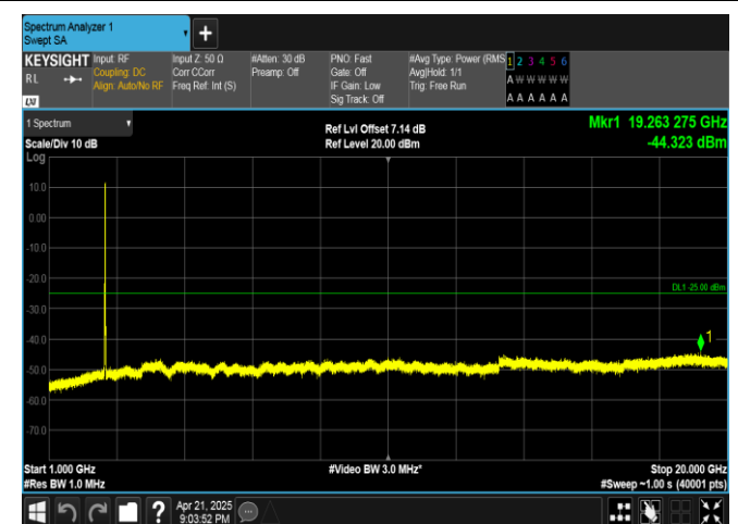
Band38-10MHz-QPSK-37800-50RB#0-1000~20000-PASS
