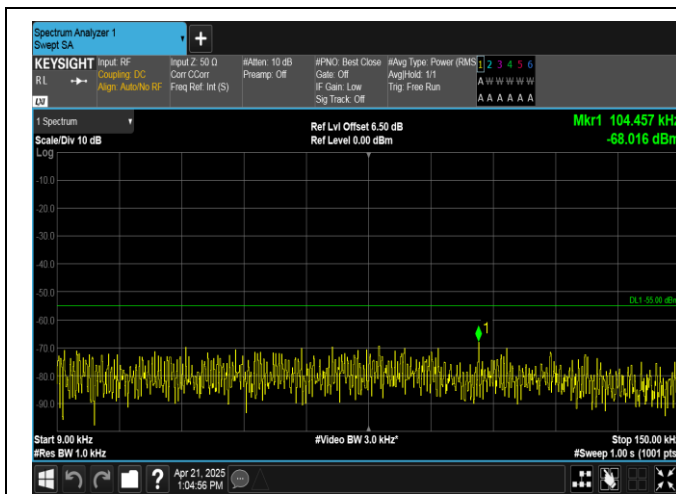
Band38-10MHz-16QAM-38200-1RB#49-0.009~0.15-PASS
