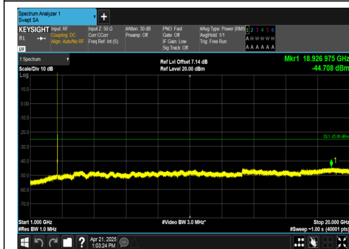
Band38-10MHz-16QAM-38200-1RB#0-1000~20000-PASS
