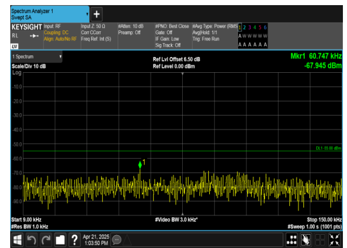
Band38-10MHz-QPSK-38200-1RB#49-0.009~0.15-PASS
