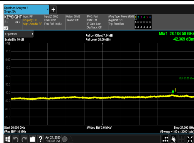
Band38-10MHz-16QAM-38200-1RB#0-20000~27000-PASS
