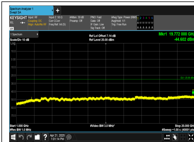
Band38-10MHz-16QAM-38000-1RB#49-1000~20000-PASS
