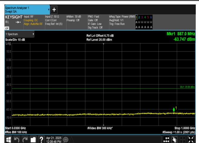
Band38-5MHz-QPSK-38225-1RB#24-30~1000-PASS
