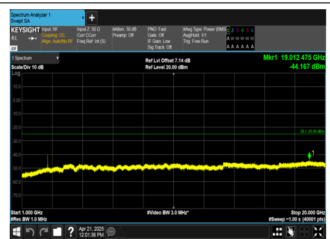
Band38-5MHz-16QAM-38000-1RB#0-1000~20000-PASS
