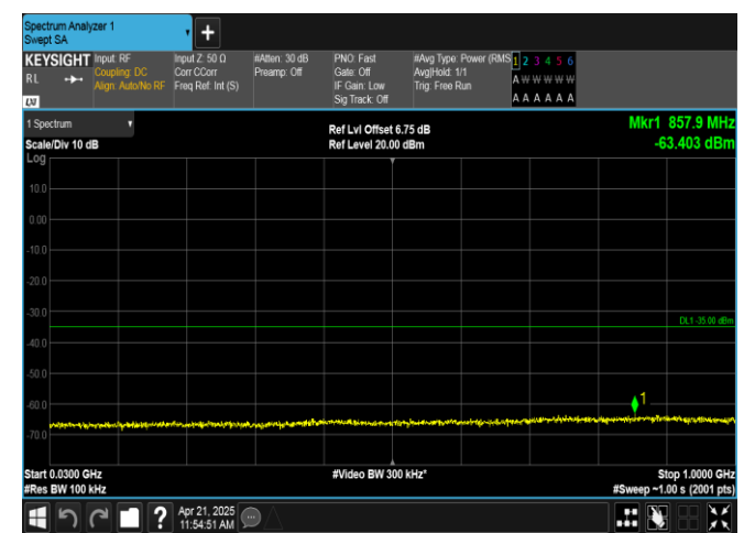
Band38-5MHz-16QAM-37775-1RB#0-30~1000-PASS
