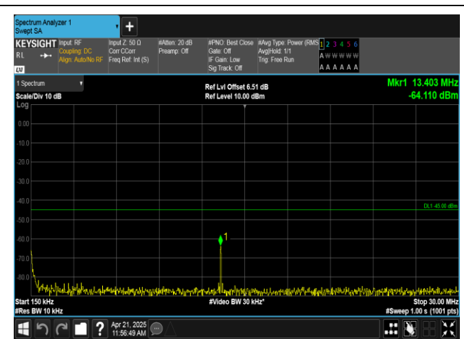
Band38-5MHz-16QAM-37775-1RB#24-0.15~30-PASS
