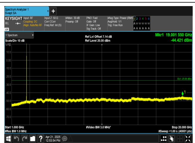
Band38-10MHz-QPSK-37800-1RB#0-1000~20000-PASS
