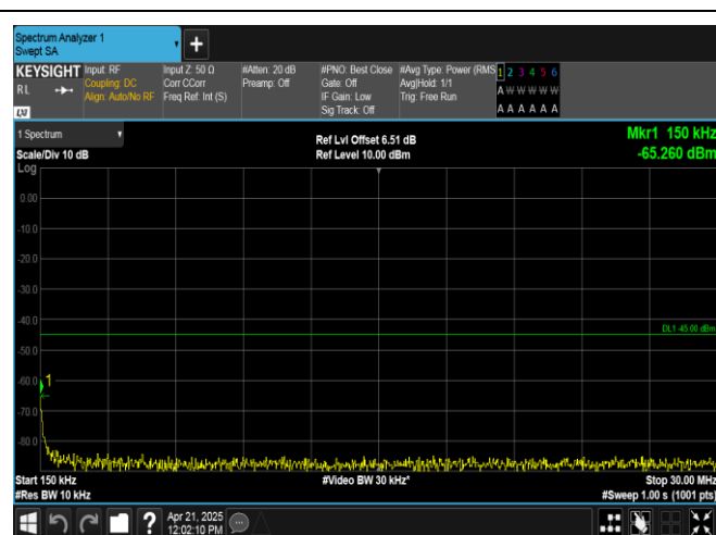
Band38-5MHz-OPSK-38000-1RB#24-0.15~30-PASS
