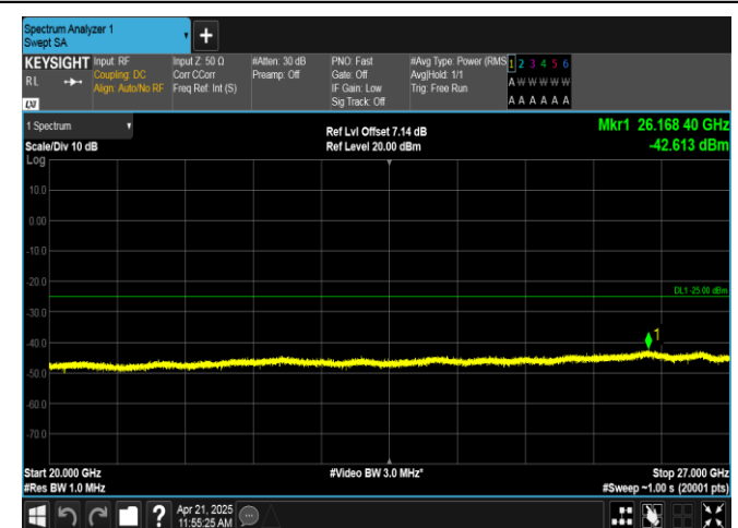
Band38-5MHz-16QAM-37775-1RB#0-20000~27000-PASS
