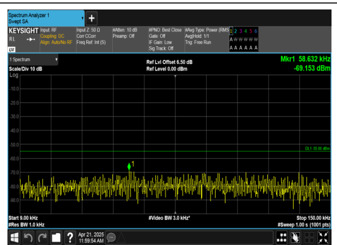
Band38-5MHz-QPSK-38000-1RB#0-0.009~0.15-PASS
