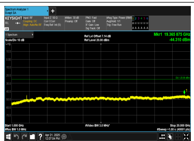
Band38-5MHz-QPSK-38225-1RB#0-1000~20000-PASS
