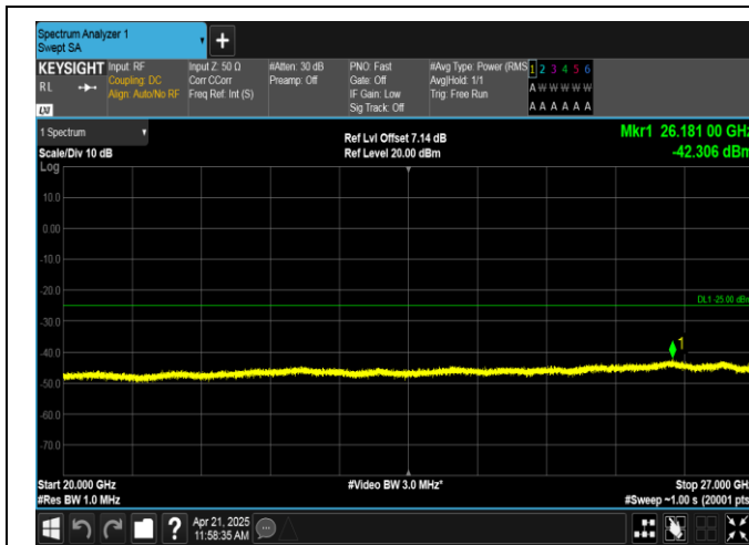
Band38-5MHz-QPSK-37775-25RB#0-20000~27000-PASS
