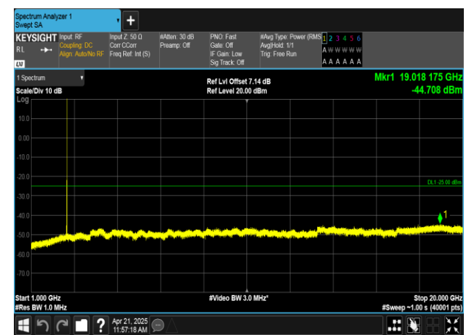
Band38-5MHz-16QAM-37775-1RB#24-1000~20000-PASS
