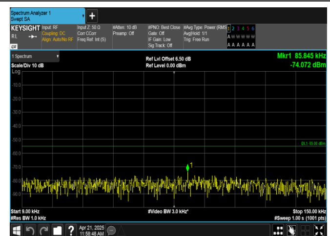
Band38-5MHz-16QAM-37775-25RB#0-0.009~0.15-PASS
