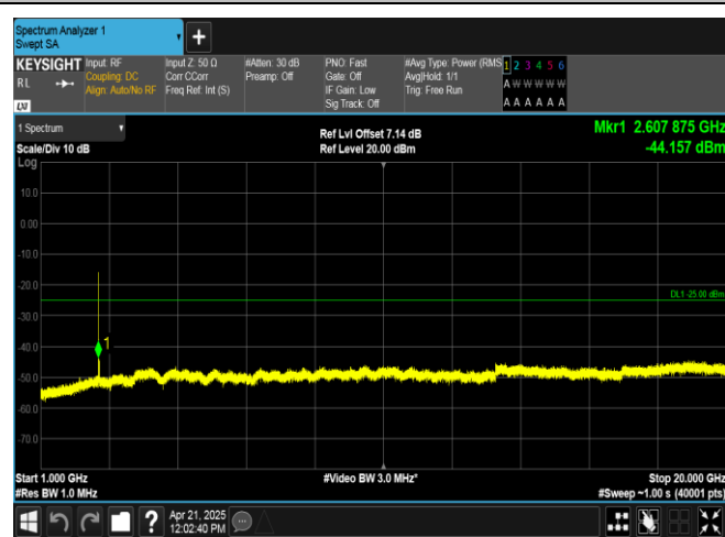
Band38-5MHz-QPSK-38000-1RB#24-1000~20000-PASS
