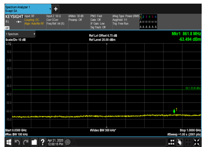
Band38-5MHz-QPSK-38000-1RB#0-30~1000-PASS
