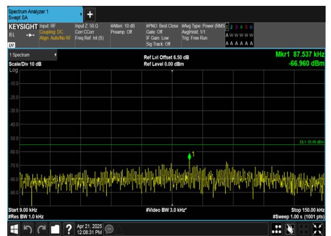
Band38-5MHz-QPSK-38225-1RB#24-0.009~0.15-PASS
