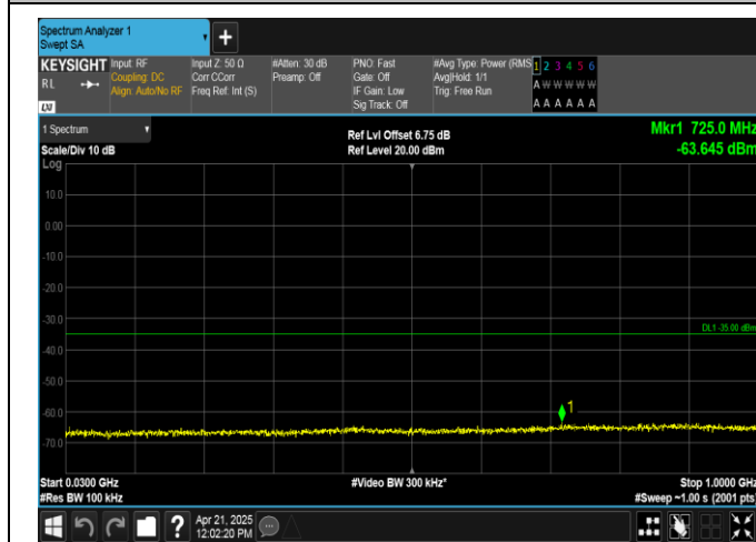
Band38-5MHz-QPSK-38000-1RB#24-30~1000-PASS
