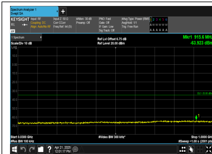
Band38-5MHz-16QAM-38000-1RB#0-30~1000-PASS
