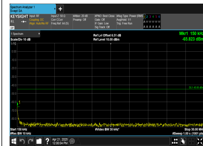
Band38-5MHz-QPSK-38000-1RB#0-0.15~30-PASS
