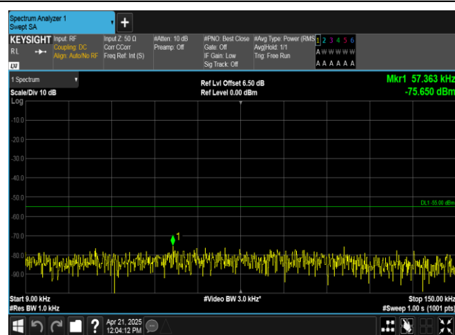
Band38-5MHz-QPSK-38000-25RB#0-0.009~0.15-PASS
