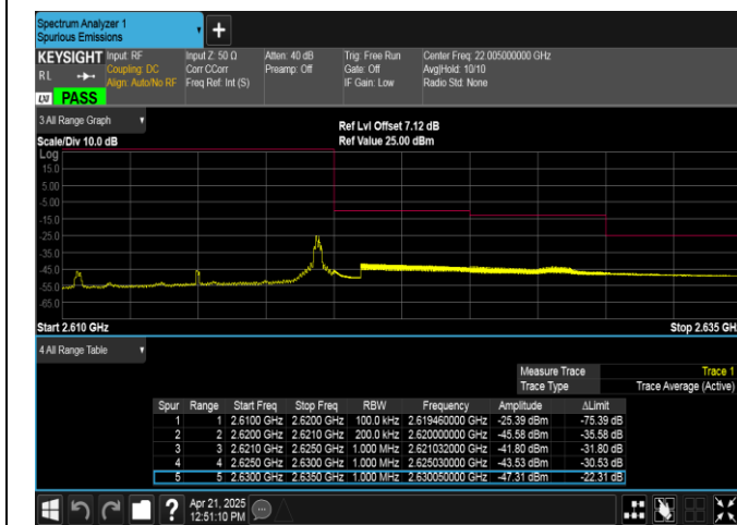
Band38-10MHz-QPSK-38200-1RB#49-PASS
