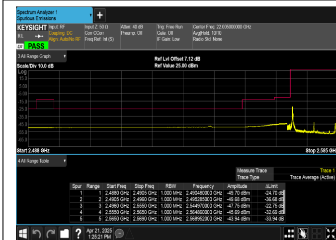
Band38-15MHz-16QAM-37825-1RB#0-PASS
