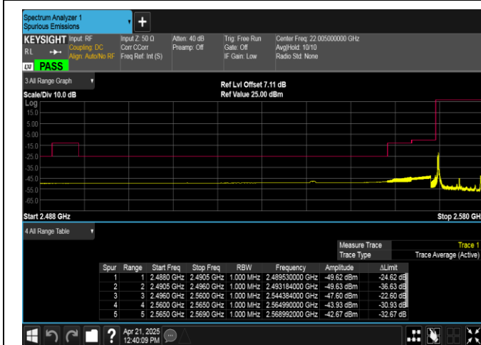
Band38-10MHz-QPSK-37800-1RB#0-PASS
