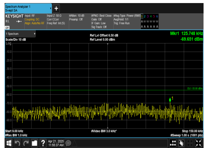
Band38-5MHz-QPSK-37775-1RB#24-0.009~0.15-PASS
