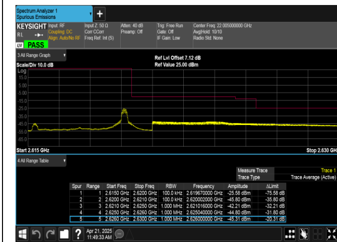
Band38-5MHz-16QAM-38225-1RB#24-PASS
