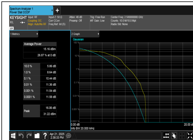
Band38-20MHz-16QAM-37850-1RB#0-PASS
