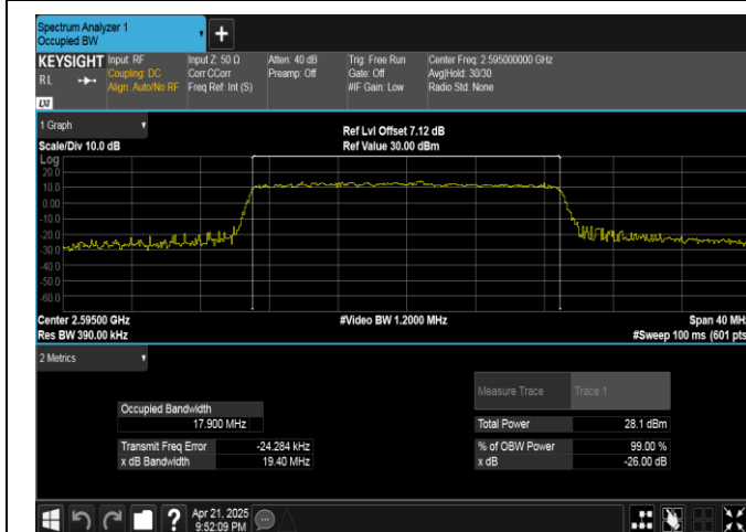
Band38-20MHz-16QAM-38000-100RB#0-PASS
