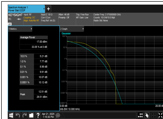
Band38-10MHz-QPSK-37800-1RB#0-PASS
