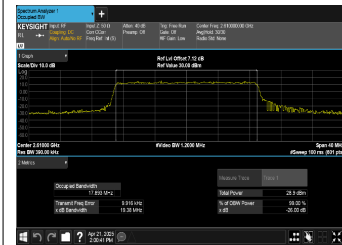
Band38-20MHz-QPSK-38150-100RB#0-PASS
