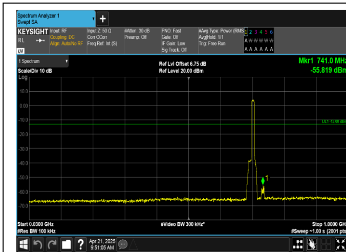
Band17-10MHz-QPSK-23800-50RB#0-30~1000-PASS
