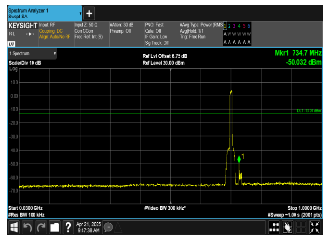
Band17-10MHz-16QAM-23780-50RB#0-30~1000-PASS
