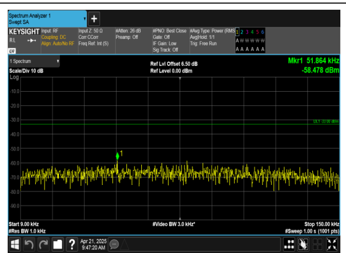
Band17-10MHz-16QAM-23780-50RB#0-0.009~0.15-PASS
