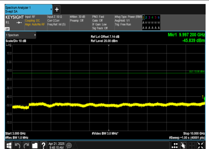
Band17-10MHz-16QAM-23780-50RB#0-3000~10000-PASS
