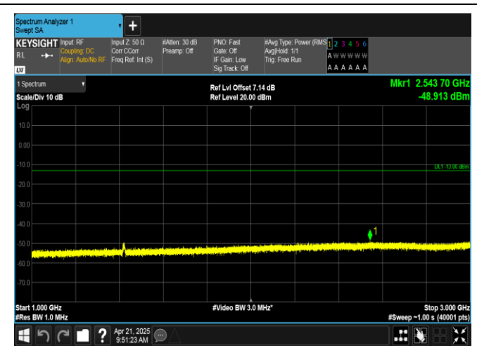
Band17-10MHz-QPSK-23800-50RB#0-1000~3000-PASS
