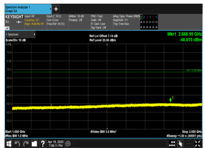
Band17-10MHz-QPSK-23800-1RB#0-1000~3000-PASS
