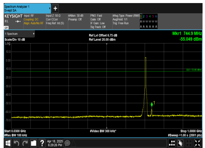
Band17-5MHz-16QAM-23825-25RB#0-30~1000-PASS
