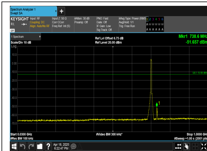
Band17-5MHz-16QAM-23790-25RB#0-30~1000-PASS
