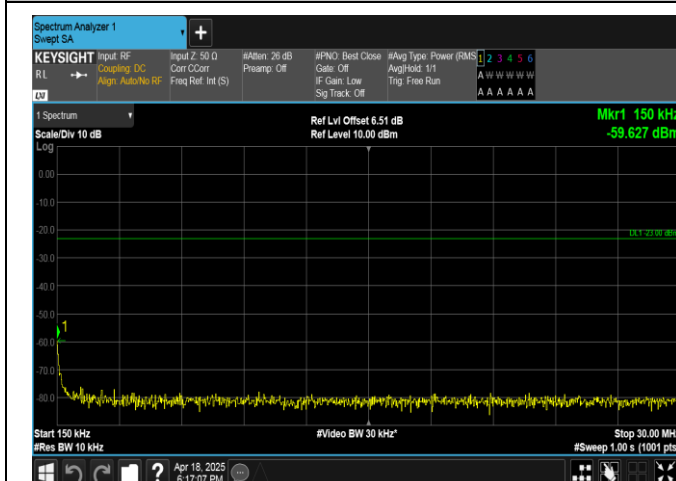
Band17-5MHz-QPSK-23790-1RB#0-0.15~30-PASS
