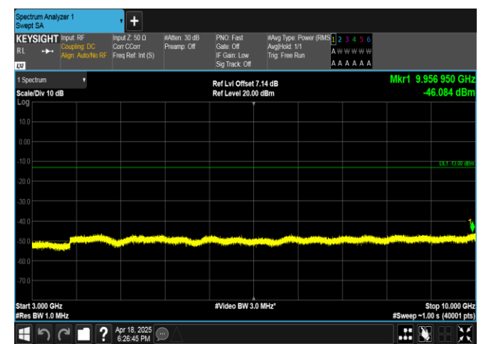
Band17-5MHz-QPSK-23825-1RB#24-3000~10000-PASS
