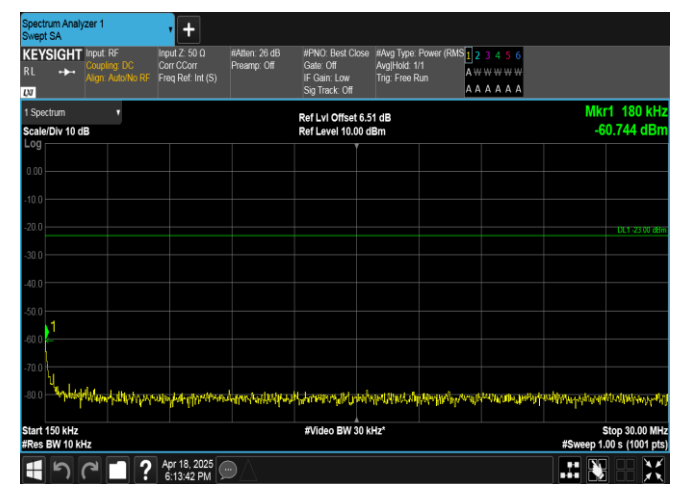
Band17-5MHz-16QAM-23755-1RB#24-0.15~30-PASS
