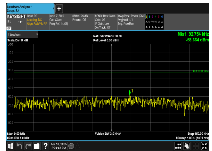
Band17-5MHz-16QAM-23825-1RB#0-0.009~0.15-PASS
