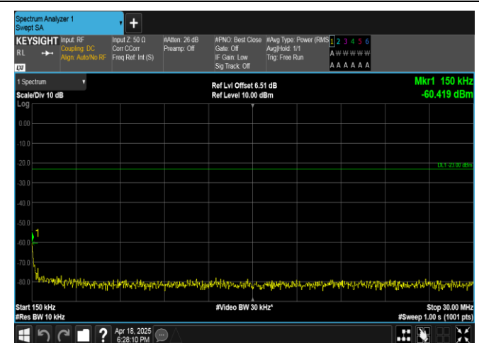
Band17-5MHz-QPSK-23825-25RB#0-0.15~30-PASS
