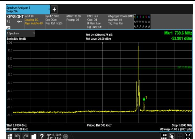
Band17-5MHz-QPSK-23790-1RB#0-30~1000-PASS
