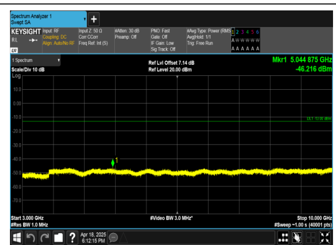
Band17-5MHz-16QAM-23755-1RB#0-3000~10000-PASS
