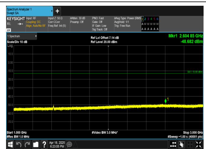
Band17-5MHz-16QAM-23790-25RB#0-1000~3000-PASS
