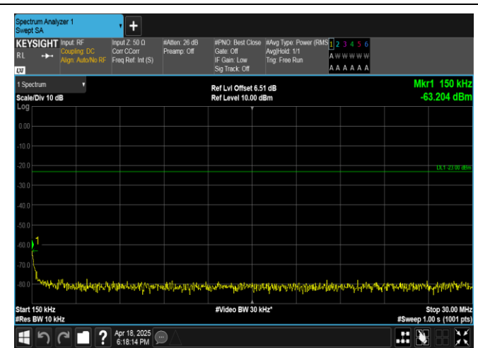
Band17-5MHz-16QAM-23790-1RB#0-0.15~30-PASS
