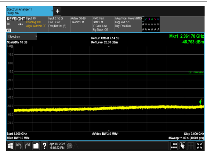
Band17-5MHz-QPSK-23755-25RB#0-1000~3000-PASS
