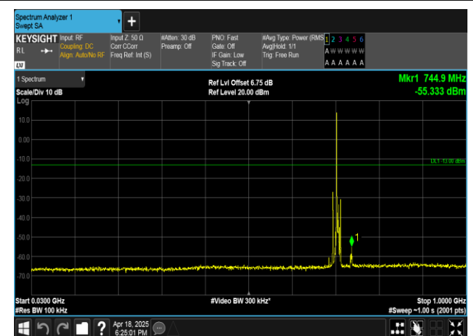
Band17-5MHz-16QAM-23825-1RB#0-30~1000-PASS
