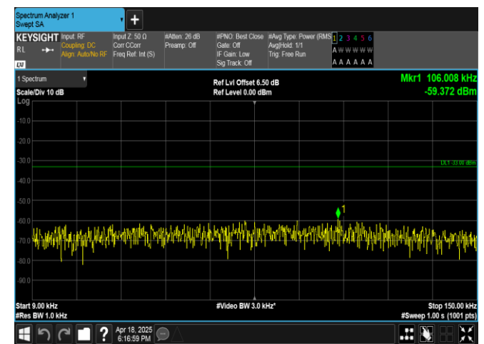
Band17-5MHz-QPSK-23790-1RB#0-0.009~0.15-PASS
