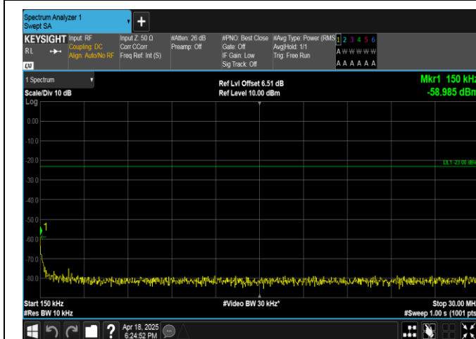
Band17-5MHz-16QAM-23825-1RB#0-0.15~30-PASS
