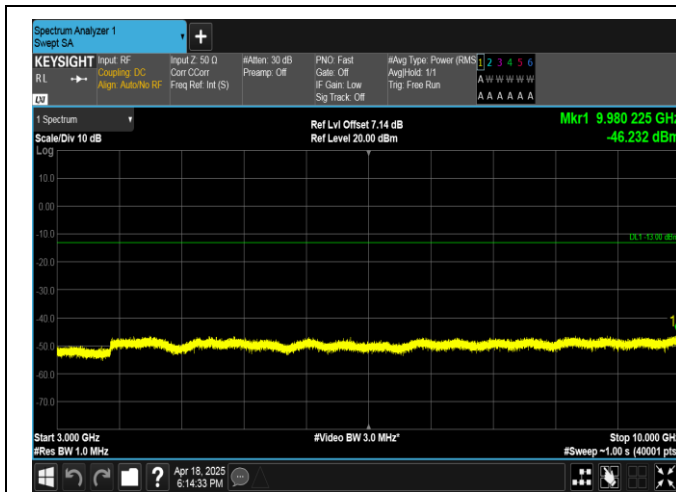
Band17-5MHz-16QAM-23755-1RB#24-3000~10000-PASS
