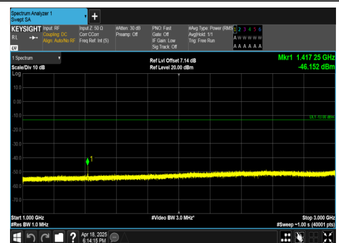
Band17-5MHz-16QAM-23755-1RB#24-1000~3000-PASS
