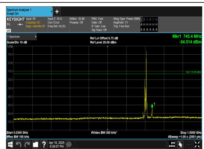
Band17-5MHz-QPSK-23825-1RB#24-30~1000-PASS
