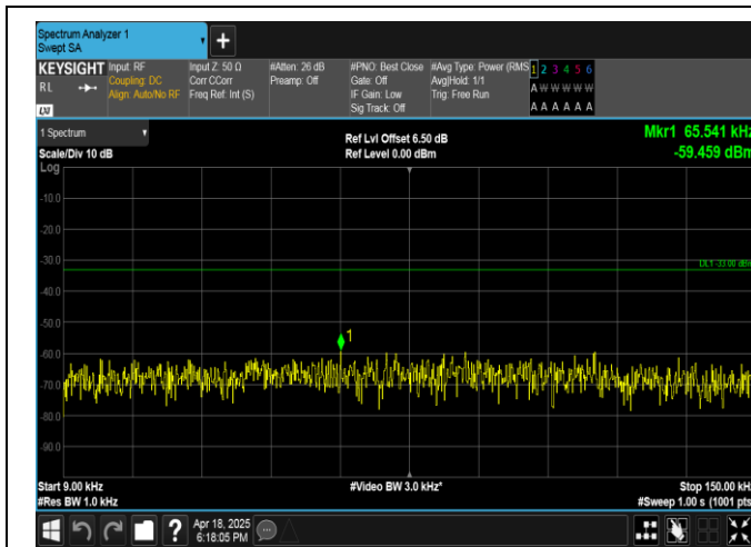
Band17-5MHz-16QAM-23790-1RB#0-0.009~0.15-PASS
