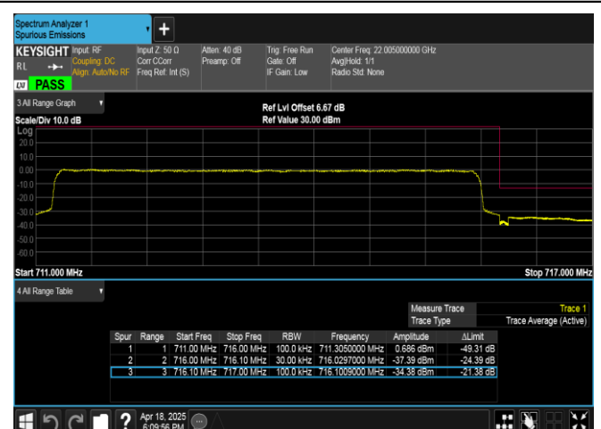
Band17-5MHz-16QAM-23825-25RB#0-PASS
