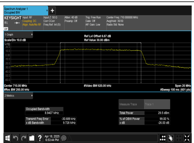
Band17-10MHz-QPSK-23790-50RB#0-PASS
