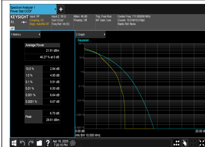
Band17-10MHz-16QAM-23800-1RB#0-PASS
