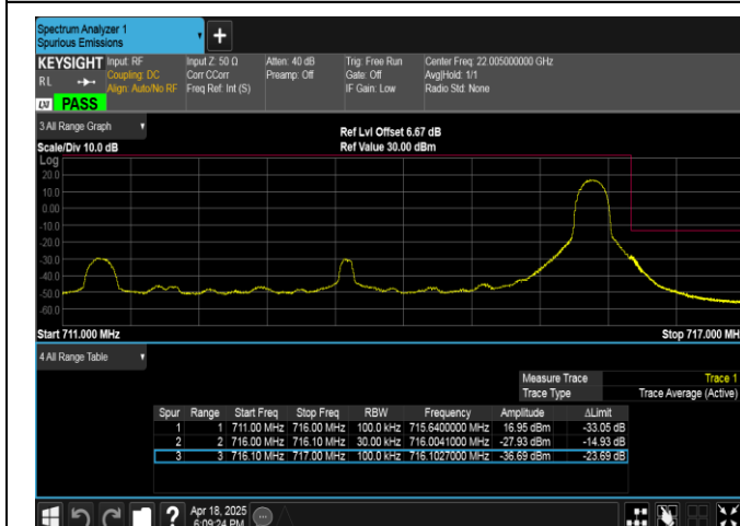
Band17-5MHz-16QAM-23825-1RB#24-PASS
