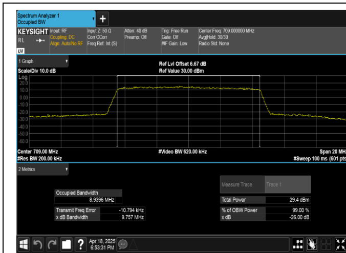
Band17-10MHz-QPSK-23780-50RB#0-PASS
