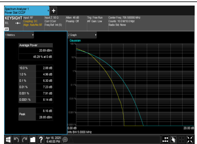
Band17-5MHz-16QAM-23755-25RB#0-PASS
