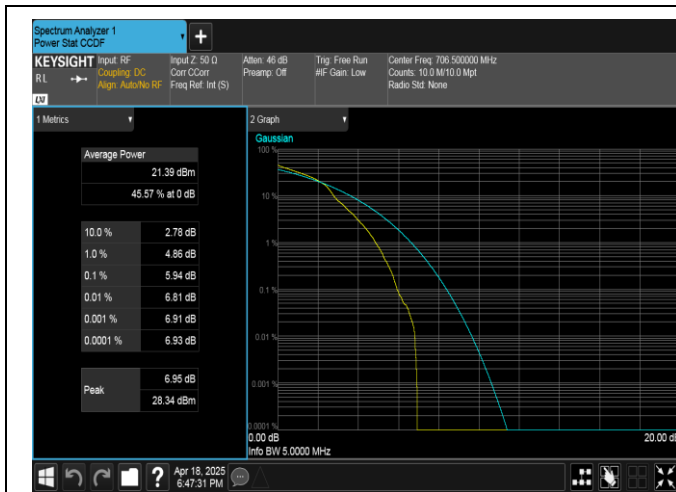
Band17-5MHz-16QAM-23755-1RB#0-PASS
