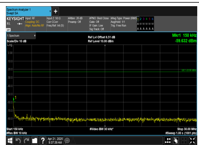
Band13-10MHz-QPSK-23230-50RB#0-0.15~30-PASS
