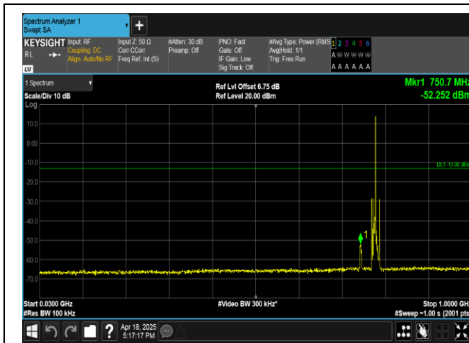
Band13-5MHz-QPSK-23230-1RB#24-30~1000-PASS
