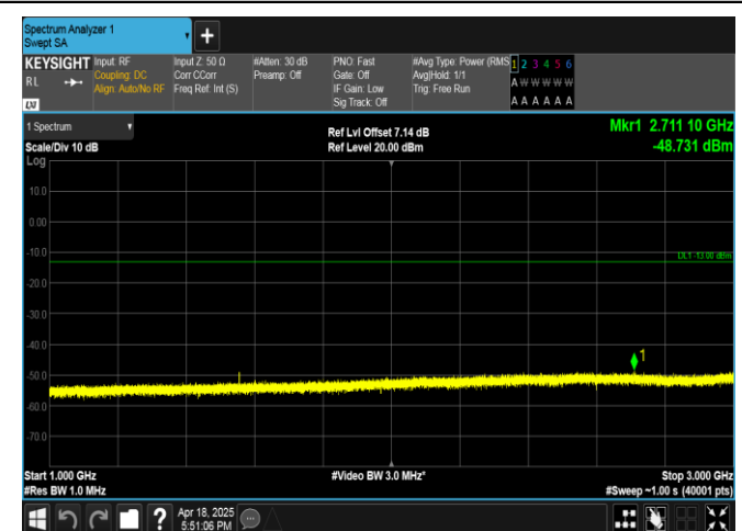
Band13-10MHz-QPSK-23230-1RB#0-1000~3000-PASS
