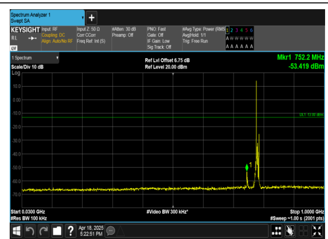
Band13-5MHz-16QAM-23255-1RB#0-30~1000-PASS
