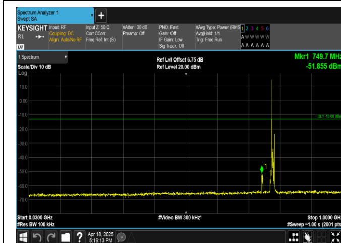
Band13-5MHz-16QAM-23230-1RB#0-30~1000-PASS
