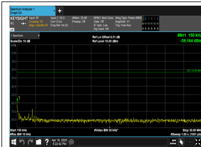
Band13-5MHz-16QAM-23255-1RB#0-0.15~30-PASS
