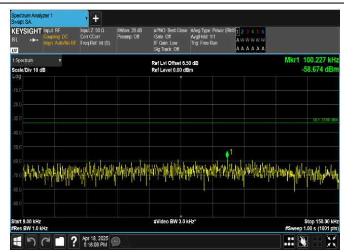
Band13-5MHz-16QAM-23230-1RB#24-0.009~0.15-PASS
