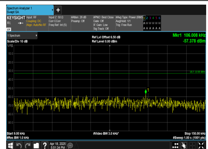
Band13-10MHz-16QAM-23230-1RB#0-0.009~0.15-PASS
