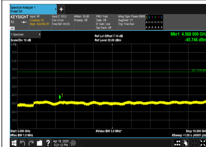
Band13-5MHz-16QAM-23230-25RB#0-3000~10000-PASS
