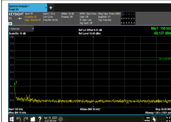
Band13-5MHz-16QAM-23255-25RB#0-0.15~30-PASS
