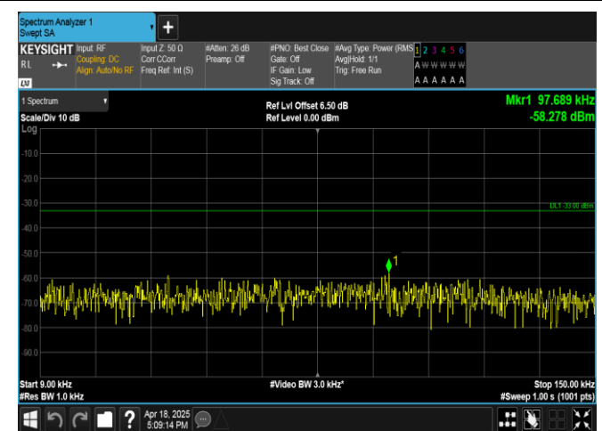
Band13-5MHz-16QAM-23205-1RB#0-0.009~0.15-PASS
