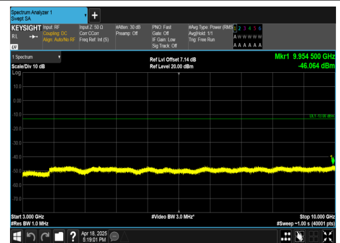
Band13-5MHz-16QAM-23230-1RB#24-3000~10000-PASS
