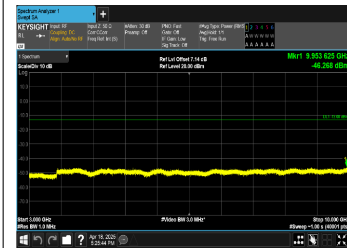
Band13-5MHz-16QAM-23255-1RB#24-3000~10000-PASS
