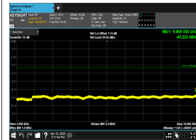
Band13-5MHz-QPSK-23230-1RB#24-3000~10000-PASS
