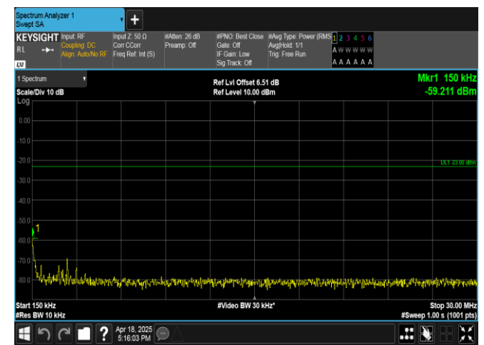
Band13-5MHz-16QAM-23230-1RB#0-0.15~30-PASS
