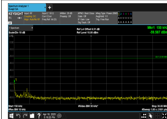
Band13-5MHz-QPSK-23230-25RB#0-0.15~30-PASS
