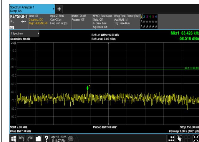
Band13-5MHz-16QAM-23205-1RB#24-0.009~0.15-PASS
