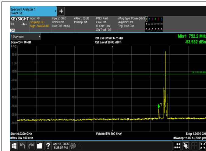
Band13-5MHz-16QAM-23255-1RB#24-30~1000-PASS
