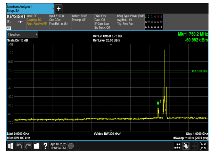
Band13-5MHz-16QAM-23230-1RB#24-30~1000-PASS
