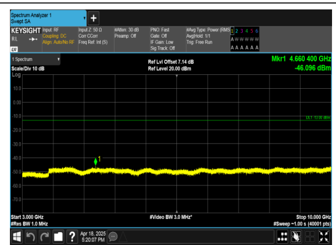
Band13-5MHz-QPSK-23230-25RB#0-3000~10000-PASS
