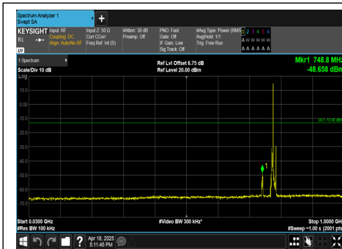
Band13-5MHz-16QAM-23205-1RB#24-30~1000-PASS
