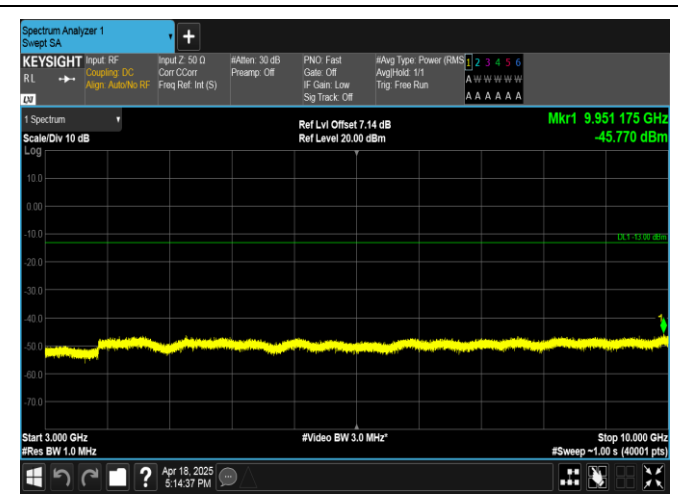
Band13-5MHz-16QAM-23205-25RB#0-3000~10000-PASS
