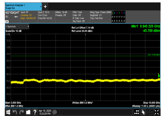
Band13-5MHz-16QAM-23255-1RB#0-3000~10000-PASS
