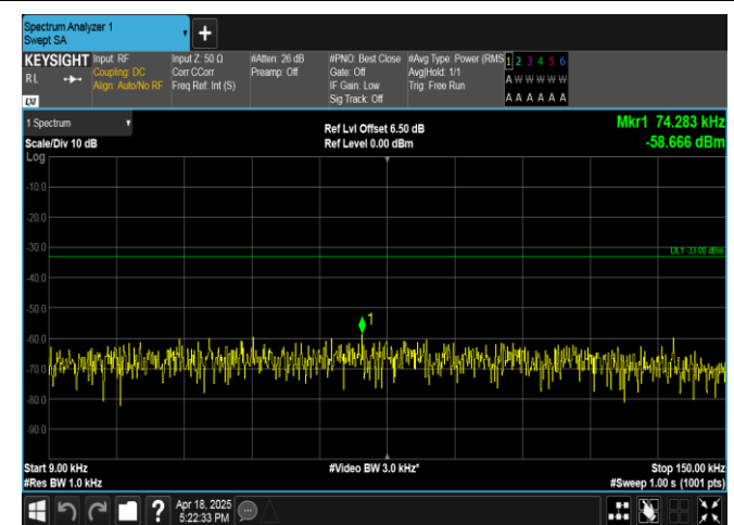
Band13-5MHz-16QAM-23255-1RB#0-0.009~0.15-PASS
