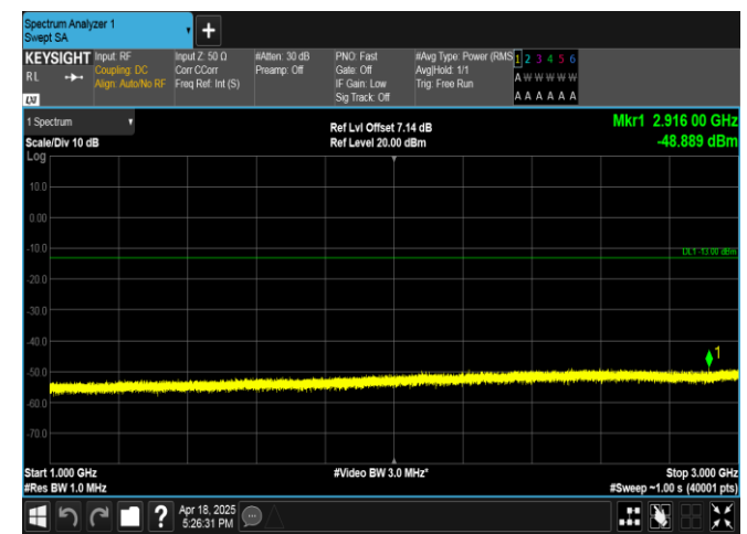
Band13-5MHz-QPSK-23255-25RB#0-1000~3000-PASS
