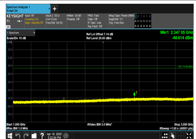
Band13-5MHz-QPSK-23255-1RB#0-1000~3000-PASS
