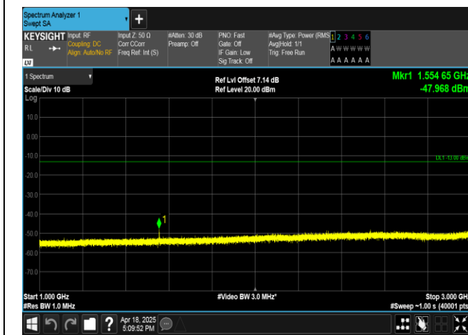
Band13-5MHz-16QAM-23205-1RB#0-1000~3000-PASS
