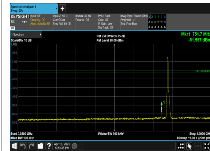
Band13-5MHz-16QAM-23230-25RB#0-30~1000-PASS
