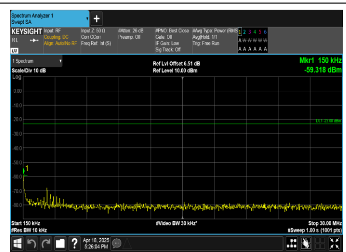
Band13-5MHz-QPSK-23255-25RB#0-0.15~30-PASS
