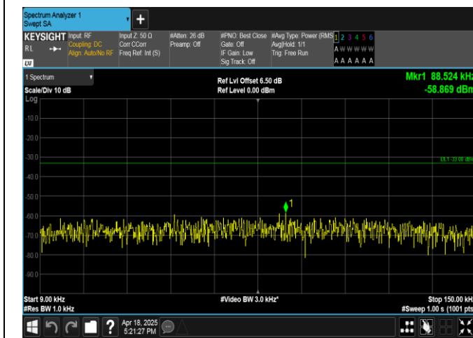
Band13-5MHz-QPSK-23255-1RB#0-0.009~0.15-PASS
