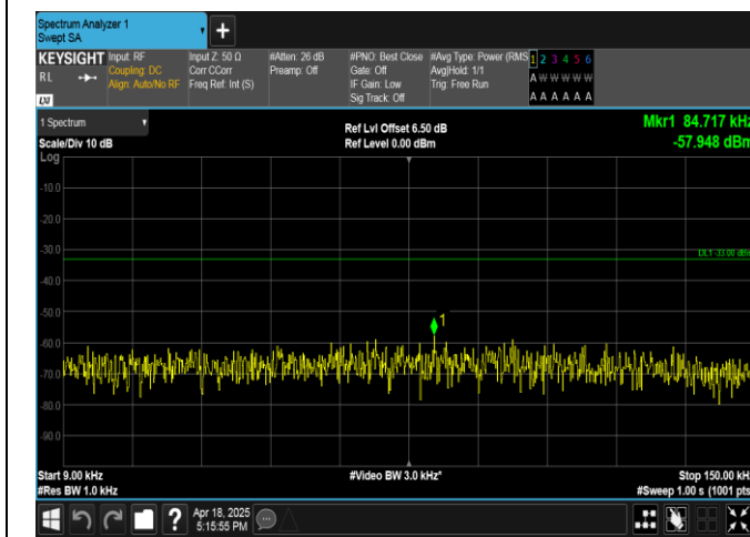
Band13-5MHz-16QAM-23230-1RB#0-0.009~0.15-PASS
