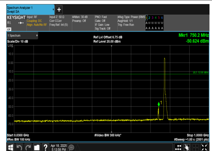
Band13-5MHz-16QAM-23205-25RB#0-30~1000-PASS
