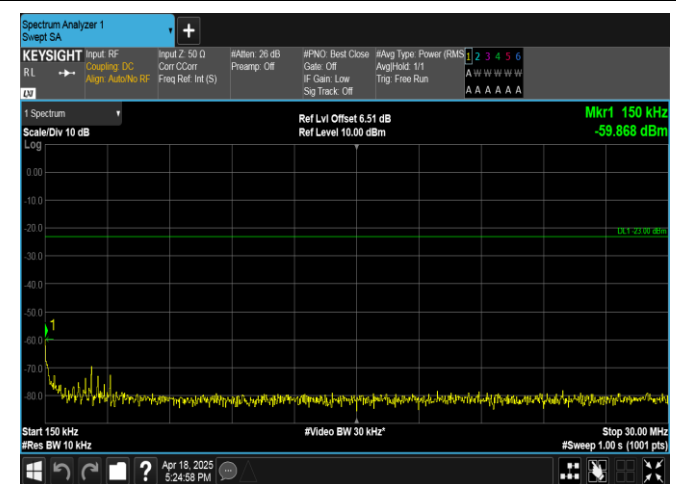
Band13-5MHz-16QAM-23255-1RB#24-0.15~30-PASS
