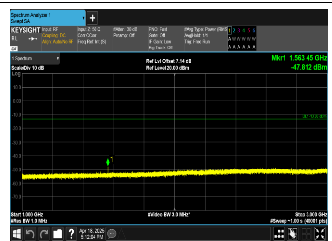
Band13-5MHz-16QAM-23205-1RB#24-1000~3000-PASS
