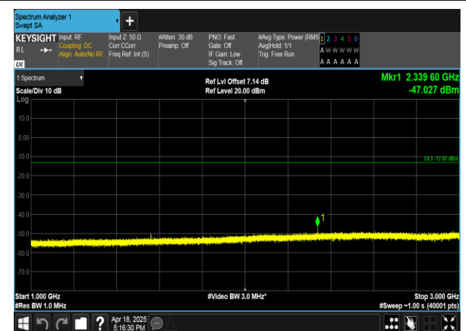
Band13-5MHz-16QAM-23230-1RB#0-1000~3000-PASS
