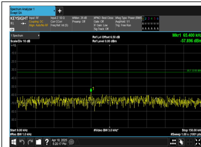
Band13-5MHz-16QAM-23230-25RB#0-0.009~0.15-PASS
