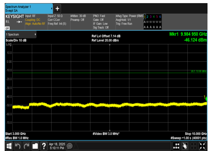
Band13-5MHz-16QAM-23205-1RB#0-3000~10000-PASS
