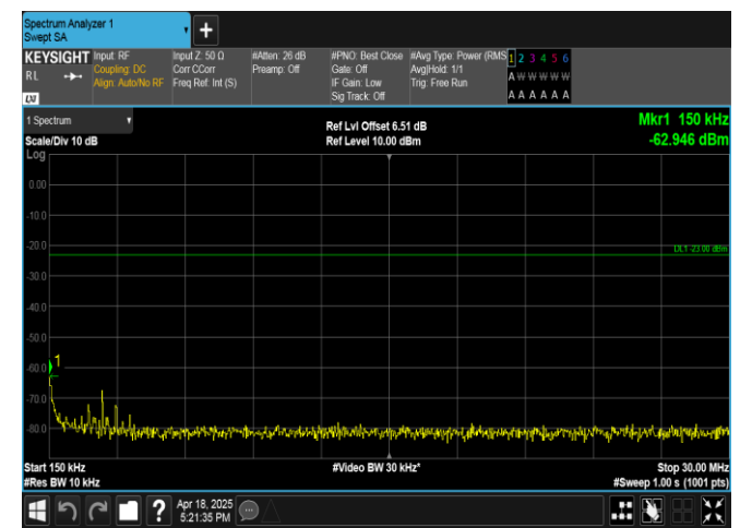
Band13-5MHz-QPSK-23255-1RB#0-0.15~30-PASS
