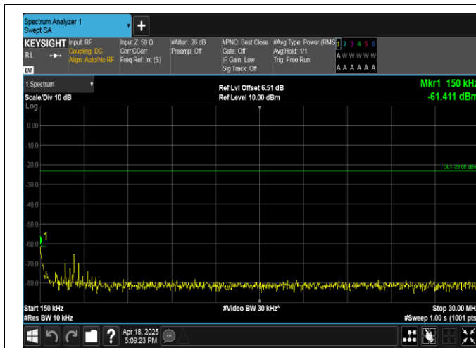
Band13-5MHz-16QAM-23205-1RB#0-0.15~30-PASS
