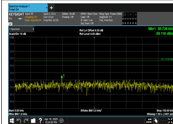
Band13-5MHz-16QAM-23255-1RB#24-0.009~0.15-PASS
