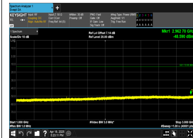
Band13-5MHz-16QAM-23255-1RB#0-1000~3000-PASS
