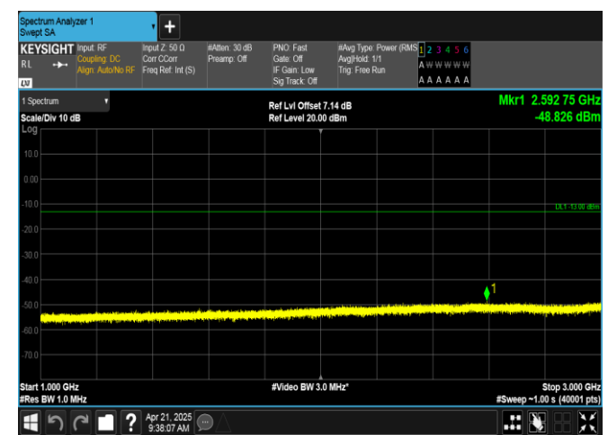
Band13-10MHz-QPSK-23230-50RB#0-1000~3000-PASS
