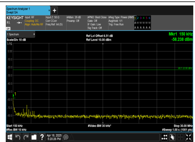
Band13-5MHz-16QAM-23230-25RB#0-0.15~30-PASS
