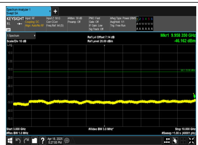
Band13-5MHz-16QAM-23255-25RB#0-3000~10000-PASS
