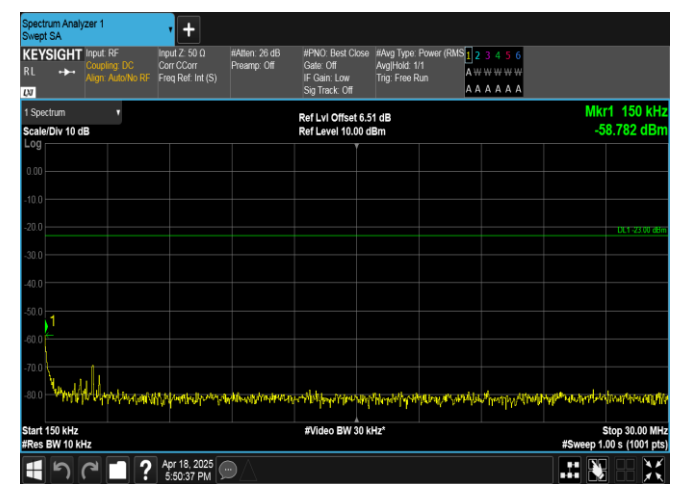
Band13-10MHz-QPSK-23230-1RB#0-0.15~30-PASS
