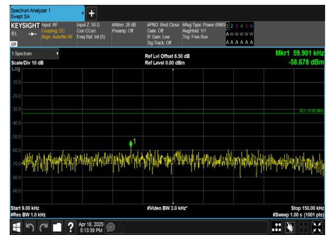
Band13-5MHz-16QAM-23205-25RB#0-0.009~0.15-PASS
