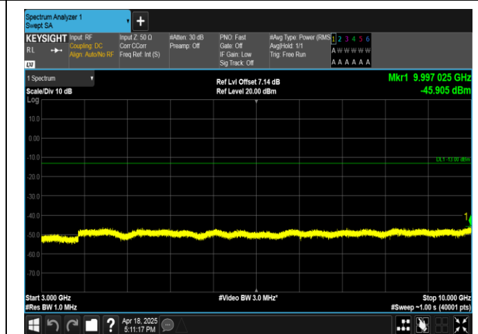
Band13-5MHz-QPSK-23205-1RB#24-3000~10000-PASS
