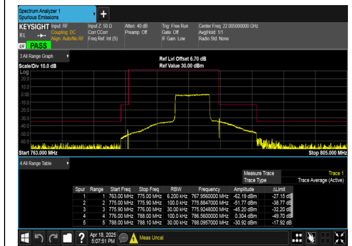
Band13-5MHz-16QAM-23255-25RB#0-PASS
