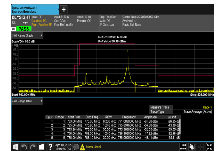
Band13-10MHz-QPSK-23230-1RB#49-PASS
