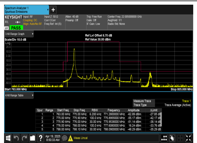
Band13-10MHz-16QAM-23230-1RB#0-PASS
