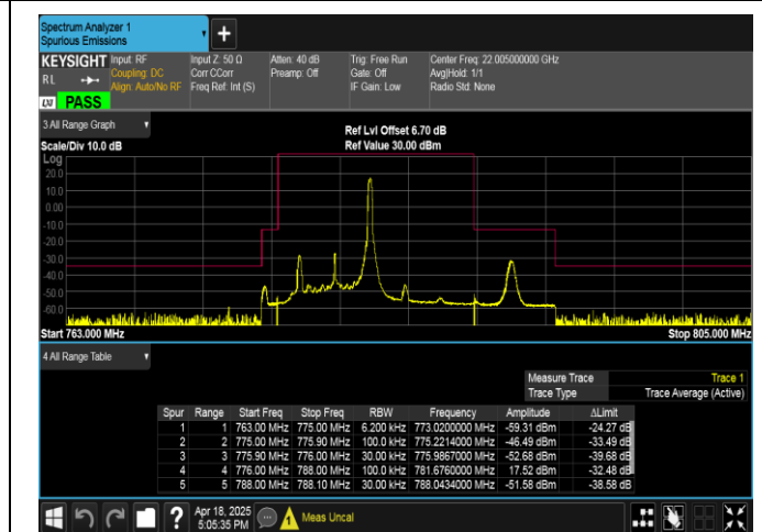
Band13-5MHz-16QAM-23205-1RB#24-PASS
