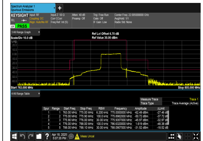
Band13-5MHz-QPSK-23255-25RB#0-PASS
