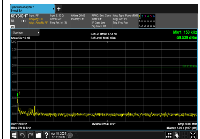
Band13-5MHz-QPSK-23230-1RB#24-0.15~30-PASS
