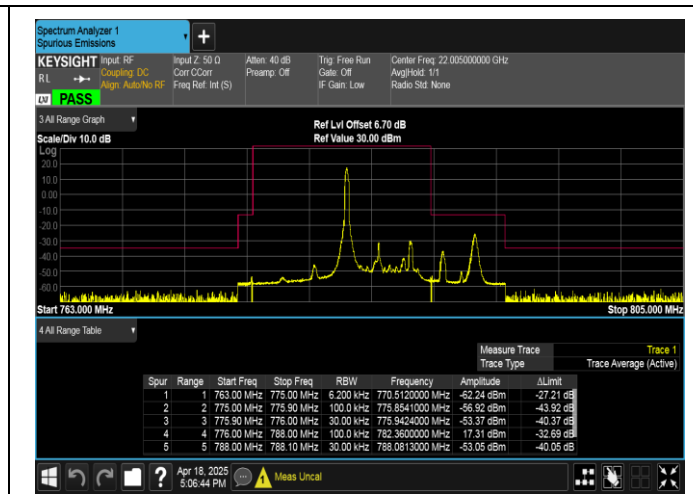
Band13-5MHz-16QAM-23255-1RB#0-PASS
