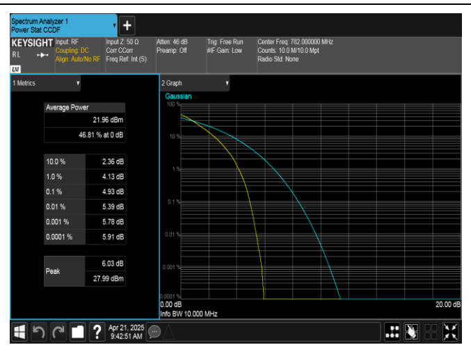
Band13-10MHz-QPSK-23230-50RB#0-PASS
