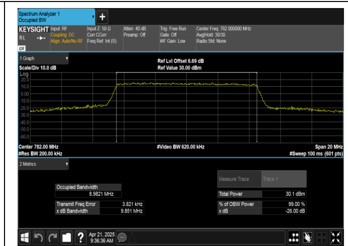
Band13-10MHz-16QAM-23230-50RB#0-PASS
