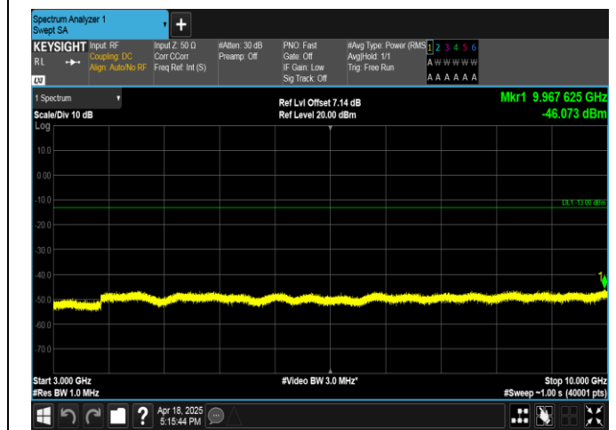
Band13-5MHz-QPSK-23230-1RB#0-3000~10000-PASS
