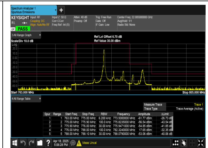
Band13-5MHz-QPSK-23255-1RB#0-PASS
