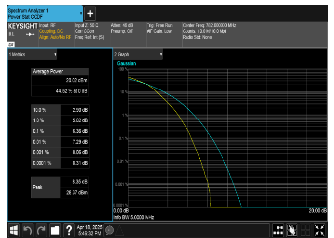
Band13-5MHz-16QAM-23230-25RB#0-PASS
