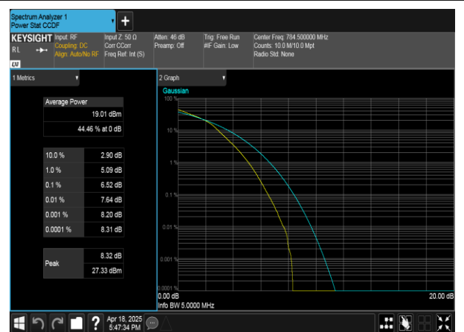
Band13-5MHz-16QAM-23255-25RB#0-PASS
