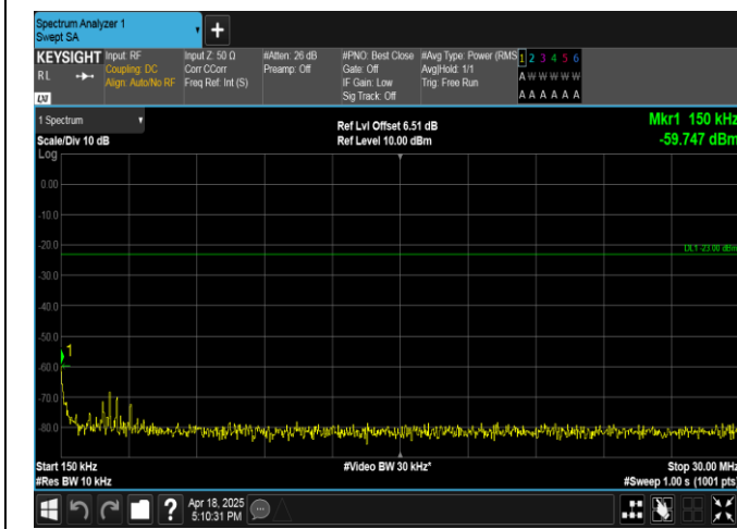
Band13-5MHz-QPSK-23205-1RB#24-0.15~30-PASS
