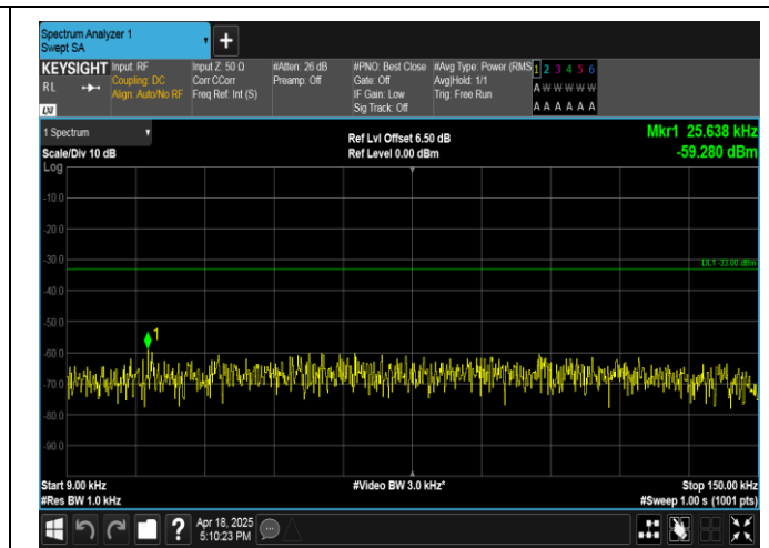
Band13-5MHz-QPSK-23205-1RB#24-0.009~0.15-PASS
