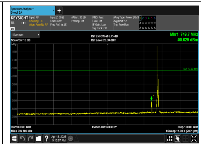
Band13-5MHz-QPSK-23230-1RB#0-30~1000-PASS
