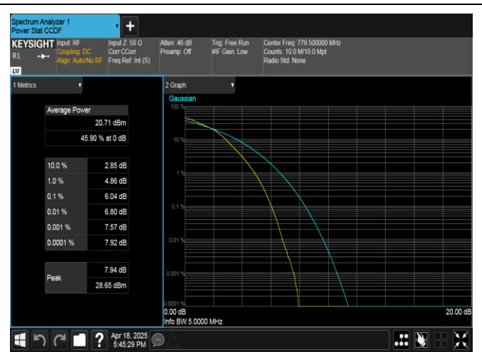
Band13-5MHz-16QAM-23205-25RB#0-PASS
