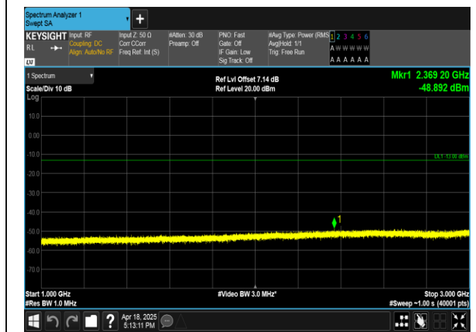
Band13-5MHz-QPSK-23205-25RB#0-1000~3000-PASS
