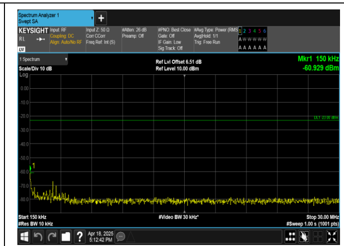
Band13-5MHz-QPSK-23205-25RB#0-0.15~30-PASS
