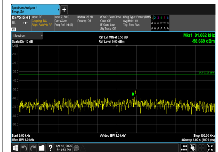
Band13-5MHz-QPSK-23230-1RB#0-0.009~0.15-PASS
