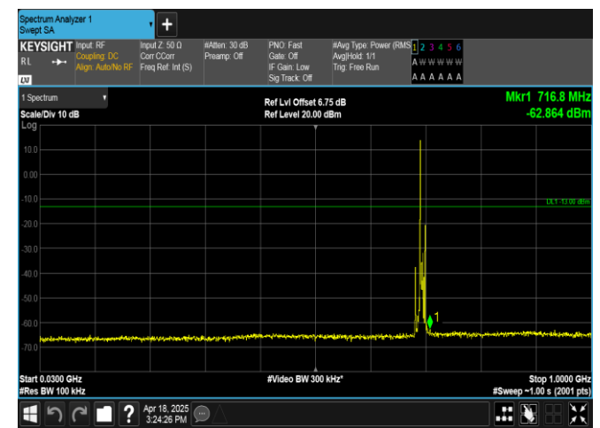
Band12-5MHz-16QAM-23035-1RB#0-30~1000-PASS
