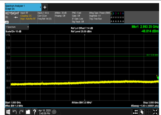
Band12-5MHz-QPSK-23155-25RB#0-1000~3000-PASS
