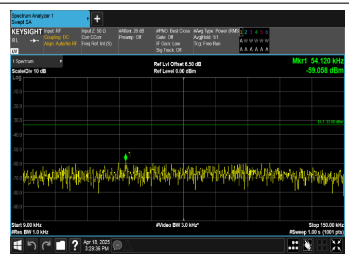
Band12-5MHz-QPSK-23095-1RB#0-0.009~0.15-PASS
