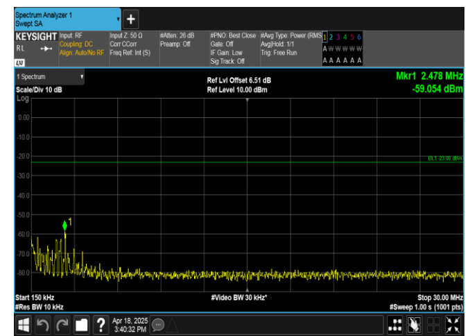
Band12-5MHz-QPSK-23155-25RB#0-0.15~30-PASS
