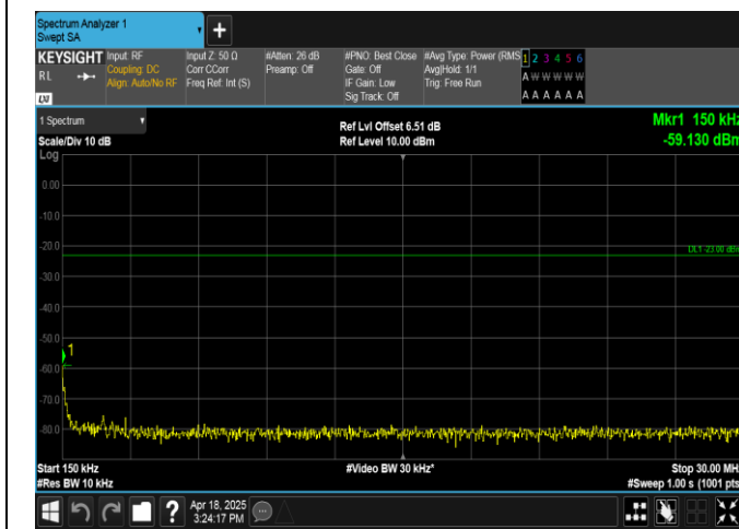
Band12-5MHz-16QAM-23035-1RB#0-0.15~30-PASS
