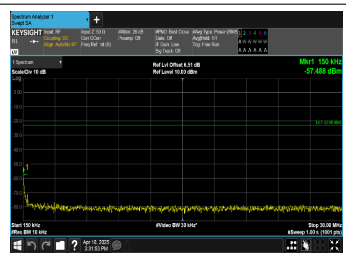
Band12-5MHz-QPSK-23095-1RB#24-0.15~30-PASS
