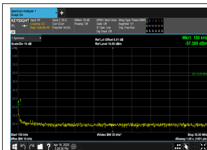
Band12-5MHz-16OAM-23035-25RB#0-0.15~30-PASS
