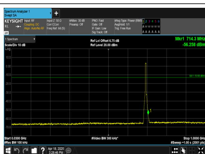
Band12-5MHz-16OAM-23035-25RB#0-30~1000-PASS
