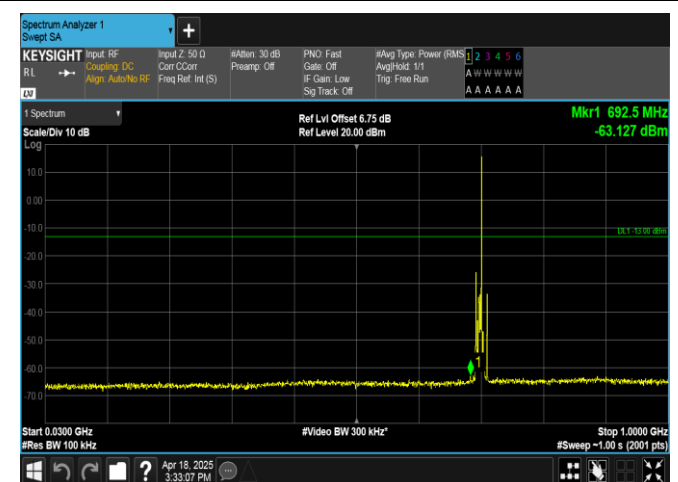
Band12-5MHz-16QAM-23095-1RB#24-30~1000-PASS
