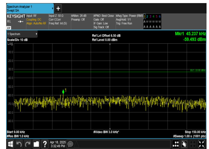
Band12-5MHz-16QAM-23095-1RB#24-0.009~0.15-PASS
