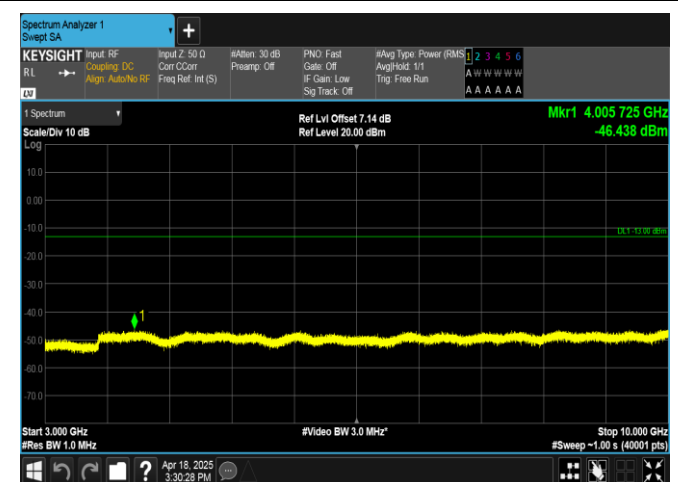
Band12-5MHz-QPSK-23095-1RB#0-3000~10000-PASS
