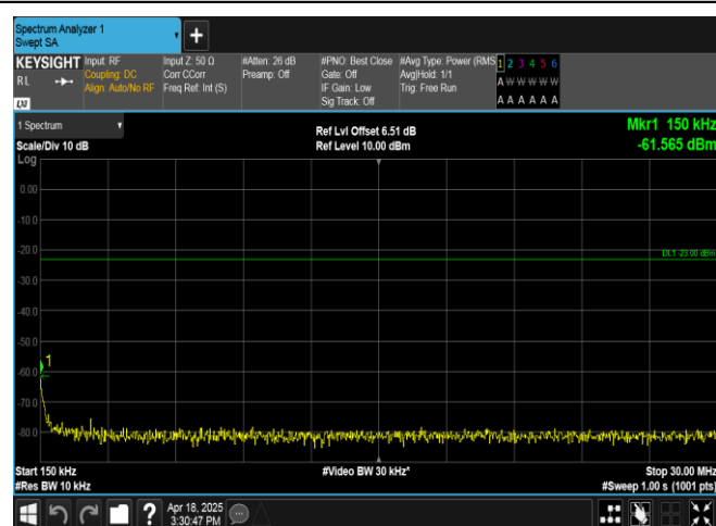
Band12-5MHz-16OAM-23095-1RB#0-0.15~30-PASS
