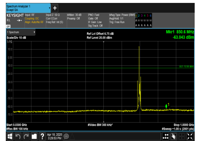
Band12-5MHz-QPSK-23095-1RB#0-30~1000-PASS
