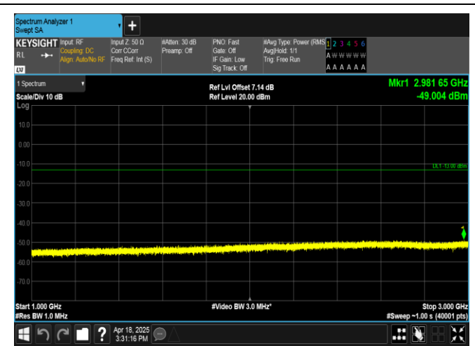
Band12-5MHz-16QAM-23095-1RB#0-1000~3000-PASS
