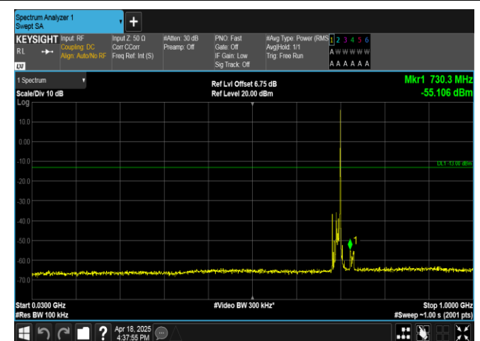
Band12-10MHz-QPSK-23060-1RB#49-30~1000-PASS
