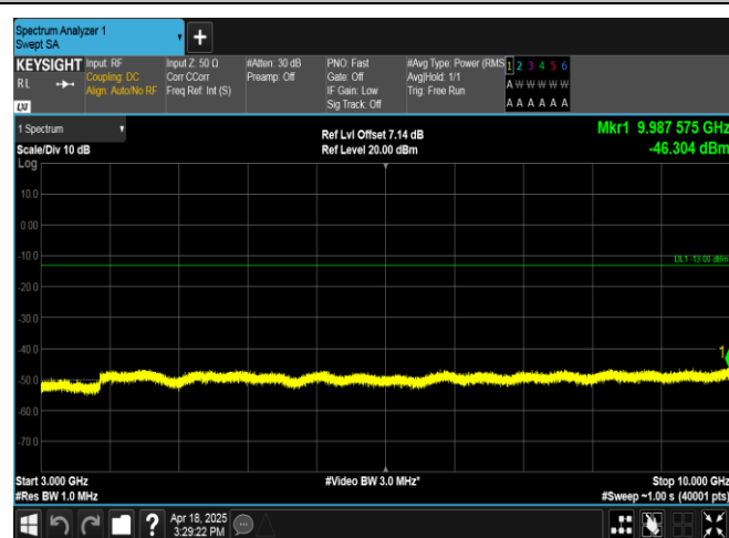
Band12-5MHz-16OAM-23035-25RB#0-3000~10000-PASS
