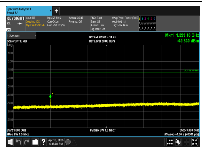
Band12-10MHz-QPSK-23060-1RB#0-1000~3000-PASS
