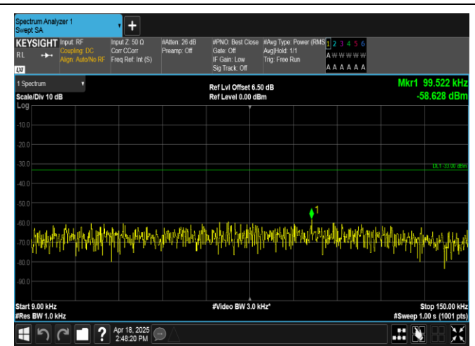
Band12-3MHz-16QAM-23165-1RB#0-0.009~0.15-PASS
