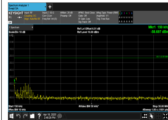
Band12-3MHz-16QAM-23165-1RB#0-0.15~30-PASS
