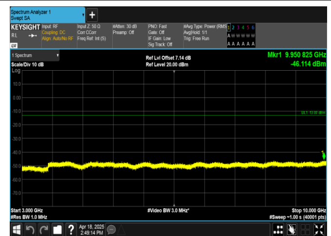
Band12-3MHz-16QAM-23165-1RB#0-3000~10000-PASS
