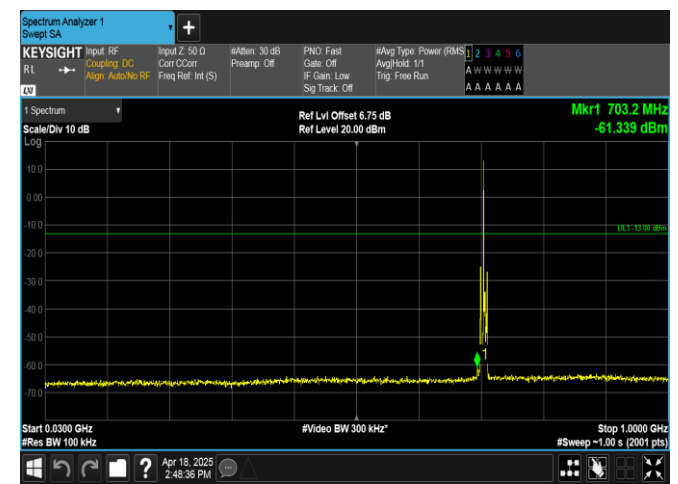
Band12-3MHz-16QAM-23165-1RB#0-30~1000-PASS
