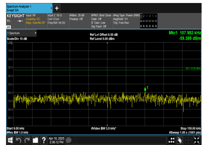
Band12-3MHz-QPSK-23025-1RB#14-0.009~0.15-PASS
