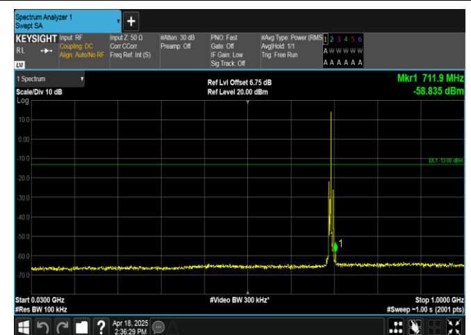
Band12-3MHz-QPSK-23025-1RB#14-30~1000-PASS
