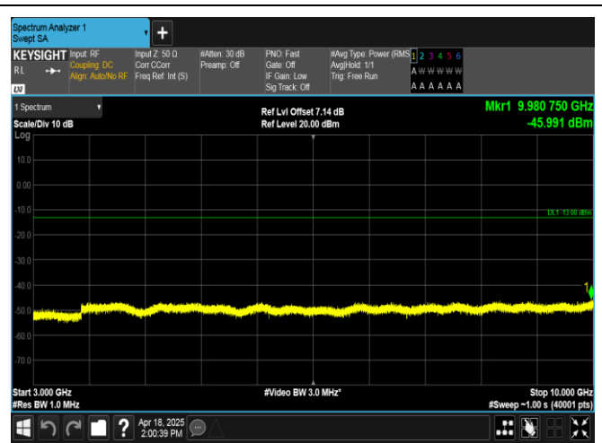
Band12-1.4MHz-QPSK-23173-1RB#5-3000~10000-PASS
