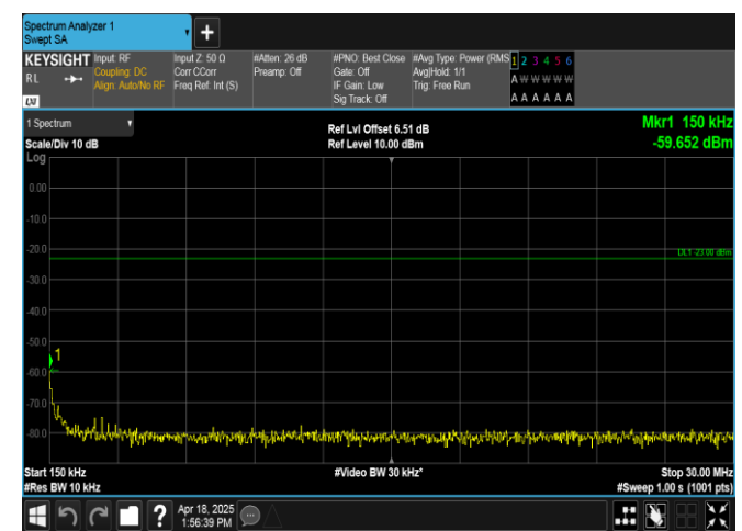
Band12-1.4MHz-16QAM-23095-6RB#0-0.15~30-PASS
