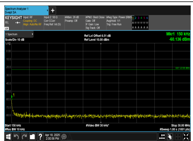
Band12-1.4MHz-16QAM-23173-1RB#5-0.15~30-PASS
