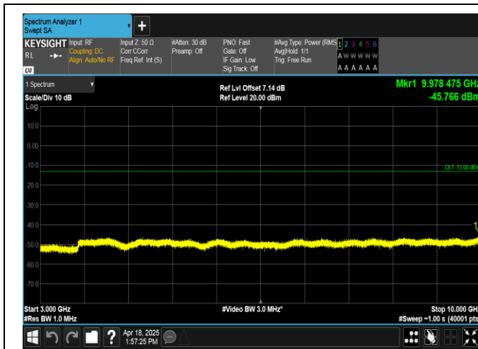
Band12-1.4MHz-16QAM-23095-6RB#0-3000~10000-PASS
