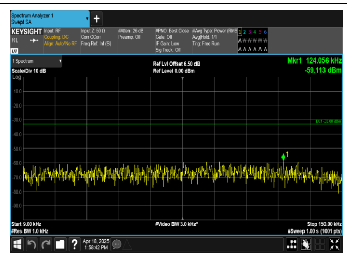
Band12-1.4MHz-16QAM-23173-1RB#0-0.009~0.15-PASS
