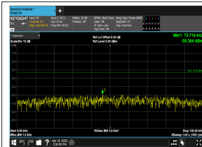
Band12-1.4MHz-16QAM-23173-1RB#5-0.009~0.15-PASS
