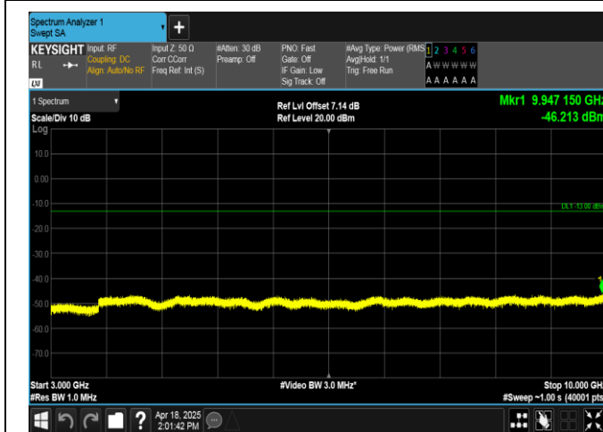
Band12-1.4MHz-16QAM-23173-1RB#5-3000~10000-PASS
