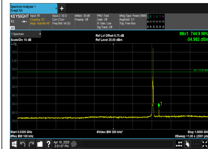
Band12-1.4MHz-16QAM-23173-1RB#5-30~1000-PASS
