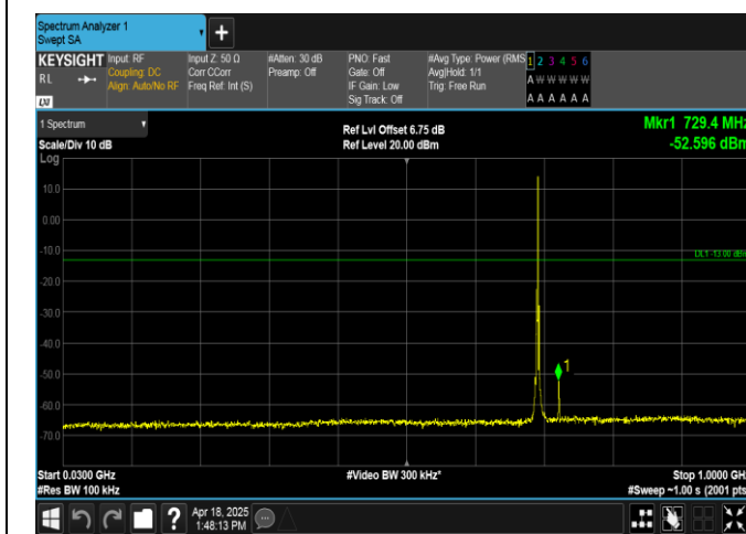
Band12-1.4MHz-16QAM-23017-1RB#5-30~1000-PASS
