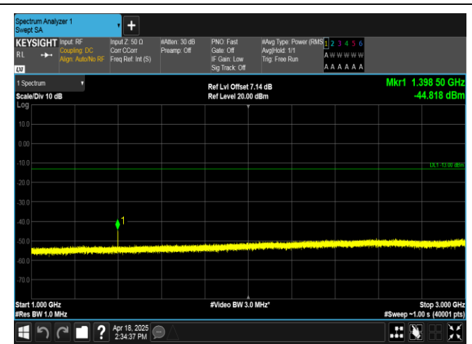
Band12-3MHz-QPSK-23025-1RB#0-1000~3000-PASS
