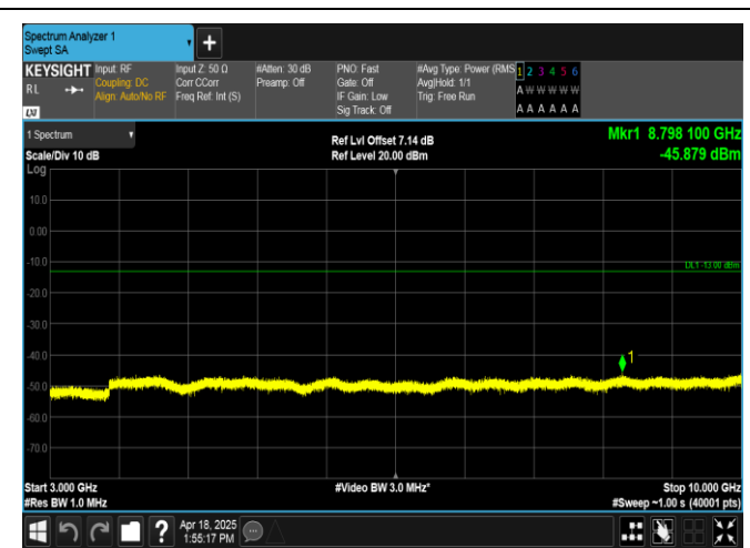
Band12-1.4MHz-16QAM-23095-1RB#5-3000~10000-PASS
