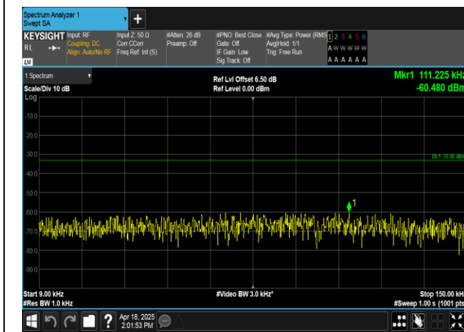
Band12-1.4MHz-QPSK-23173-6RB#0-0.009~0.15-PASS
