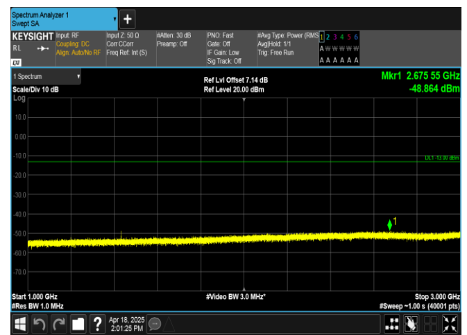
Band12-1.4MHz-16QAM-23173-1RB#5-1000~3000-PASS
