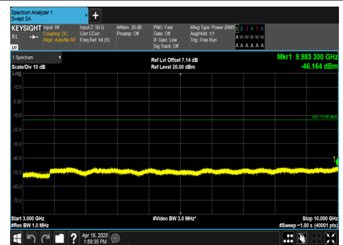
Band12-1.4MHz-16QAM-23173-1RB#0-3000~10000-PASS
