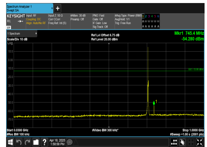
Band12-1.4MHz-16QAM-23173-1RB#0-30~1000-PASS
