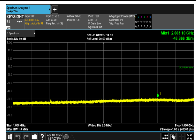
Band12-1.4MHz-16QAM-23095-6RB#0-1000~3000-PASS
