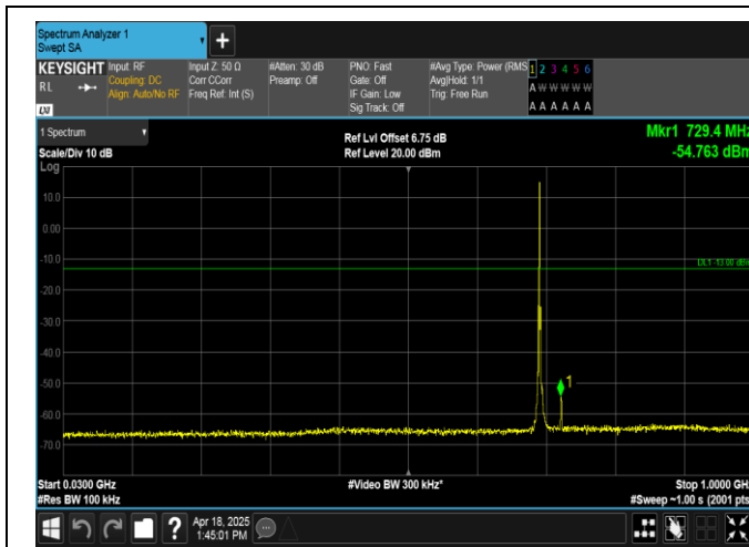
Band12-1.4MHz-QPSK-23017-1RB#0-30~1000-PASS
