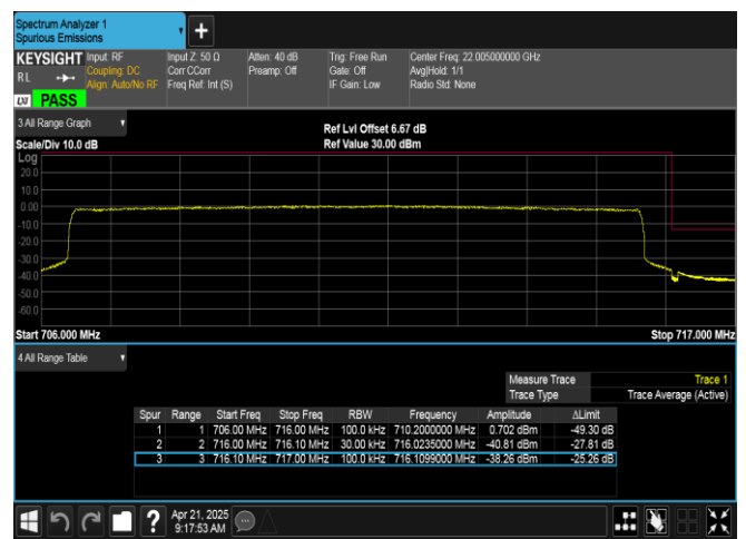
Band12-10MHz-QPSK-23130-50RB#0-PASS
