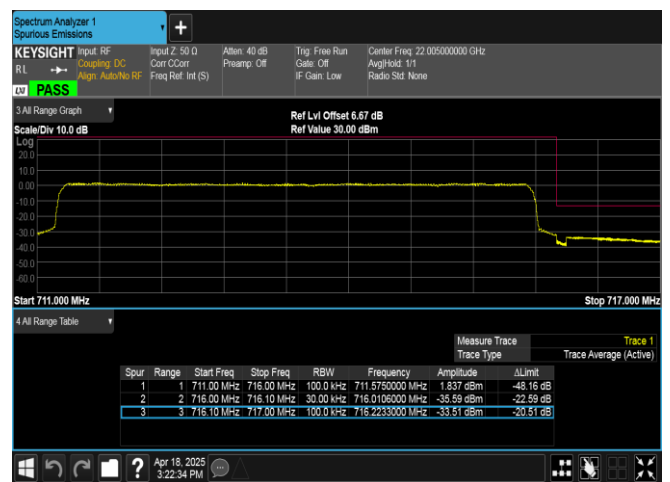
Band12-5MHz-QPSK-23155-25RB#0-PASS
