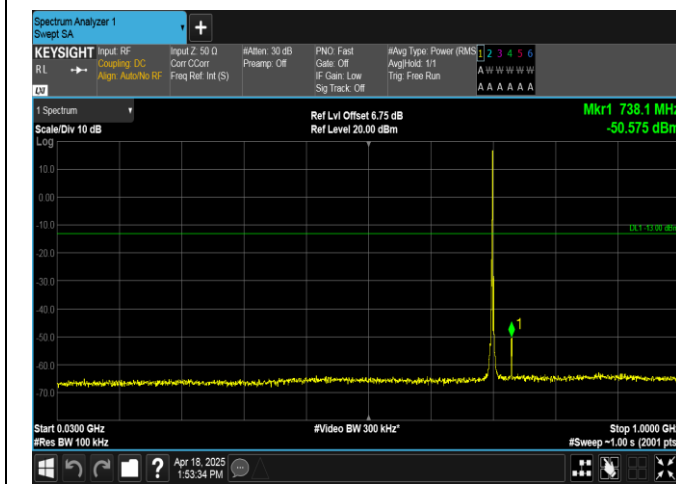
Band12-1.4MHz-QPSK-23095-1RB#5-30~1000-PASS
