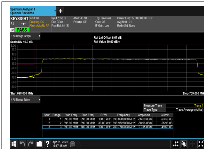
Band12-10MHz-QPSK-23060-50RB#0-PASS
