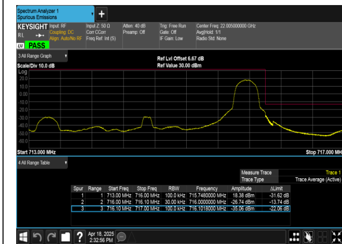
Band12-3MHz-QPSK-23165-1RB#14-PASS
