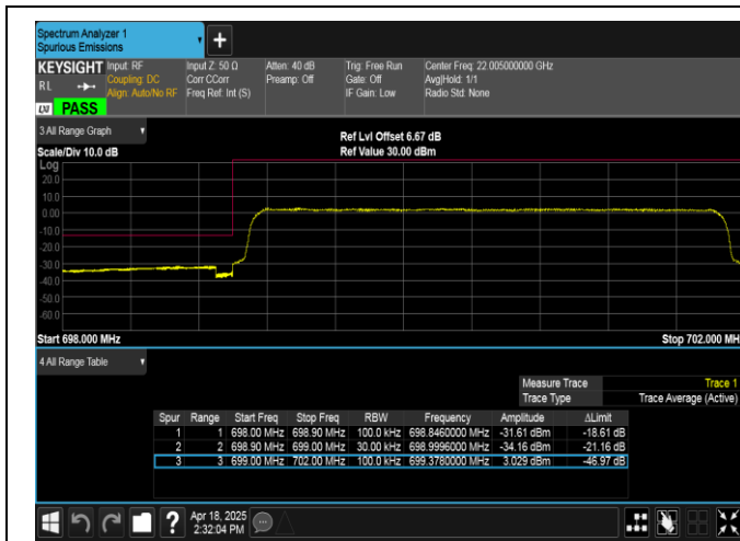
Band12-3MHz-16QAM-23025-15RB#0-PASS
