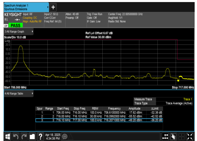
Band12-10MHz-16QAM-23130-1RB#0-PASS
