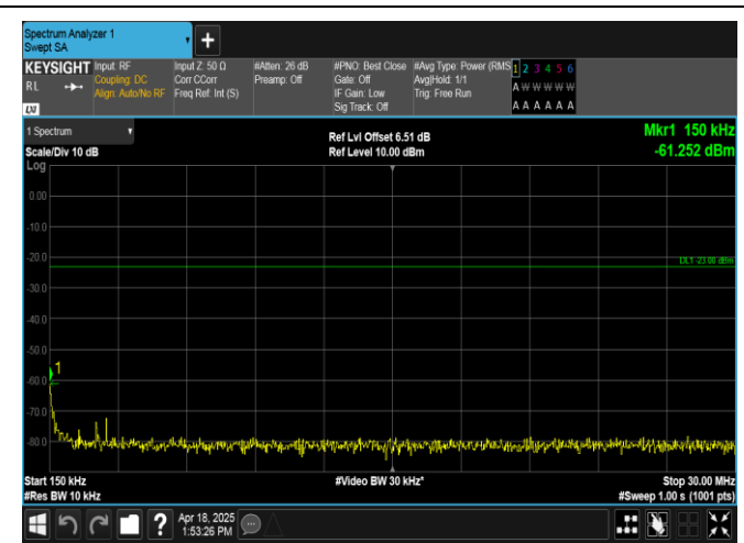
Band12-1.4MHz-QPSK-23095-1RB#5-0.15~30-PASS
