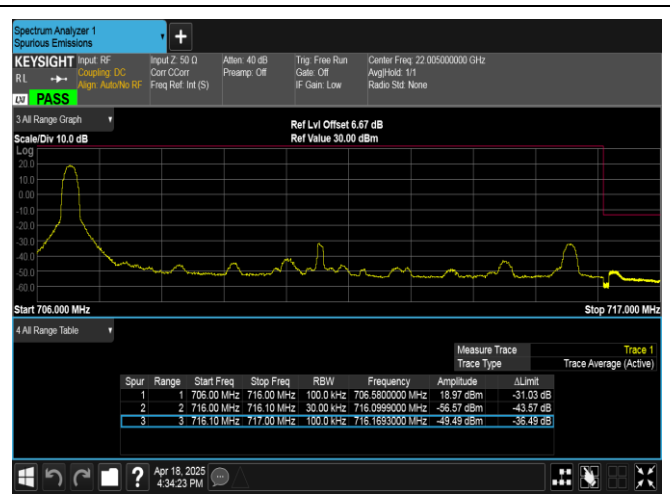
Band12-10MHz-QPSK-23130-1RB#0-PASS
