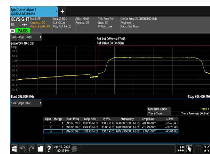
Band12-1.4MHz-16QAM-23017-6RB#0-PASS
