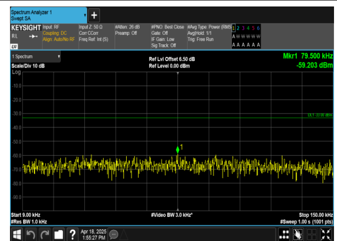
Band12-1.4MHz-QPSK-23095-6RB#0-0.009~0.15-PASS
