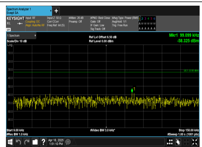
Band12-1.4MHz-QPSK-23095-1RB#0-0.009~0.15-PASS
