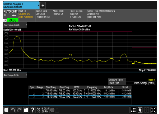
Band12-5MHz-QPSK-23155-1RB#0-PASS
