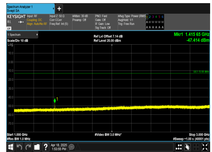
Band12-1.4MHz-QPSK-23095-1RB#5-1000~3000-PASS
