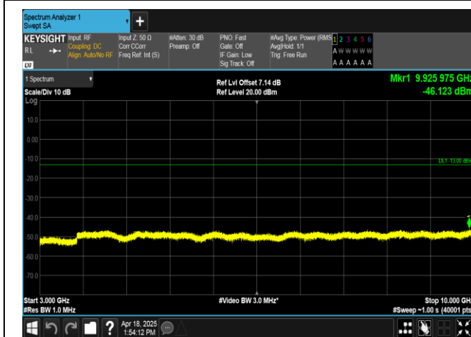
Band12-1.4MHz-QPSK-23095-1RB#5-3000~10000-PASS
