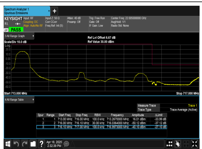
Band12-3MHz-16QAM-23165-1RB#0-PASS
