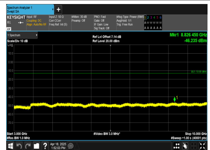
Band12-1.4MHz-QPSK-23095-1RB#0-3000~10000-PASS
