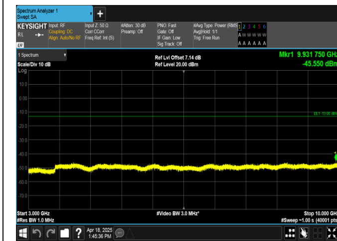
Band12-1.4MHz-QPSK-23017-1RB#0-3000~10000-PASS
