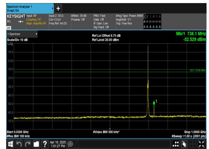
Band12-1.4MHz-QPSK-23095-1RB#0-30~1000-PASS
