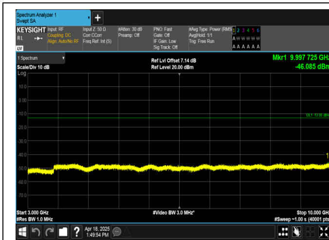
Band12-1.4MHz-QPSK-23017-6RB#0-3000~10000-PASS
