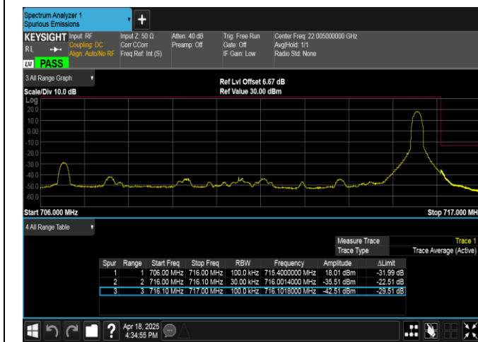
Band12-10MHz-QPSK-23130-1RB#49-PASS
