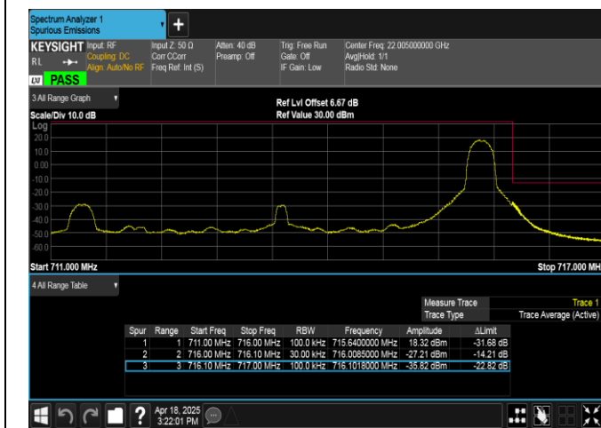
Band12-5MHz-QPSK-23155-1RB#24-PASS
