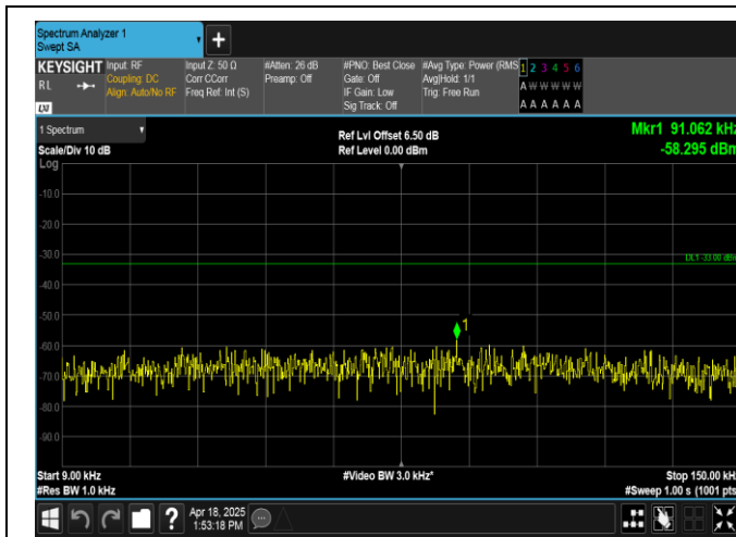
Band12-1.4MHz-QPSK-23095-1RB#5-0.009~0.15-PASS
