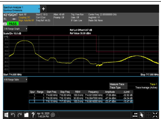
Band12-1.4MHz-16QAM-23173-1RB#0-PASS
