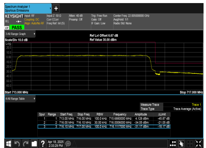
Band12-3MHz-QPSK-23165-15RB#0-PASS
