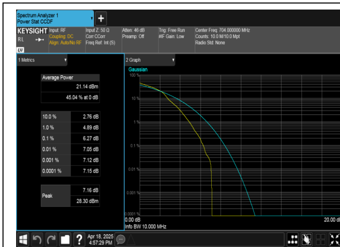
Band12-10MHz-16QAM-23060-1RB#0-PASS
