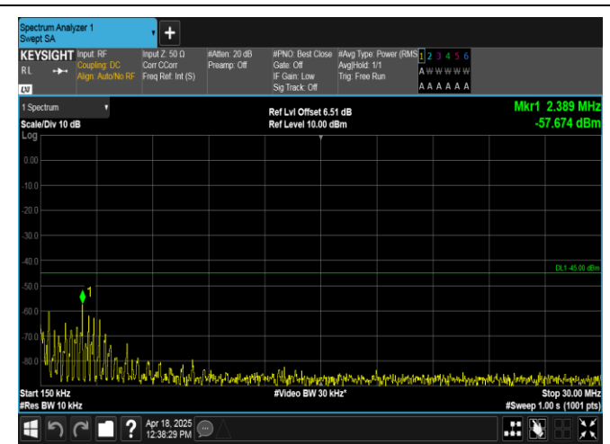
Band7-20MHz-16QAM-20850-1RB#99-0.15~30-PASS
