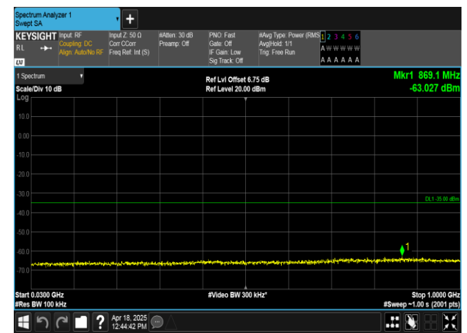
Band7-20MHz-16QAM-21350-1RB#0-30~1000-PASS
