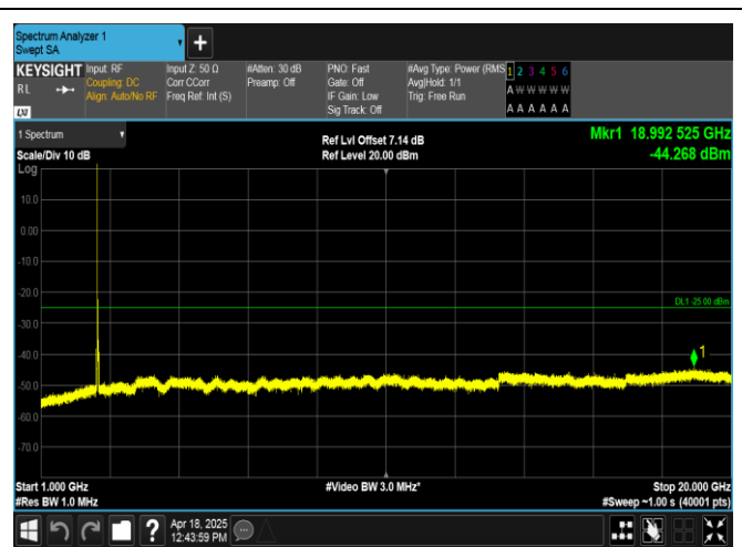
Band7-20MHz-QPSK-21350-1RB#0-1000~20000-PASS
