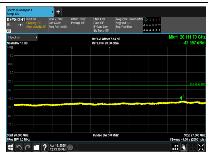
Band7-20MHz-16QAM-21100-1RB#99-20000~27000-PASS
