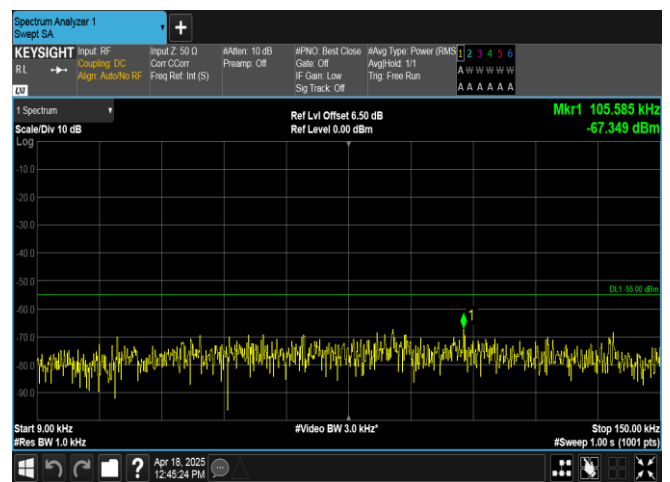
Band7-20MHz-QPSK-21350-1RB#99-0.009~0.15-PASS
