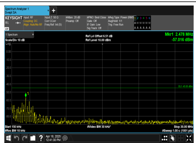
Band7-20MHz-QPSK-21100-1RB#99-0.15~30-PASS
