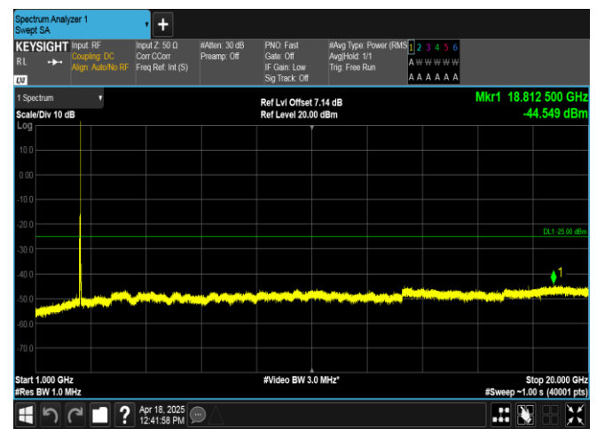
Band7-20MHz-QPSK-21100-1RB#99-1000~20000-PASS
