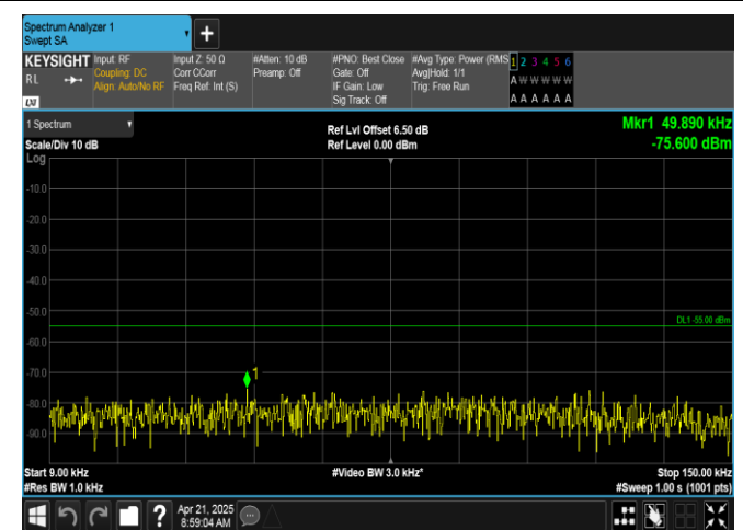
Band7-20MHz-16QAM-20850-100RB#0-0.009~0.15-PASS
