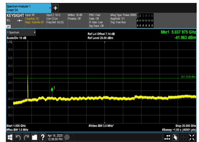
Band7-20MHz-16QAM-20850-1RB#99-1000~20000-PASS
