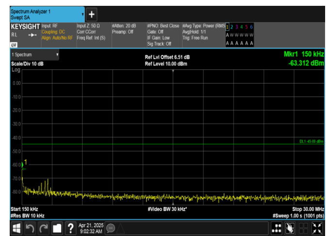
Band7-20MHz-QPSK-21350-100RB#0-0.15~30-PASS
