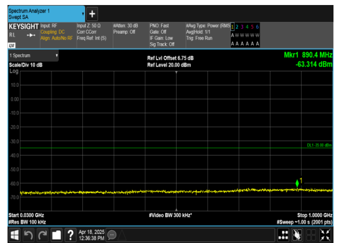
Band7-20MHz-16QAM-20850-1RB#0-30~1000-PASS
