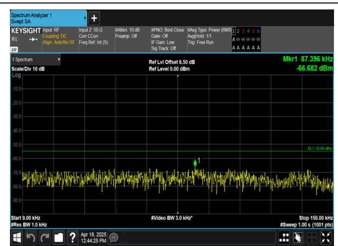
Band7-20MHz-16QAM-21350-1RB#0-0.009~0.15-PASS
