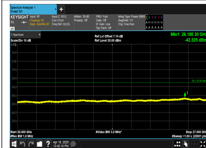
Band7-20MHz-QPSK-21100-1RB#99-20000~27000-PASS
