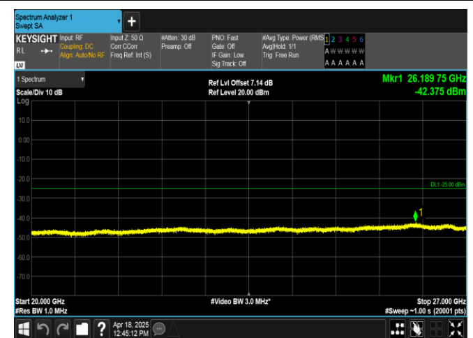
Band7-20MHz-16QAM-21350-1RB#0-20000~27000-PASS
