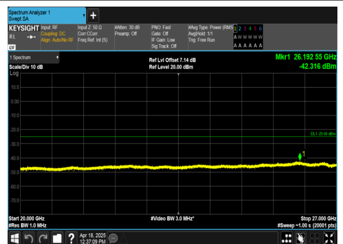
Band7-20MHz-16QAM-20850-1RB#0-20000~27000-PASS
