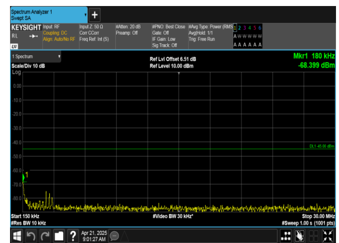
Band7-20MHz-16QAM-21100-100RB#0-0.15~30-PASS
