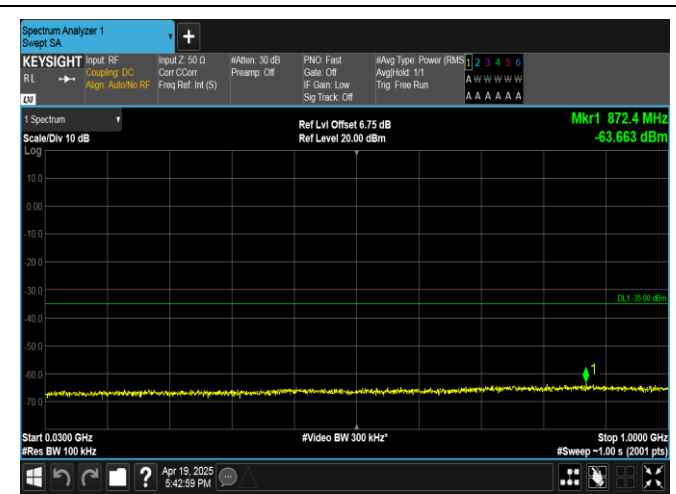
Band7-15MHz-16QAM-21375-75RB#0-30~1000-PASS
