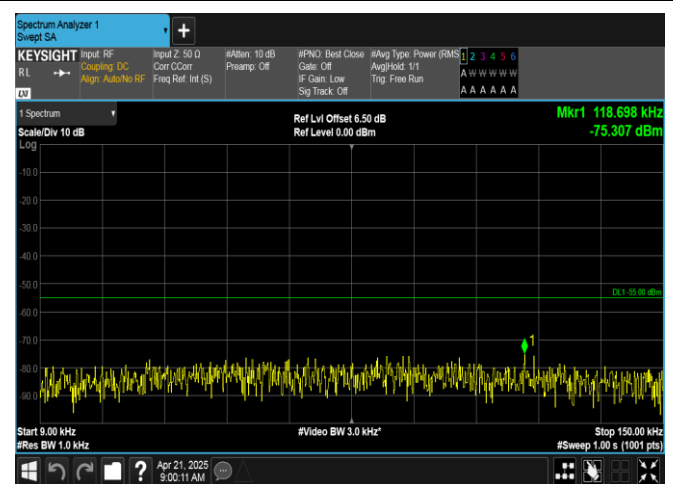
Band7-20MHz-QPSK-21100-100RB#0-0.009~0.15-PASS
