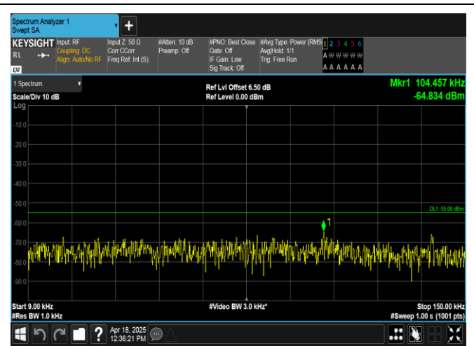
Band7-20MHz-16QAM-20850-1RB#0-0.009~0.15-PASS
