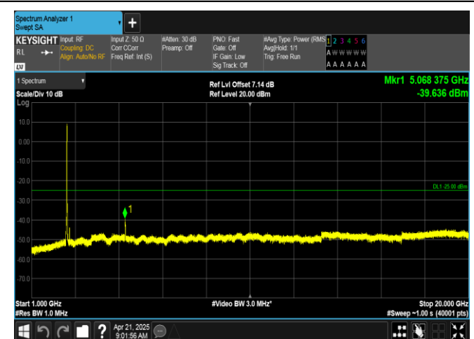
Band7-20MHz-16QAM-21100-100RB#0-1000~20000-PASS
