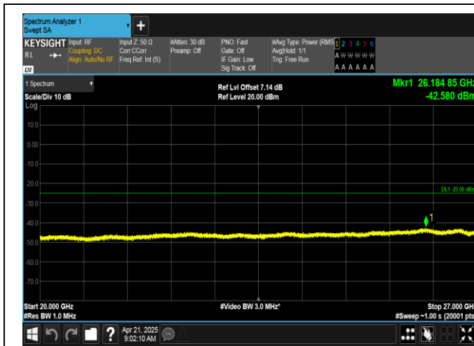
Band7-20MHz-16QAM-21100-100RB#0-20000~27000-PASS
