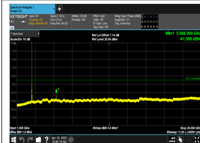
Band7-5MHz-QPSK-21100-1RB#0-1000~20000-PASS
