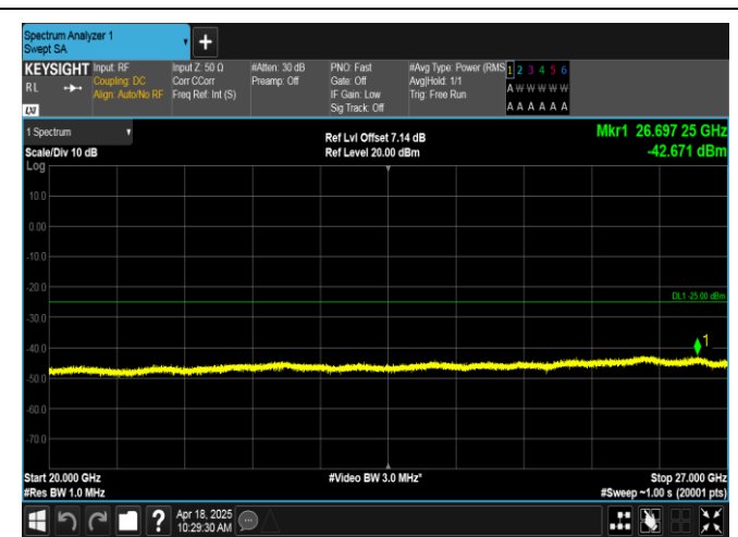
Band7-5MHz-16QAM-21100-1RB#24-20000~27000-PASS
