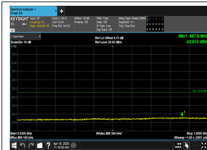
Band7-10MHz-QPSK-20800-1RB#0-30~1000-PASS
