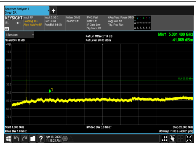
Band7-10MHz-QPSK-20800-1RB#0-1000~20000-PASS
