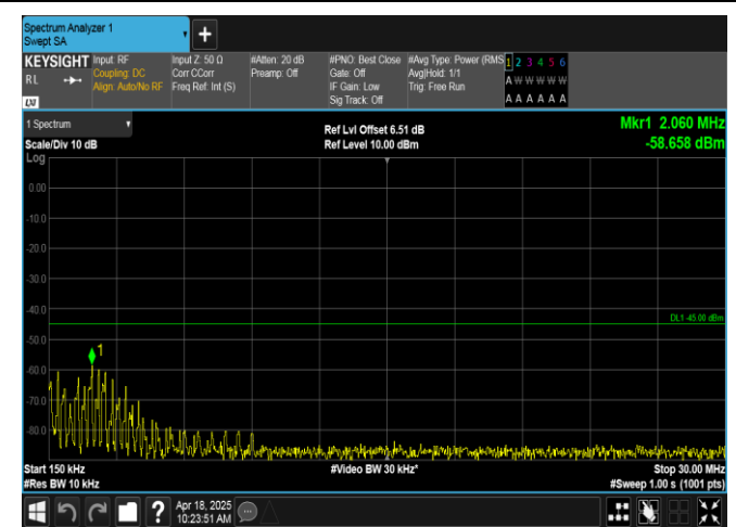
Band7-5MHz-QPSK-20775-25RB#0-0.15~30-PASS
