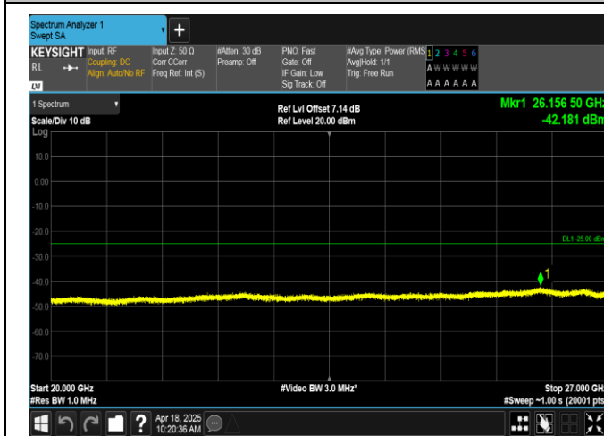
Band7-5MHz-QPSK-20775-1RB#0-20000~27000-PASS
