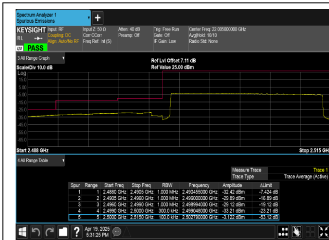
Band7-15MHz-QPSK-20825-75RB#0-PASS
