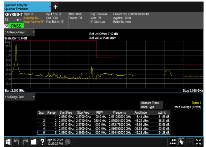
Band7-20MHz-QPSK-21350-1RB#0-PASS
