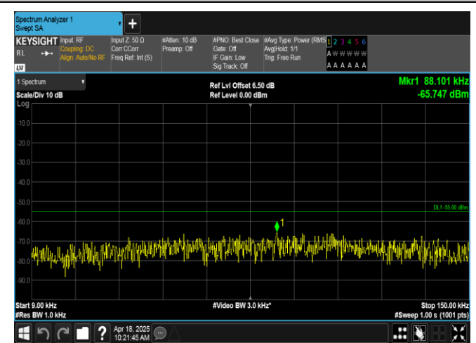
Band7-5MHz-QPSK-20775-1RB#24-0.009~0.15-PASS
