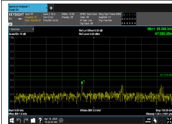
Band7-5MHz-QPSK-20775-25RB#0-0.009~0.15-PASS
