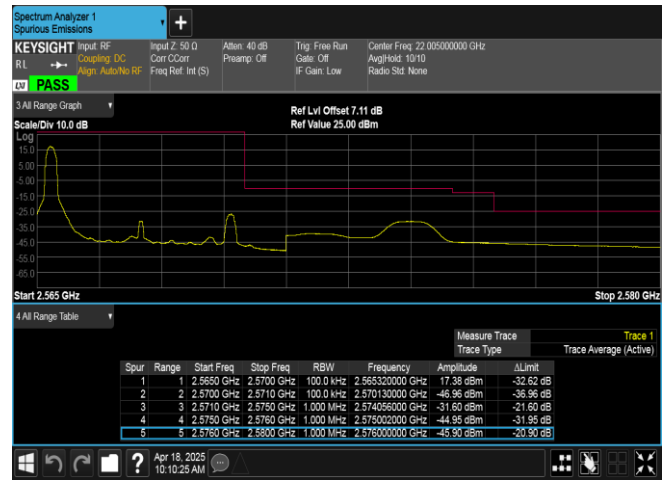
Band7-5MHz-QPSK-21425-1RB#0-PASS
