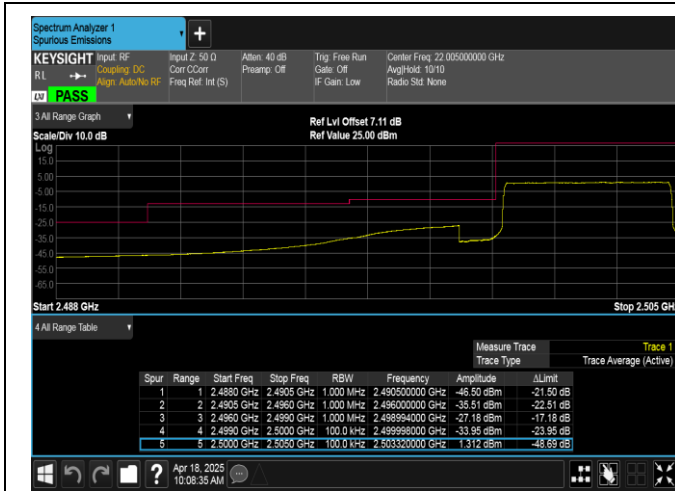
Band7-5MHz-16QAM-20775-25RB#0-PASS
