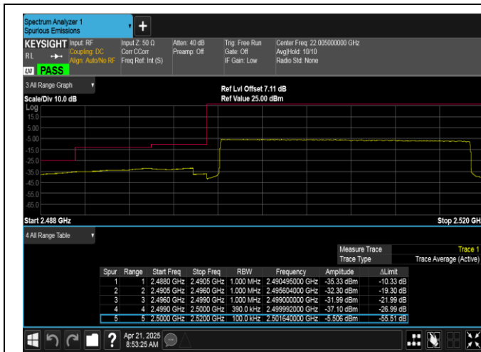
Band7-20MHz-16QAM-20850-100RB#0-PASS
