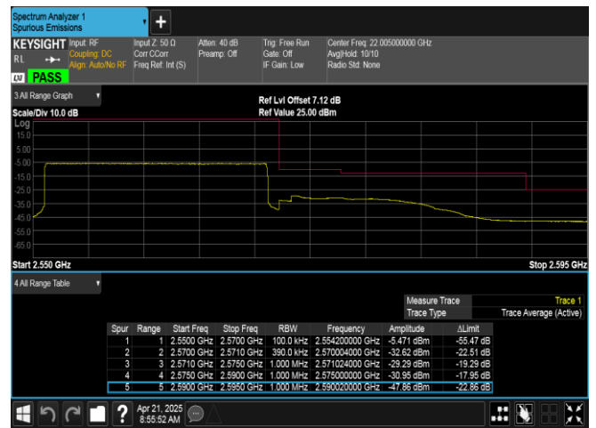
Band7-20MHz-QPSK-21350-100RB#0-PASS
