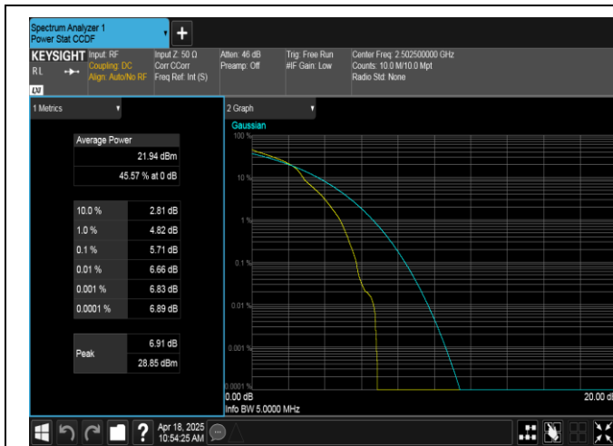
Band7-5MHz-16QAM-20775-1RB#0-PASS
