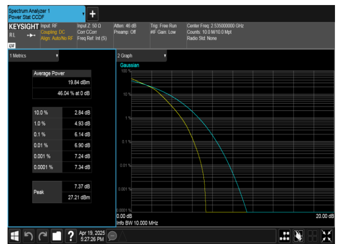
Band7-10MHz-16QAM-21100-50RB#0-PASS
