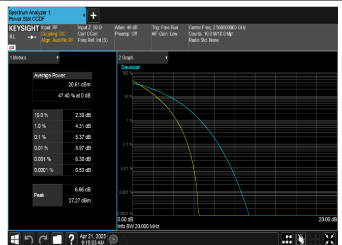
Band7-20MHz-QPSK-21350-100RB#0-PASS
