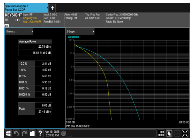
Band7-15MHz-QPSK-21100-75RB#0-PASS
