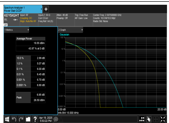
Band7-15MHz-16QAM-20825-75RB#0-PASS
