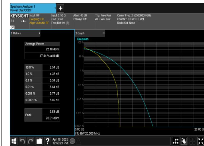
Band7-20MHz-QPSK-21100-1RB#0-PASS
