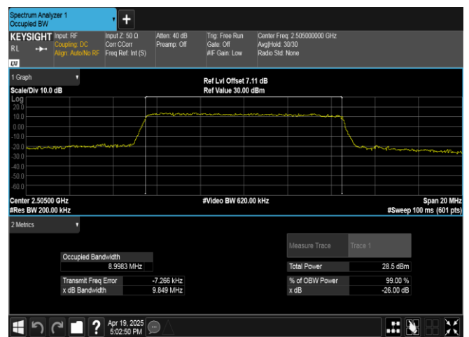
Band7-10MHz-16QAM-20800-50RB#0-PASS
