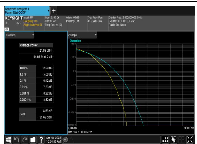
Band7-5MHz-16QAM-20775-25RB#0-PASS
