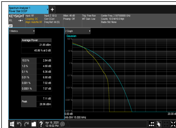
Band7-15MHz-16QAM-20825-1RB#0-PASS
