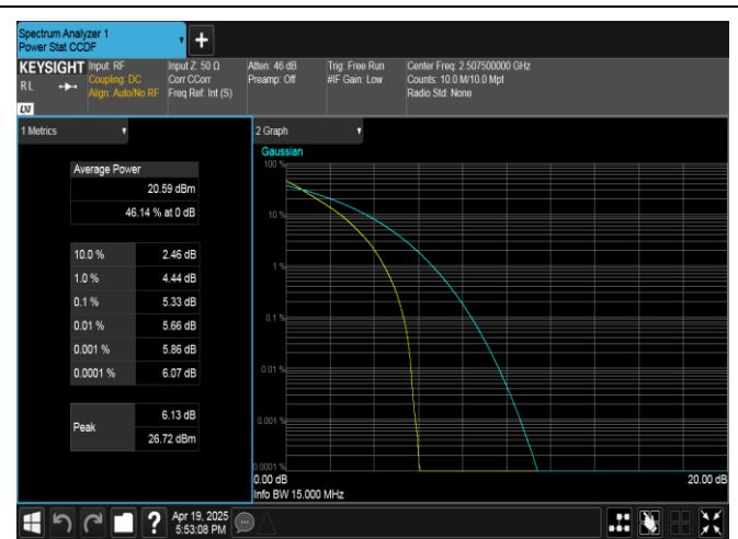
Band7-15MHz-QPSK-20825-75RB#0-PASS
