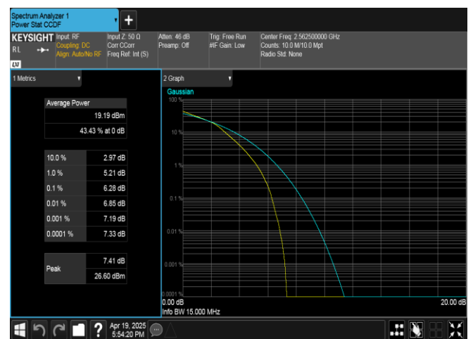
Band7-15MHz-16QAM-21375-75RB#0-PASS
