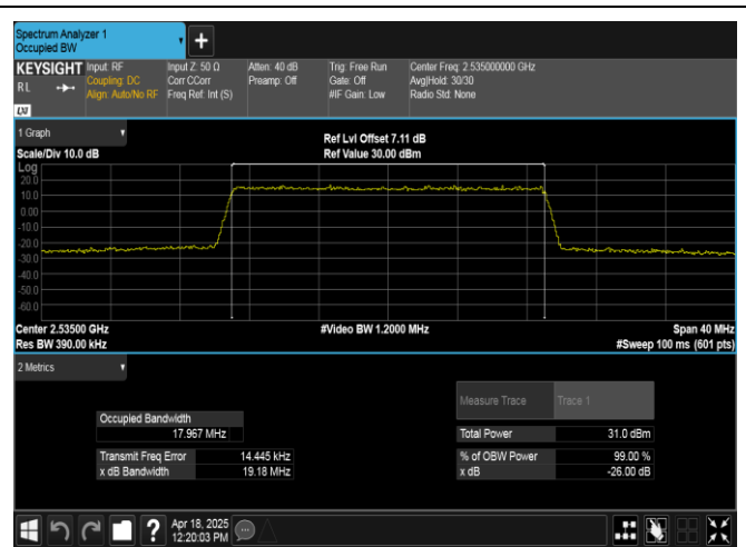
Band7-20MHz-QPSK-21100-100RB#0-PASS
