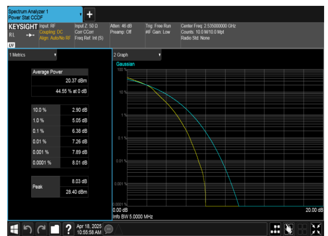
Band7-5MHz-16QAM-21100-25RB#0-PASS
