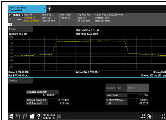
Band7-20MHz-QPSK-20850-100RB#0-PASS
