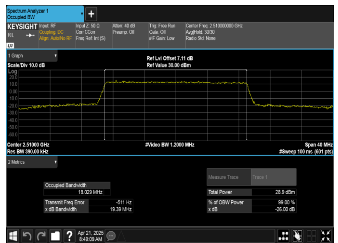
Band7-20MHz-16QAM-20850-100RB#0-PASS
