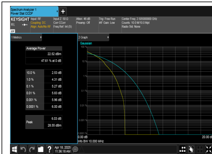
Band7-10MHz-QPSK-20800-1RB#0-PASS
