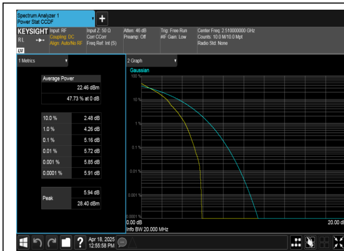
Band7-20MHz-QPSK-20850-1RB#0-PASS
