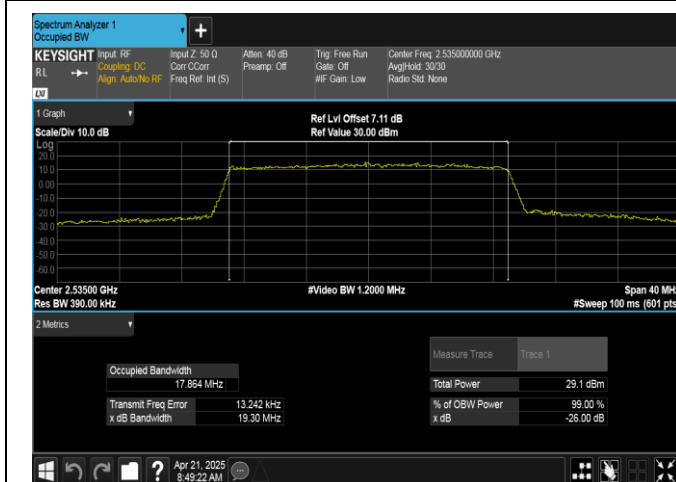
Band7-20MHz-16QAM-21100-100RB#0-PASS
