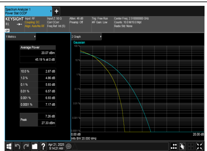
Band7-20MHz-16QAM-20850-100RB#0-PASS
