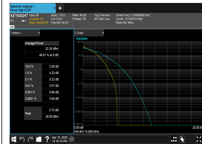
Band7-15MHz-QPSK-21100-1RB#0-PASS
