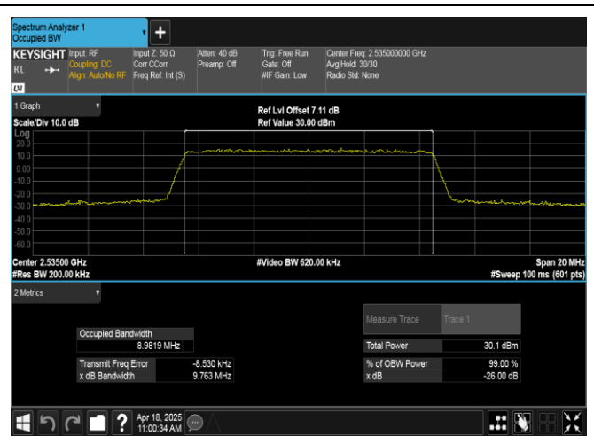
Band7-10MHz-QPSK-21100-50RB#0-PASS
