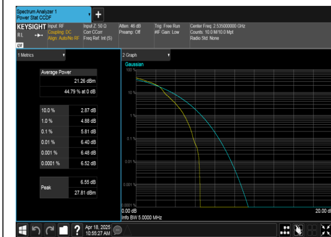
Band7-5MHz-16QAM-21100-1RB#0-PASS
