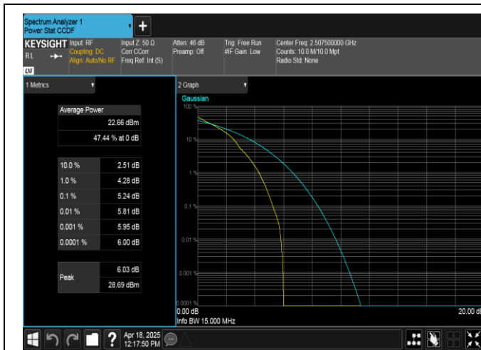
Band7-15MHz-QPSK-20825-1RB#0-PASS
