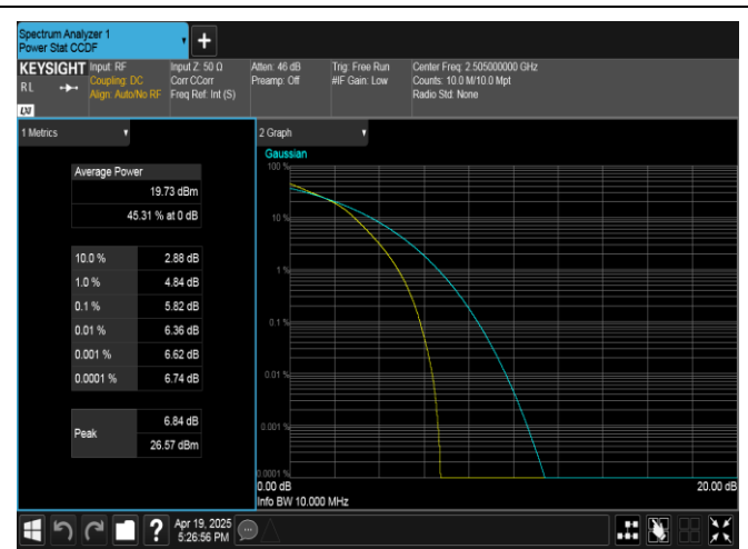
Band7-10MHz-16QAM-20800-50RB#0-PASS
