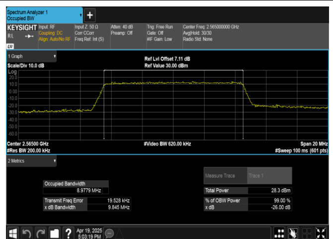
Band7-10MHz-16QAM-21400-50RB#0-PASS
