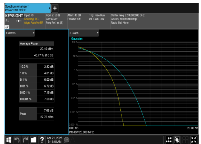
Band7-20MHz-16QAM-21100-100RB#0-PASS
