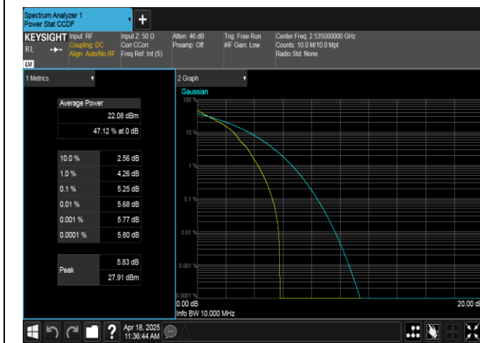
Band7-10MHz-QPSK-21100-1RB#0-PASS
