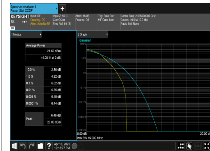
Band7-15MHz-16QAM-21100-1RB#0-PASS
