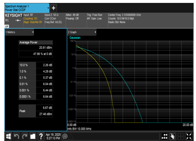
Band7-10MHz-QPSK-21100-50RB#0-PASS
