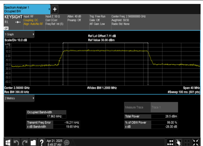
Band7-20MHz-16QAM-21350-100RB#0-PASS
