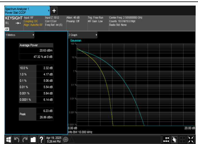
Band7-10MHz-QPSK-20800-50RB#0-PASS
