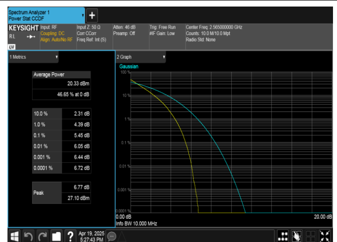
Band7-10MHz-QPSK-21400-50RB#0-PASS
