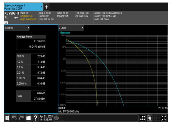
Band7-20MHz-QPSK-21100-100RB#0-PASS
