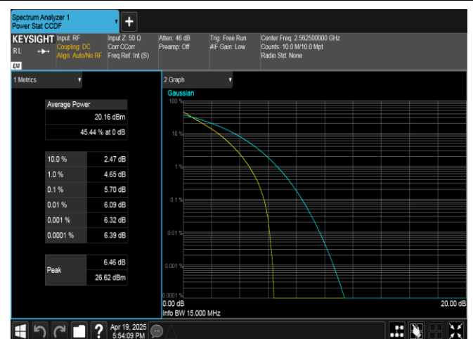
Band7-15MHz-QPSK-21375-75RB#0-PASS
