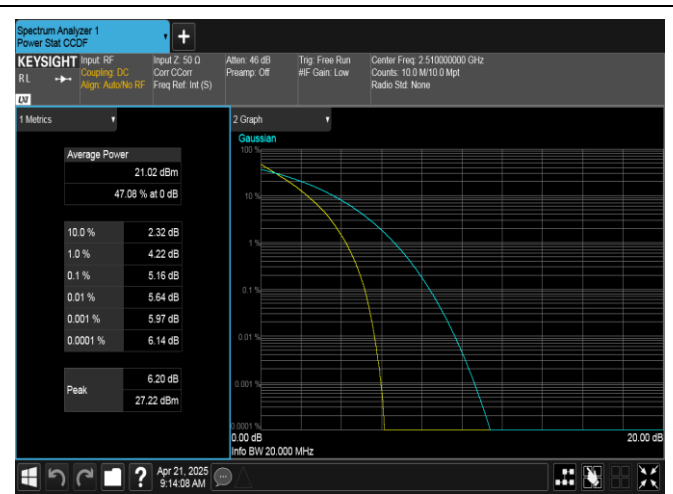
Band7-20MHz-QPSK-20850-100RB#0-PASS
