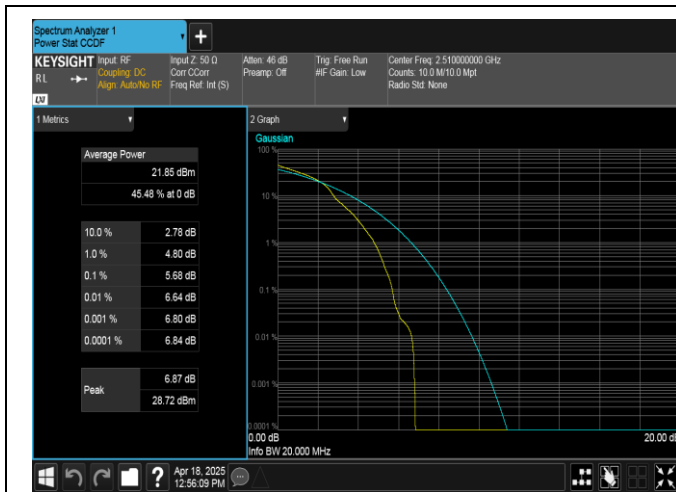
Band7-20MHz-16QAM-20850-1RB#0-PASS
