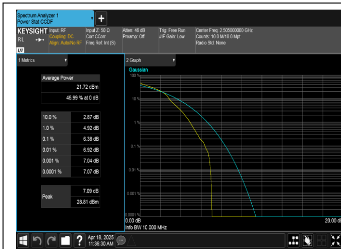
Band7-10MHz-16QAM-20800-1RB#0-PASS
