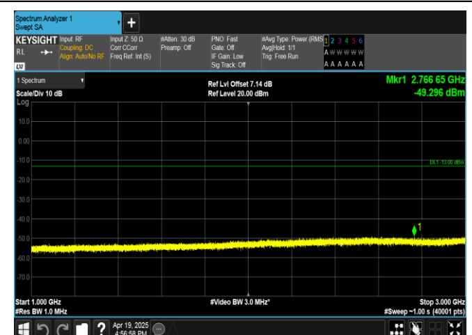
Band5-10MHz-QPSK-20600-50RB#0-1000~3000-PASS
