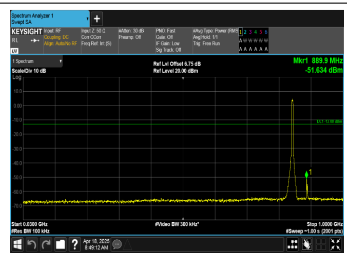
Band5-5MHz-16QAM-20625-25RB#0-30~1000-PASS
