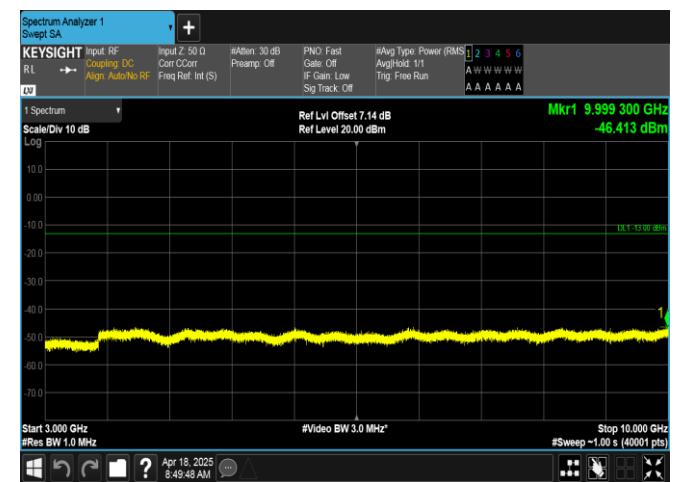
Band5-5MHz-16QAM-20625-25RB#0-3000~10000-PASS
