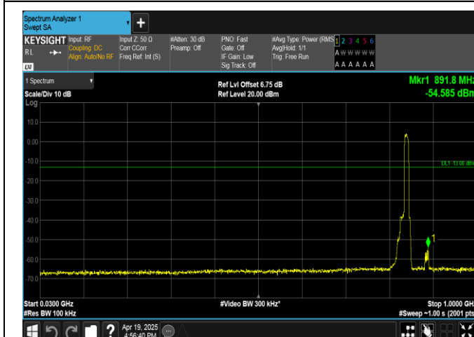
Band5-10MHz-QPSK-20600-50RB#0-30~1000-PASS
