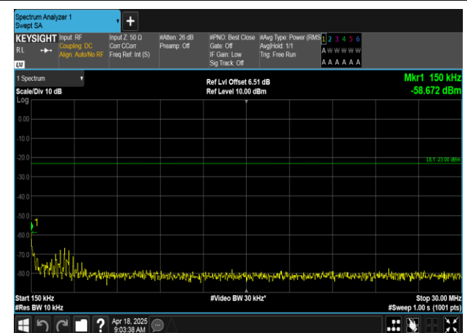
Band5-10MHz-QPSK-20450-1RB#0-0.15~30-PASS
