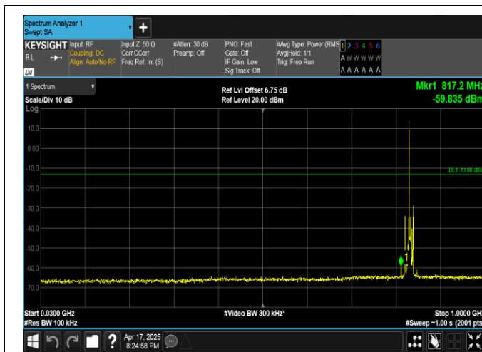
Band5-5MHz-16QAM-20525-1RB#0-30~1000-PASS
