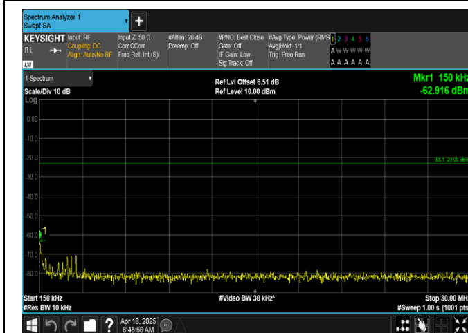
Band5-5MHz-QPSK-20625-1RB#24-0.15~30-PASS
