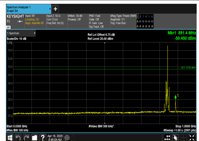
Band5-5MHz-QPSK-20625-1RB#24-30~1000-PASS
