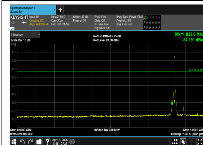
Band5-5MHz-QPSK-20625-25RB#0-30~1000-PASS
