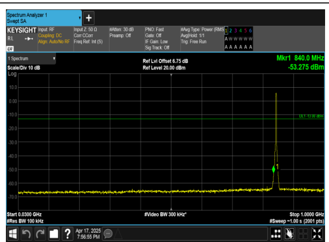
Band5-3MHz-16QAM-20635-15RB#0-30~1000-PASS
