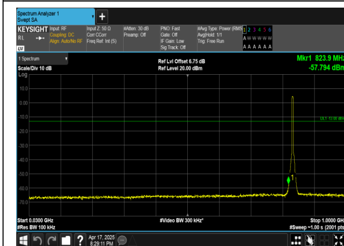
Band5-5MHz-16QAM-20525-25RB#0-30~1000-PASS
