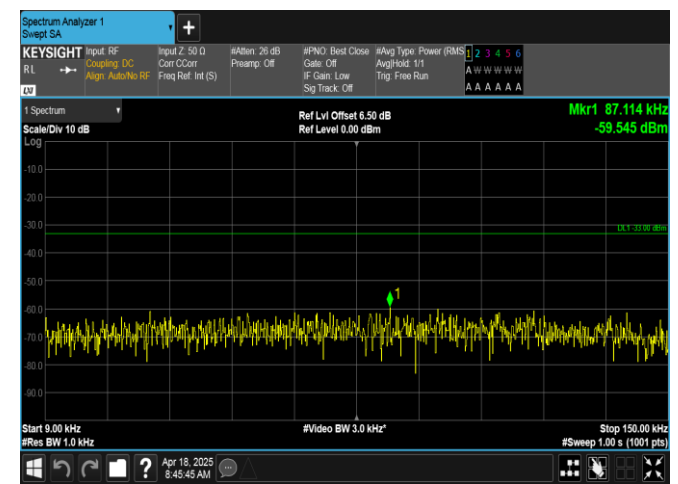
Band5-5MHz-QPSK-20625-1RB#24-0.009~0.15-PASS
