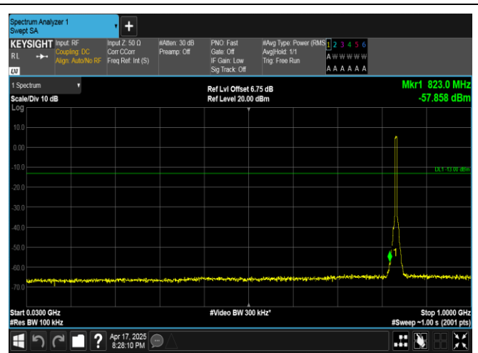
Band5-5MHz-QPSK-20525-25RB#0-30~1000-PASS
