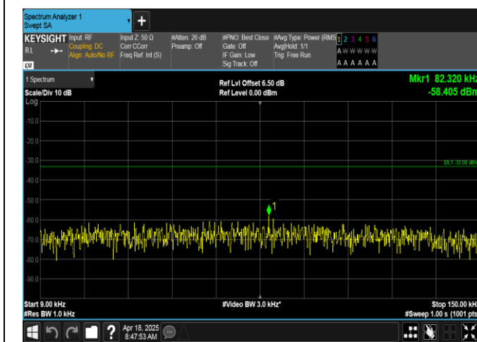
Band5-5MHz-QPSK-20625-25RB#0-0.009~0.15-PASS
