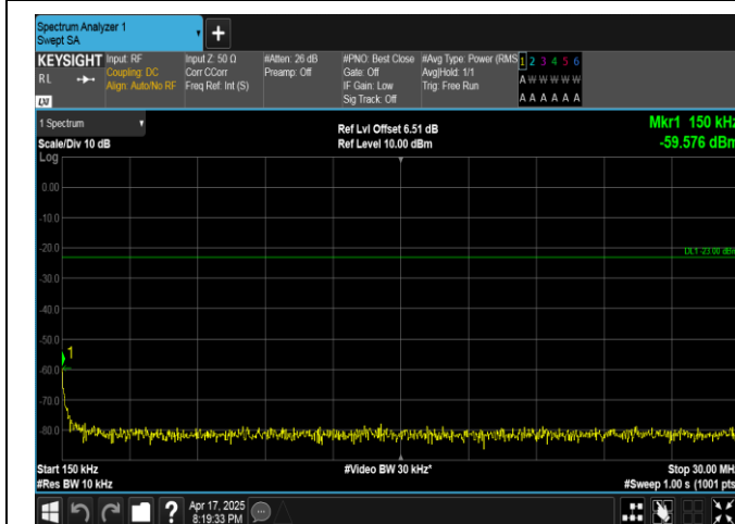
Band5-5MHz-QPSK-20425-1RB#24-0.15~30-PASS
