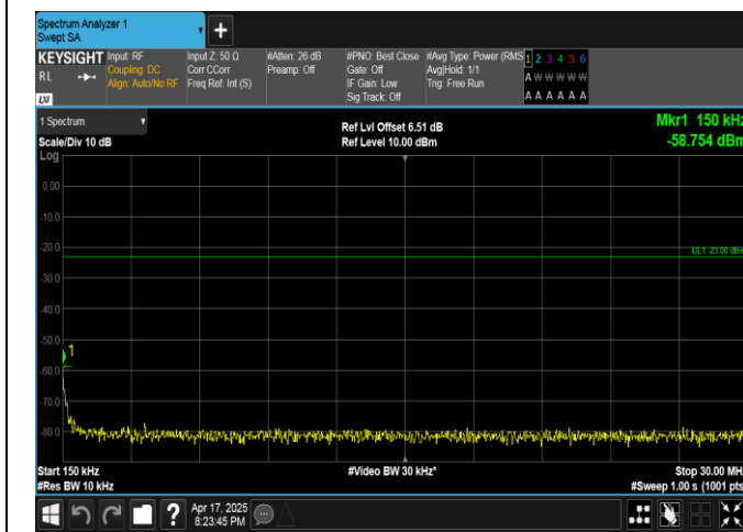
Band5-5MHz-QPSK-20525-1RB#0-0.15~30-PASS
