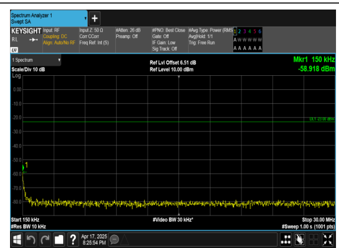
Band5-5MHz-QPSK-20525-1RB#24-0.15~30-PASS
