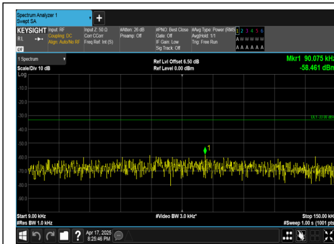
Band5-5MHz-QPSK-20525-1RB#24-0.009~0.15-PASS
