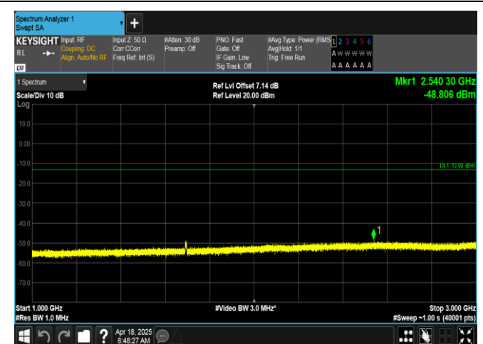
Band5-5MHz-QPSK-20625-25RB#0-1000~3000-PASS
