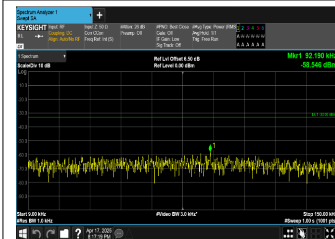
Band5-5MHz-QPSK-20425-1RB#0-0.009~0.15-PASS
