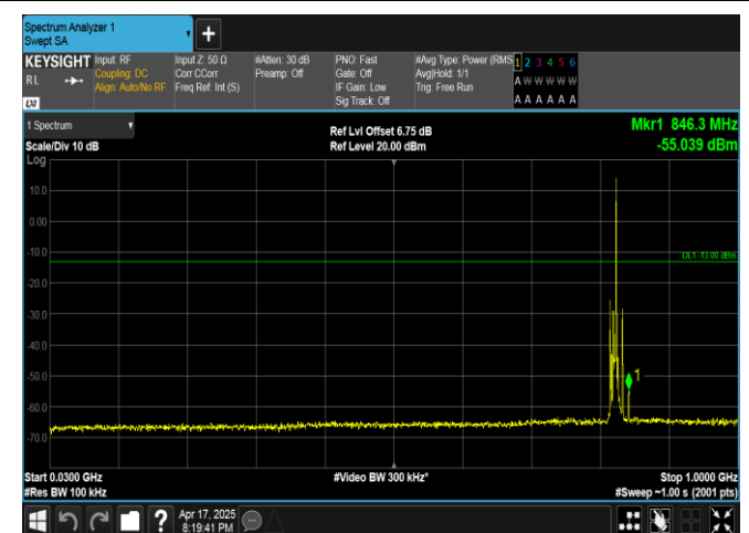
Band5-5MHz-QPSK-20425-1RB#24-30~1000-PASS
