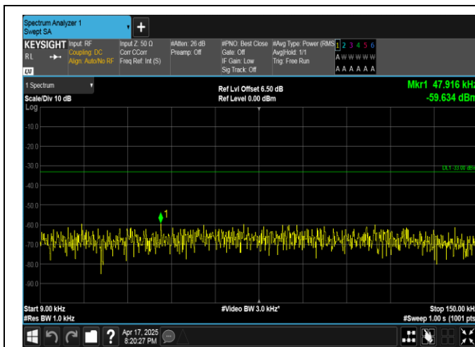
Band5-5MHz-16QAM-20425-1RB#24-0.009~0.15-PASS
