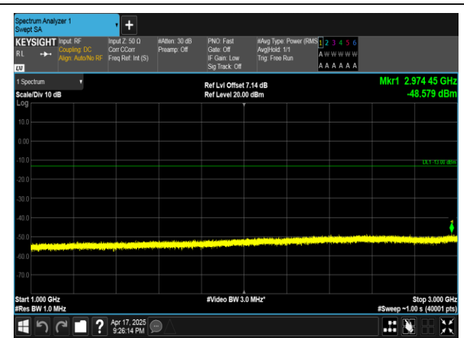
Band5-5MHz-QPSK-20625-1RB#0-1000~3000-PASS
