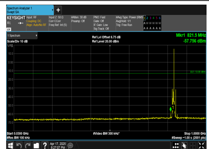
Band5-5MHz-16QAM-20525-1RB#24-30~1000-PASS
