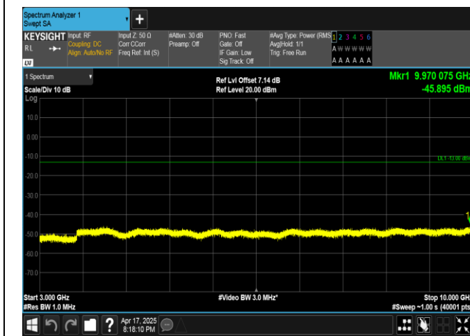
Band5-5MHz-QPSK-20425-1RB#0-3000~10000-PASS
