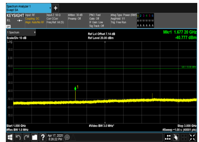
Band5-5MHz-QPSK-20525-1RB#24-1000~3000-PASS
