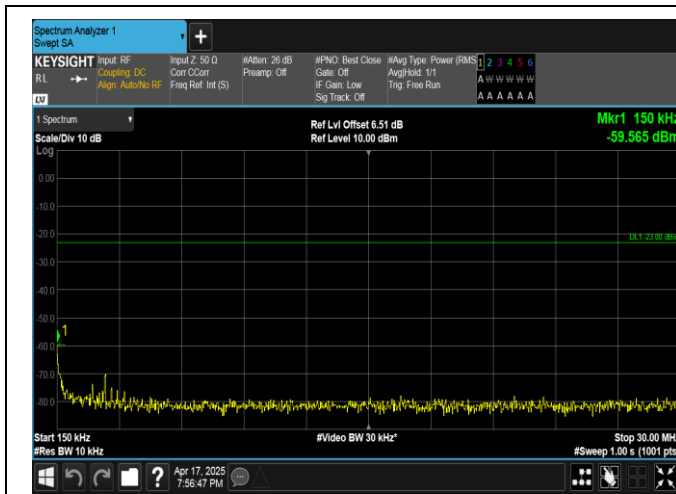
Band5-3MHz-16QAM-20635-15RB#0-0.15~30-PASS
