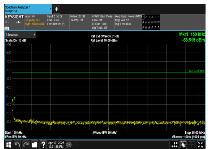
Band5-5MHz-QPSK-20425-25RB#0-0.15~30-PASS
