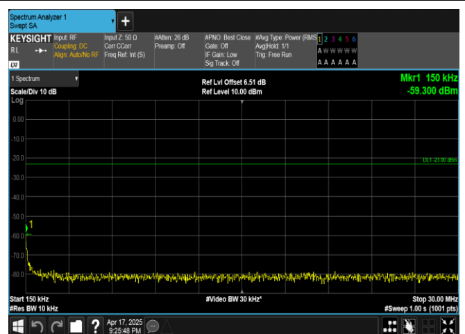
Band5-5MHz-QPSK-20625-1RB#0-0.15~30-PASS
