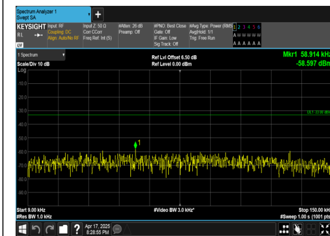
Band5-5MHz-16QAM-20525-25RB#0-0.009~0.15-PASS
