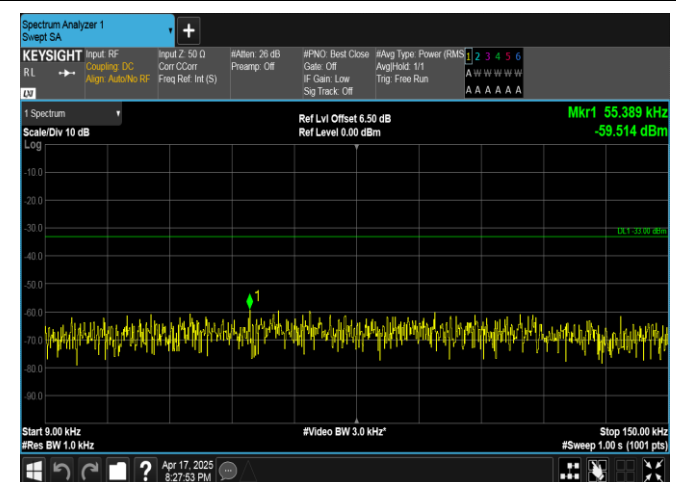
Band5-5MHz-QPSK-20525-25RB#0-0.009~0.15-PASS
