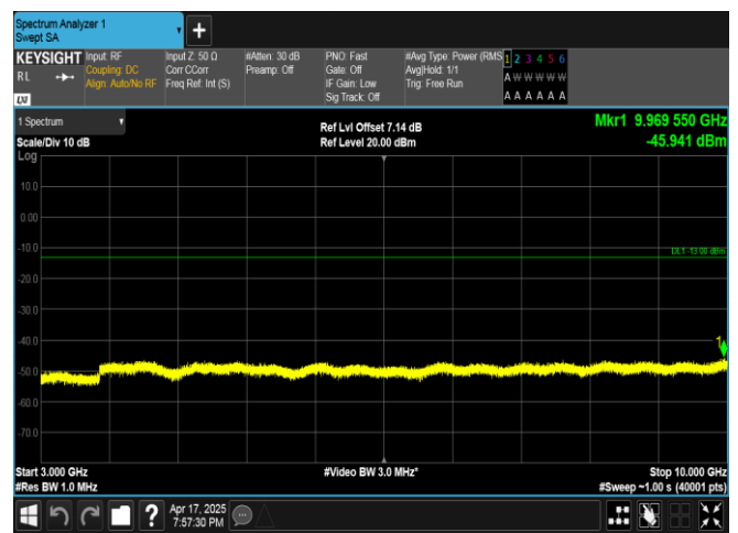
Band5-3MHz-16QAM-20635-15RB#0-3000~10000-PASS
