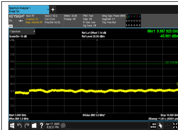
Band5-5MHz-QPSK-20425-25RB#0-3000~10000-PASS
