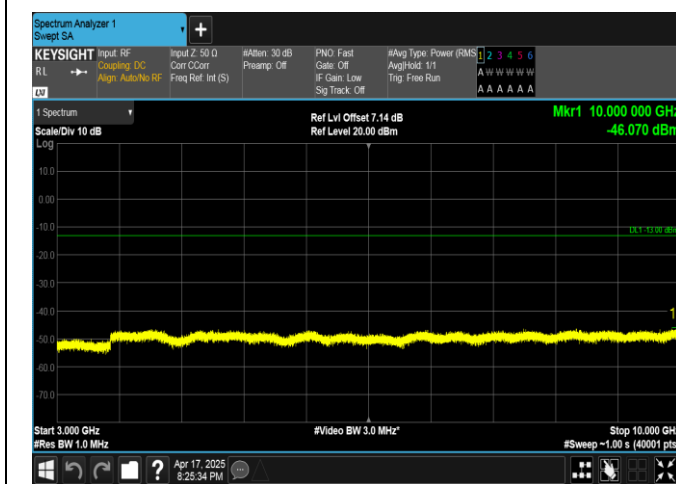
Band5-5MHz-16QAM-20525-1RB#0-3000~10000-PASS
