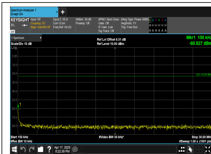
Band5-5MHz-16QAM-20425-25RB#0-0.15~30-PASS
