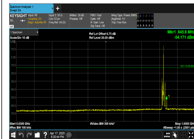
Band5-5MHz-16QAM-20425-1RB#24-30~1000-PASS
