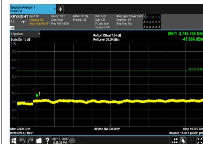
Band5-5MHz-QPSK-20525-1RB#24-3000~10000-PASS
