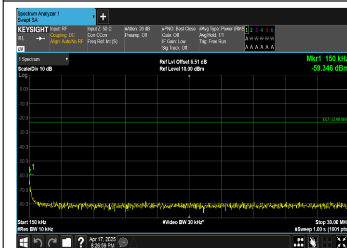
Band5-5MHz-16QAM-20525-1RB#24-0.15~30-PASS
