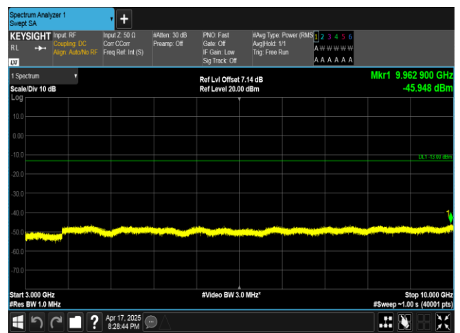
Band5-5MHz-QPSK-20525-25RB#0-3000~10000-PASS
