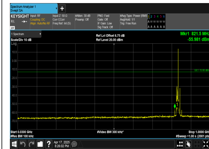
Band5-5MHz-QPSK-20525-1RB#24-30~1000-PASS
