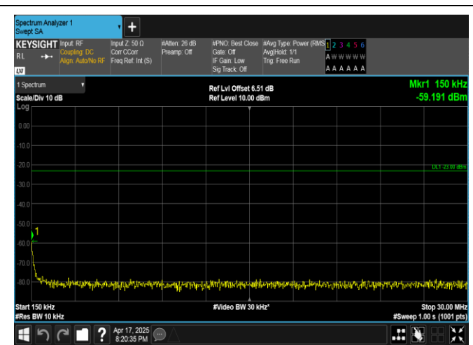
Band5-5MHz-16QAM-20425-1RB#24-0.15~30-PASS
