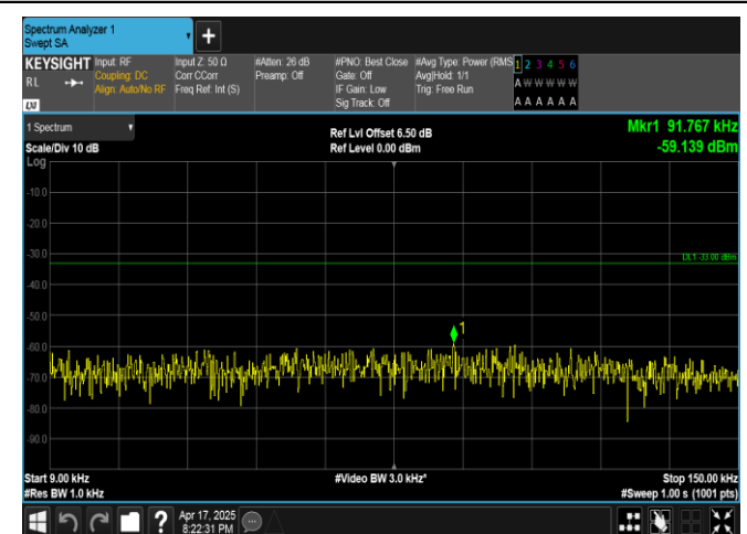
Band5-5MHz-16QAM-20425-25RB#0-0.009~0.15-PASS
