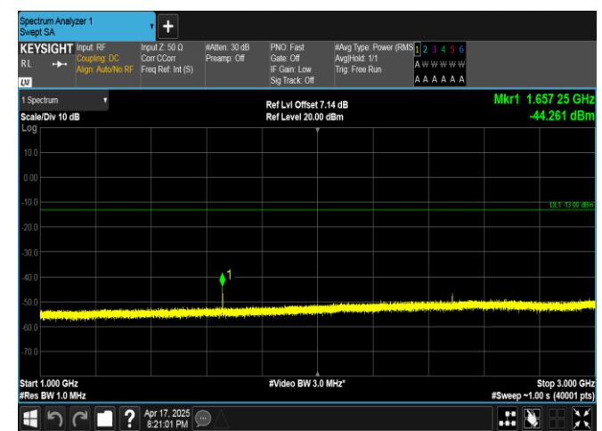
Band5-5MHz-16QAM-20425-1RB#24-1000~3000-PASS
