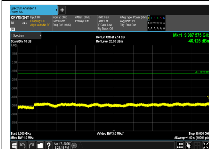
Band5-5MHz-16QAM-20425-1RB#24-3000~10000-PASS
