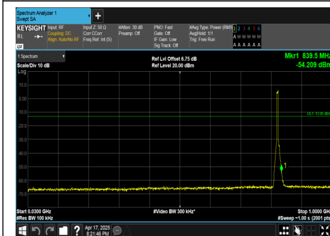
Band5-5MHz-QPSK-20425-25RB#0-30~1000-PASS
