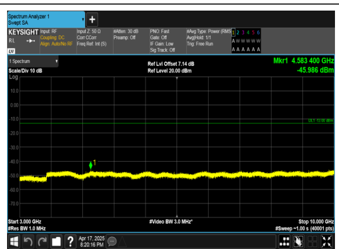
Band5-5MHz-QPSK-20425-1RB#24-3000~10000-PASS
