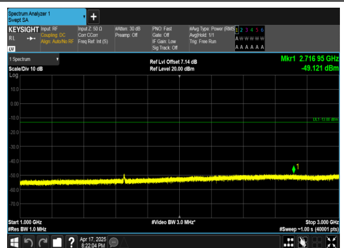
Band5-5MHz-QPSK-20425-25RB#0-1000~3000-PASS
