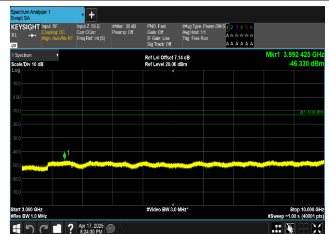
Band5-5MHz-QPSK-20525-1RB#0-3000~10000-PASS
