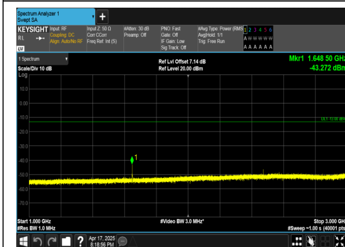
Band5-5MHz-16QAM-20425-1RB#0-1000~3000-PASS
