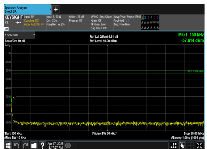
Band5-5MHz-QPSK-20425-1RB#0-0.15~30-PASS
