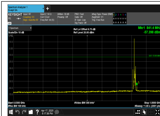
Band5-5MHz-QPSK-20425-1RB#0-30~1000-PASS
