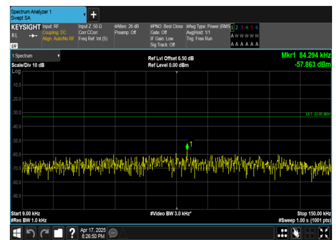
Band5-5MHz-16QAM-20525-1RB#24-0.009~0.15-PASS
