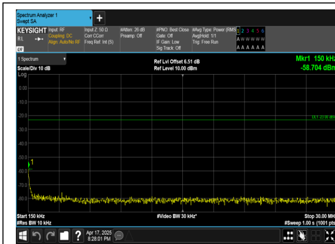
Band5-5MHz-QPSK-20525-25RB#0-0.15~30-PASS
