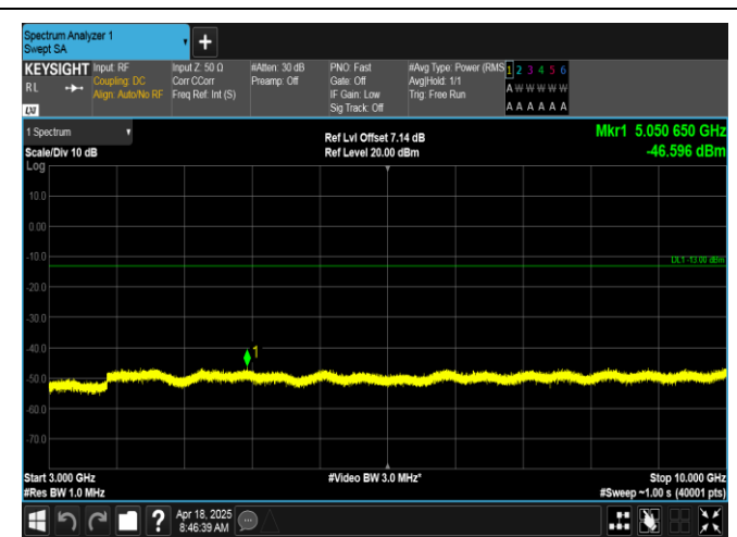
Band5-5MHz-QPSK-20625-1RB#24-3000~10000-PASS
