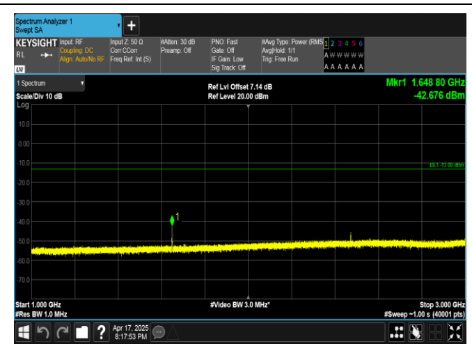
Band5-5MHz-QPSK-20425-1RB#0-1000~3000-PASS
