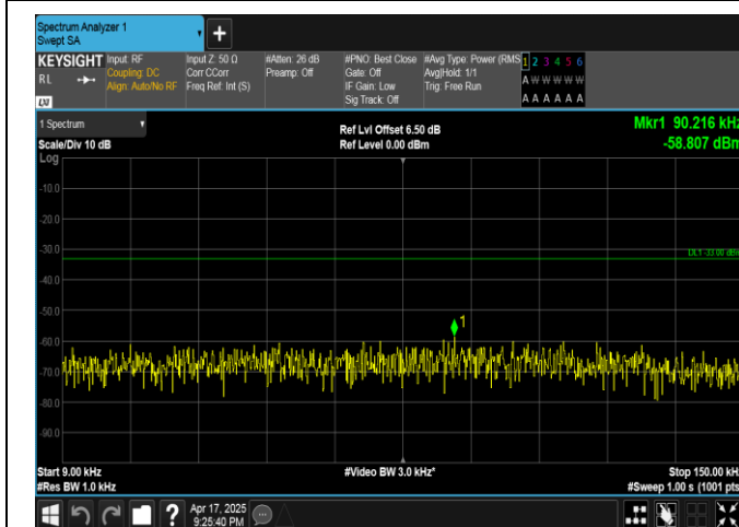
Band5-5MHz-QPSK-20625-1RB#0-0.009~0.15-PASS
