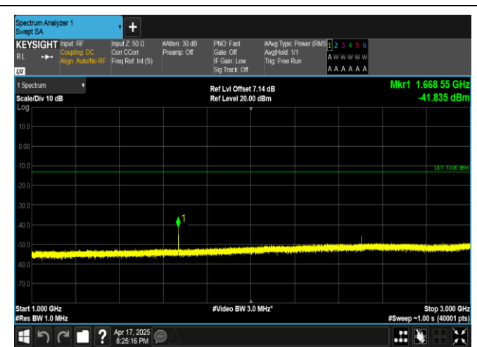
Band5-5MHz-16QAM-20525-1RB#0-1000~3000-PASS
