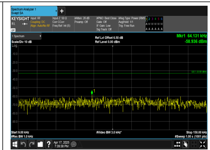
Band5-3MHz-16QAM-20415-1RB#0-0.009~0.15-PASS
