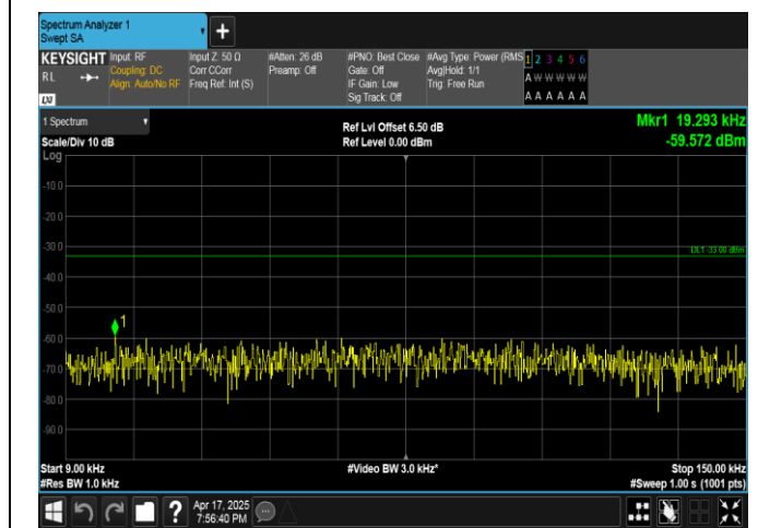
Band5-3MHz-16QAM-20635-15RB#0-0.009~0.15-PASS
