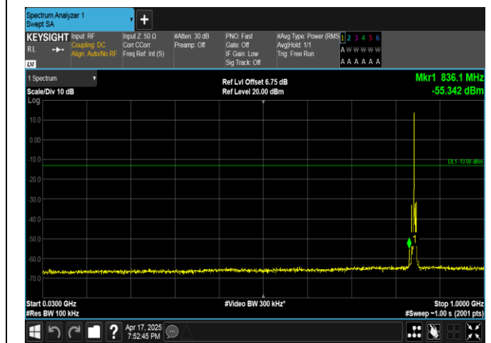
Band5-3MHz-16QAM-20635-1RB#0-30~1000-PASS
