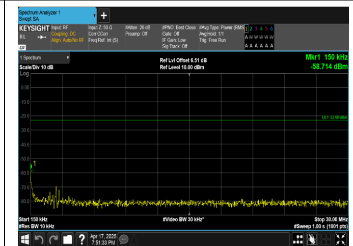
Band5-3MHz-QPSK-20635-1RB#0-0.15~30-PASS
