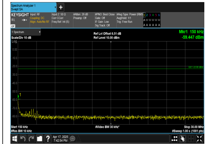
Band5-3MHz-QPSK-20415-15RB#0-0.15~30-PASS
