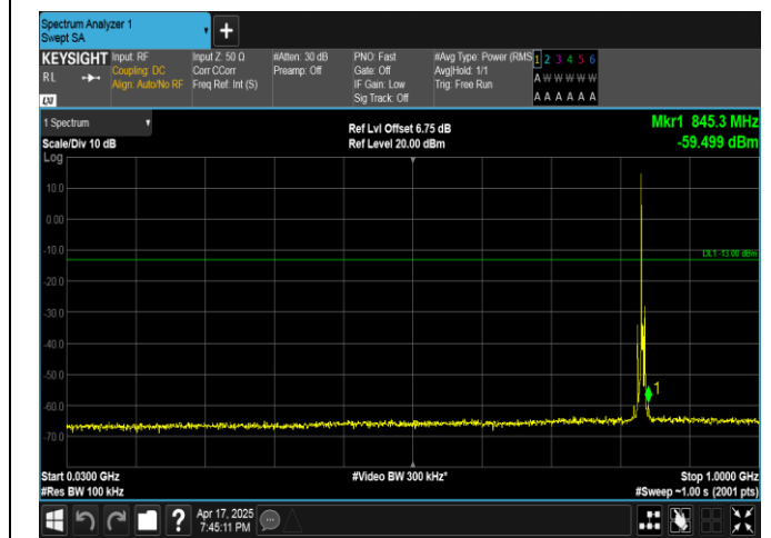
Band5-3MHz-QPSK-20525-1RB#0-30~1000-PASS
