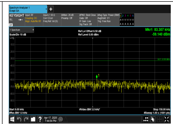
Band5-3MHz-QPSK-20525-1RB#0-0.009~0.15-PASS
