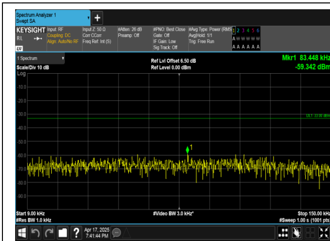
Band5-3MHz-16QAM-20415-1RB#14-0.09~0.15-PASS
