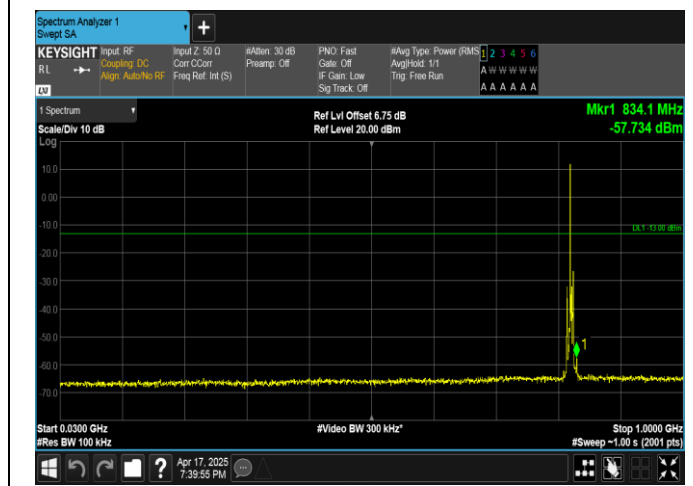
Band5-3MHz-16QAM-20415-1RB#0-30~1000-PASS
