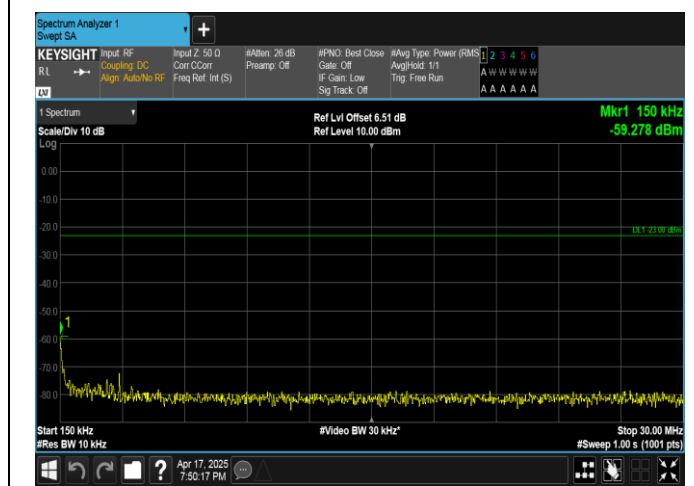
Band5-3MHz-16QAM-20525-15RB#0-0.15~30-PASS
