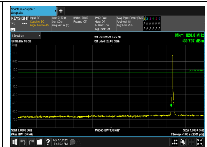
Band5-3MHz-QPSK-20525-15RB#0-30~1000-PASS
