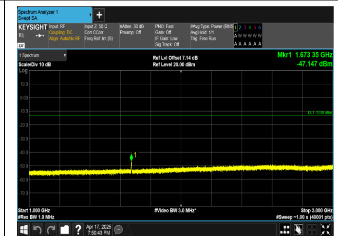
Band5-3MHz-16QAM-20525-15RB#0-1000~3000-PASS
