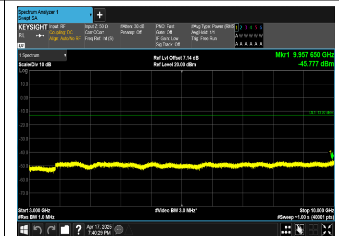
Band5-3MHz-16QAM-20415-1RB#0-3000~10000-PASS
