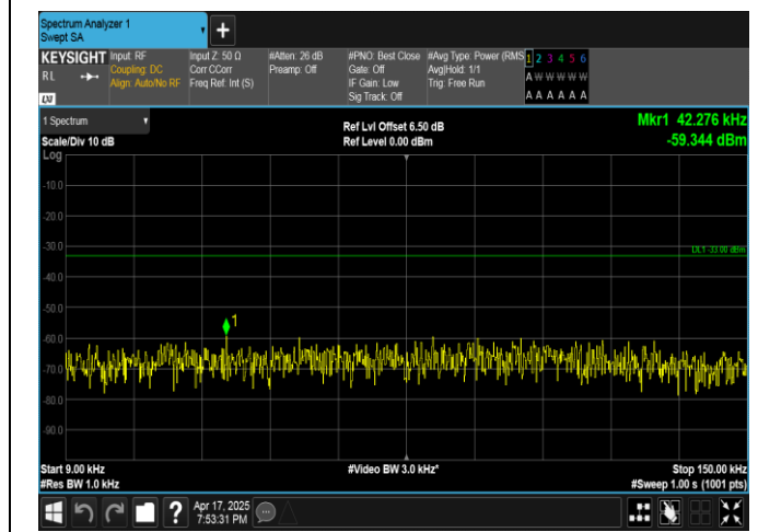
Band5-3MHz-QPSK-20635-1RB#14-0.009~0.15-PASS
