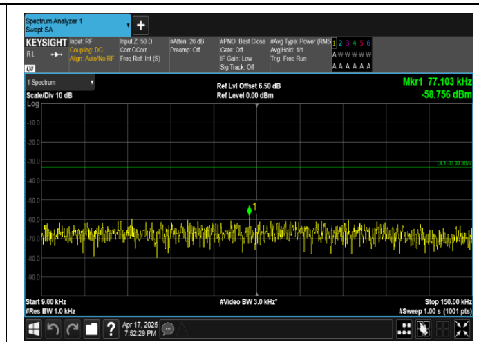
Band5-3MHz-16QAM-20635-1RB#0-0.009~0.15-PASS
