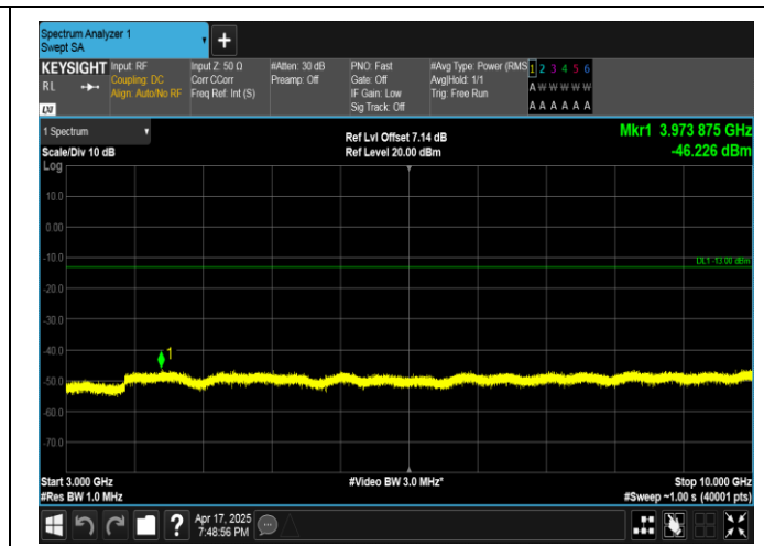
Band5-3MHz-16QAM-20525-1RB#14-3000~10000-PASS
