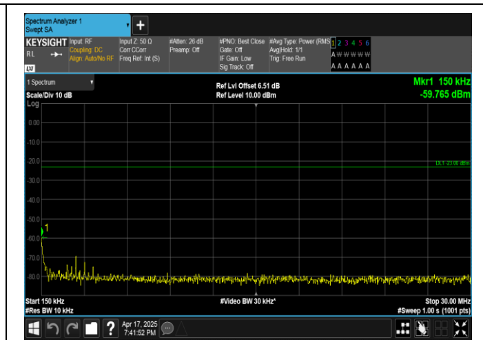
Band5-3MHz-16QAM-20415-1RB#14-0.15~30-PASS
