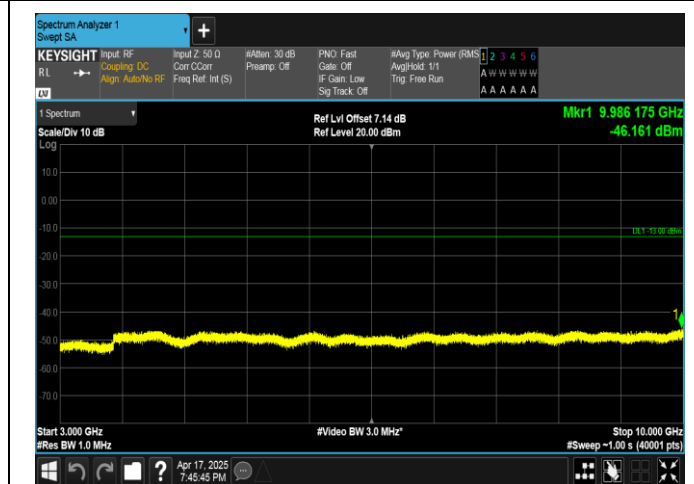
Band5-3MHz-QPSK-20525-1RB#0-3000~10000-PASS
