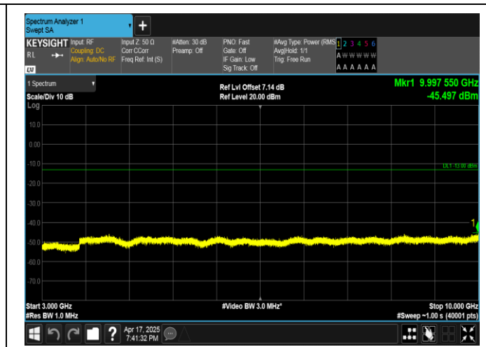
Band5-3MHz-QPSK-20415-1RB#14-3000~10000-PASS
