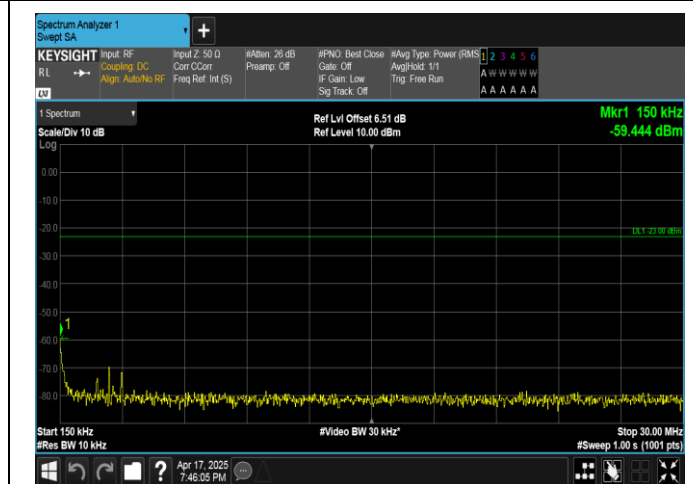
Band5-3MHz-16QAM-20525-1RB#0-0.15~30-PASS
