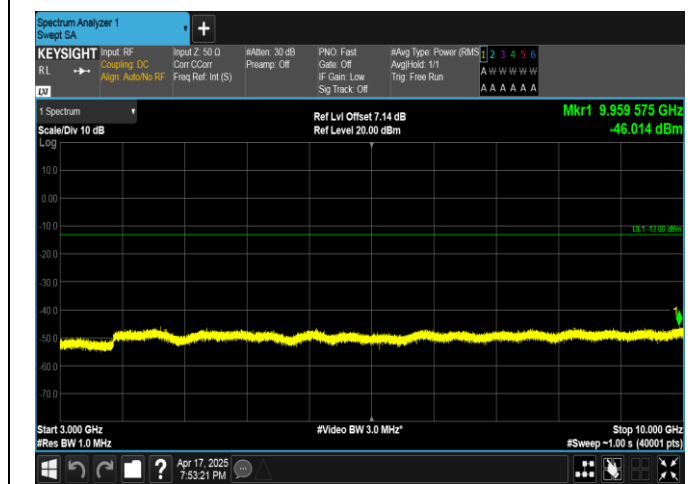
Band5-3MHz-16QAM-20635-1RB#0-3000~10000-PASS
