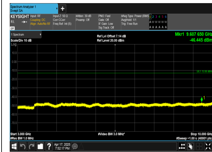
Band5-3MHz-QPSK-20635-1RB#0-3000~10000-PASS
