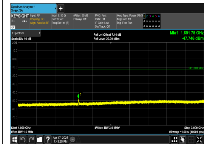
Band5-3MHz-QPSK-20415-15RB#0-1000~3000-PASS
