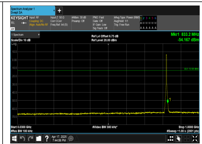
Band5-3MHz-16QAM-20415-15RB#0-30~1000-PASS
