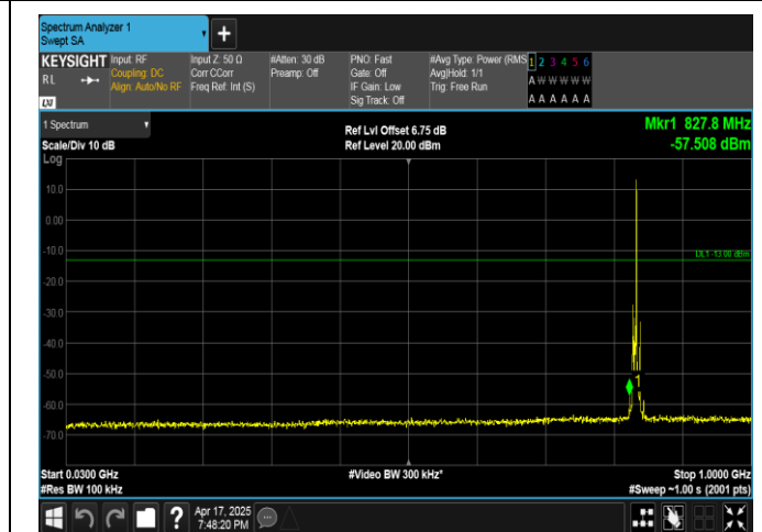
Band5-3MHz-16QAM-20525-1RB#14-30~1000-PASS
