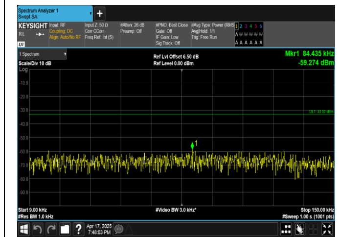
Band5-3MHz-16QAM-20525-1RB#14-0.009~0.15-PASS
