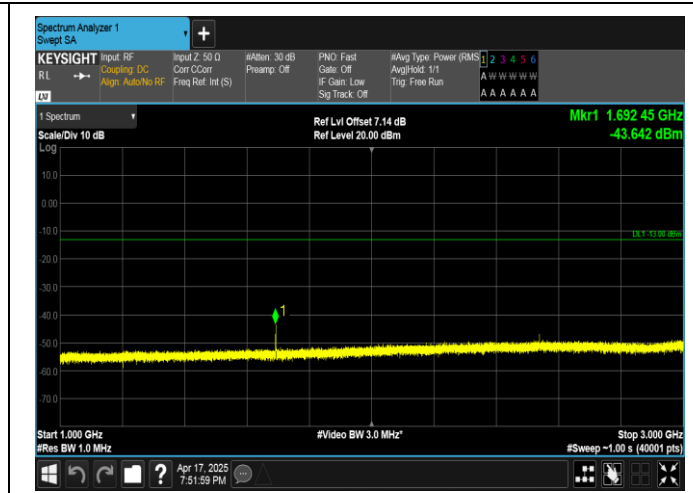
Band5-3MHz-QPSK-20635-1RB#0-1000~3000-PASS
