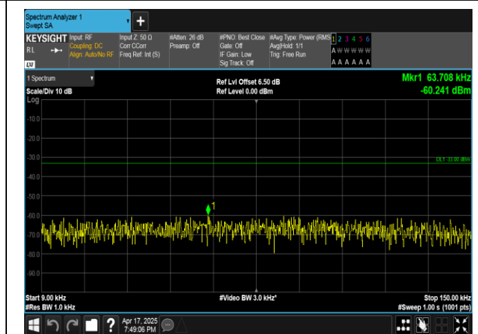
Band5-3MHz-QPSK-20525-15RB#0-0.009~0.15-PASS
