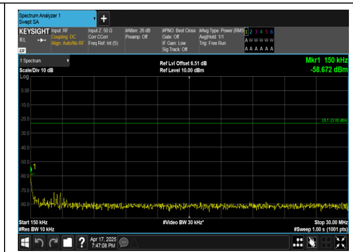
Band5-3MHz-QPSK-20525-1RB#14-0.15~30-PASS
