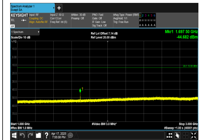
Band5-3MHz-16QAM-20635-1RB#14-1000~3000-PASS
