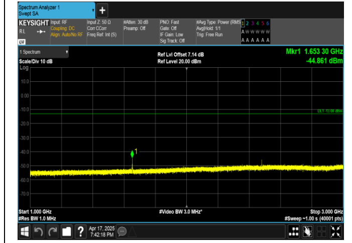
Band5-3MHz-16QAM-20415-1RB#14-1000~3000-PASS
