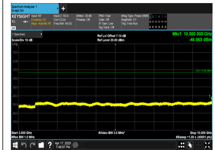
Band5-3MHz-QPSK-20525-15RB#0-3000~10000-PASS
