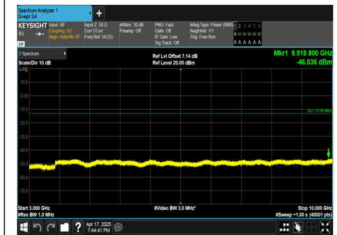
Band5-3MHz-16QAM-20415-15RB#0-3000~10000-PASS
