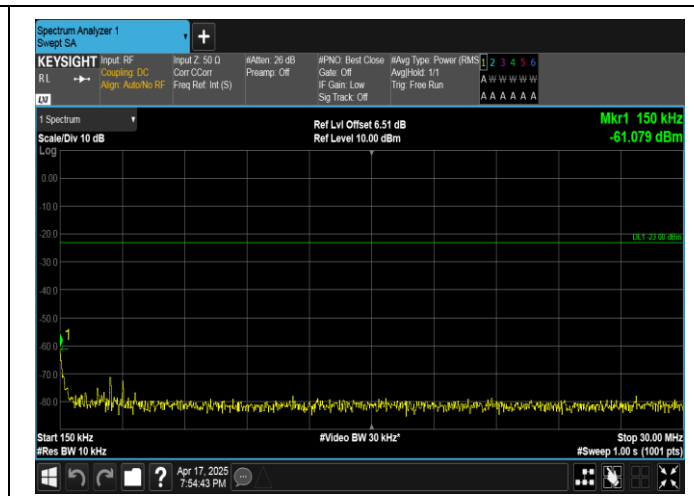
Band5-3MHz-16QAM-20635-1RB#14-0.15~30-PASS
