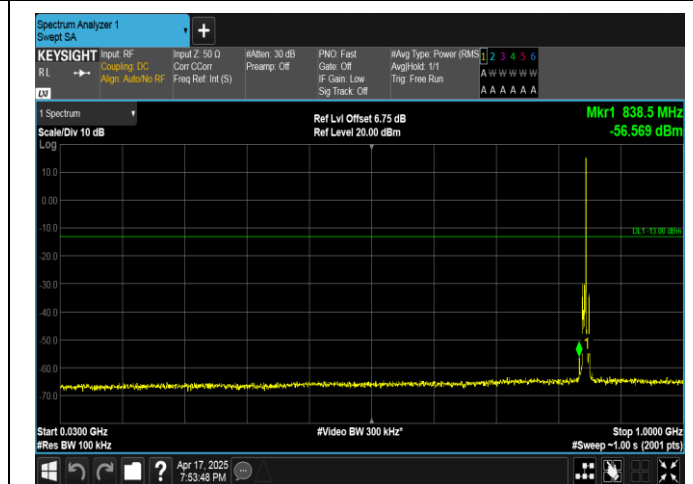
Band5-3MHz-QPSK-20635-1RB#14-30~1000-PASS
