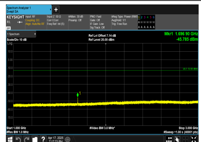
Band5-1.4MHz-QPSK-20643-6RB#0-1000~3000-PASS
