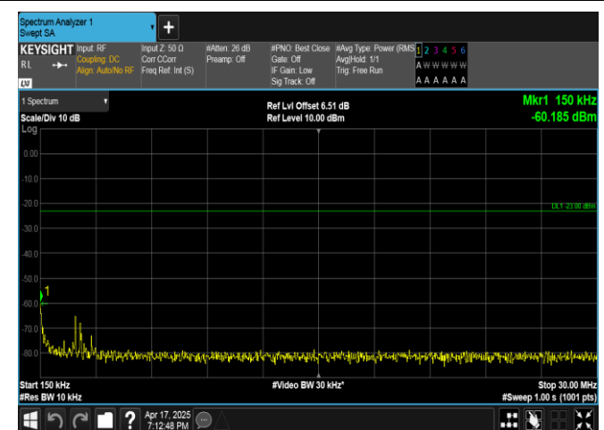
Band5-1.4MHz-QPSK-20643-1RB#0-0.15~30-PASS
