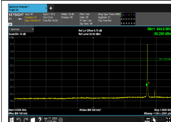
Band5-1.4MHz-QPSK-20643-6RB#0-30~1000-PASS
