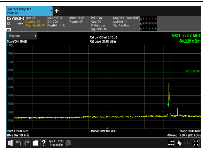
Band5-1.4MHz-QPSK-20525-6RB#0-30~1000-PASS
