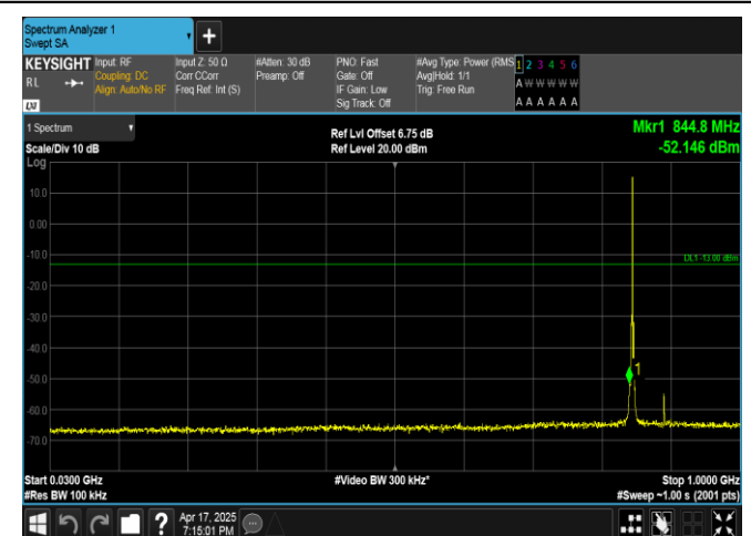
Band5-1.4MHz-QPSK-20643-1RB#5-30~1000-PASS
