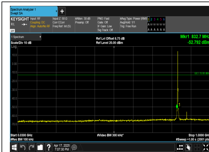
Band5-1.4MHz-16QAM-20525-1RB#0-30~1000-PASS
