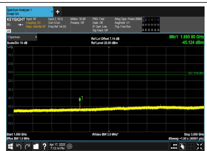
Band5-1.4MHz-QPSK-20643-1RB#0-1000~3000-PASS
