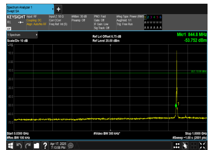
Band5-1.4MHz-16QAM-20643-1RB#0-30~1000-PASS
