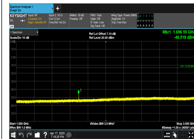
Band5-1.4MHz-16QAM-20643-6RB#0-1000~3000-PASS
