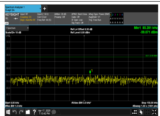
Band5-1.4MHz-16QAM-20643-1RB#0-0.009~0.15-PASS
