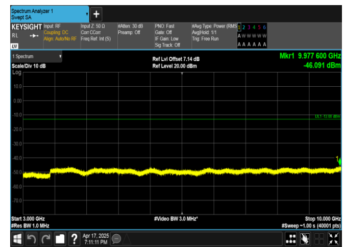
Band5-1.4MHz-QPSK-20525-6RB#0-3000~10000-PASS
