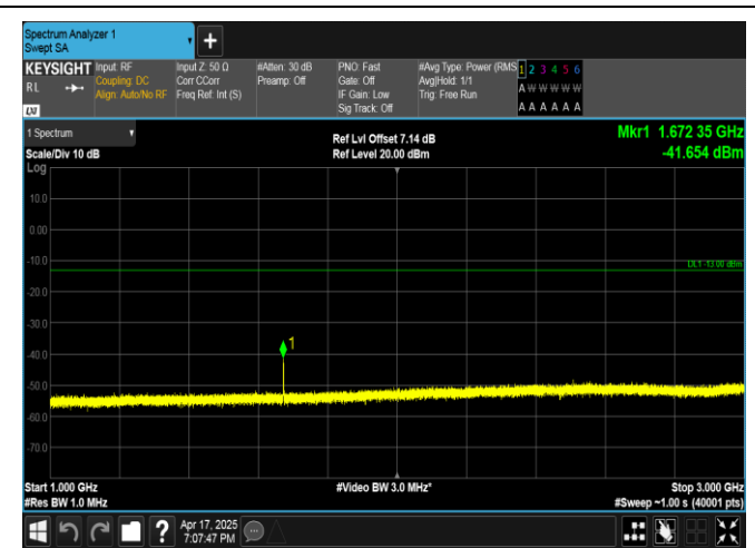
Band5-1.4MHz-16QAM-20525-1RB#0-1000~3000-PASS
