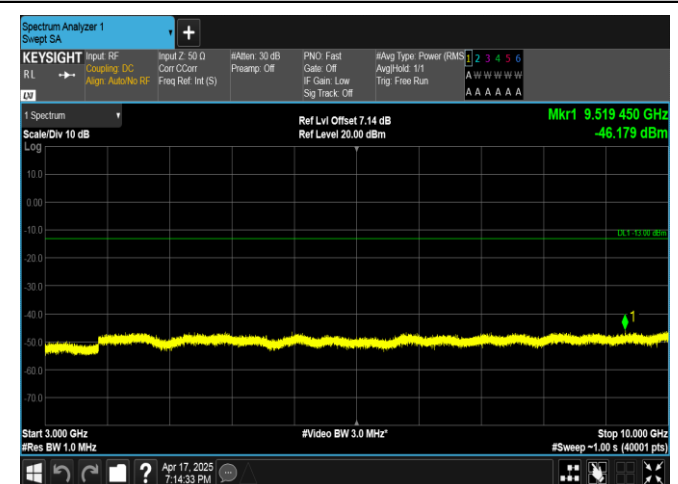
Band5-1.4MHz-16QAM-20643-1RB#0-3000~10000-PASS
