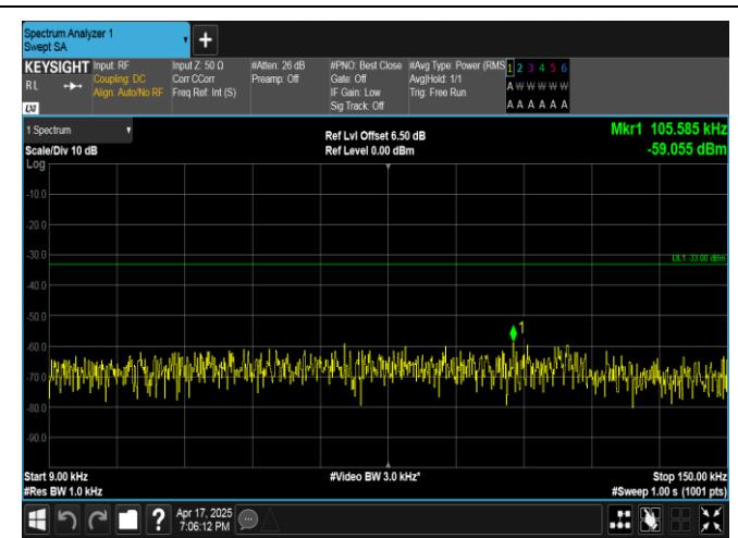
Band5-1.4MHz-QPSK-20525-1RB#0-0.009~0.15-PASS
