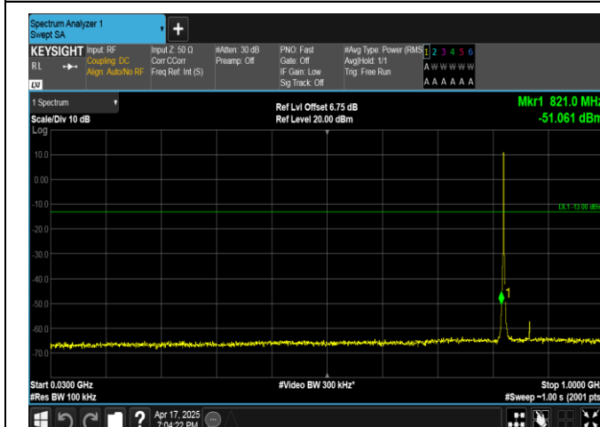
Band5-1.4MHz-QPSK-20407-6RB#0-30~1000-PASS
