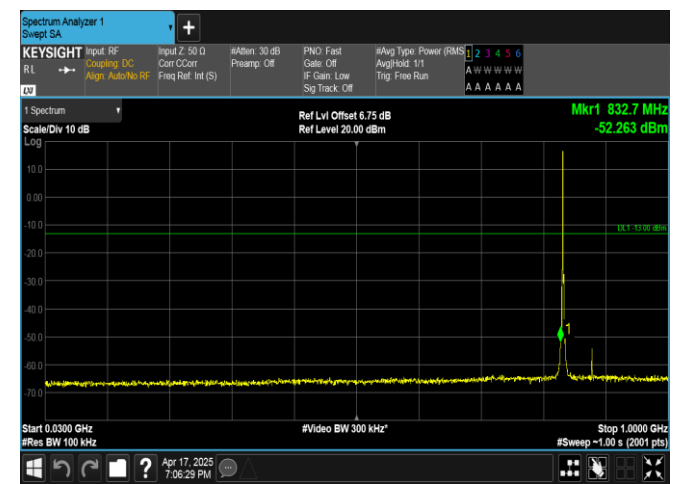
Band5-1.4MHz-QPSK-20525-1RB#0-30~1000-PASS
