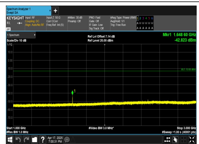
Band5-1.4MHz-QPSK-20407-1RB#0-1000~3000-PASS
