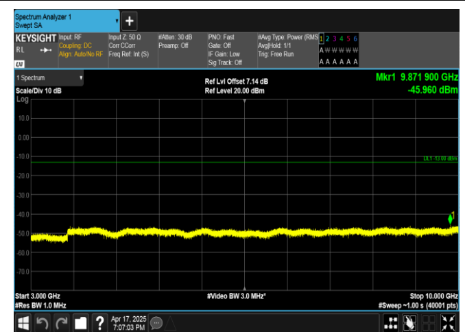
Band5-1.4MHz-QPSK-20525-1RB#0-3000~10000-PASS
