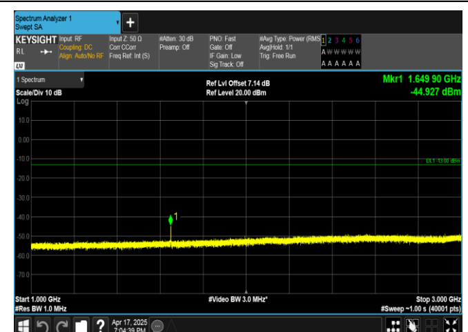
Band5-1.4MHz-QPSK-20407-6RB#0-1000~3000-PASS
