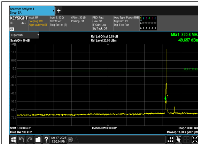
Band5-1.4MHz-QPSK-20407-1RB#0-30~1000-PASS
