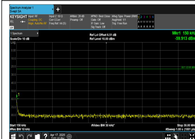
Band5-1.4MHz-QPSK-20407-1RB#5-0.15~30-PASS
