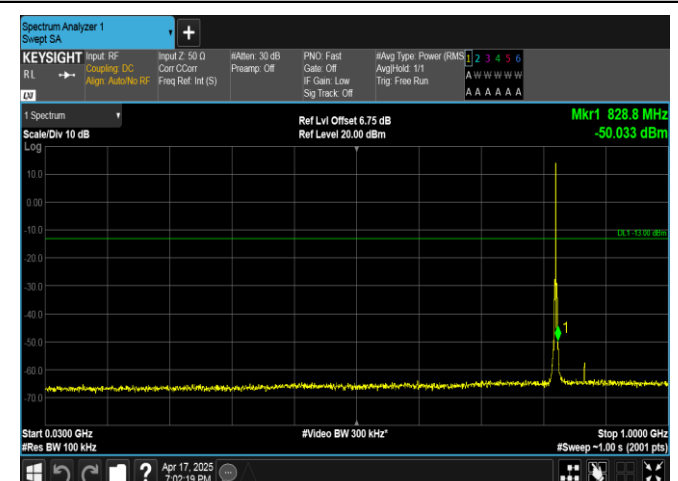
Band5-1.4MHz-QPSK-20407-1RB#5-30~1000-PASS
