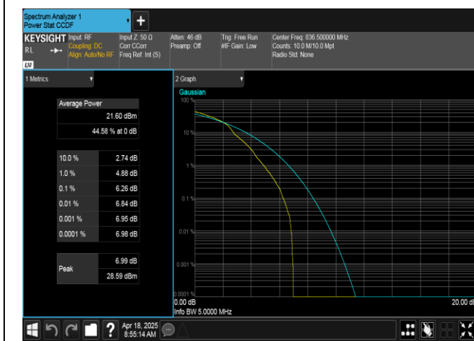
Band5-5MHz-16QAM-20525-1RB#0-PASS
