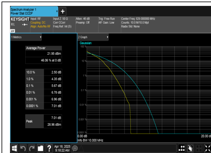
Band5-10MHz-QPSK-20450-1RB#0-PASS
