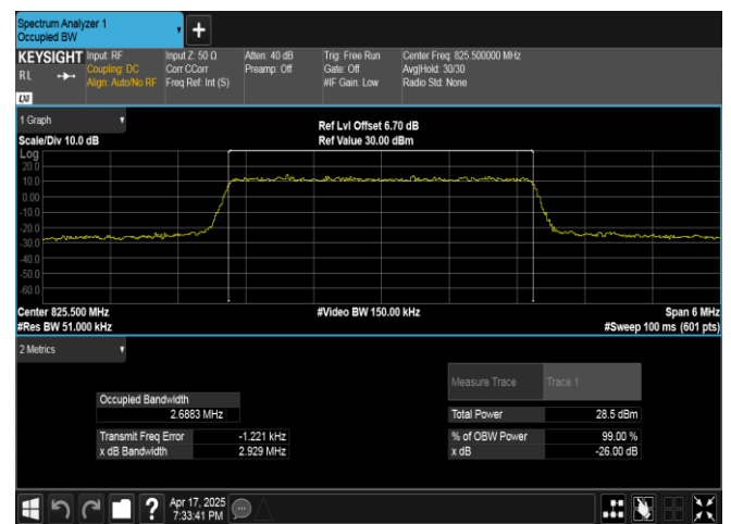
Band5-3MHz-16QAM-20415-15RB#0-PASS
