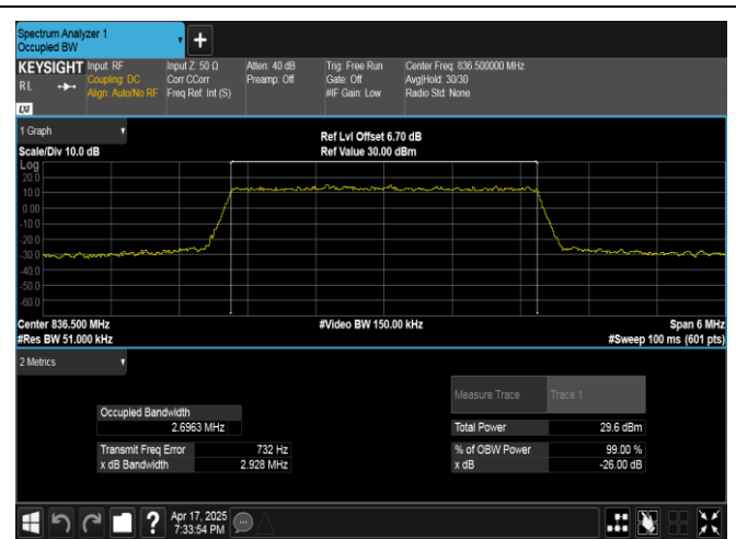
Band5-3MHz-QPSK-20525-15RB#0-PASS
