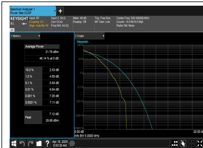
Band5-5MHz-QPSK-20425-1RB#0-PASS
