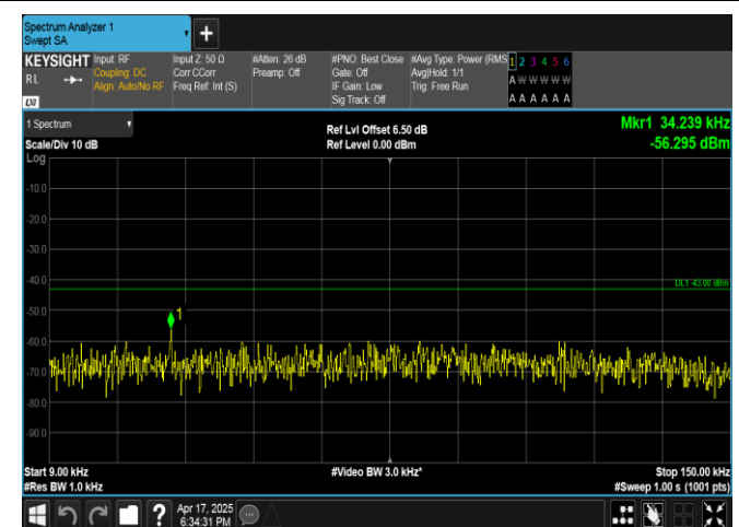
Band4-20MHz-16QAM-20175-1RB#99-0.009~0.15-PASS
