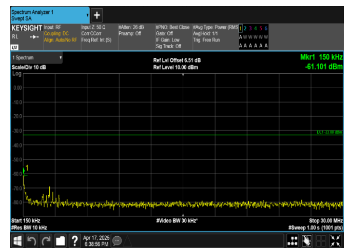
Band4-20MHz-16QAM-20300-1RB#99-0.15~30-PASS
