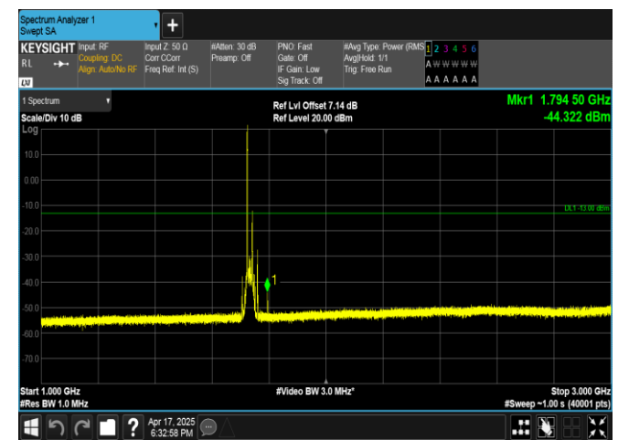
Band4-20MHz-16QAM-20175-1RB#0-1000~3000-PASS
