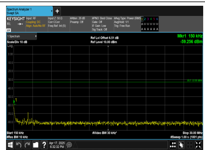
Band4-20MHz-16QAM-20175-1RB#0-0.15~30-PASS
