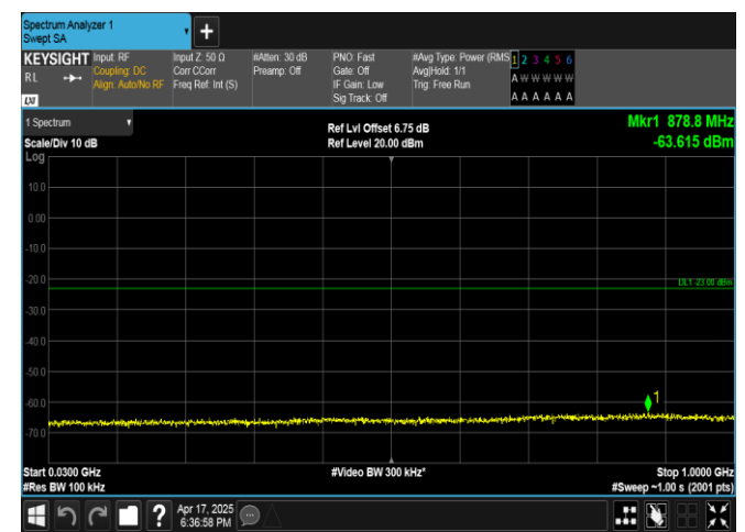
Band4-20MHz-16QAM-20300-1RB#0-30~1000-PASS
