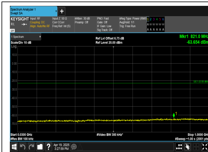
Band4-20MHz-16QAM-20175-100RB#0-30~1000-PASS
