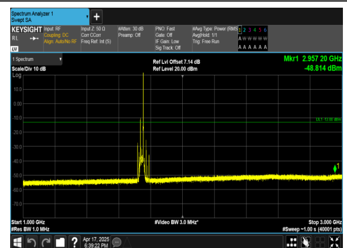
Band4-20MHz-16QAM-20300-1RB#99-1000~3000-PASS
