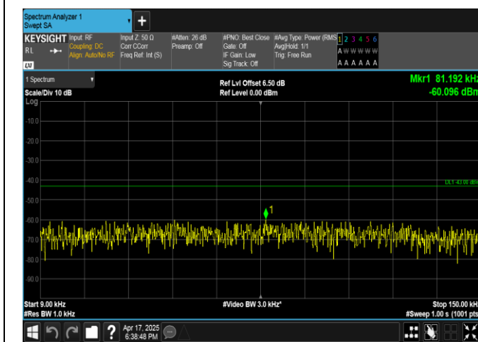
Band4-20MHz-16QAM-20300-1RB#99-0.009~0.15-PASS
