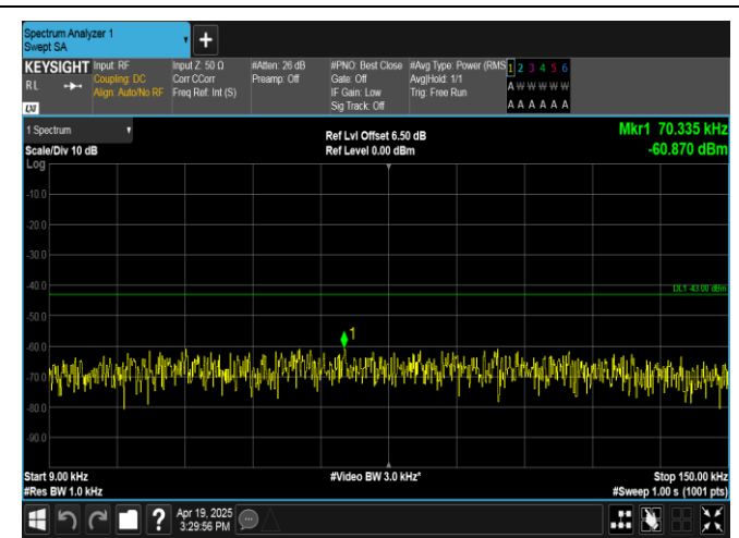
Band4-20MHz-16QAM-20300-100RB#0-0.009~0.15-PASS
