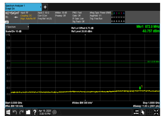
Band4-20MHz-16QAM-20300-100RB#0-30~1000-PASS
