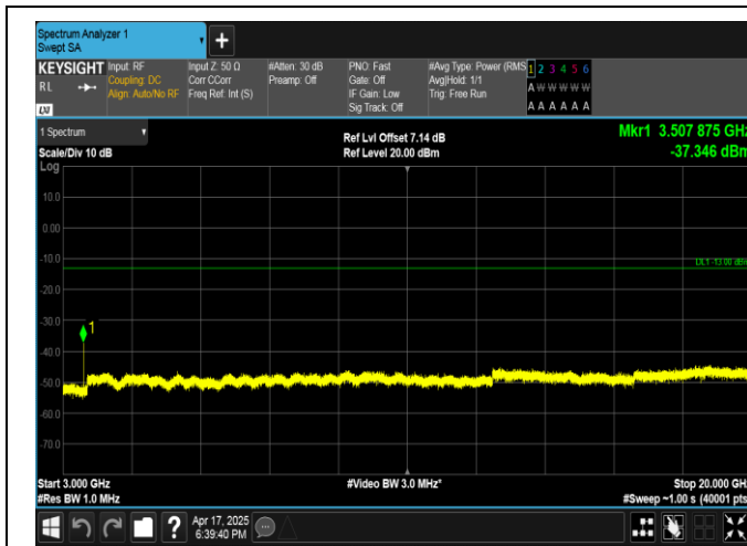
Band4-20MHz-16QAM-20300-1RB#99-3000~20000-PASS
