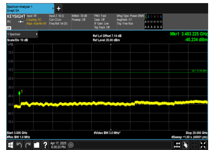
Band4-20MHz-16QAM-20175-1RB#99-3000~20000-PASS
