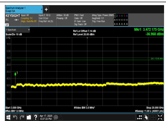
Band4-20MHz-16QAM-20300-1RB#0-3000~20000-PASS
