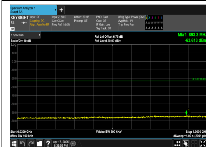
Band4-20MHz-16QAM-20300-1RB#99-30~1000-PASS
