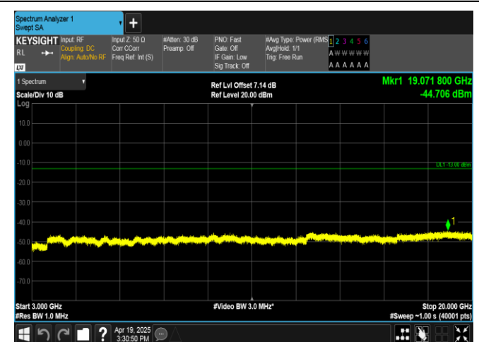
Band4-20MHz-16QAM-20300-100RB#0-3000~20000-PAS
