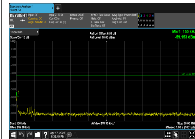
Band4-20MHz-16QAM-20300-1RB#0-0.15~30-PASS
