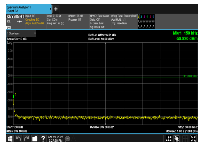
Band4-20MHz-16QAM-20175-100RB#0-0.15~30-PASS
