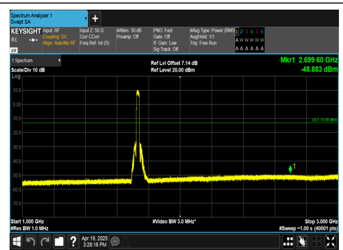
Band4-20MHz-16QAM-20175-100RB#0-1000~3000-PASS
