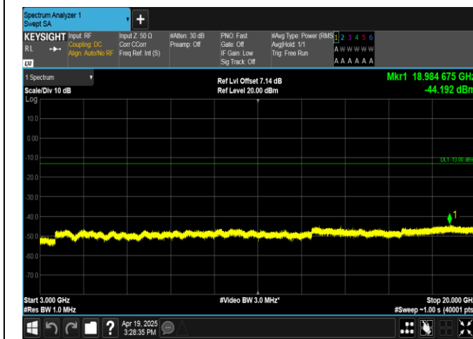
Band4-20MHz-16QAM-20175-100RB#0-3000~20000-PAS S
