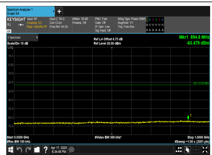
Band4-20MHz-16QAM-20175-1RB#99-30~1000-PASS
