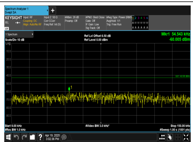
Band4-15MHz-QPSK-20175-75RB#0-0.009~0.15-PASS
