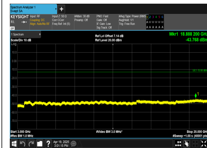
Band4-15MHz-QPSK-20025-75RB#0-3000~20000-PASS
