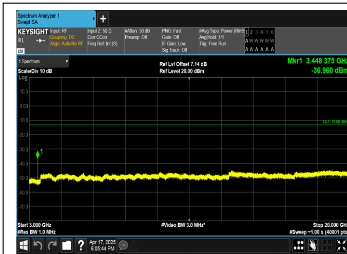
Band4-15MHz-16QAM-20025-1RB#74-3000~20000-PASS
