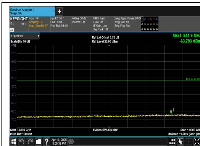
Band4-15MHz-QPSK-20025-75RB#0-30~1000-PASS
