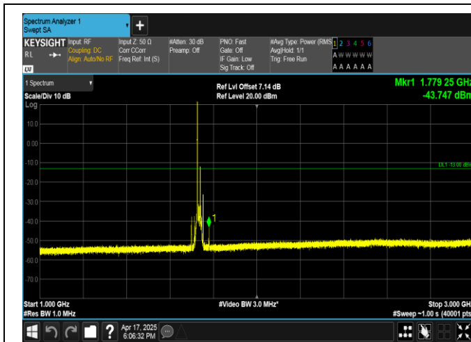
Band4-15MHz-QPSK-20175-1RB#0-1000~3000-PASS
