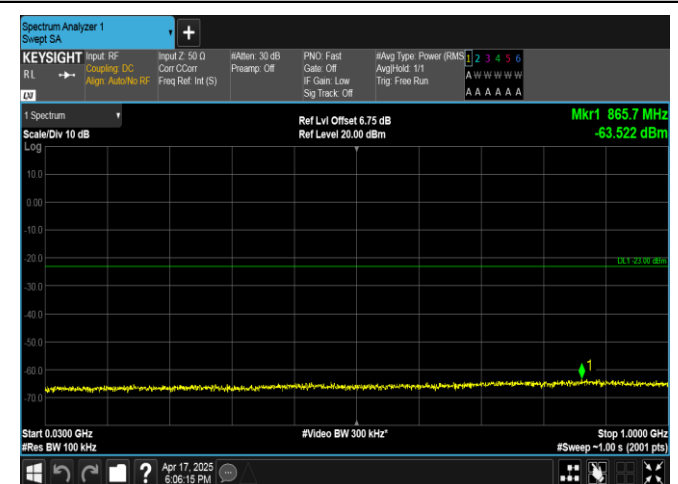
Band4-15MHz-QPSK-20175-1RB#0-30~1000-PASS
