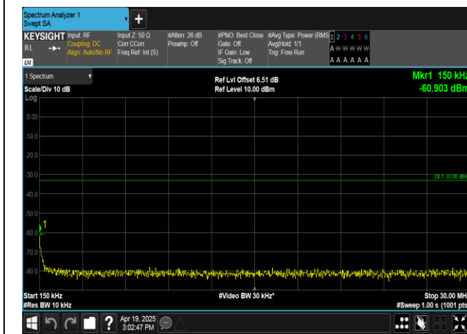
Band4-15MHz-QPSK-20175-75RB#0-0.15~30-PASS
