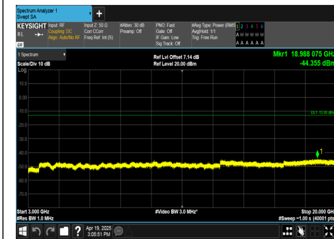
Band4-15MHz-QPSK-20325-75RB#0-3000~20000-PASS
