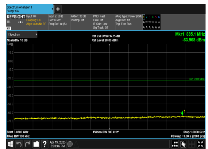
Band4-15MHz-16QAM-20025-75RB#0-30~1000-PASS
