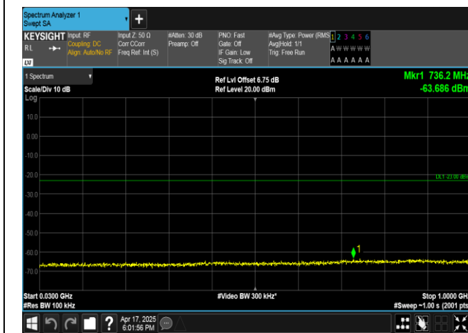
Band4-15MHz-QPSK-2025-1RB#0-30~1000-PASS
