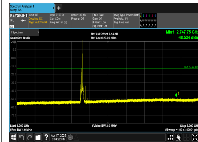
Band4-15MHz-QPSK-20025-1RB#74-1000~3000-PASS
