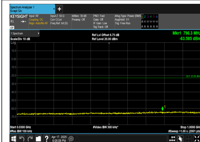
Band4-15MHz-16QAM-2025-1RB#74-30~1000-PASS
