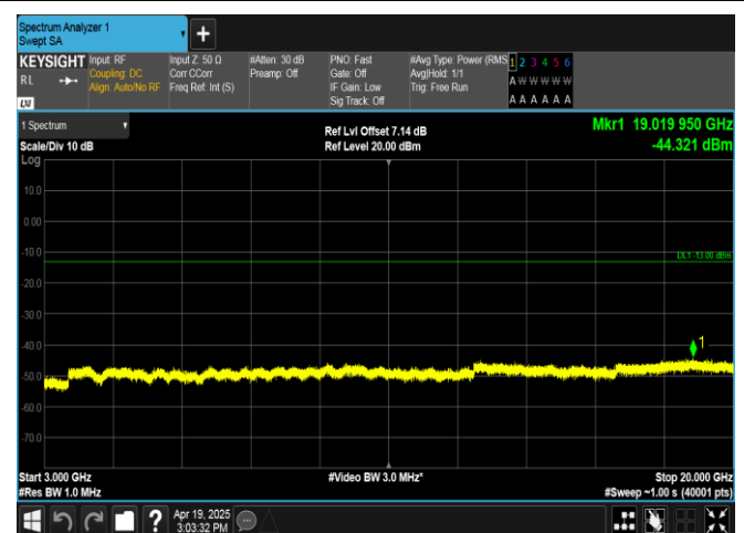
Band4-15MHz-QPSK-20175-75RB#0-3000~20000-PASS
