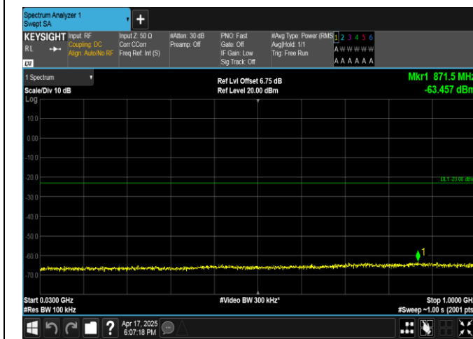
Band4-15MHz-16QAM-20175-1RB#0-30~1000-PASS
