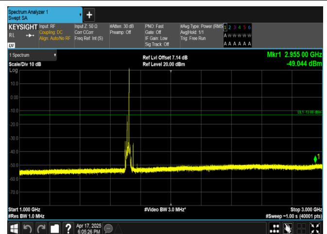
Band4-15MHz-16QAM-2025-1RB#74-1000~3000-PASS
