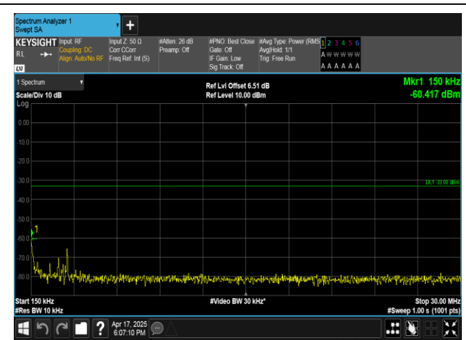
Band4-15MHz-16QAM-20175-1RB#0-0.15~30-PASS
