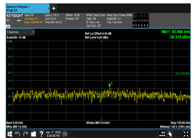
Band4-15MHz-QPSK-20175-1RB#0-0.009~0.15-PASS
