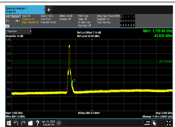
Band4-15MHz-QPSK-20025-75RB#0-1000~3000-PASS
