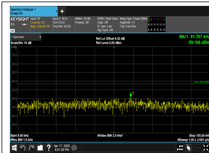
Band4-15MHz-QPSK-2025-1RB#0-0.009~0.15-PASS
