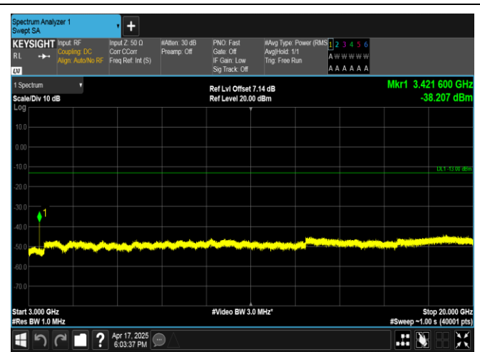
Band4-15MHz-16QAM-2025-1RB#0-3000~20000-PASS
