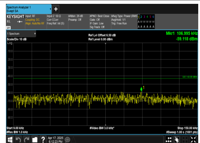
Band4-15MHz-QPSK-20325-1RB#74-0.009~0.15-PASS
