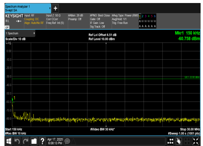
Band4-15MHz-QPSK-20175-1RB#74-0.15~30-PASS
