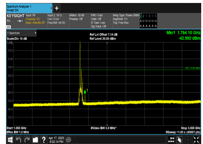
Band4-15MHz-QPSK-2025-1RB#0-1000~3000-PASS
