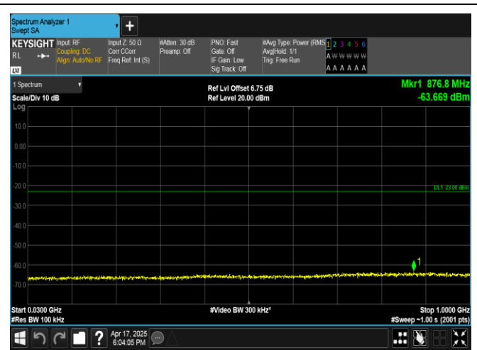
Band4-15MHz-QPSK-20025-1RB#74-30~1000-PASS
