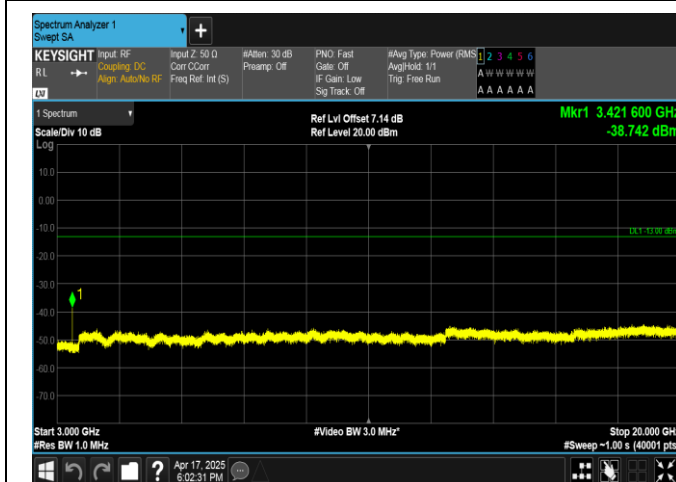
Band4-15MHz-QPSK-2025-1RB#0-3000~20000-PASS
