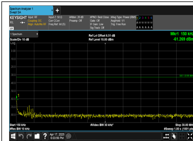
Band4-15MHz-QPSK-20025-1RB#74-0.15~30-PASS
