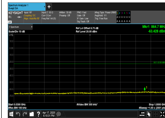
Band4-15MHz-QPSK-20325-1RB#0-30~1000-PASS
