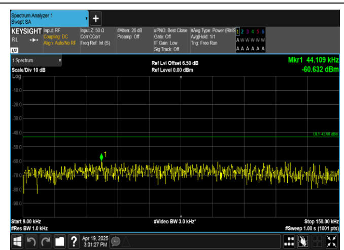
Band4-15MHz-16QAM-20025-75RB#0-0.009~0.15-PASS
