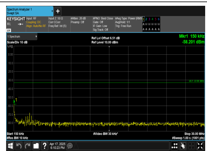
Band4-15MHz-QPSK-20325-1RB#0-0.15~30-PASS
