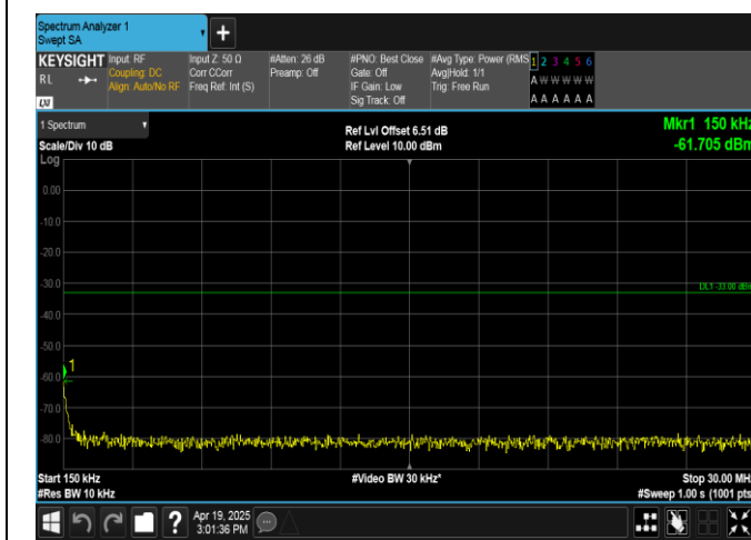
Band4-15MHz-16QAM-20025-75RB#0-0.15~30-PASS
