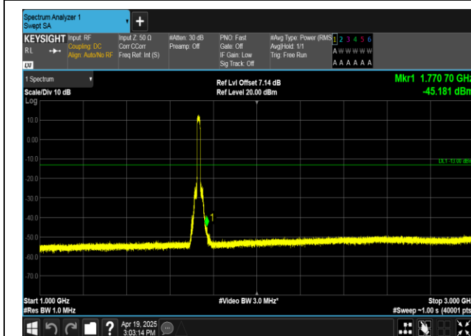
Band4-15MHz-QPSK-20175-75RB#0-1000~3000-PASS
