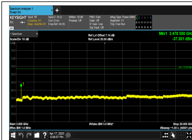
Band4-15MHz-QPSK-20175-1RB#74-3000~20000-PASS
