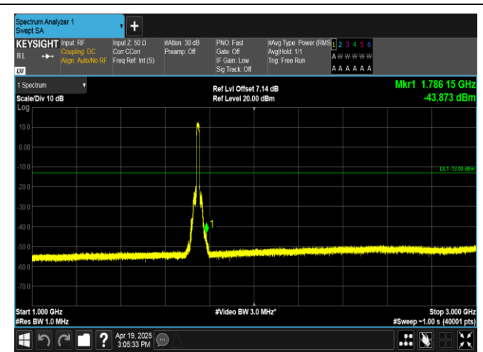
Band4-15MHz-QPSK-20325-75RB#0-1000~3000-PASS
