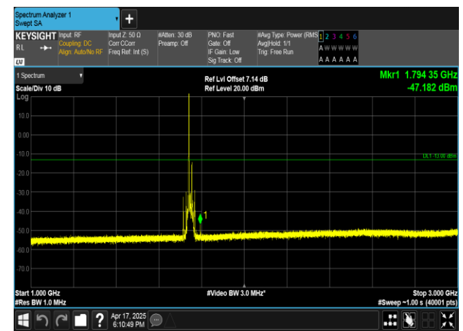
Band4-15MHz-QPSK-20325-1RB#0-1000~3000-PASS
