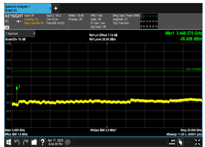
Band4-15MHz-QPSK-20025-1RB#74-3000~20000-PASS
