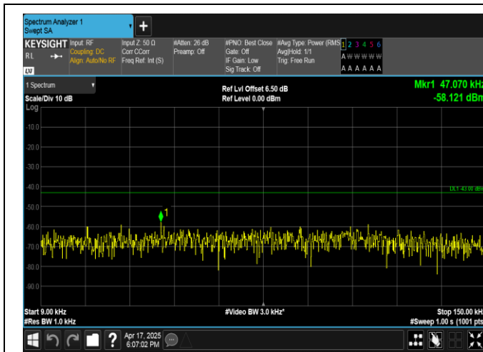
Band4-15MHz-16QAM-20175-1RB#0-0.009~0.15-PASS
