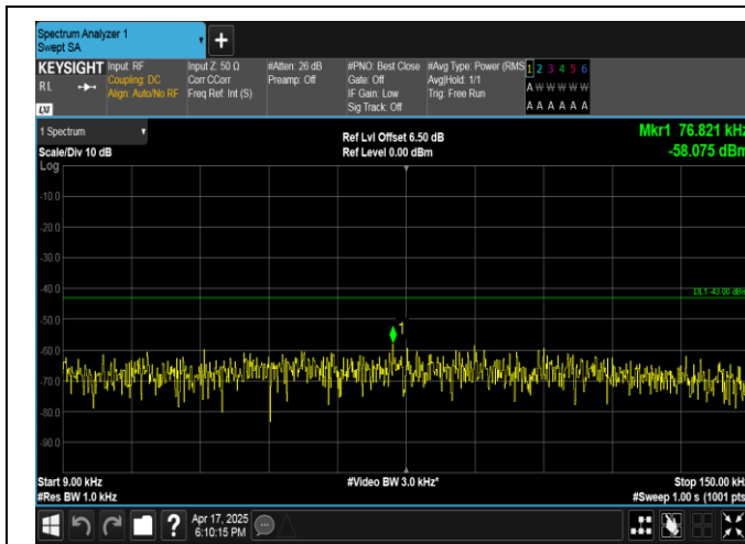
Band4-15MHz-QPSK-20325-1RB#0-0.009~0.15-PASS
