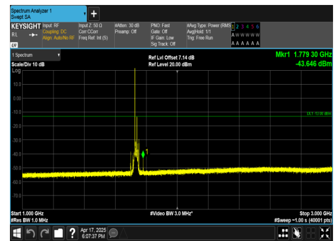
Band4-15MHz-16QAM-20175-1RB#0-1000~3000-PASS
