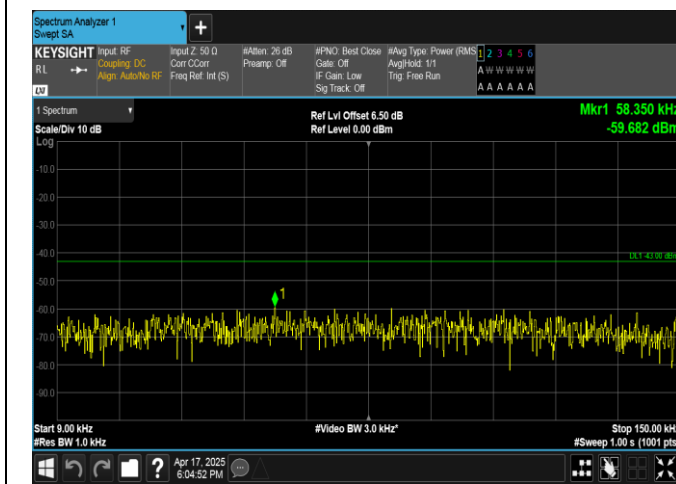
Band4-15MHz-16QAM-2025-1RB#74-0.009~0.15-PASS
