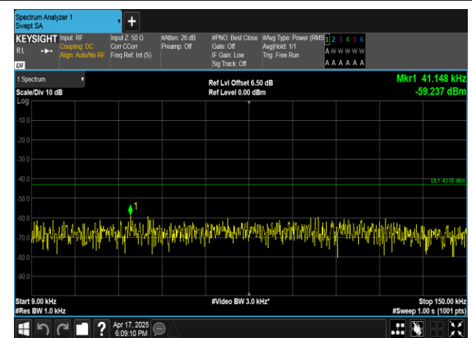
Band4-15MHz-16QAM-20175-1RB#74-0.009~0.15-PASS
