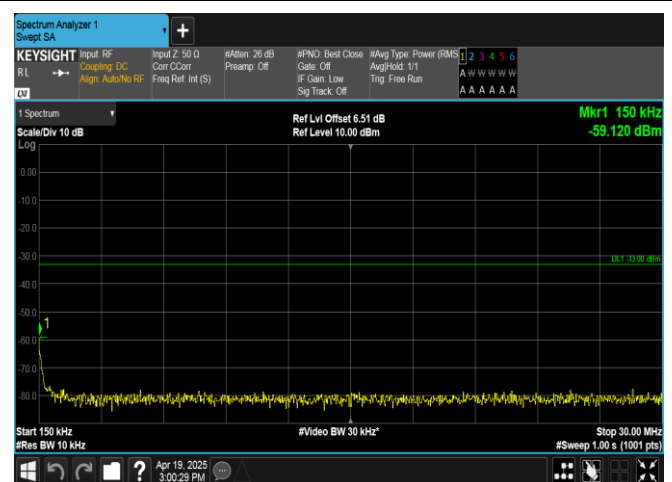
Band4-15MHz-QPSK-20025-75RB#0-0.15~30-PASS
