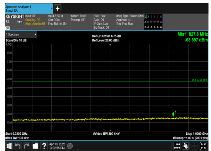
Band4-15MHz-QPSK-20175-75RB#0-30~1000-PASS
