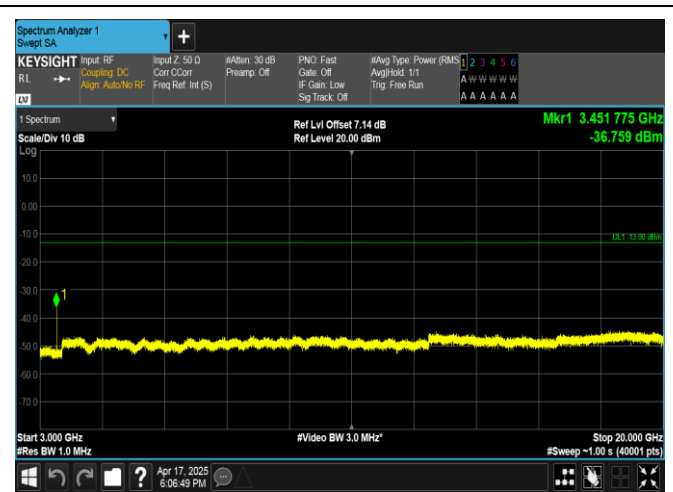
Band4-15MHz-QPSK-20175-1RB#0-3000~20000-PASS
