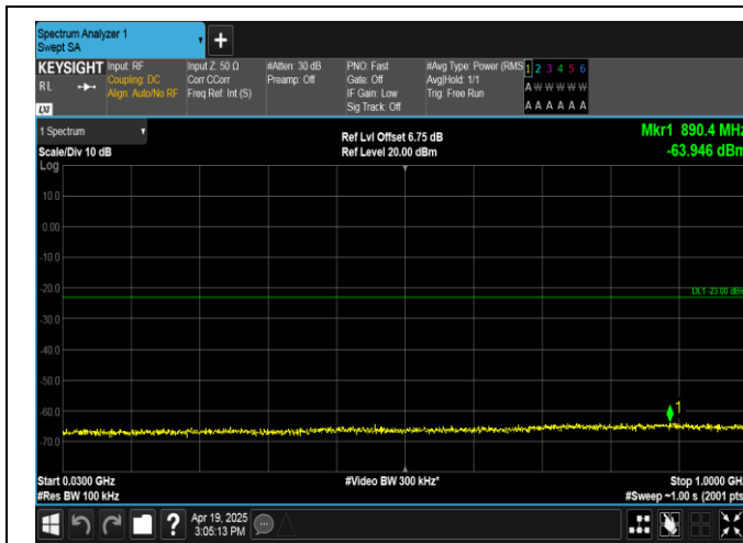
Band4-15MHz-QPSK-20325-75RB#0-30~1000-PASS
