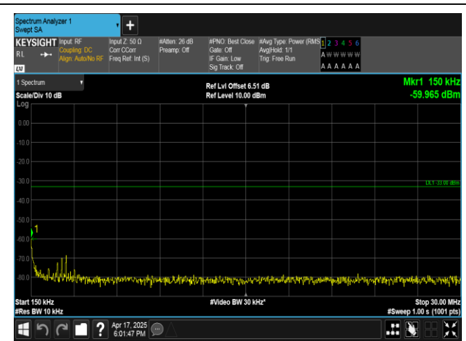
Band4-15MHz-QPSK-2025-1RB#0-0.15~30-PASS
