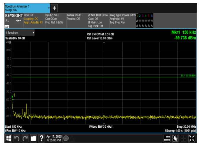
Band4-15MHz-16QAM-2025-1RB#74-0.15~30-PASS
