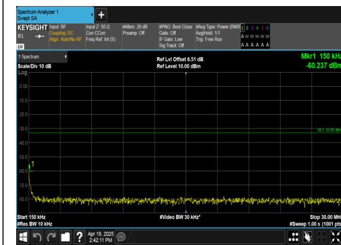
Band4-10MHz-QPSK-20175-50RB#0-0.15~30-PASS
