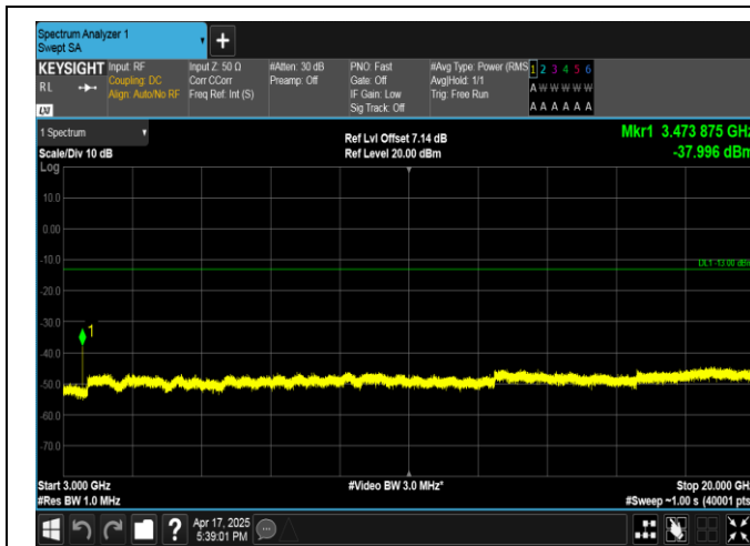
Band4-10MHz-QPSK-20175-1RB#49-3000~20000-PASS
