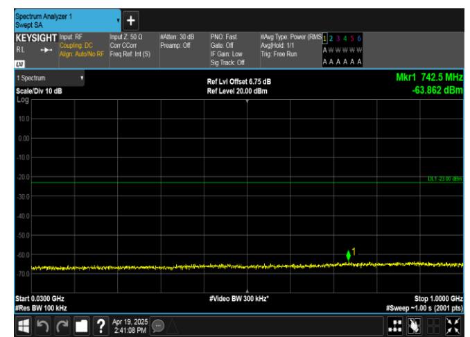
Band4-10MHz-16QAM-20000-50RB#0-30~1000-PASS
