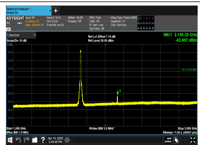
Band4-10MHz-16QAM-20175-50RB#0-1000~3000-PASS
