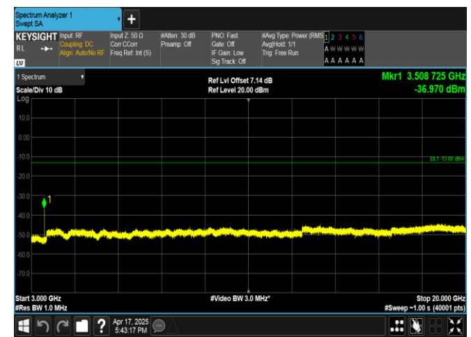
Band4-10MHz-QPSK-20350-1RB#49-3000~20000-PASS
