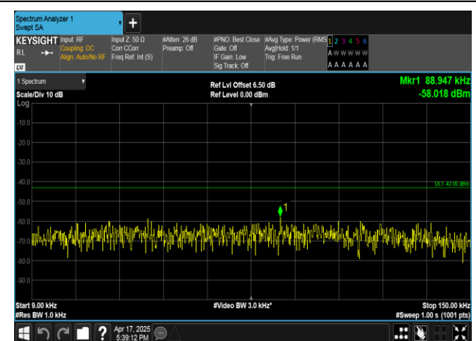
Band4-10MHz-16QAM-20175-1RB#49-0.009~0.15-PASS
