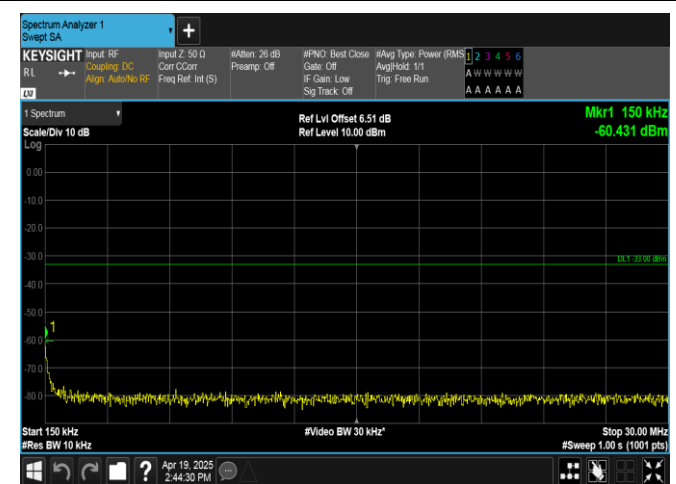
Band4-10MHz-QPSK-20350-50RB#0-0.15~30-PASS
