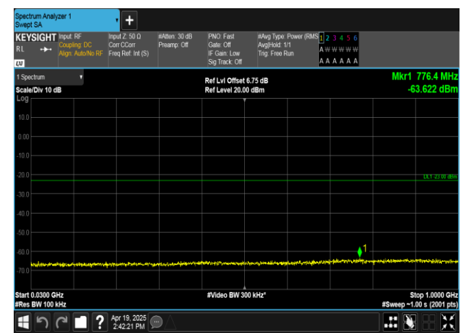
Band4-10MHz-QPSK-20175-50RB#0-30~1000-PASS
