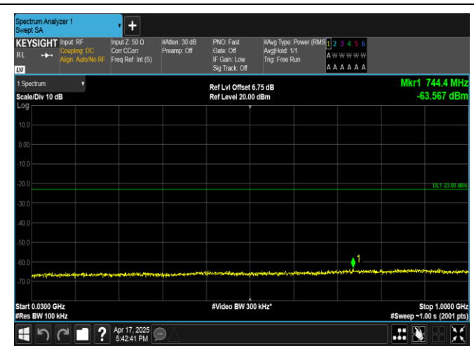
Band4-10MHz-QPSK-20350-1RB#49-30~1000-PASS
