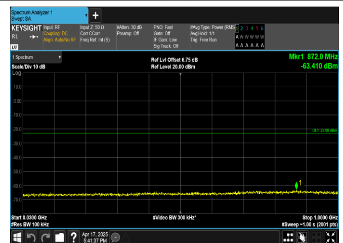
Band4-10MHz-16QAM-20350-1RB#0-30~1000-PASS
