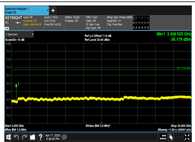
Band4-10MHz-QPSK-20175-1RB#0-3000~20000-PASS
