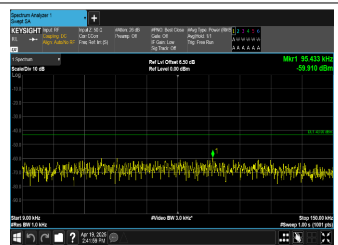
Band4-10MHz-QPSK-20175-50RB#0-0.009~0.15-PASS
