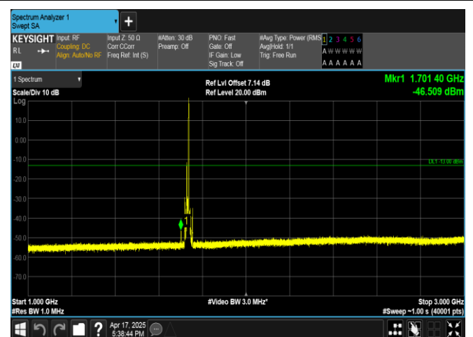
Band4-10MHz-QPSK-20175-1RB#49-1000~3000-PASS
