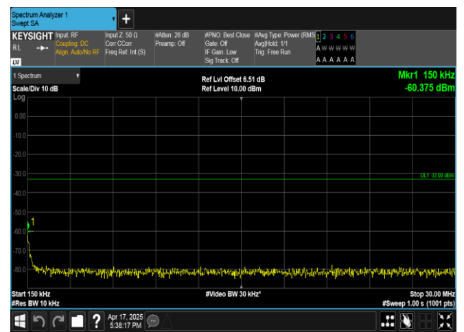
Band4-10MHz-QPSK-20175-1RB#49-0.15~30-PASS
