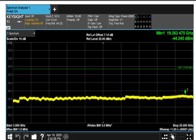
Band4-10MHz-QPSK-20175-50RB#0-3000~20000-PASS
