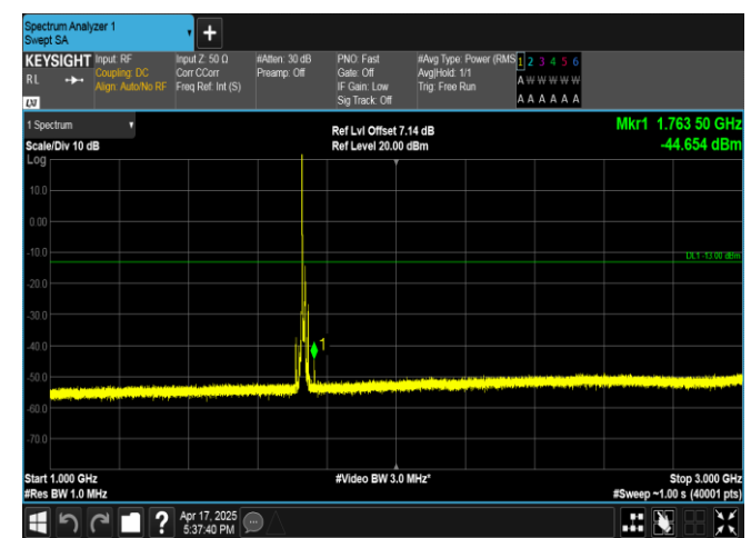
Band4-10MHz-16QAM-20175-1RB#0-1000~3000-PASS
