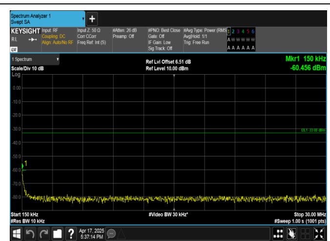
Band4-10MHz-16QAM-20175-1RB#0-0.15~30-PASS
