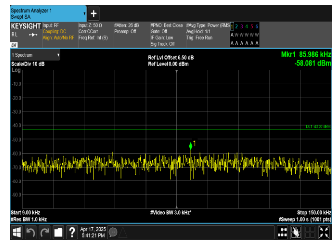
Band4-10MHz-16QAM-20350-1RB#0-0.009~0.15-PASS
