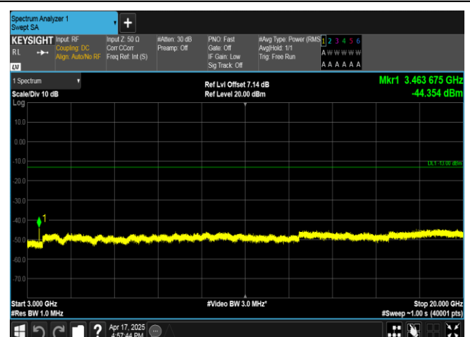
Band4-5MHz-QPSK-20175-25RB#0-3000~20000-PASS
