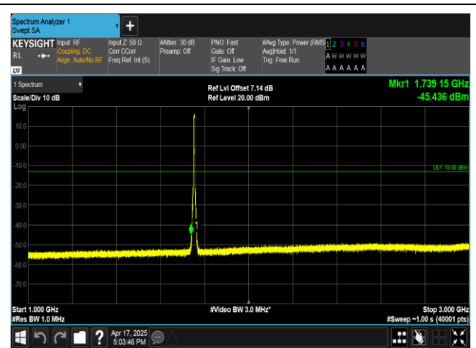
Band4-5MHz-QPSK-20375-25RB#0-1000~3000-PASS
