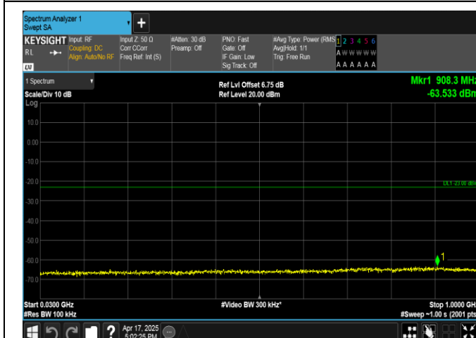
Band4-5MHz-16QAM-20375-1RB#24-30~1000-PASS
