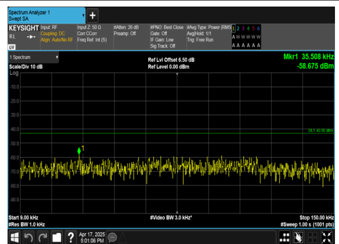
Band4-5MHz-QPSK-20375-1RB#24-0.009~0.15-PASS
