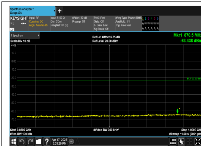
Band4-5MHz-QPSK-20375-25RB#0-30~1000-PASS
