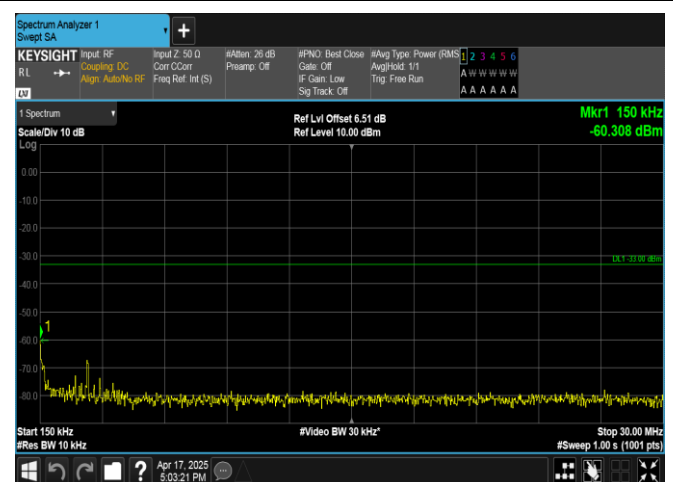
Band4-5MHz-QPSK-20375-25RB#0-0.15~30-PASS
