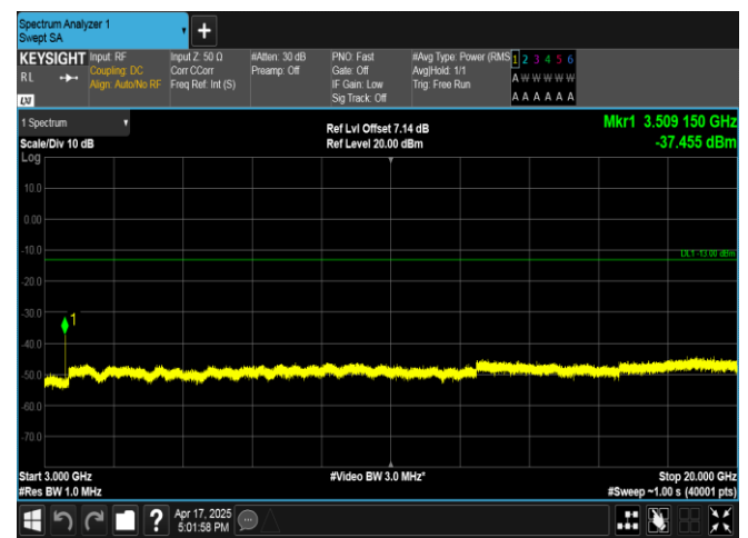
Band4-5MHz-QPSK-20375-1RB#24-3000~20000-PASS
