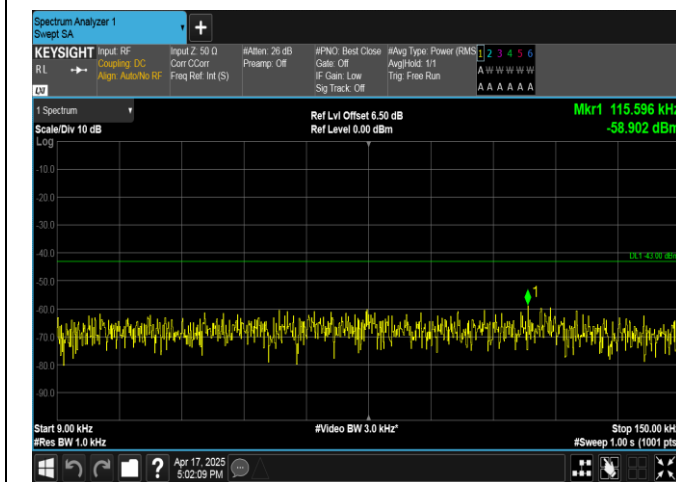
Band4-5MHz-16QAM-20375-1RB#24-0.009~0.15-PASS
