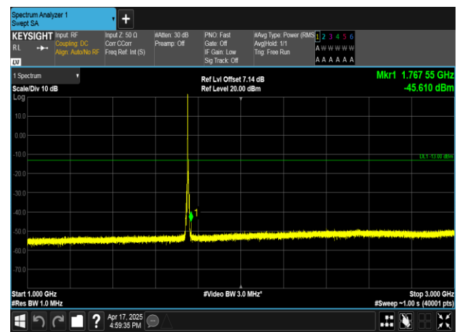
Band4-5MHz-QPSK-20375-1RB#0-1000~3000-PASS
