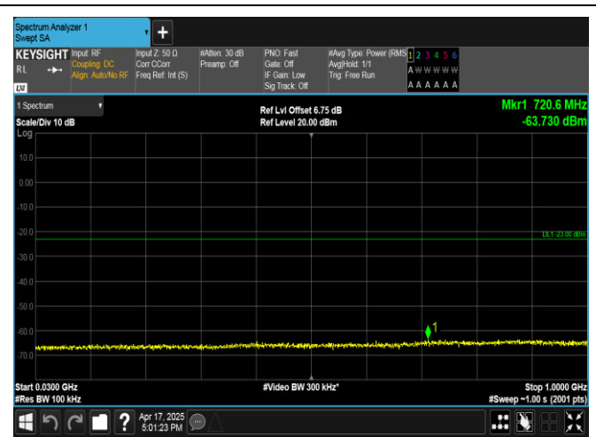
Band4-5MHz-QPSK-20375-1RB#24-30~1000-PASS
