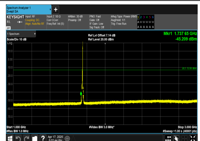
Band4-5MHz-16QAM-20375-1RB#24-1000~3000-PASS
