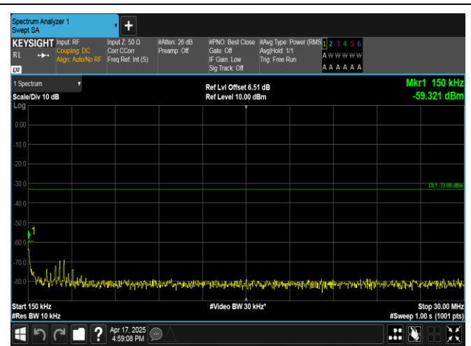
Band4-5MHz-QPSK-20375-1RB#0-0.15~30-PASS
