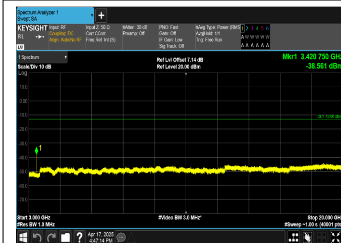
Band4-5MHz-QPSK-19975-1RB#0-3000~20000-PASS
