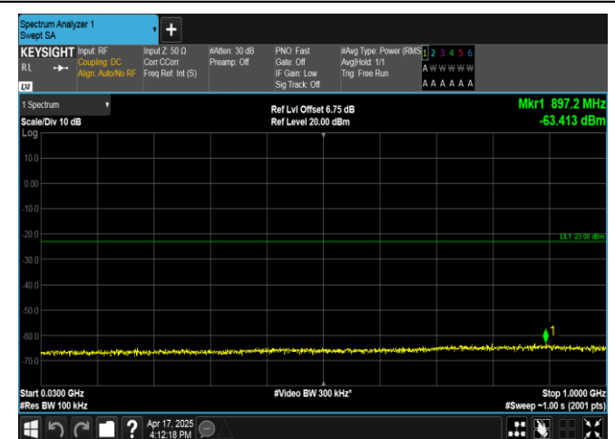
Band4-3MHz-16QAM-20385-1RB#0-30~1000-PASS
