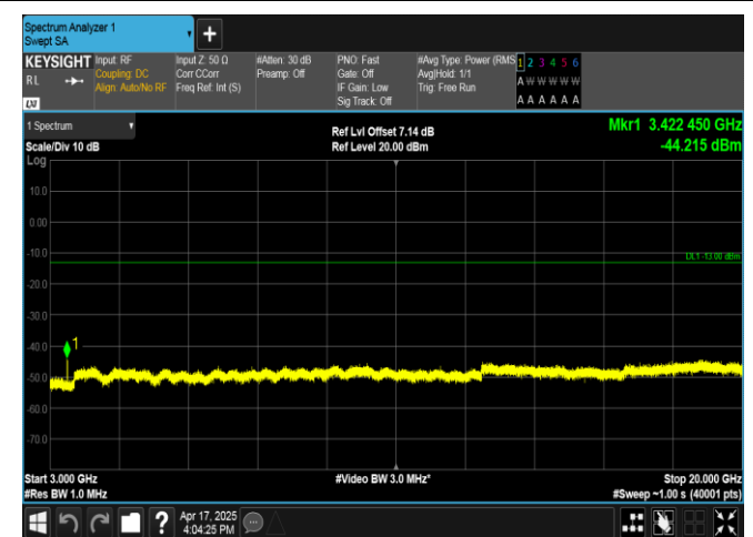
Band4-3MHz-16QAM-19965-15RB#0-3000~20000-PASS
