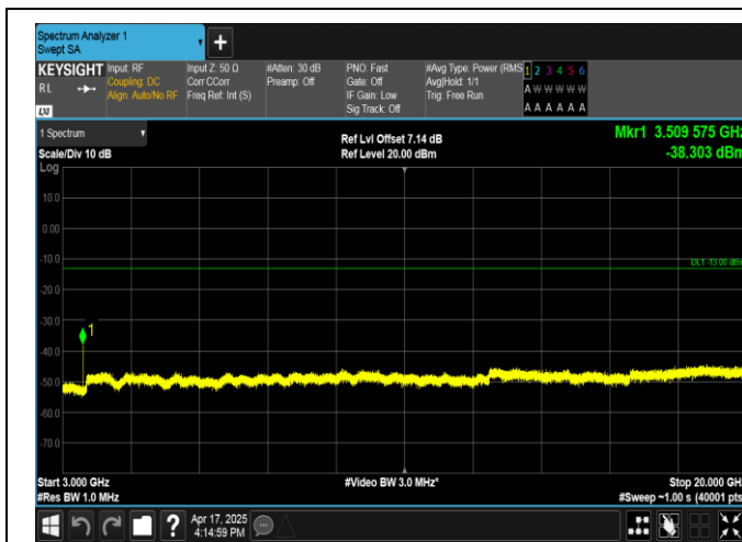
Band4-3MHz-16QAM-20385-1RB#14-3000~20000-PASS
