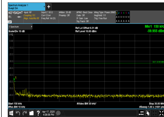
Band4-3MHz-QPSK-20175-15RB#0-0.15~30-PASS
