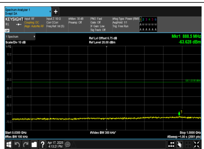
Band4-3MHz-QPSK-20385-1RB#14-30~1000-PASS
