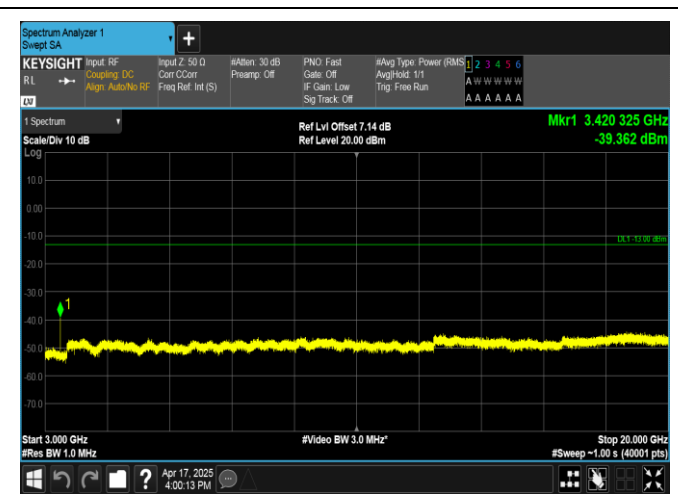
Band4-3MHz-16QAM-19965-1RB#0-3000~20000-PASS
