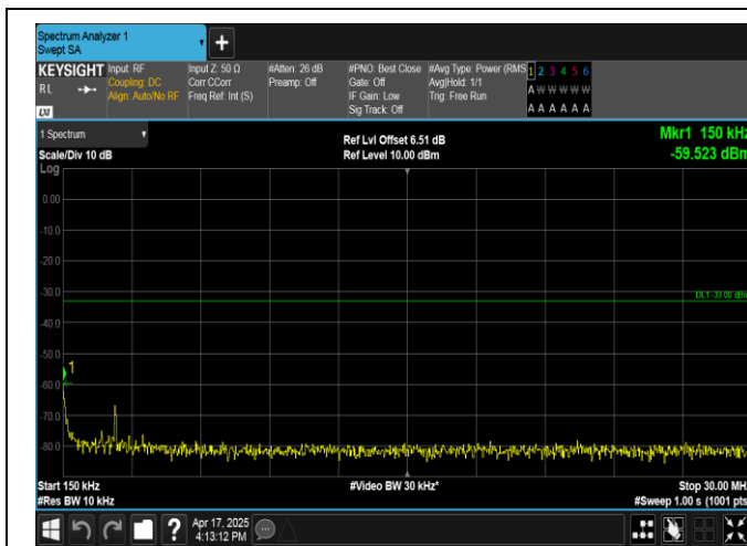
Band4-3MHz-QPSK-20385-1RB#14-0.15~30-PASS
