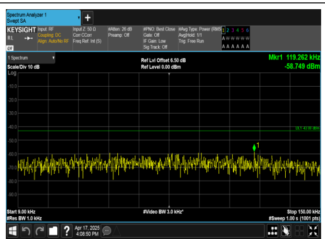
Band4-3MHz-QPSK-20175-15RB#0-0.009~0.15-PASS
