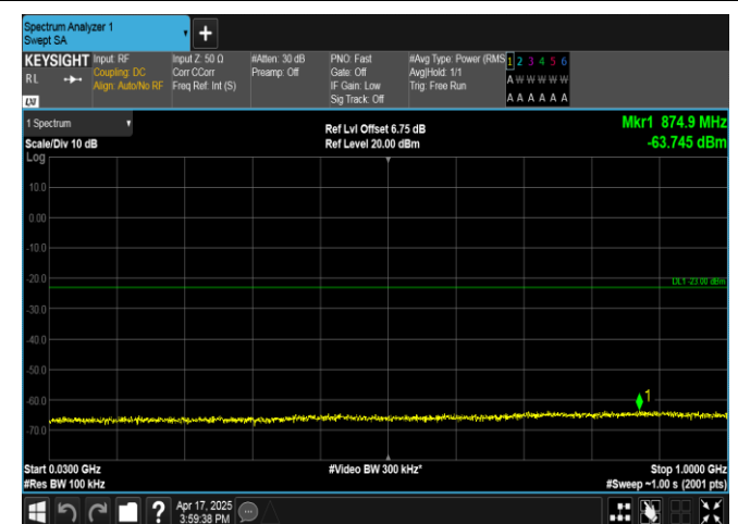
Band4-3MHz-16QAM-19965-1RB#0-30~1000-PASS
