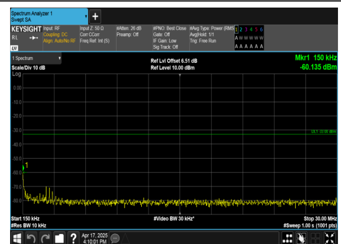
Band4-3MHz-16QAM-20175-15RB#0-0.15~30-PASS
