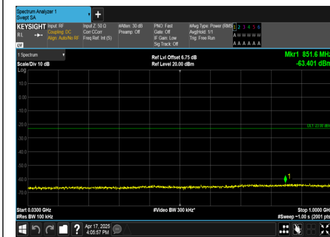
Band4-3MHz-16QAM-20175-1RB#0-30~1000-PASS
