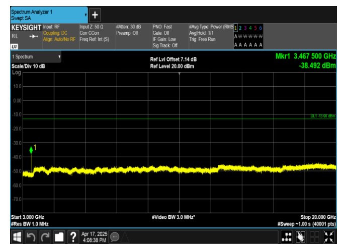
Band4-3MHz-16QAM-20175-1RB#14-3000~20000-PASS
