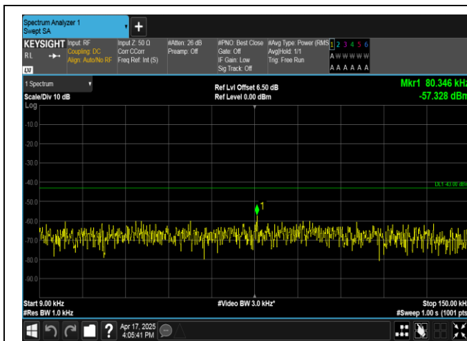
Band4-3MHz-16QAM-20175-1RB#0-0.009~0.15-PASS
