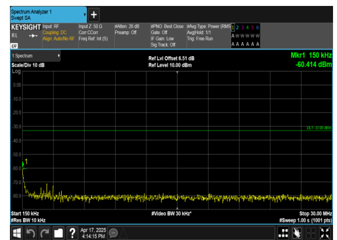
Band4-3MHz-16QAM-20385-1RB#14-0.15~30-PASS
