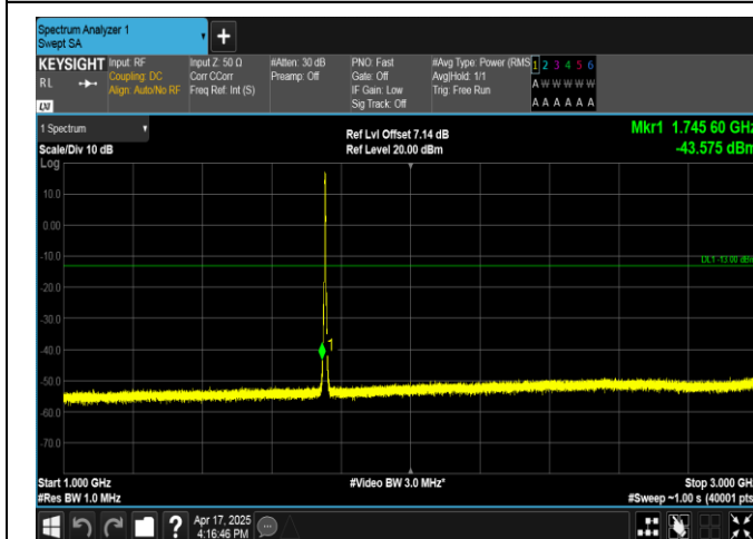
Band4-3MHz-16QAM-20385-15RB#0-1000~3000-PASS
