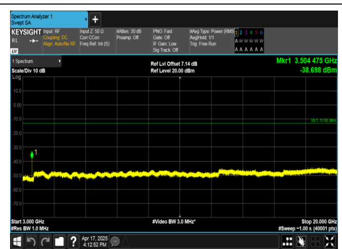
Band4-3MHz-16QAM-20385-1RB#0-3000~20000-PASS
