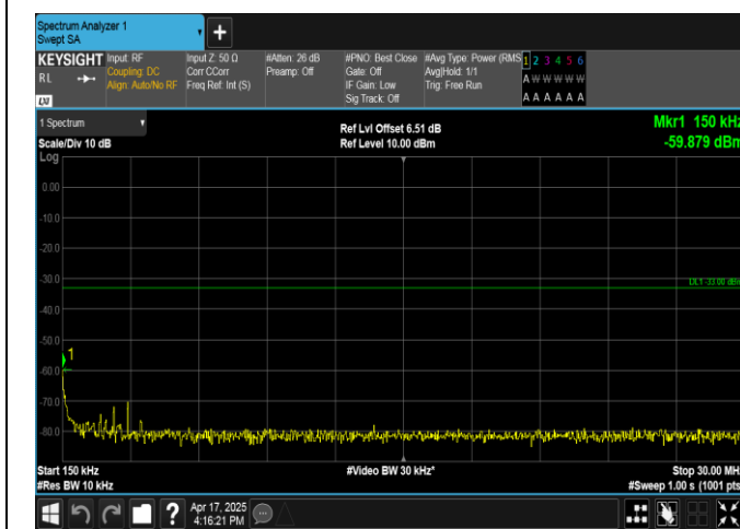
Band4-3MHz-16QAM-20385-15RB#0-0.15~30-PASS
