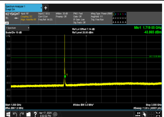
Band4-3MHz-16QAM-19965-1RB#14-1000~3000-PASS
