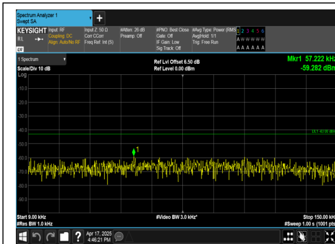
Band4-5MHz-QPSK-19975-1RB#0-0.009~0.15-PASS
