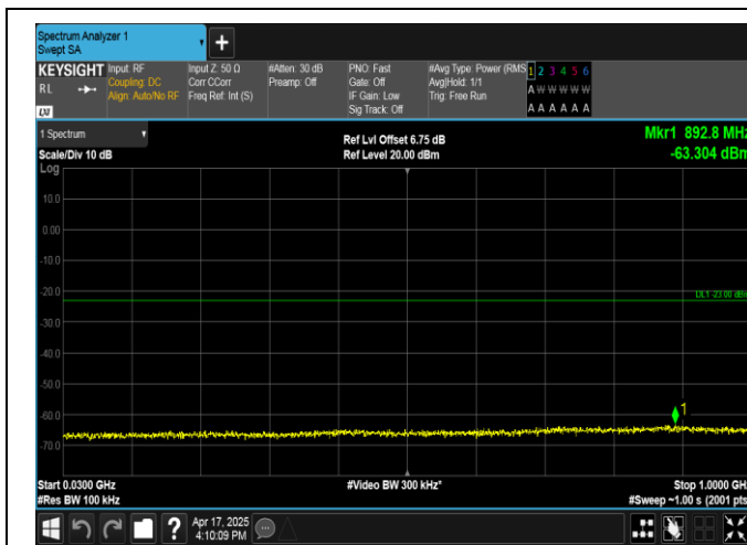
Band4-3MHz-16QAM-20175-15RB#0-30~1000-PASS
