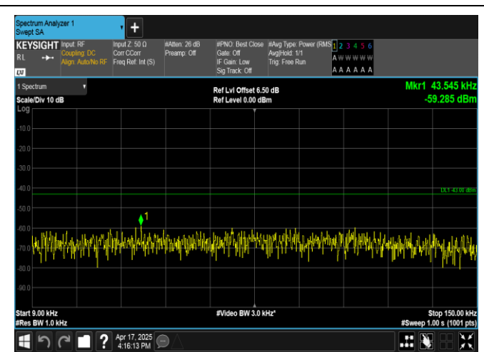
Band4-3MHz-16QAM-20385-15RB#0-0.009~0.15-PASS
