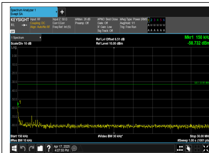
Band4-3MHz-16QAM-20175-1RB#14-0.15~30-PASS
