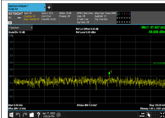
Band4-5MHz-QPSK-19975-25RB#0-0.009~0.15-PASS
