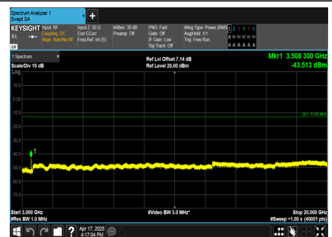
Band4-3MHz-16QAM-20385-15RB#0-3000~20000-PASS
