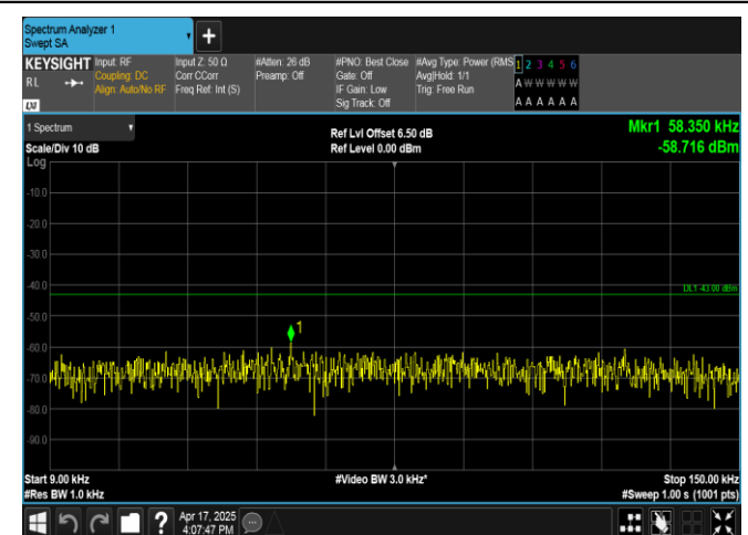
Band4-3MHz-16QAM-20175-1RB#14-0.009~0.15-PASS
