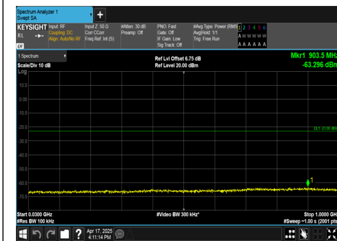
Band4-3MHz-QPSK-20385-1RB#0-30~1000-PASS
