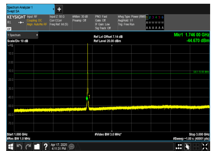
Band4-3MHz-QPSK-20385-1RB#0-1000~3000-PASS
