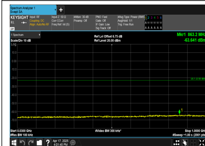
Band4-3MHz-16QAM-19965-1RB#14-30~1000-PASS
