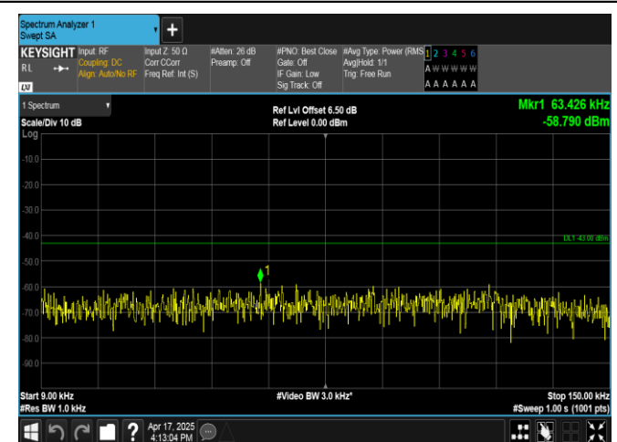
Band4-3MHz-QPSK-20385-1RB#14-0.009~0.15-PASS
