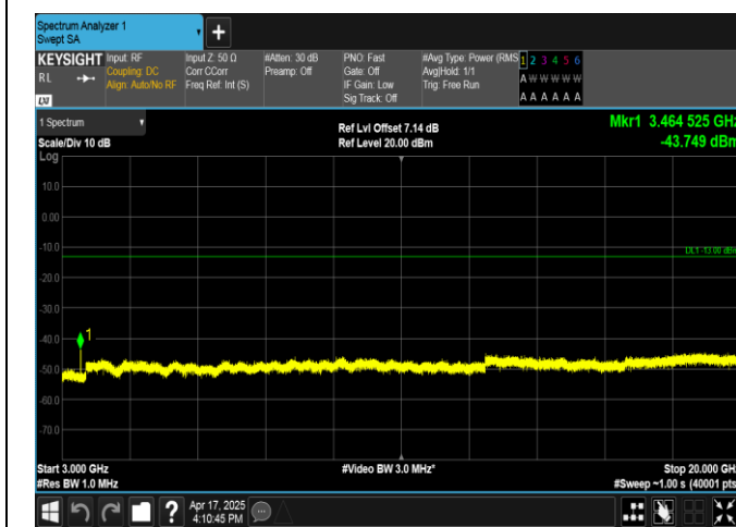
Band4-3MHz-16QAM-20175-15RB#0-3000~20000-PASS
