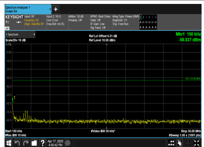
Band4-5MHz-QPSK-19975-25RB#0-0.15~30-PASS
