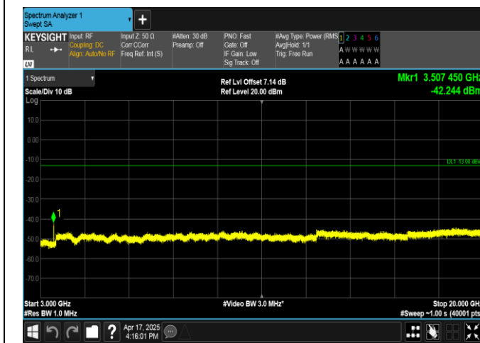
Band4-3MHz-QPSK-20385-15RB#0-3000~20000-PASS
