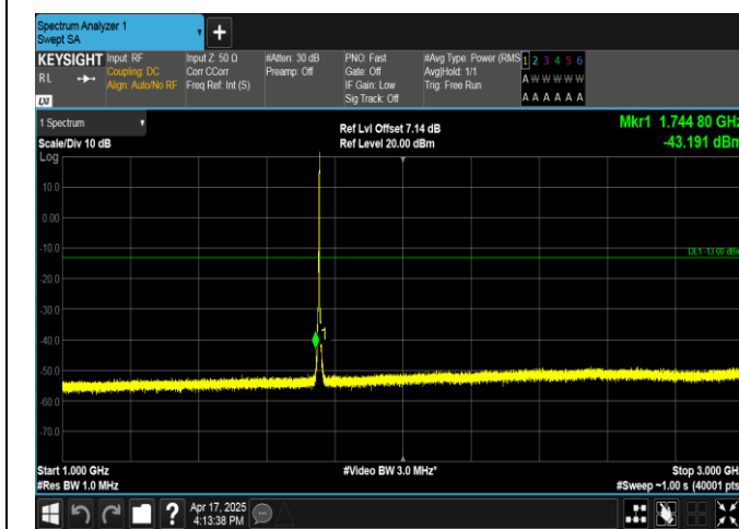
Band4-3MHz-QPSK-20385-1RB#14-1000~3000-PASS
