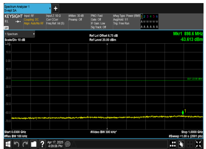
Band4-3MHz-QPSK-20175-15RB#0-30~1000-PASS
