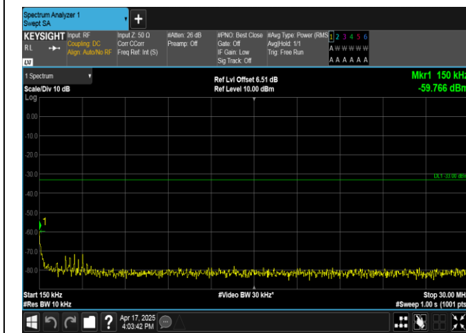
Band4-3MHz-16QAM-19965-15RB#0-0.15~30-PASS
