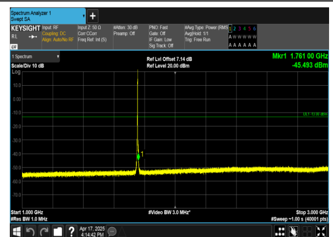
Band4-3MHz-16QAM-20385-1RB#14-1000~3000-PASS
