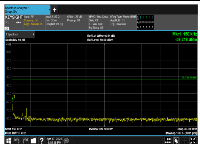
Band4-3MHz-QPSK-20385-15RB#0-0.15~30-PASS
