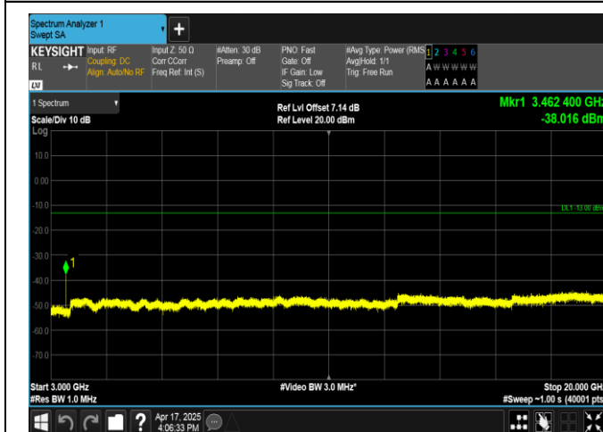
Band4-3MHz-16QAM-20175-1RB#0-3000~20000-PASS
