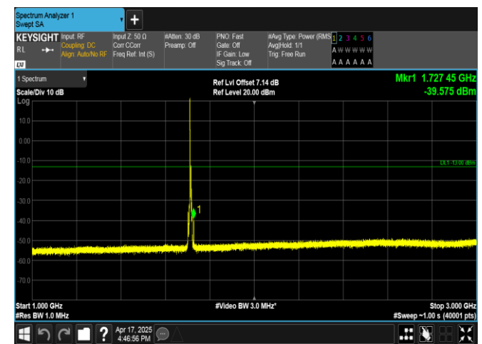
Band4-5MHz-QPSK-19975-1RB#0-1000~3000-PASS
