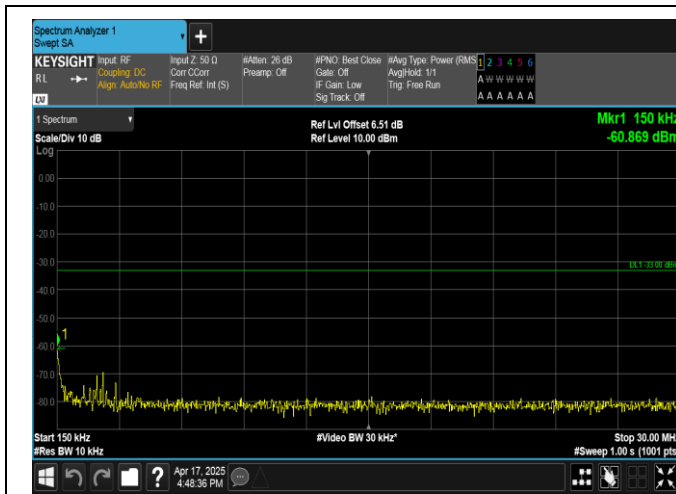
Band4-5MHz-QPSK-19975-1RB#24-0.15~30-PASS
