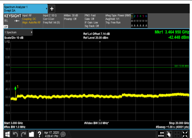
Band4-3MHz-QPSK-20175-15RB#0-3000~20000-PASS
