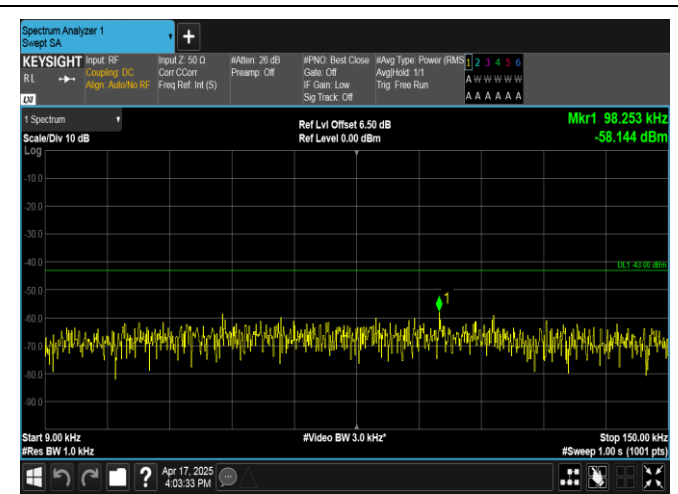
Band4-3MHz-16QAM-19965-15RB#0-0.009~0.15-PASS
