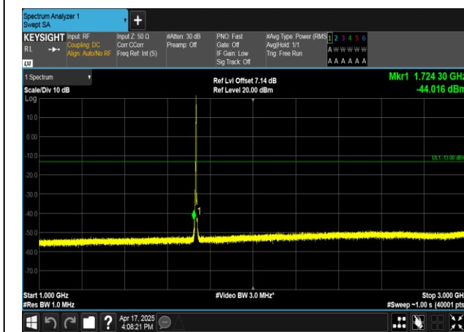
Band4-3MHz-16QAM-20175-1RB#14-1000~3000-PASS
