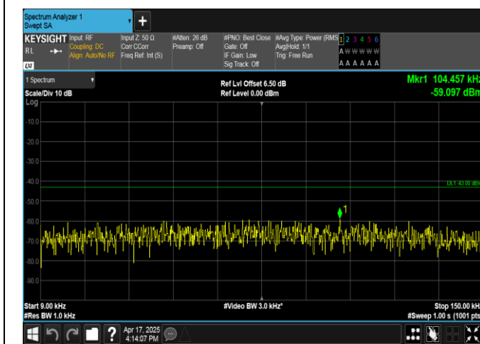
Band4-3MHz-16QAM-20385-1RB#14-0.009~0.15-PASS
