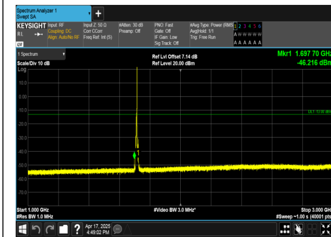
Band4-5MHz-QPSK-19975-1RB#24-1000~3000-PASS
