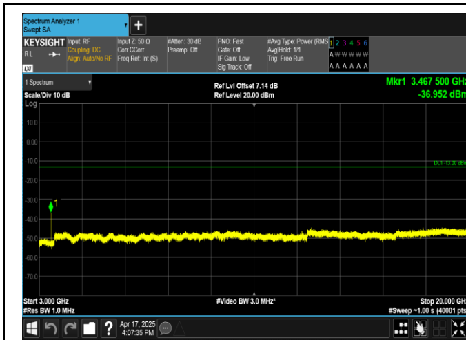
Band4-3MHz-QPSK-20175-1RB#14-3000~20000-PASS
