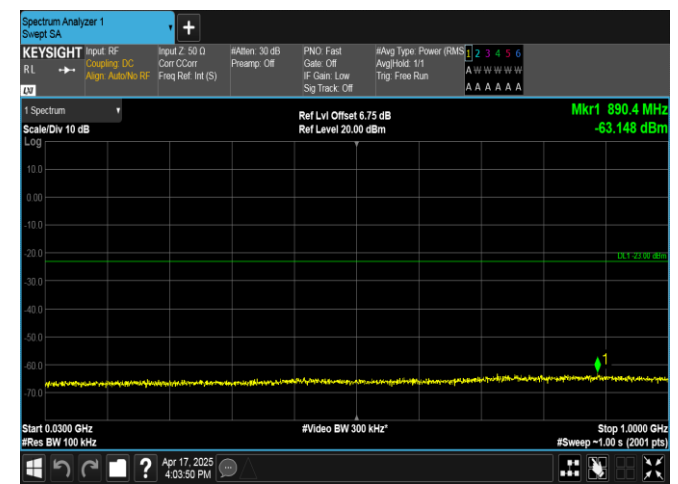
Band4-3MHz-16QAM-19965-15RB#0-30~1000-PASS
