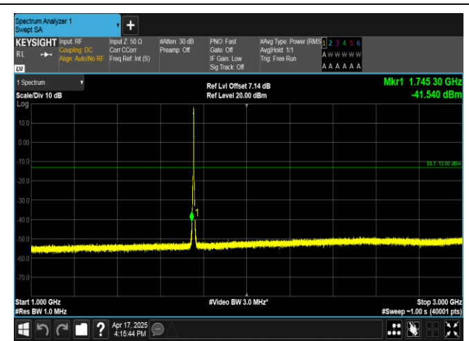
Band4-3MHz-QPSK-20385-15RB#0-1000~3000-PASS
