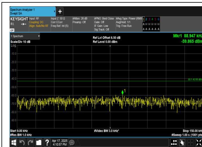
Band4-3MHz-QPSK-20385-1RB#0-0.009~0.15-PASS
