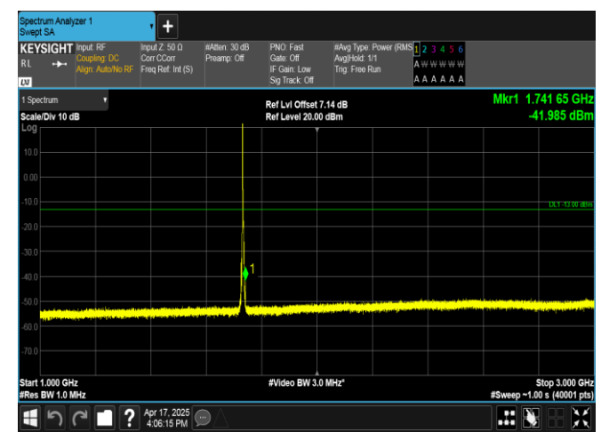
Band4-3MHz-16QAM-20175-1RB#0-1000~3000-PASS
