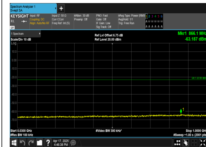
Band4-5MHz-QPSK-19975-1RB#0-30~1000-PASS
