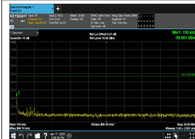
Band4-3MHz-16QAM-19965-1RB#0-0.15~30-PASS
