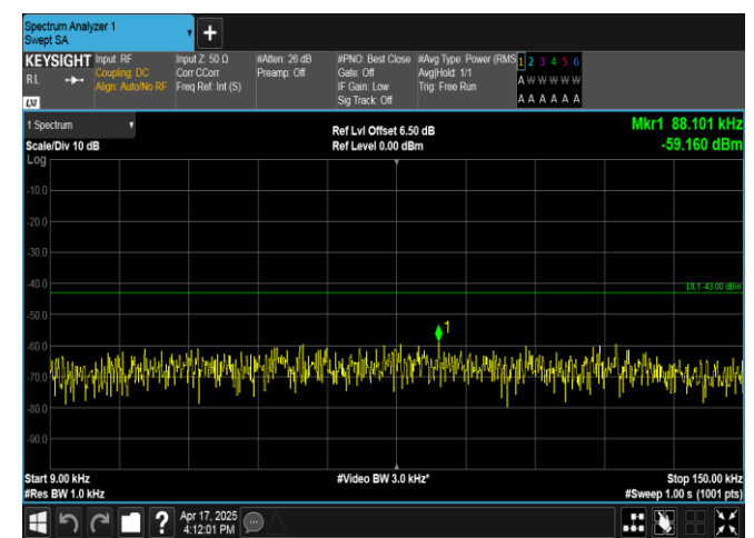
Band4-3MHz-16QAM-20385-1RB#0-0.009~0.15-PASS
