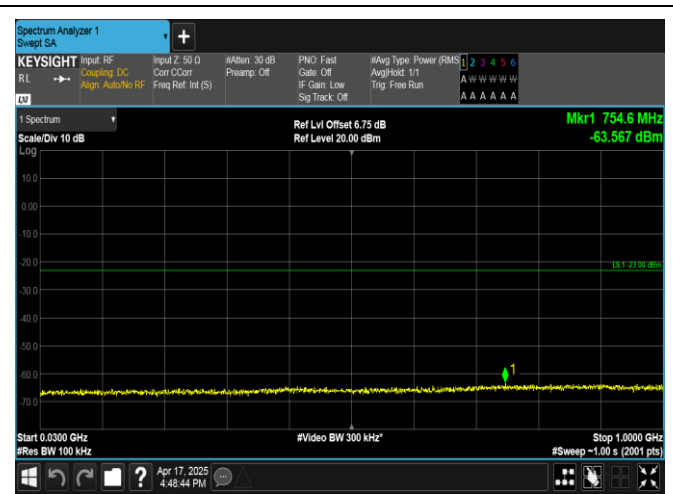
Band4-5MHz-QPSK-19975-1RB#24-30~1000-PASS
