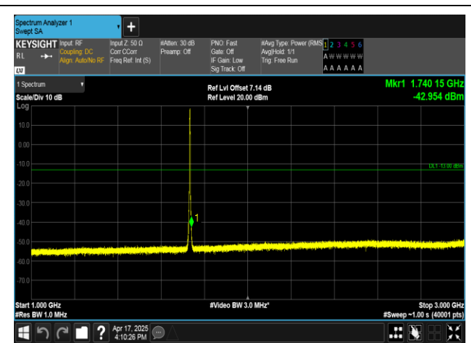
Band4-3MHz-16QAM-20175-15RB#0-1000~3000-PASS
