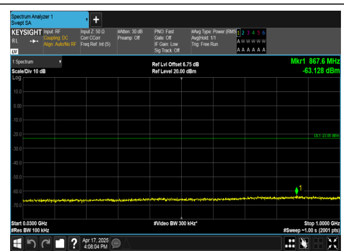
Band4-3MHz-16QAM-20175-1RB#14-30~1000-PASS
