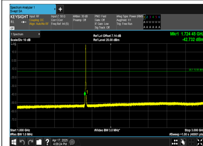
Band4-3MHz-QPSK-20175-15RB#0-1000~3000-PASS
