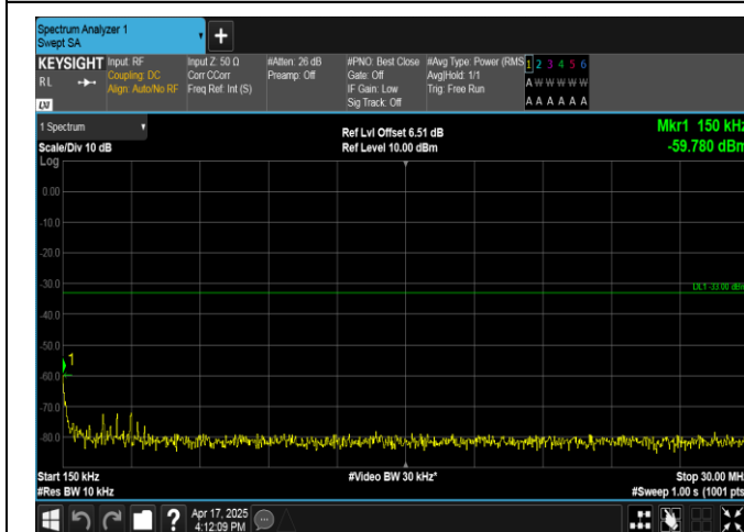
Band4-3MHz-16QAM-20385-1RB#0-0.15~30-PASS
