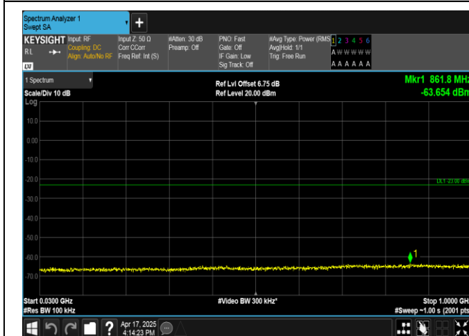
Band4-3MHz-16QAM-20385-1RB#14-30~1000-PASS
