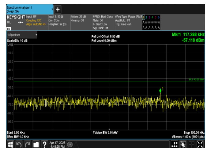
Band4-5MHz-QPSK-19975-1RB#24-0.009~0.15-PASS
