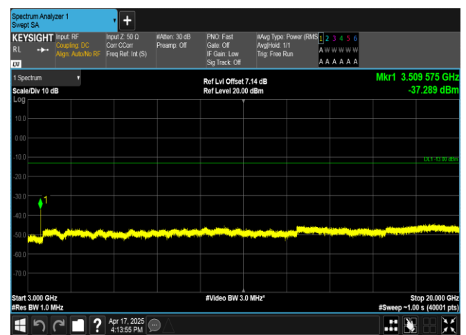
Band4-3MHz-QPSK-20385-1RB#14-3000~20000-PASS
