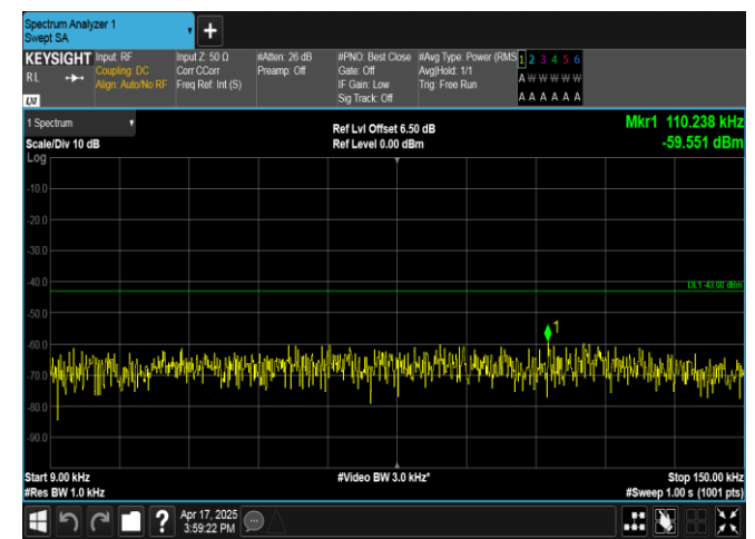
Band4-3MHz-16QAM-19965-1RB#0-0.009~0.15-PASS
