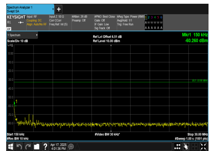
Band4-3MHz-16QAM-19965-1RB#14-0.15~30-PASS
