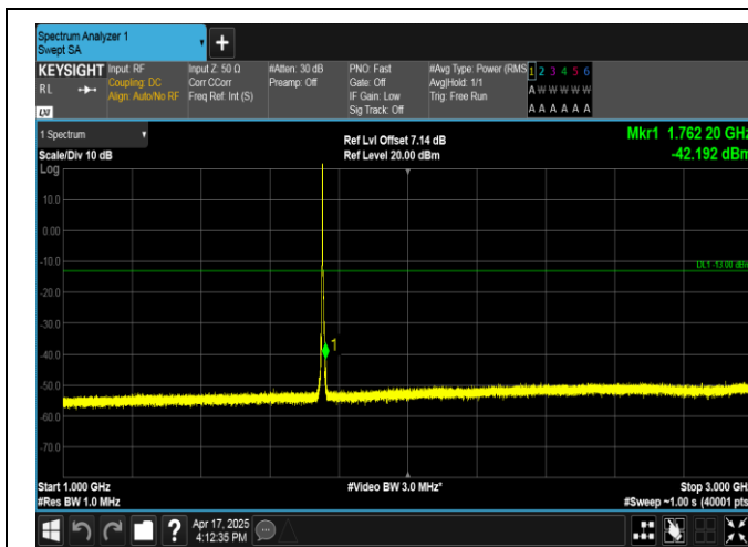
Band4-3MHz-16QAM-20385-1RB#0-1000~3000-PASS
