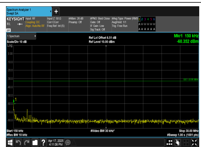
Band4-3MHz-QPSK-20385-1RB#0-0.15~30-PASS
