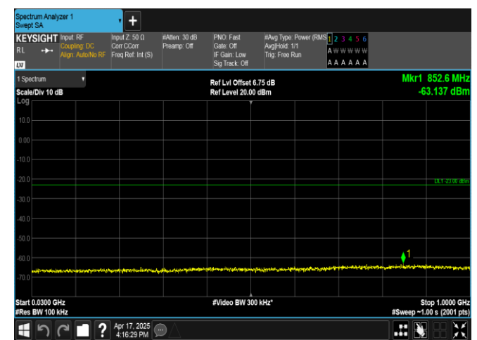
Band4-3MHz-16QAM-20385-15RB#0-30~1000-PASS
