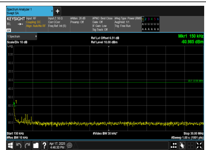
Band4-5MHz-QPSK-19975-1RB#0-0.15~30-PASS
