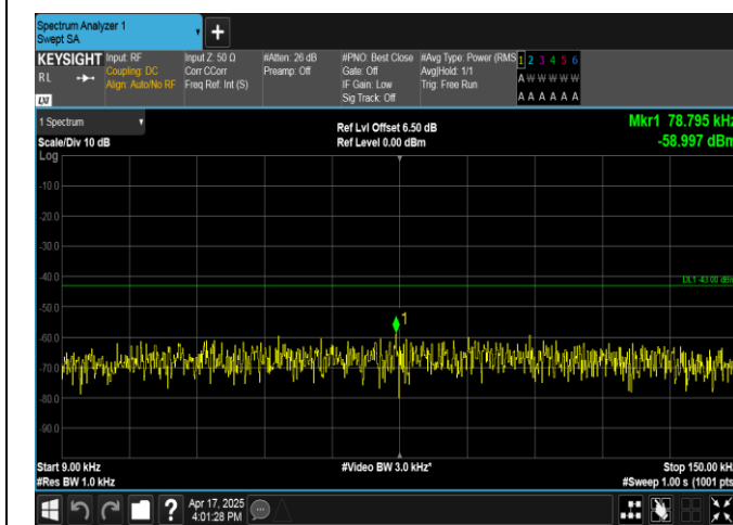
Band4-3MHz-16QAM-19965-1RB#14-0.009~0.15-PASS
