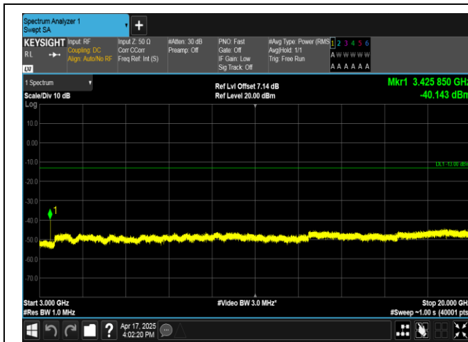
Band4-3MHz-16QAM-19965-1RB#14-3000~20000-PASS
