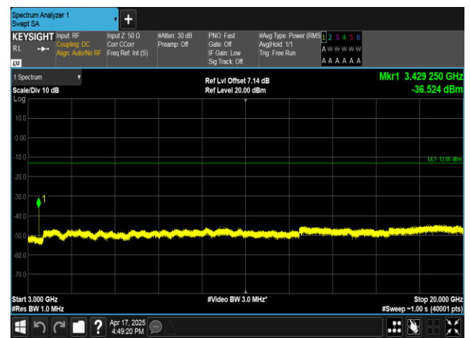
Band4-5MHz-QPSK-19975-1RB#24-3000~20000-PASS
