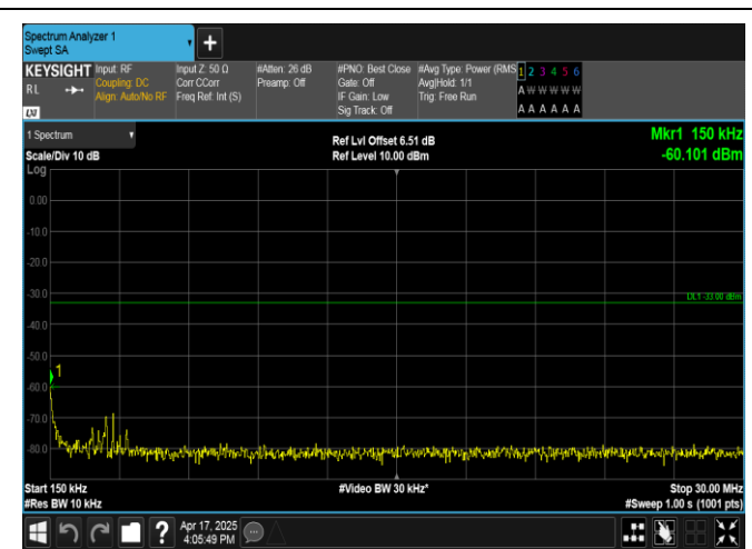
Band4-3MHz-16QAM-20175-1RB#0-0.15~30-PASS
