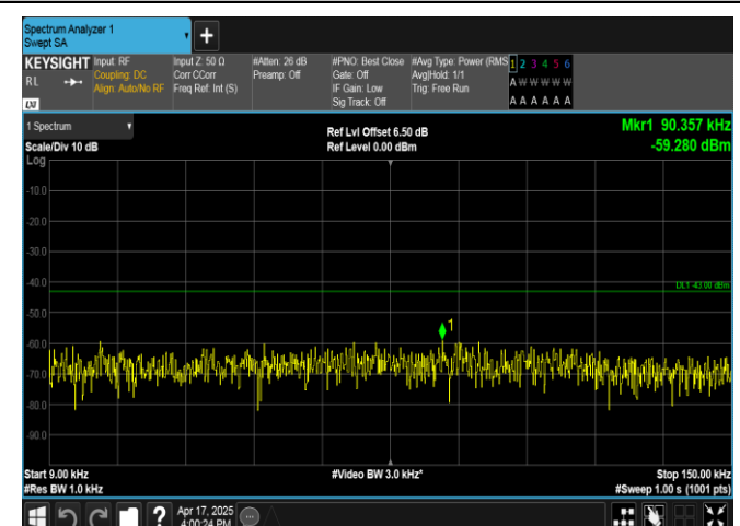
Band4-3MHz-QPSK-19965-1RB#14-0.009~0.15-PASS
