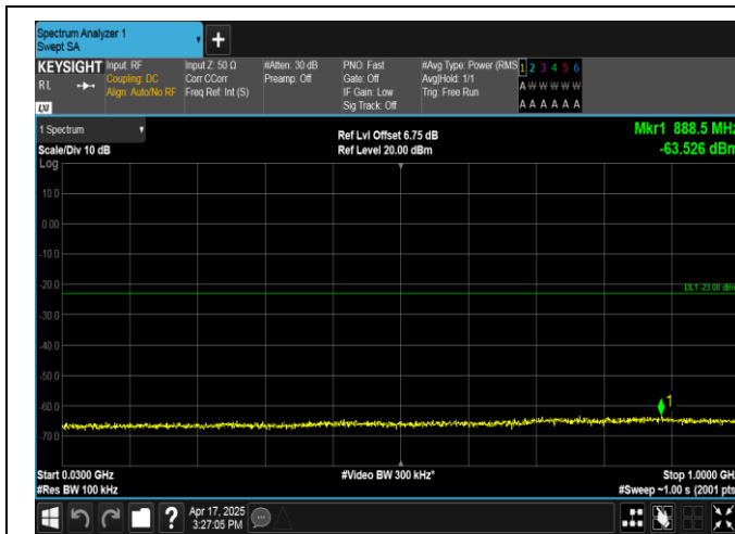
Band4-1.4MHz-QPSK-20393-6RB#0-30~1000-PASS
