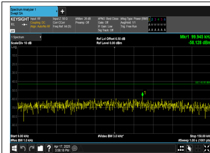
Band4-3MHz-QPSK-19965-1RB#0-0.009~0.15-PASS
