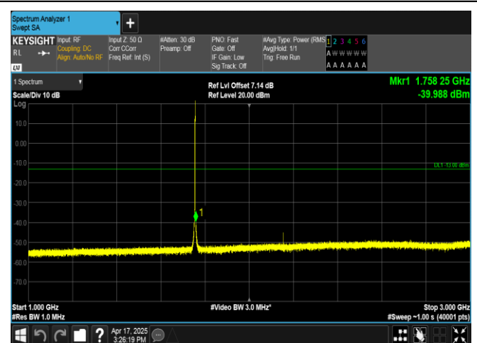
Band4-1.4MHz-16QAM-20393-1RB#5-1000~3000-PASS
