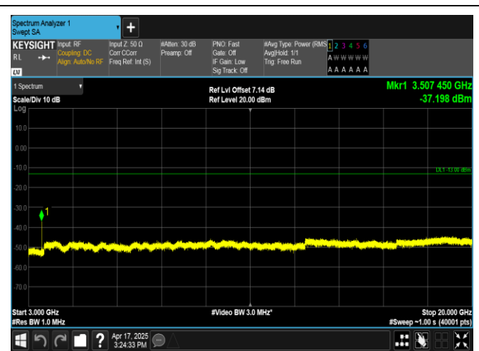
Band4-1.4MHz-16QAM-20393-1RB#0-3000~20000-PASS
