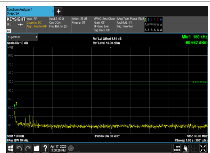
Band4-3MHz-QPSK-19965-1RB#0-0.15~30-PASS
