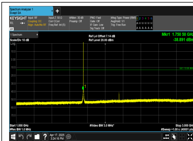
Band4-1.4MHz-16QAM-20393-1RB#0-1000~3000-PASS
