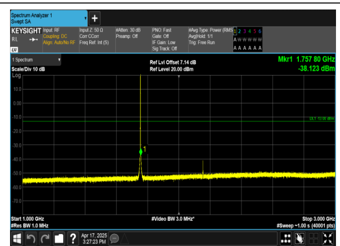
Band4-1.4MHz-QPSK-20393-6RB#0-1000~3000-PASS
