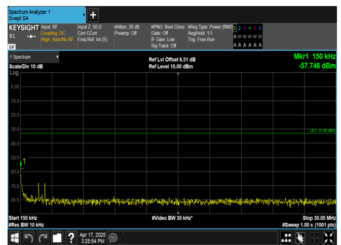
Band4-1.4MHz-16QAM-20393-1RB#5-0.15~30-PASS
