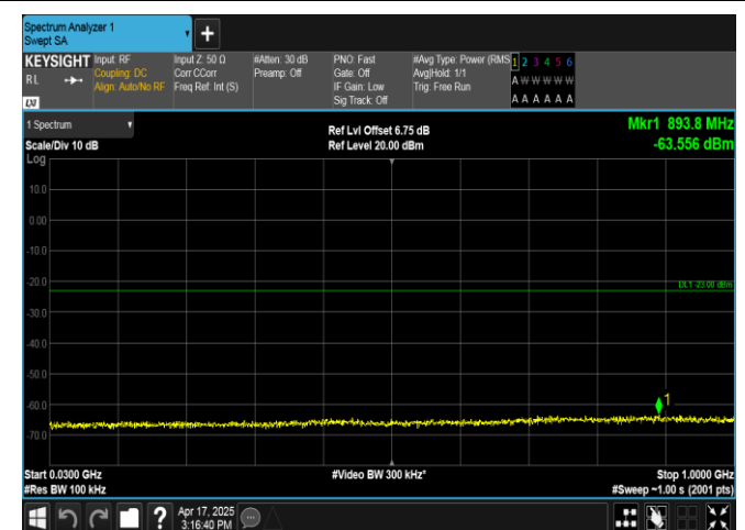
Band4-1.4MHz-QPSK-20175-1RB#0-30~1000-PASS
