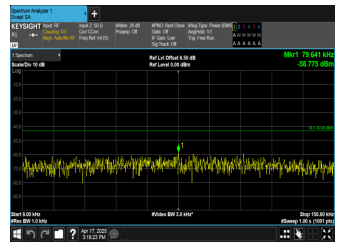
Band4-1.4MHz-QPSK-20175-1RB#0-0.009~0.15-PASS
