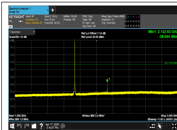
Band4-1.4MHz-QPSK-20175-1RB#0-1000~3000-PASS
