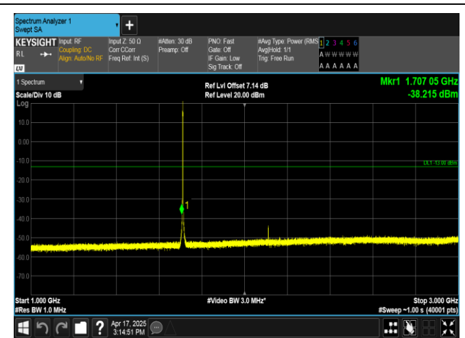
Band4-1.4MHz-QPSK-19957-6RB#0-1000~3000-PASS
