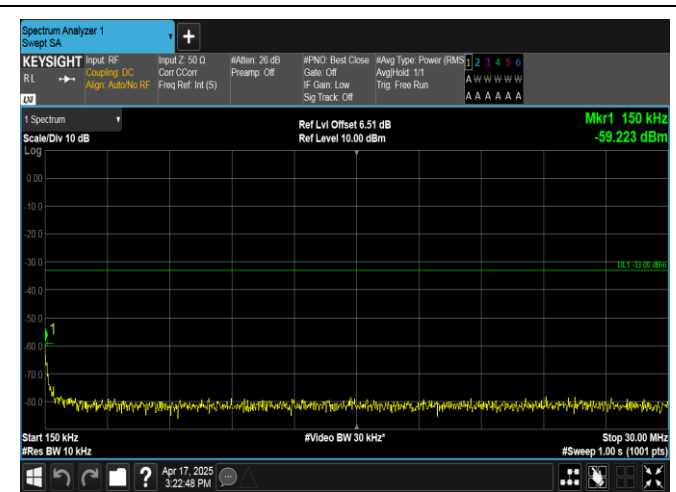
Band4-1.4MHz-QPSK-20393-1RB#0-0.15~30-PASS
