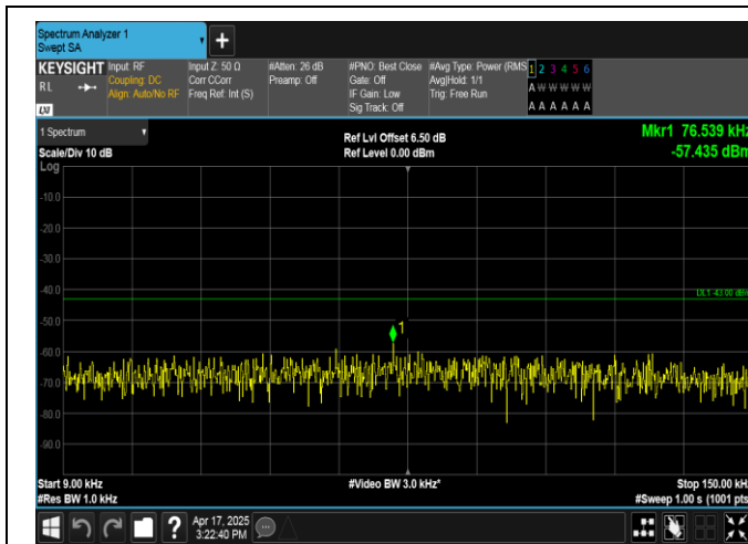
Band4-1.4MHz-QPSK-20393-1RB#0-0.009~0.15-PASS
