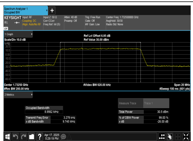
Band4-10MHz-QPSK-20175-50RB#0-PASS
