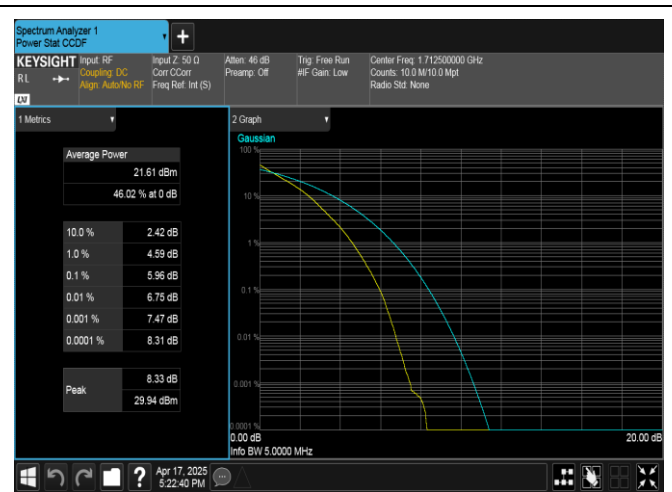
Band4-5MHz-QPSK-19975-25RB#0-PASS
