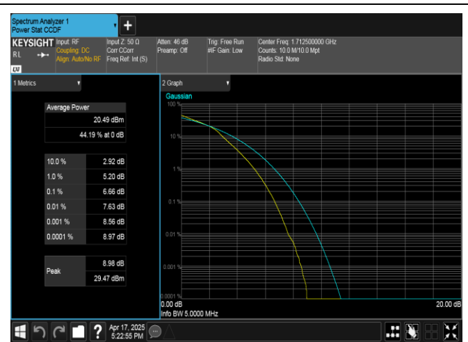
Band4-5MHz-16QAM-19975-25RB#0-PASS
