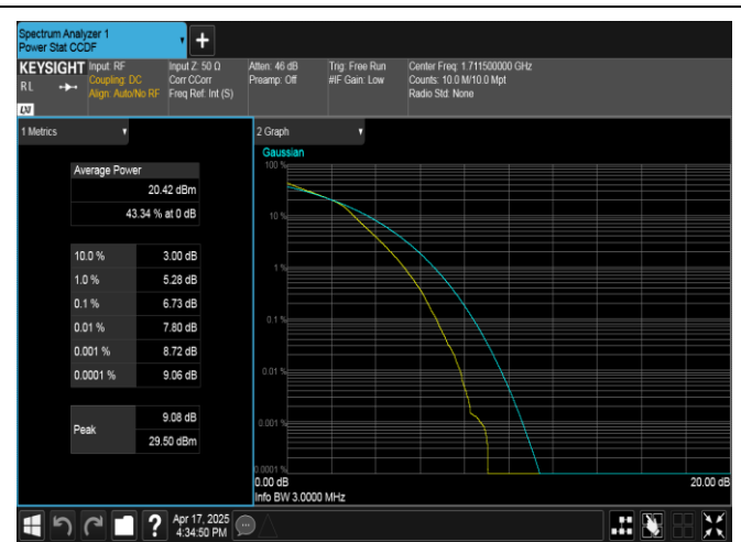
Band4-3MHz-16QAM-19965-15RB#0-PASS
