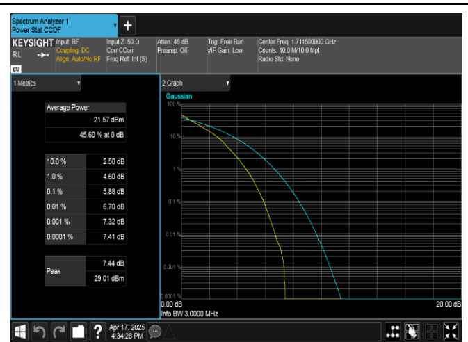
Band4-3MHz-QPSK-19965-15RB#0-PASS
