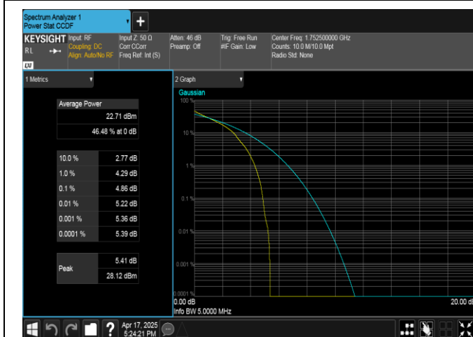
Band4-5MHz-QPSK-20375-1RB#0-PASS
