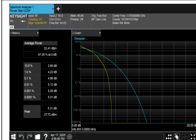
Band4-3MHz-QPSK-20385-1RB#0-PASS
