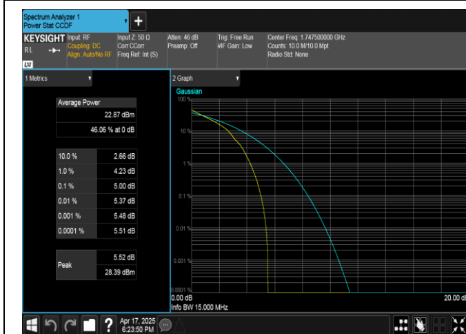
Band4-15MHz-QPSK-20325-1RB#0-PASS
