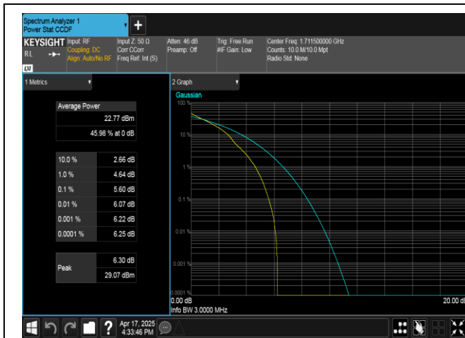
Band4-3MHz-QPSK-19965-1RB#0-PASS
