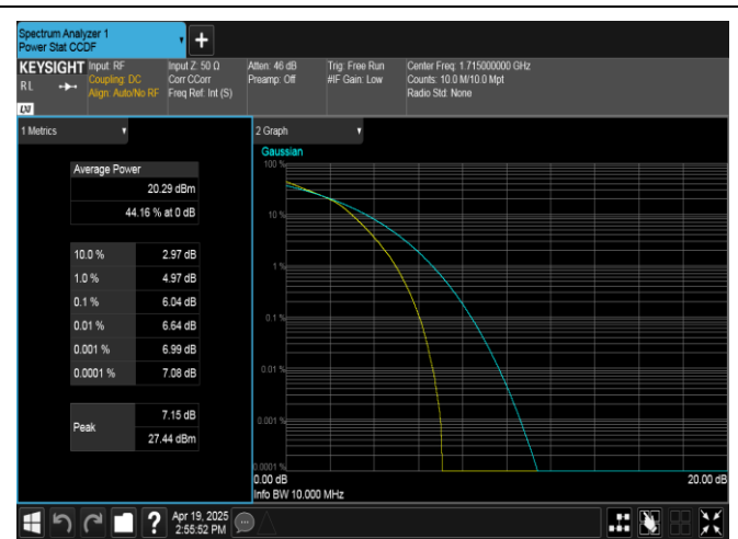
Band4-10MHz-16QAM-20000-50RB#0-PASS
