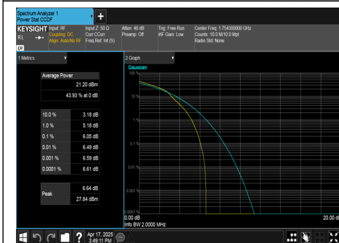
Band4-1.4MHz-16QAM-20393-1RB#0-PASS
