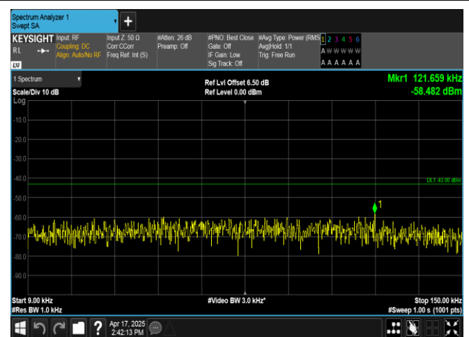
Band2-20MHz-QPSK-18700-1RB#99-0.009~0.15-PASS
