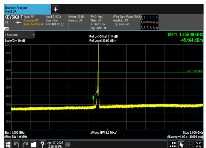
Band2-15MHz-16QAM-19125-1RB#74-1000~3000-PASS
