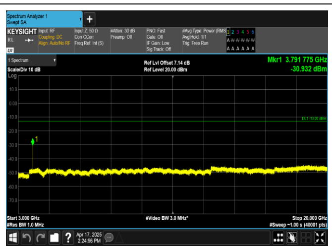
Band2-15MHz-16QAM-19125-1RB#0-3000~20000-PASS
