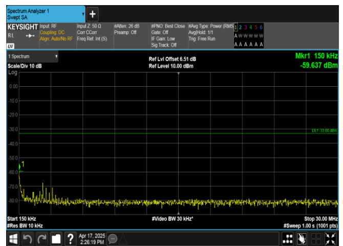
Band2-15MHz-16QAM-19125-1RB#74-0.15~30-PASS
