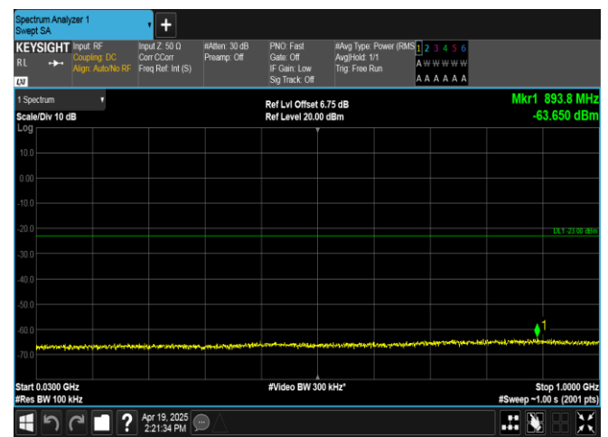
Band2-20MHz-QPSK-18900-100RB#0-30~1000-PASS
