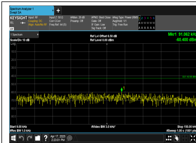
Band2-15MHz-QPSK-19125-1RB#0-0.009~0.15-PASS
