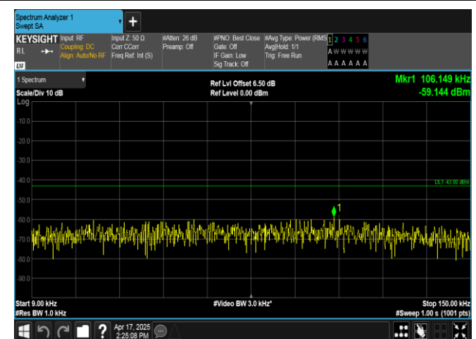
Band2-15MHz-QPSK-19125-1RB#74-0.009~0.15-PASS
