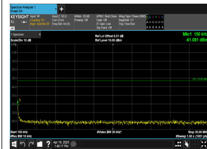
Band2-10MHz-16QAM-19150-50RB#0-0.15~30-PASS
