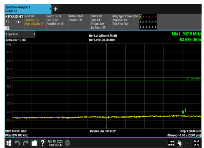
Band2-10MHz-16QAM-19150-50RB#0-30~1000-PASS
