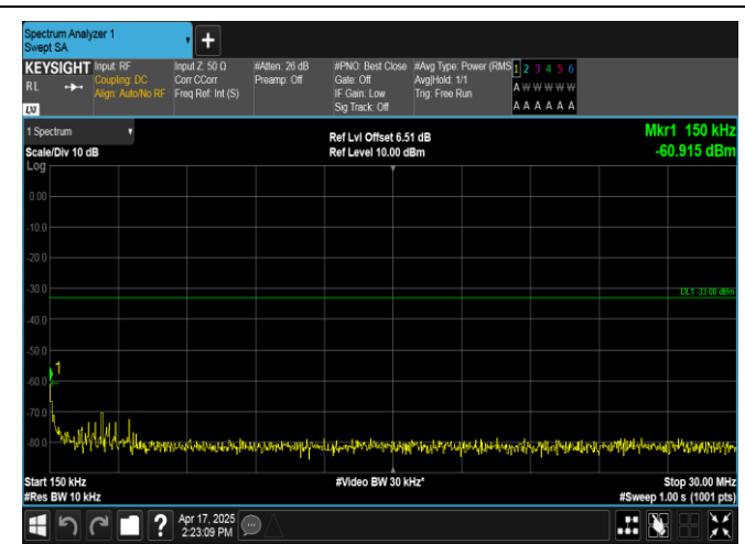
Band2-15MHz-QPSK-19125-1RB#0-0.15~30-PASS
