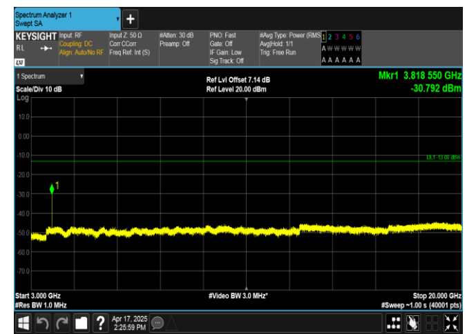
Band2-15MHz-QPSK-19125-1RB#74-3000~20000-PASS
