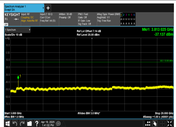
Band2-10MHz-16QAM-19150-50RB#0-3000~20000-PASS
