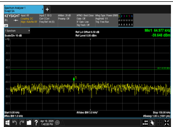
Band2-10MHz-16QAM-19150-50RB#0-0.009~0.15-PASS
