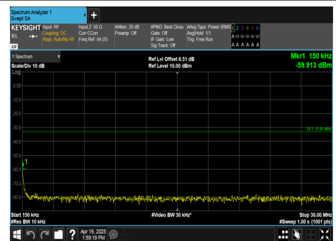
Band2-15MHz-QPSK-19125-75RB#0-0.15~30-PASS
