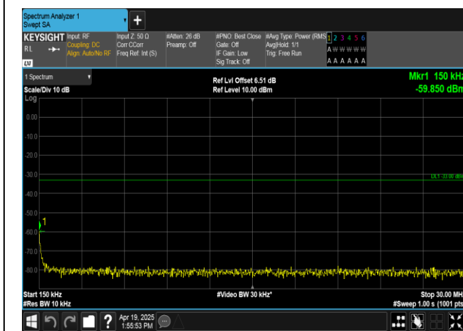
Band2-15MHz-16QAM-18675-75RB#0-0.15~30-PASS
