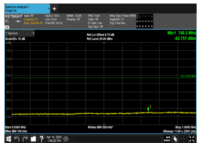
Band2-15MHz-16QAM-18675-75RB#0-30~1000-PASS
