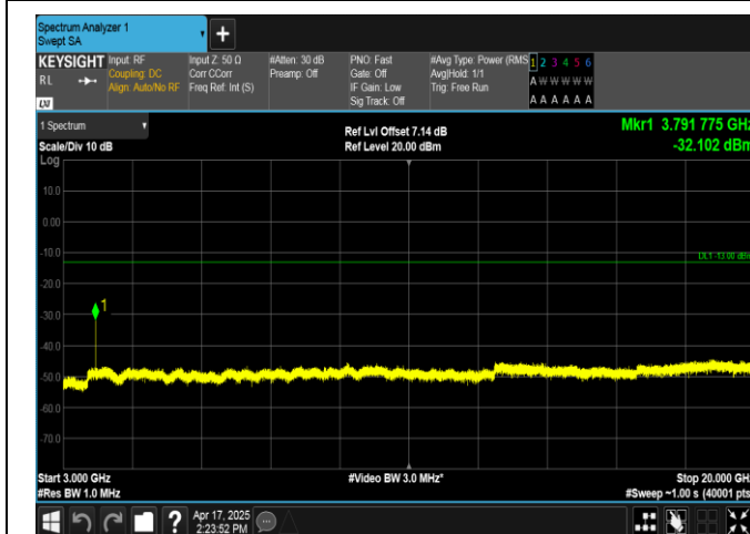
Band2-15MHz-QPSK-19125-1RB#0-3000~20000-PASS
