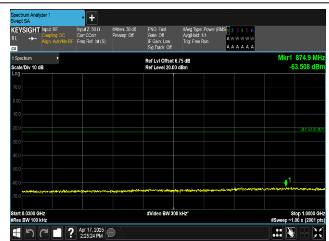
Band2-15MHz-QPSK-19125-1RB#74-30~1000-PASS
