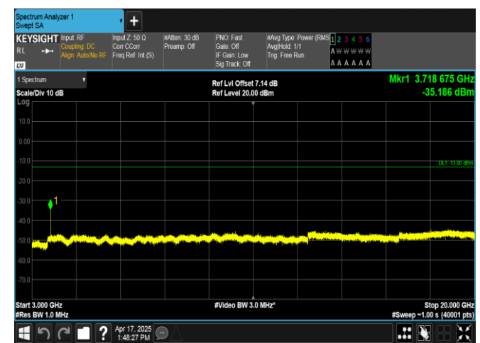
Band2-10MHz-QPSK-18650-1RB#49-3000~20000-PASS
