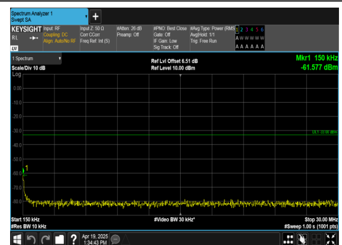
Band2-10MHz-QPSK-18650-50RB#0-0.15~30-PASS
