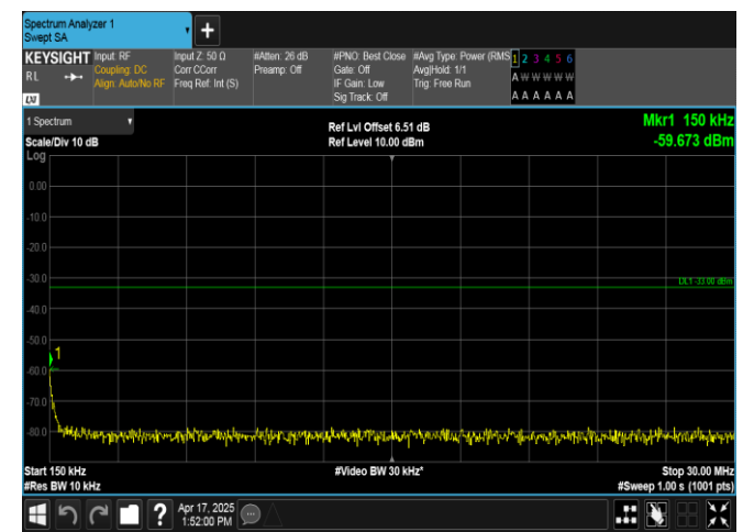
Band2-10MHz-QPSK-18900-1RB#49-0.15~30-PASS
