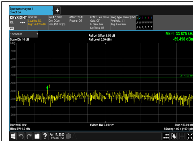
Band2-10MHz-QPSK-19150-1RB#0-0.009~0.15-PASS
