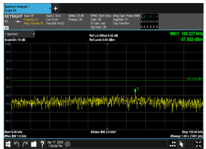
Band2-10MHz-16QAM-19150-1RB#0-0.009~0.15-PASS
