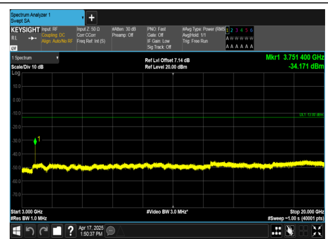
Band2-10MHz-QPSK-18900-1RB#0-3000~20000-PASS
