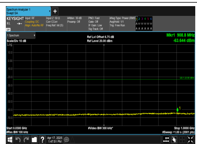
Band2-10MHz-QPSK-18650-1RB#49-30~1000-PASS
