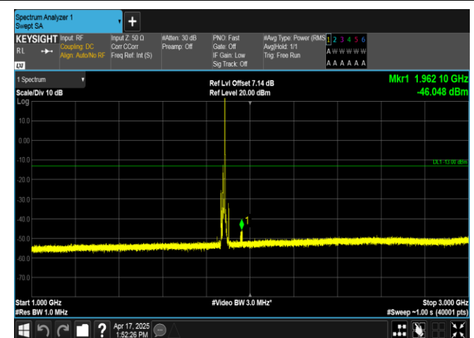
Band2-10MHz-QPSK-18900-1RB#49-1000~3000-PASS
