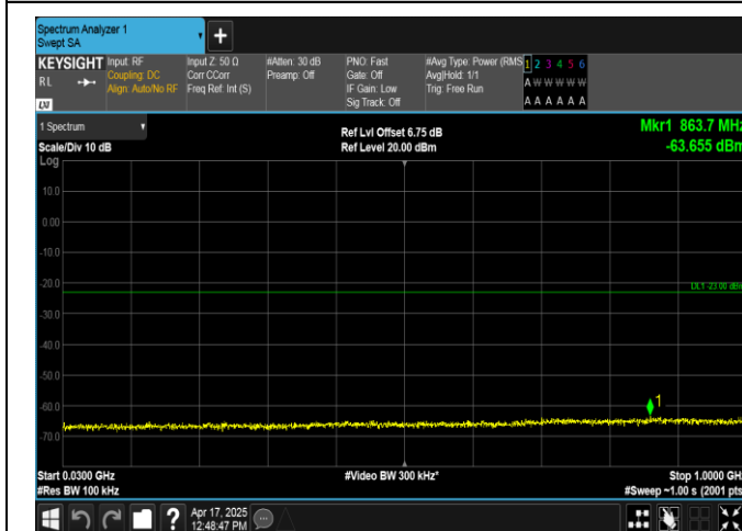
Band2-5MHz-16QAM-18625-1RB#24-30~1000-PASS
