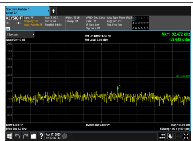
Band2-5MHz-16QAM-18625-25RB#0-0.009~0.15-PASS
