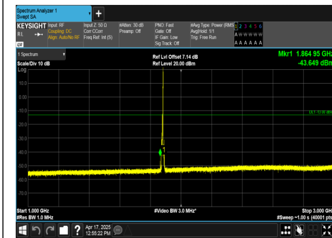
Band2-5MHz-16QAM-18900-1RB#24-1000~3000-PASS
