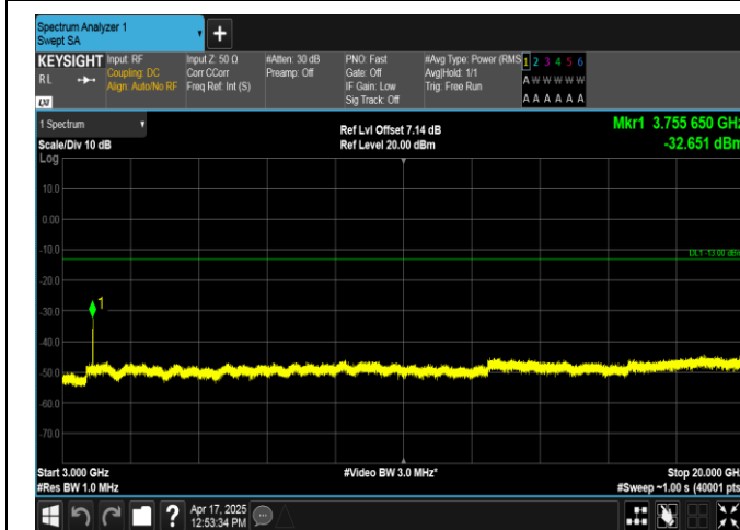
Band2-5MHz-16QAM-18900-1RB#0-3000~20000-PASS
