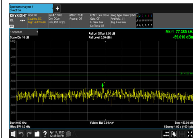
Band2-5MHz-16QAM-18625-1RB#24-0.009~0.15-PASS
