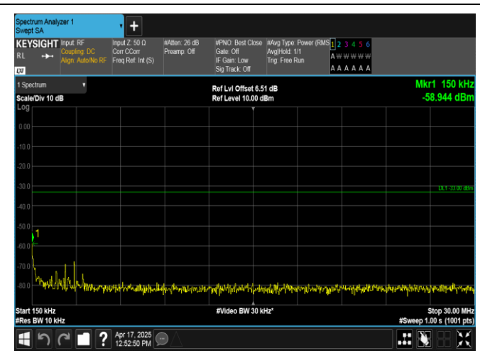
Band2-5MHz-16QAM-18900-1RB#0-0.15~30-PASS
