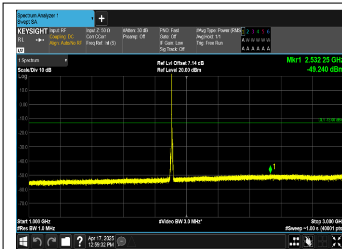
Band2-5MHz-16QAM-19175-1RB#0-1000~3000-PASS
