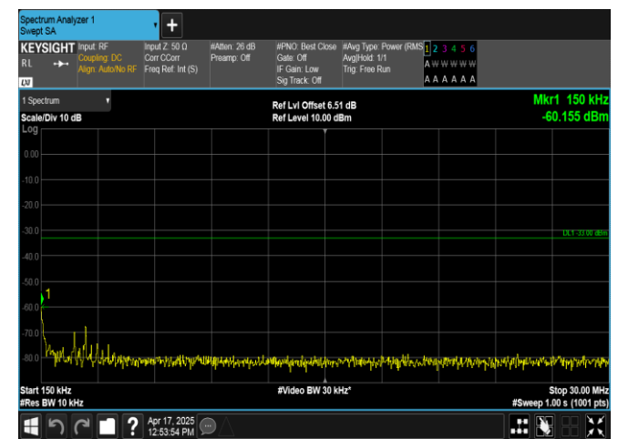
Band2-5MHz-QPSK-18900-1RB#24-0.15~30-PASS
