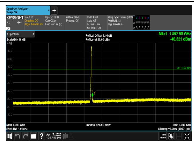
Band2-5MHz-16QAM-18900-25RB#0-1000~3000-PASS
