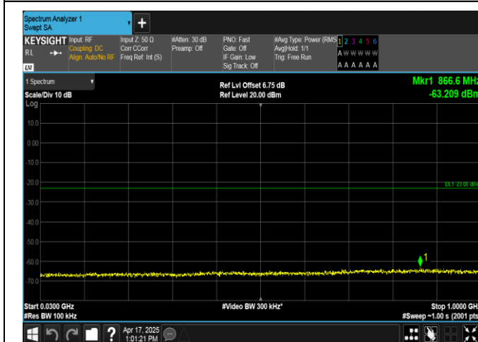
Band2-5MHz-16QAM-19175-1RB#24-30~1000-PASS
