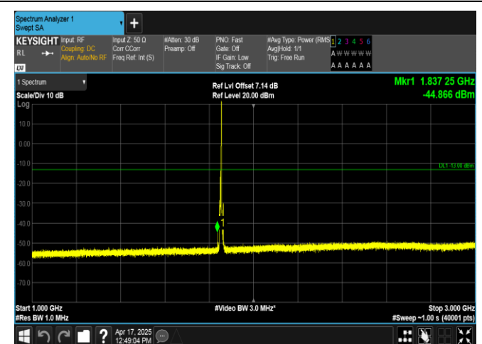
Band2-5MHz-16QAM-18625-1RB#24-1000~3000-PASS
