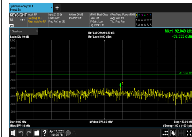
Band2-5MHz-16QAM-19175-1RB#24-0.009~0.15-PASS
