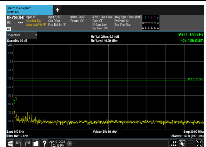
Band2-5MHz-QPSK-19175-25RB#0-0.15~30-PASS
