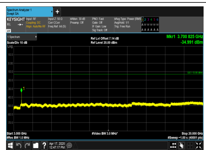
Band2-5MHz-16QAM-18625-1RB#0-3000~20000-PASS
