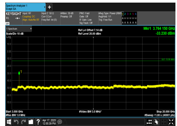
Band2-5MHz-16QAM-18900-1RB#24-3000~20000-PASS
