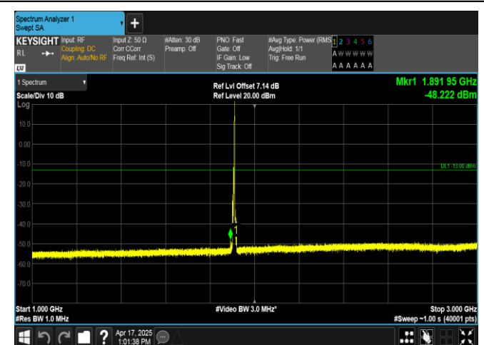
Band2-5MHz-16QAM-19175-1RB#24-1000~3000-PASS
