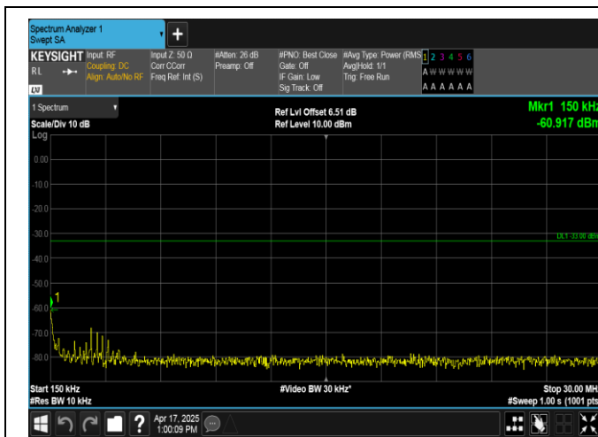
Band2-5MHz-QPSK-19175-1RB#24-0.15~30-PASS
