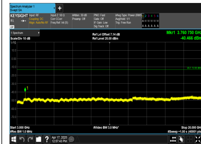
Band2-5MHz-16QAM-18900-25RB#0-3000~20000-PASS
