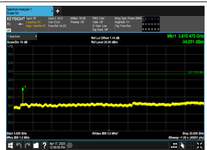
Band2-5MHz-16QAM-19175-1RB#0-3000~20000-PASS
