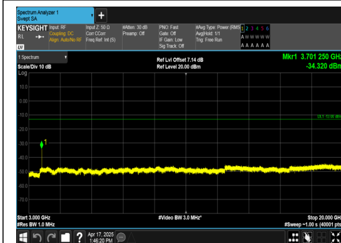
Band2-10MHz-QPSK-18650-1RB#0-3000~20000-PASS
