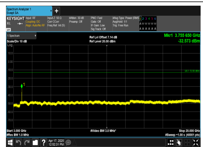
Band2-5MHz-QPSK-18900-1RB#0-3000~20000-PASS
