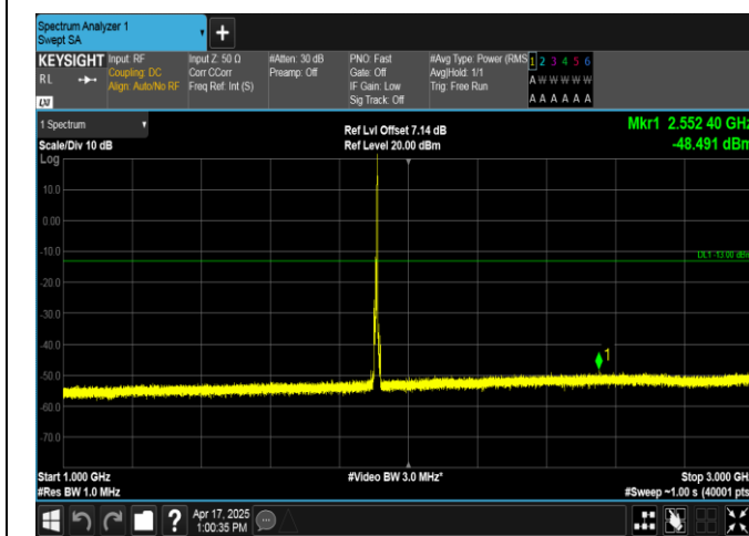
Band2-5MHz-QPSK-19175-1RB#24-1000~3000-PASS
