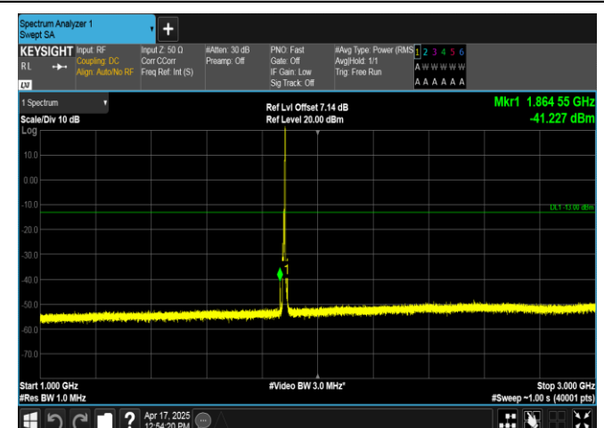
Band2-5MHz-QPSK-18900-1RB#24-1000~3000-PASS
