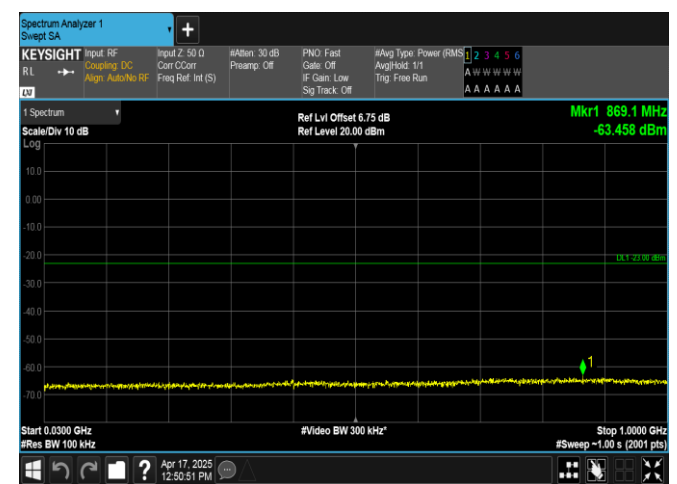
Band2-5MHz-16QAM-18625-25RB#0-30~1000-PASS
