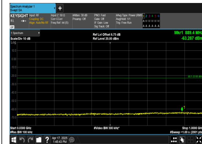
Band2-10MHz-QPSK-18650-1RB#0-30~1000-PASS
