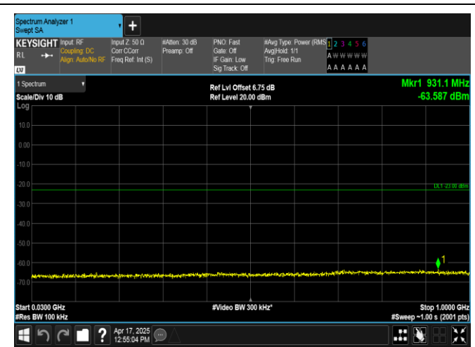
Band2-5MHz-16QAM-18900-1RB#24-30~1000-PASS
