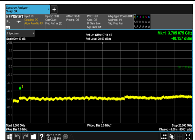
Band2-5MHz-16QAM-18625-25RB#0-3000~20000-PASS
