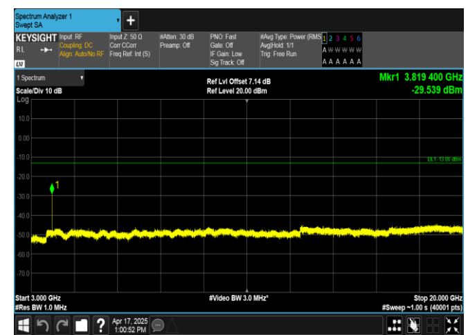
Band2-5MHz-QPSK-19175-1RB#24-3000~20000-PASS
