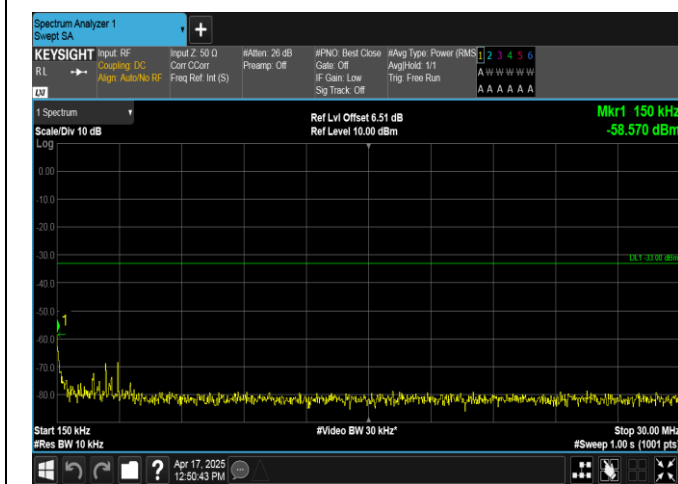
Band2-5MHz-16QAM-18625-25RB#0-0.15~30-PASS
