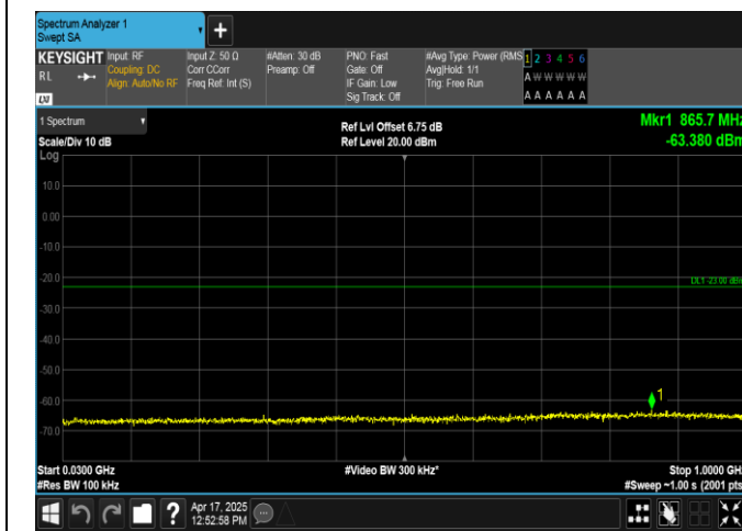
Band2-5MHz-16QAM-18900-1RB#0-30~1000-PASS
