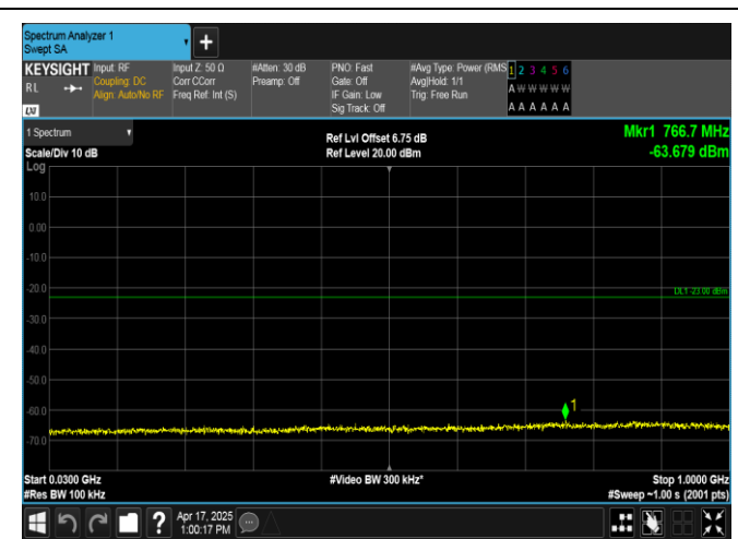
Band2-5MHz-QPSK-19175-1RB#24-30~1000-PASS
