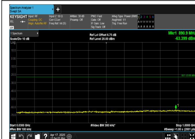
Band2-5MHz-QPSK-18900-1RB#24-30~1000-PASS
