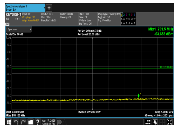
Band2-5MHz-16QAM-19175-1RB#0-30~1000-PASS
