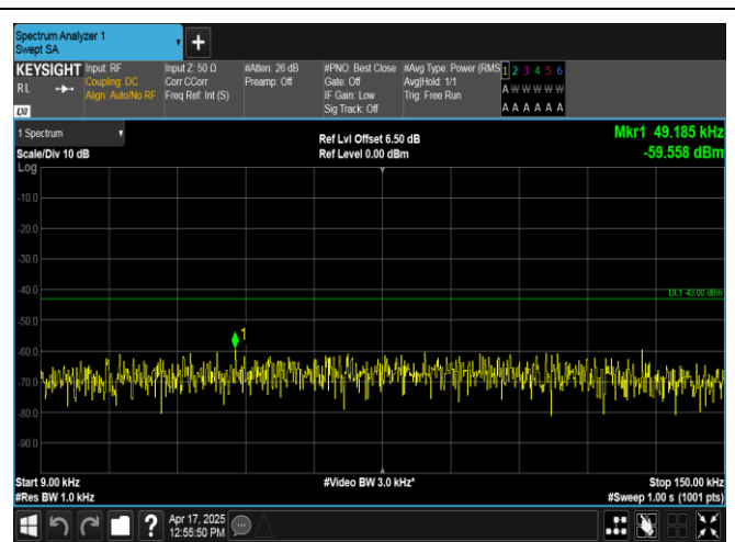
Band2-5MHz-QPSK-18900-25RB#0-0.009~0.15-PASS
