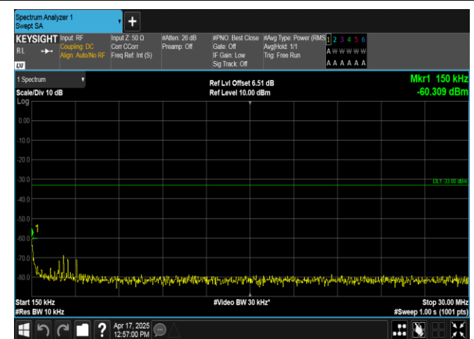
Band2-5MHz-16QAM-18900-25RB#0-0.15~30-PASS
