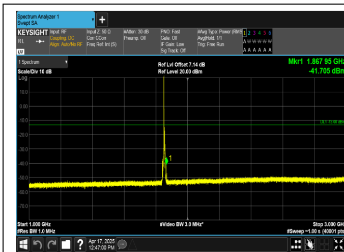
Band2-5MHz-16QAM-18625-1RB#0-1000~3000-PASS
