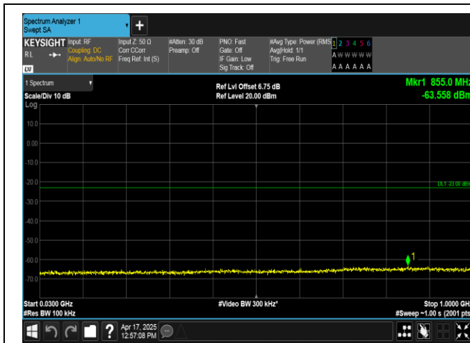
Band2-5MHz-16QAM-18900-25RB#0-30~1000-PASS
