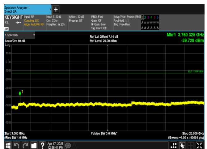
Band2-5MHz-QPSK-18900-25RB#0-3000~20000-PASS
