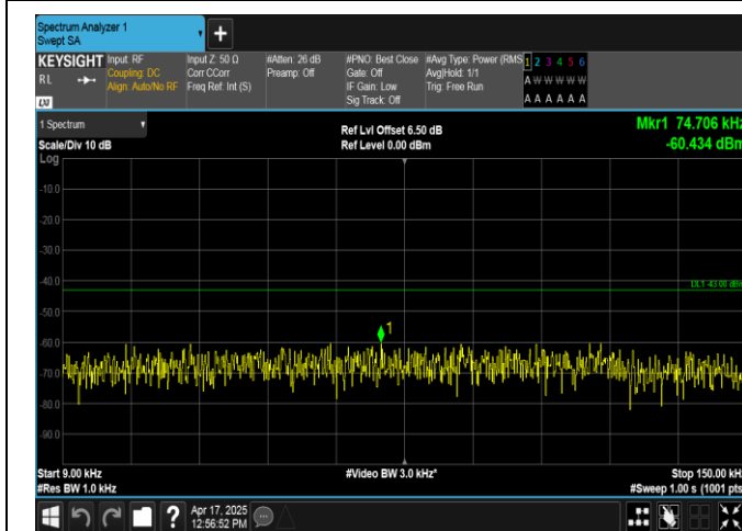
Band2-5MHz-16QAM-18900-25RB#0-0.009~0.15-PASS
