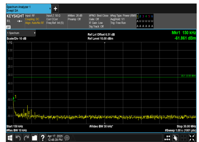
Band2-5MHz-16QAM-18625-1RB#24-0.15~30-PASS
