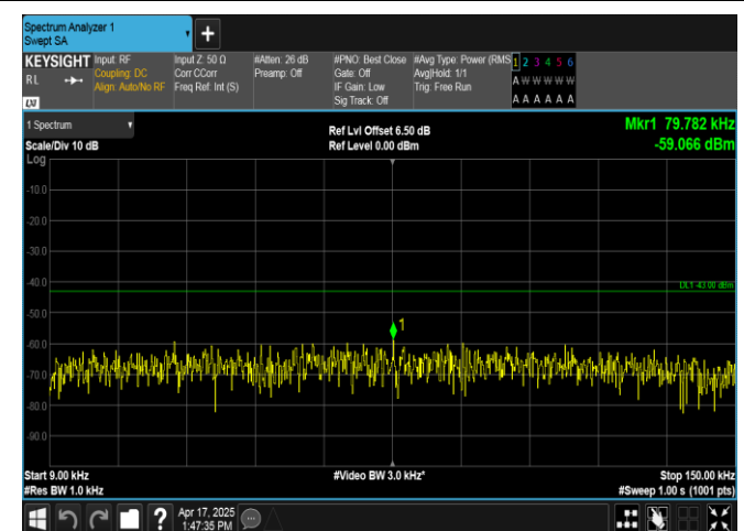
Band2-10MHz-QPSK-18650-1RB#49-0.009~0.15-PASS
