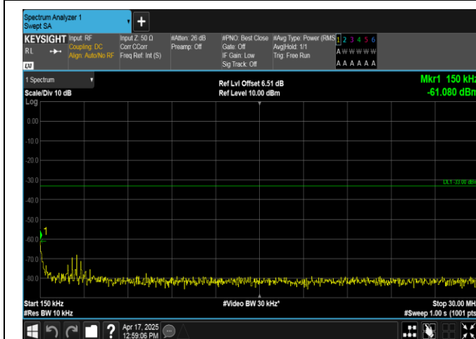
Band2-5MHz-16QAM-19175-1RB#0-0.15~30-PASS
