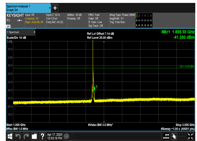
Band2-5MHz-16QAM-18900-1RB#0-1000~3000-PASS
