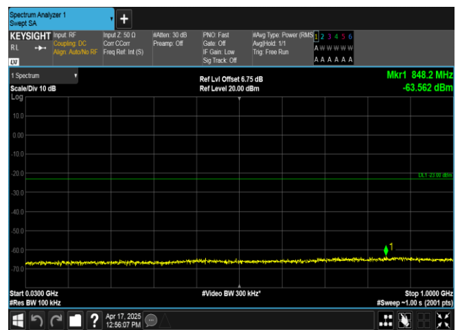
Band2-5MHz-QPSK-18900-25RB#0-30~1000-PASS
