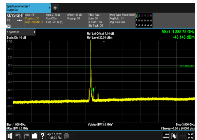
Band2-10MHz-QPSK-18650-1RB#0-1000~3000-PASS
