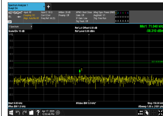
Band2-5MHz-QPSK-18900-1RB#24-0.009~0.15-PASS
