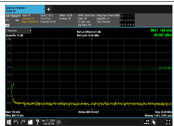
Band2-10MHz-QPSK-18650-1RB#0-0.15~30-PASS
