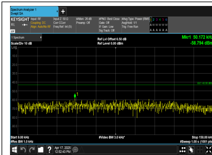
Band2-5MHz-16QAM-18900-1RB#0-0.009~0.15-PASS
