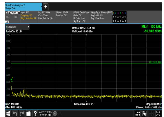
Band2-5MHz-16QAM-19175-1RB#24-0.15~30-PASS
