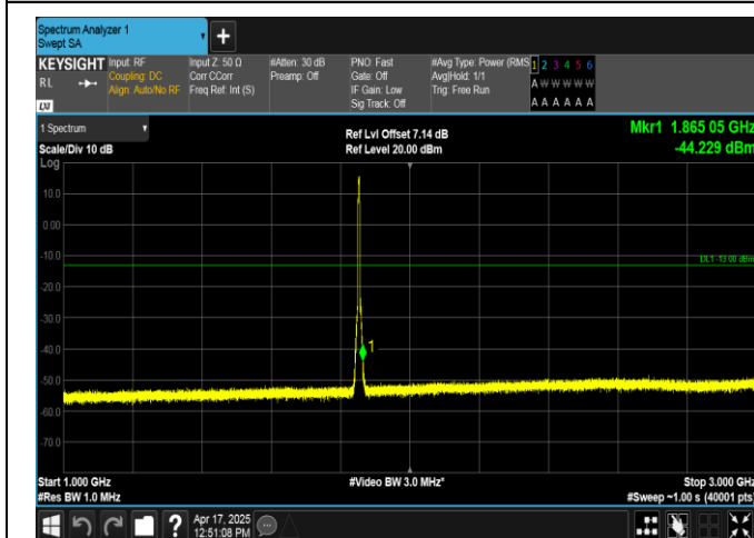
Band2-5MHz-16QAM-18625-25RB#0-1000~3000-PASS
