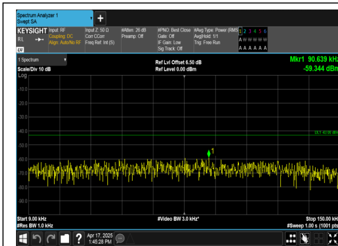
Band2-10MHz-QPSK-18650-1RB#0-0.009~0.15-PASS
