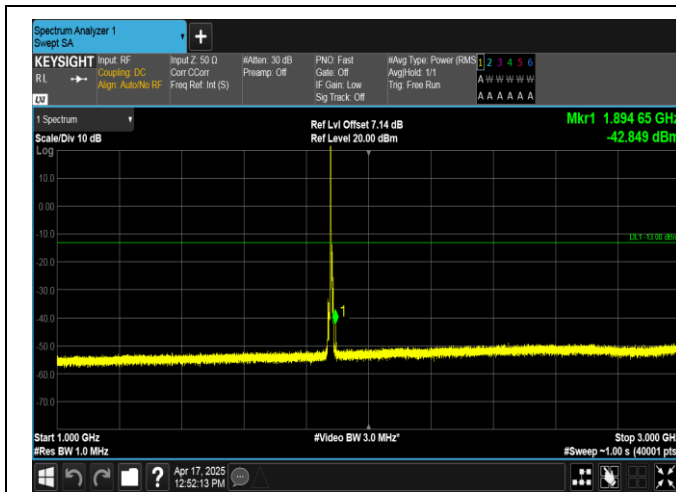
Band2-5MHz-QPSK-18900-1RB#0-1000~3000-PASS
