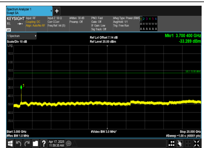
Band2-3MHz-16QAM-18615-1RB#0-3000~20000-PASS
