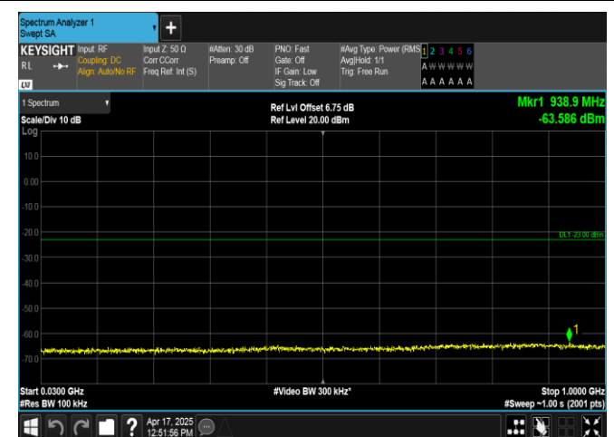
Band2-5MHz-QPSK-18900-1RB#0-30~1000-PASS
