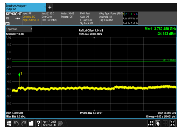
Band2-3MHz-16QAM-18900-1RB#14-3000~20000-PASS
