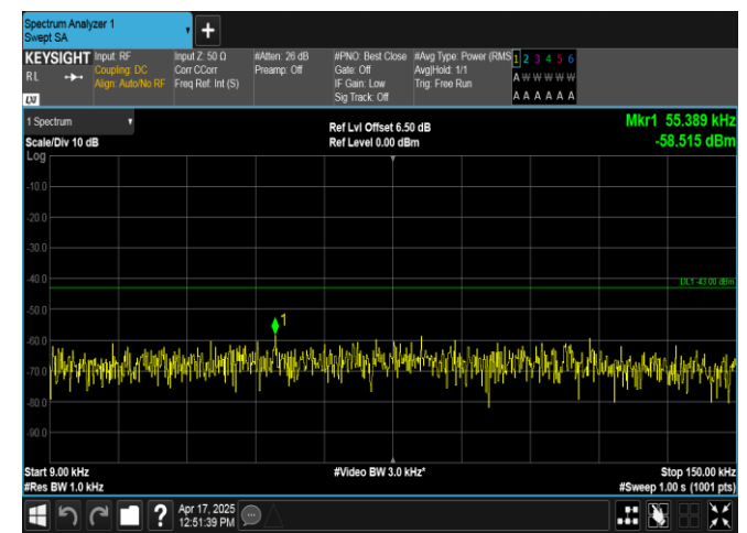
Band2-5MHz-QPSK-18900-1RB#0-0.009~0.15-PASS
