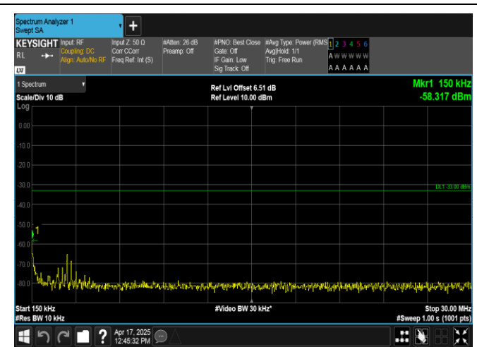
Band2-5MHz-QPSK-18625-1RB#0-0.15~30-PASS
