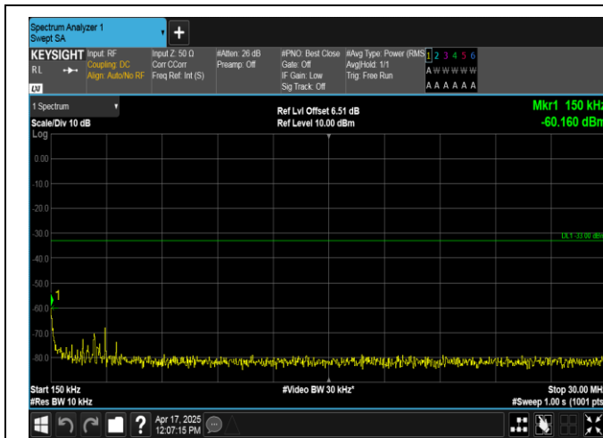
Band2-3MHz-16QAM-18900-1RB#14-0.15~30-PASS
