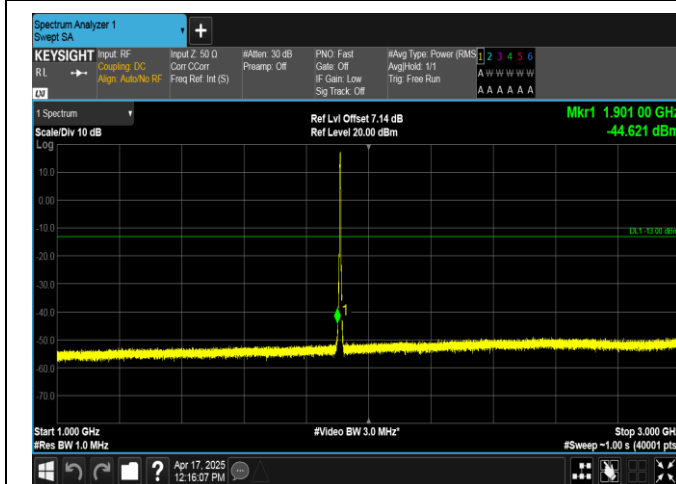
Band2-3MHz-16QAM-19185-15RB#0-1000~3000-PASS
