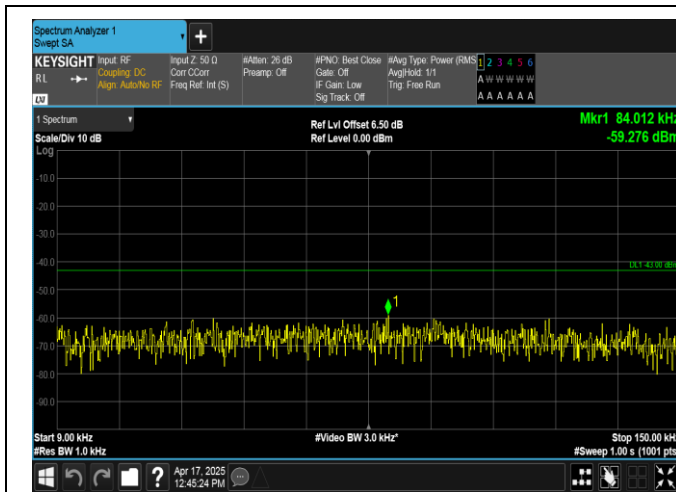
Band2-5MHz-QPSK-18625-1RB#0-0.009~0.15-PASS
