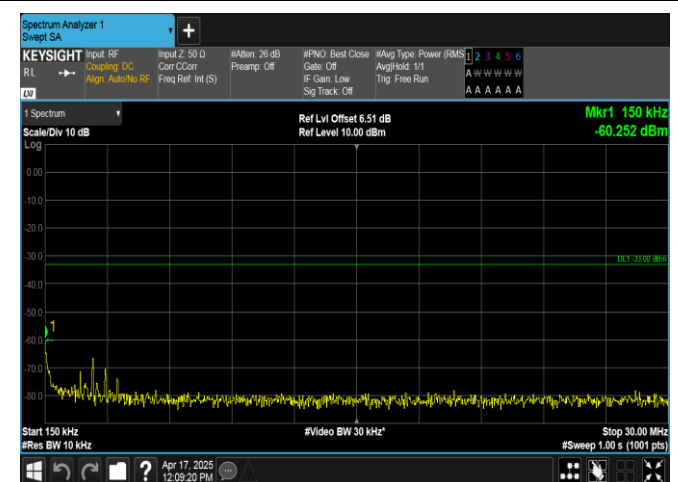
Band2-3MHz-16QAM-18900-15RB#0-0.15~30-PASS
