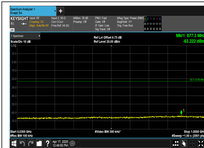
Band2-5MHz-QPSK-18625-25RB#0-30~1000-PASS
