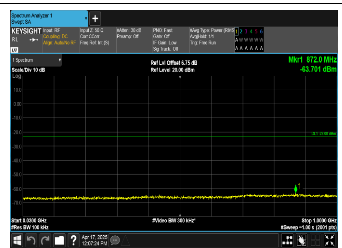
Band2-3MHz-16QAM-18900-1RB#14-30~1000-PASS
