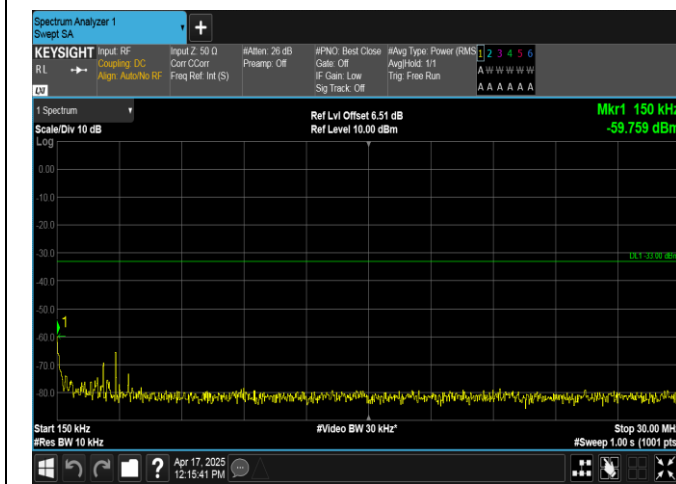
Band2-3MHz-16QAM-19185-15RB#0-0.15~30-PASS
