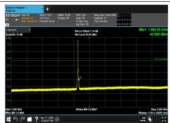
Band2-5MHz-QPSK-18625-25RB#0-1000~3000-PASS
