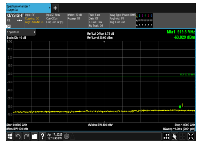
Band2-3MHz-16QAM-19185-15RB#0-30~1000-PASS
