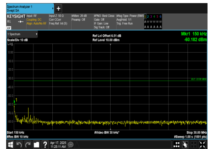
Band2-1.4MHz-16QAM-19193-1RB#5-0.15~30-PASS
