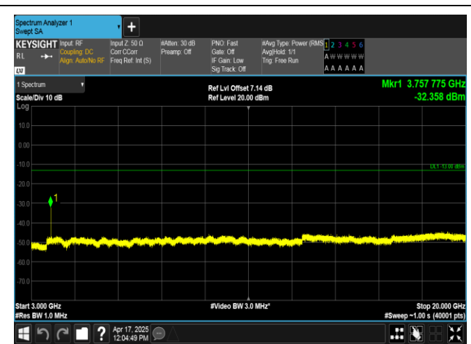
Band2-3MHz-QPSK-18900-1RB#0-3000~20000-PASS
