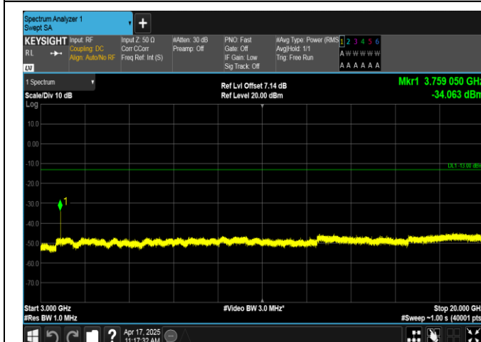
Band2-1.4MHz-16QAM-18900-1RB#0-3000~20000-PASS
