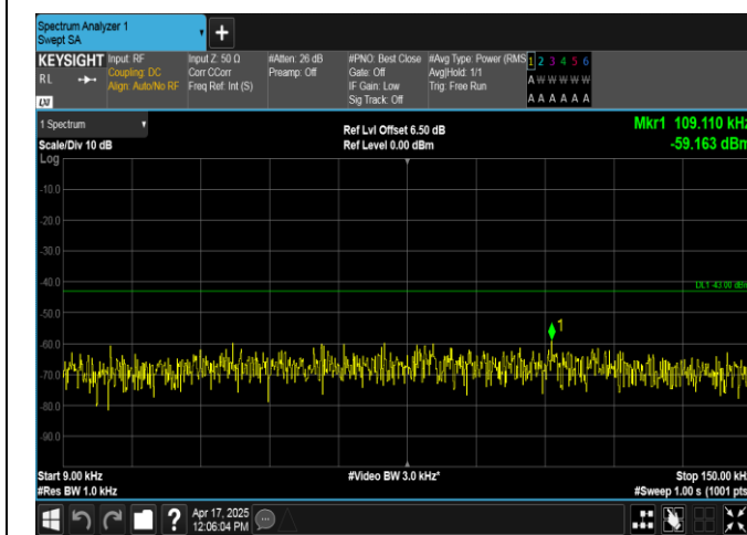
Band2-3MHz-QPSK-18900-1RB#14-0.009~0.15-PASS
