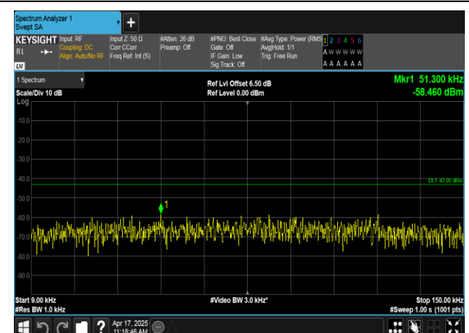
Band2-1.4MHz-16QAM-18900-1RB#5-0.009~0.15-PASS
