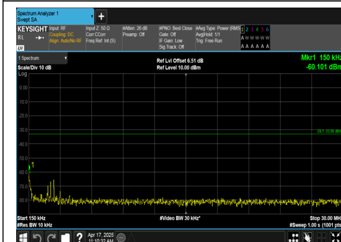
Band2-1.4MHz-16QAM-18607-1RB#0-0.15~30-PASS
