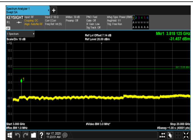
Band2-1.4MHz-16QAM-19193-1RB#0-3000~20000-PASS
