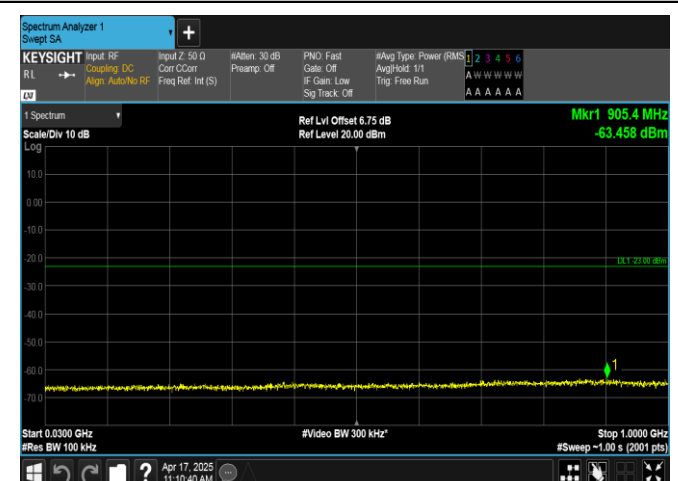
Band2-1.4MHz-16QAM-18607-1RB#0-30~1000-PASS
