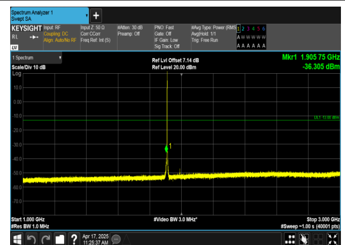
Band2-1.4MHz-16QAM-19193-1RB#5-1000~3000-PASS
