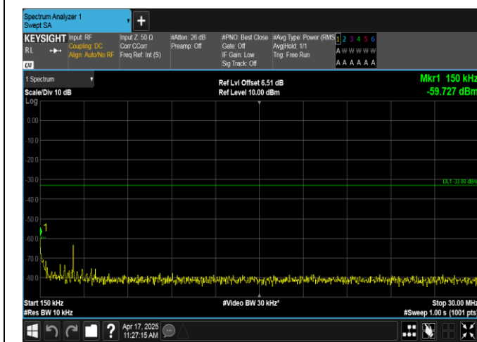
Band2-1.4MHz-16QAM-19193-6RB#0-0.15~30-PASS
