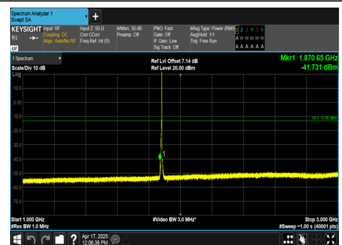
Band2-3MHz-QPSK-18900-1RB#14-1000~3000-PASS
