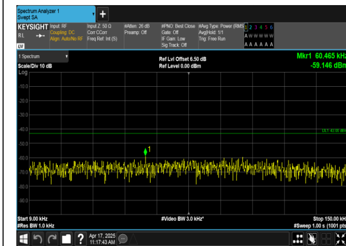
Band2-1.4MHz-QPSK-18900-1RB#5-0.009~0.15-PASS
