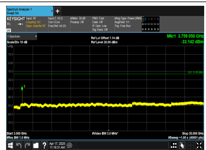
Band2-1.4MHz-QPSK-18900-1RB#0-3000~20000-PASS
