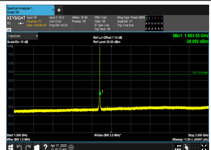
Band2-1.4MHz-QPSK-18900-1RB#5-1000~3000-PASS
