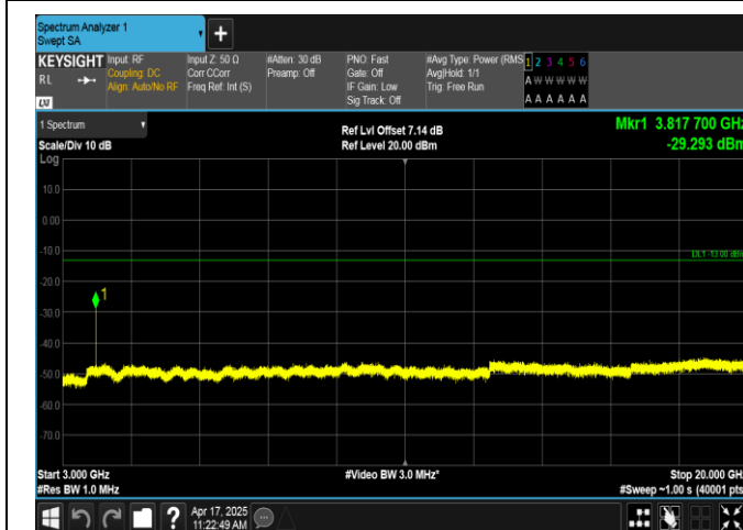
Band2-1.4MHz-QPSK-19193-1RB#0-3000~20000-PASS
