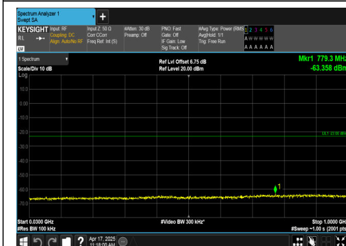
Band2-1.4MHz-QPSK-18900-1RB#5-30~1000-PASS
