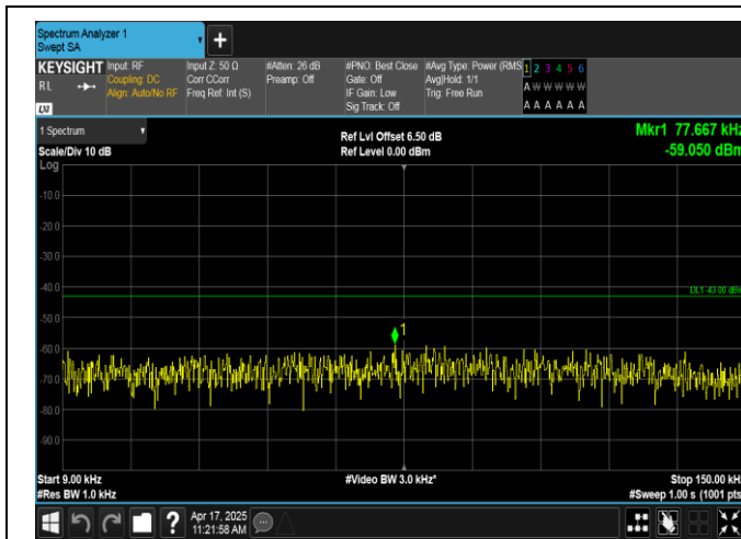
Band2-1.4MHz-QPSK-19193-1RB#0-0.009~0.15-PASS
