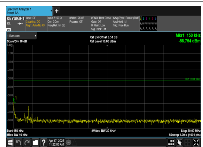
Band2-1.4MHz-QPSK-19193-1RB#0-0.15~30-PASS
