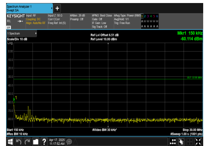
Band2-1.4MHz-QPSK-18900-1RB#5-0.15~30-PASS
