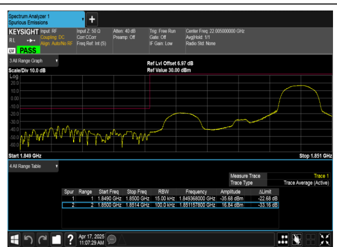
Band2-1.4MHz-16QAM-18607-1RB#5-PASS
