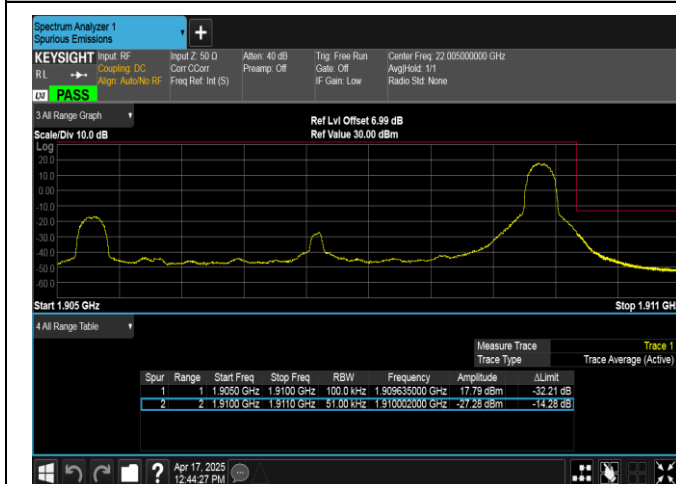
Band2-5MHz-QPSK-19175-1RB#24-PASS
