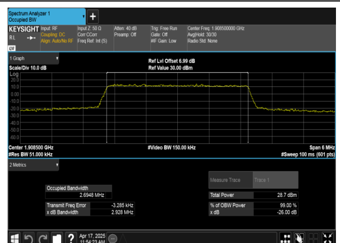
Band2-3MHz-16QAM-19185-15RB#0-PASS
